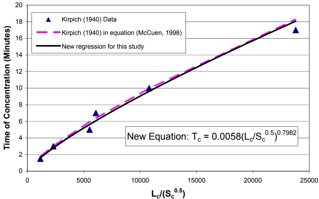
Figure 3.3. Kirpich's data and regression equation comparison (after Kirpich, 1940).
