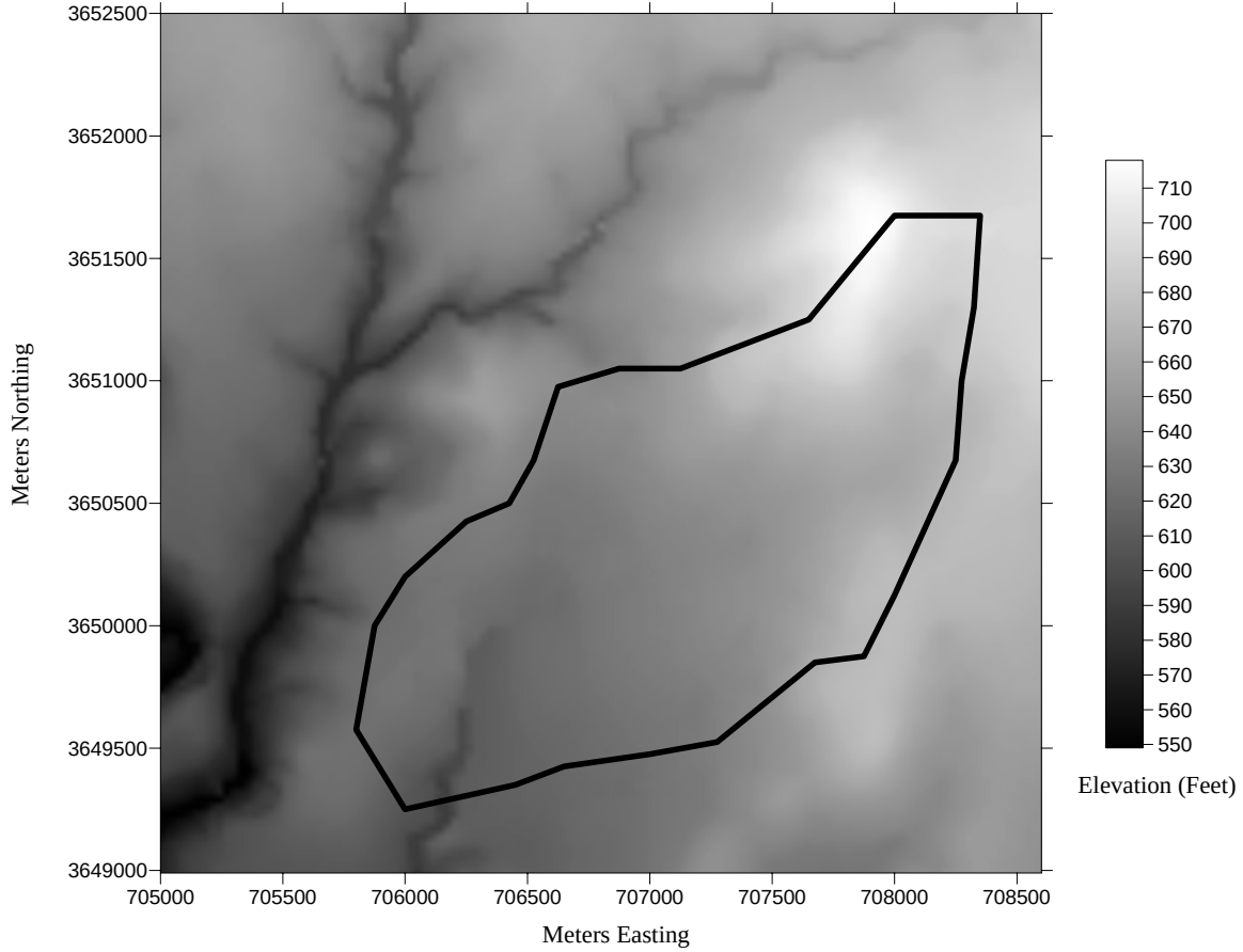
Figure A.8 Rush Branch – Extracted Area.
