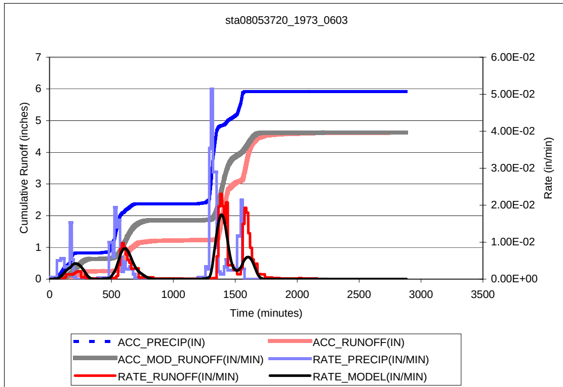
Figure A.13 Ash Creek response under rainfall on 06-03-1973.
