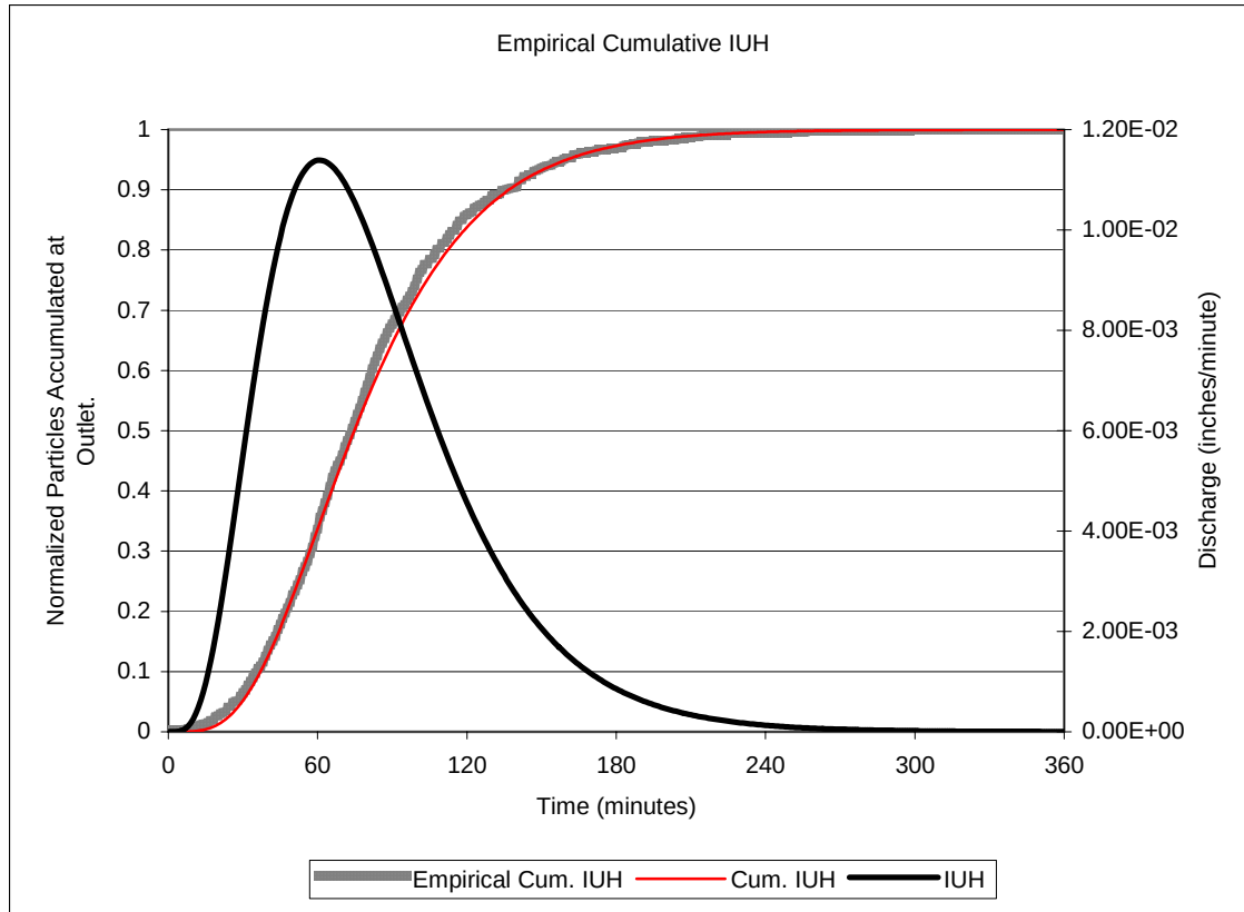
Figure A.9 Empirical cumulative and fitted IUH for Rush Branch.
