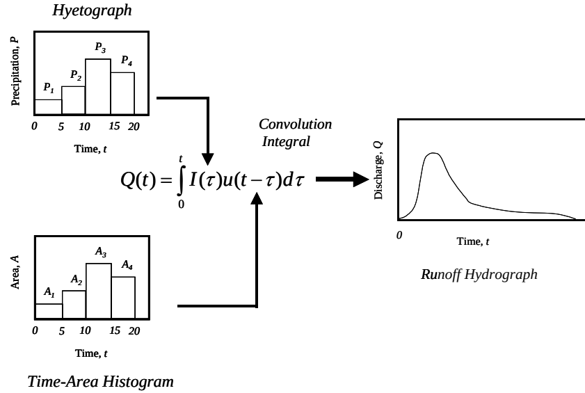
Figure A.3 Time-area-convolution to produce a runoff hydrograph.
