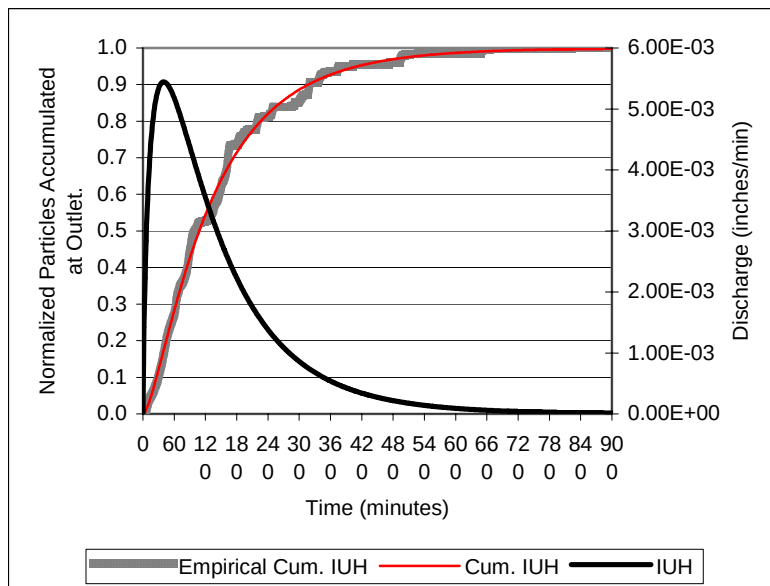
Figure A.17 Empirical and fitted IUH for Slaughter Creek.
