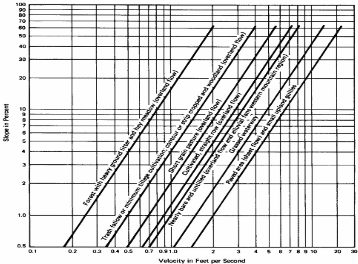
Figure 3.2. Velocities for overland flow method of estimating T_c (from McCuen, 1998).
