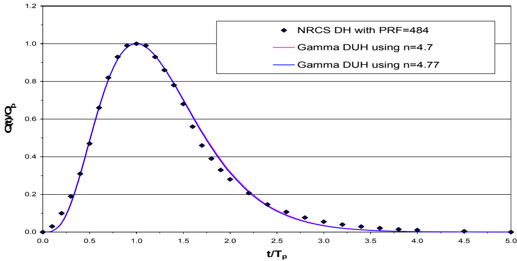
Figure 3.6. Comparison of NRCS UH (stars) with Gamma UH approximation (lines).
