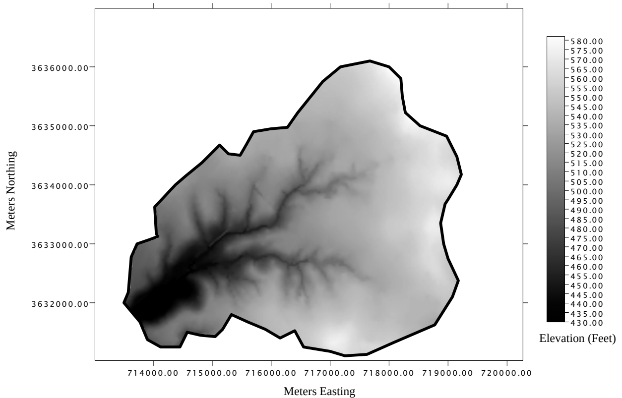
Figure A.6 Ash Creek watershed - manual boundary delineation.
