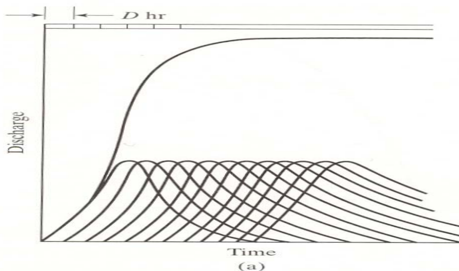
Figure 2.2. S-hydrograph developed by lagging of known D hour UH for infinite times (from Viessman and Lewis, 2002).
