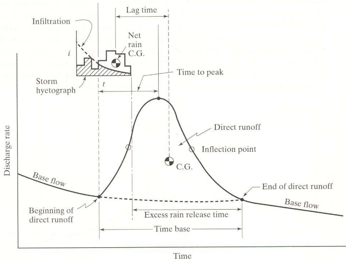
Figure 2.1. Hydrograph time relations and timing parameters of hydrographs (from Viessman and Lewis, 2002).
