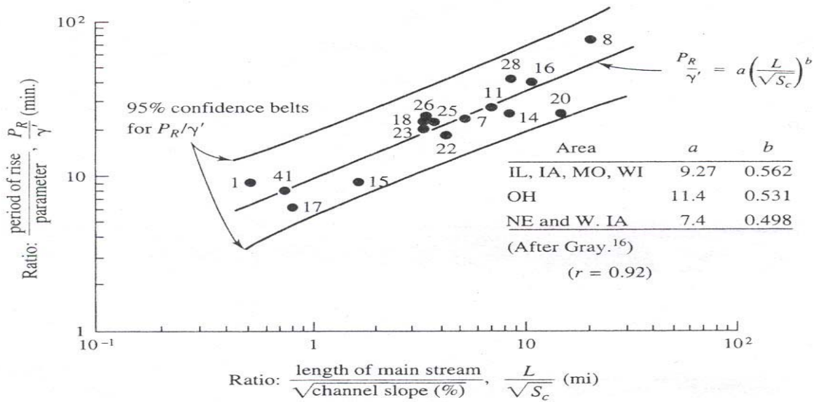
Figure 3.4. Relation of storage factor, P_R/\gamma' , and watershed parameter, L/\sqrt{S_c} , for watersheds in Nebraska, Iowa, Missouri, Illinois, and Wisconsin (after Gray, 1961).
