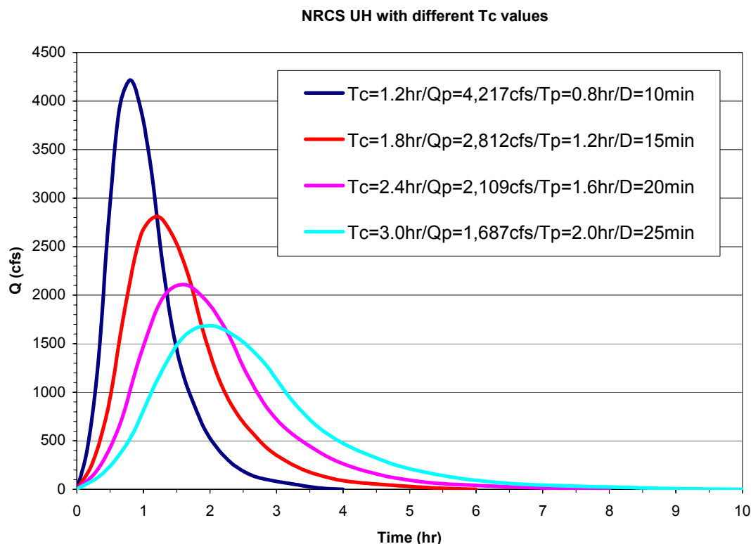
Figure 3.1. Example unit hydrographs developed from NRCS DUH with four T_c values.
