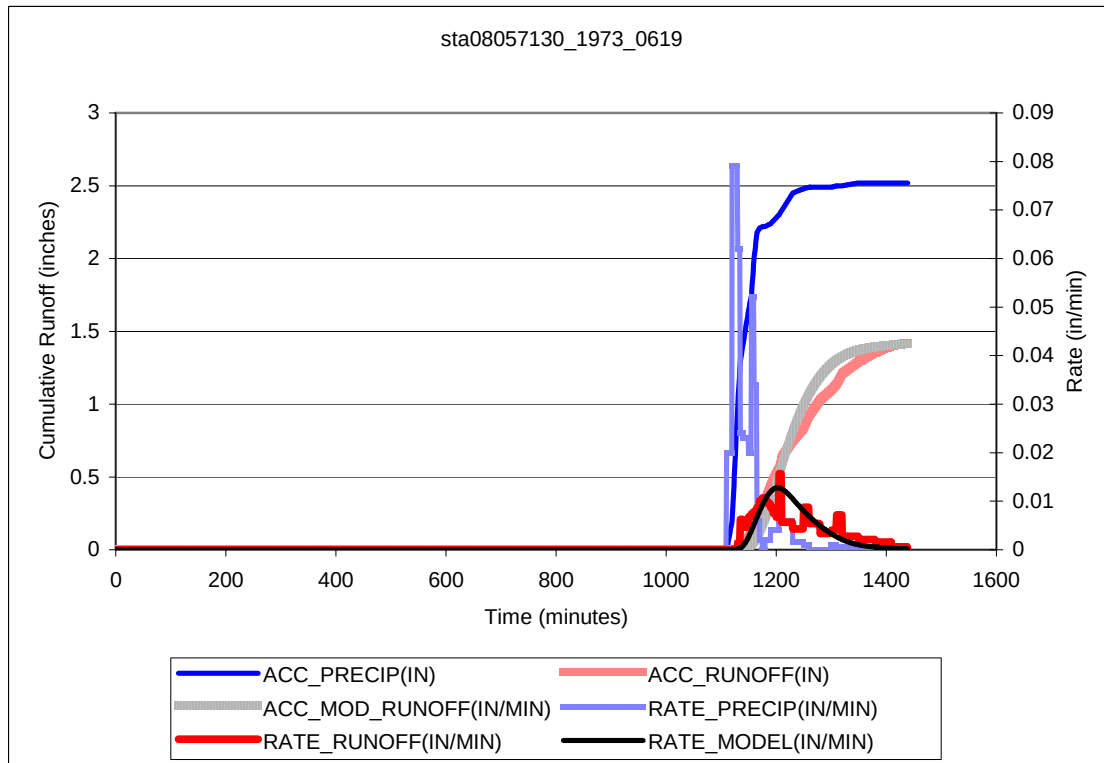
Figure A.10 Rush Branch response under rainfall on 06-19-1973.
