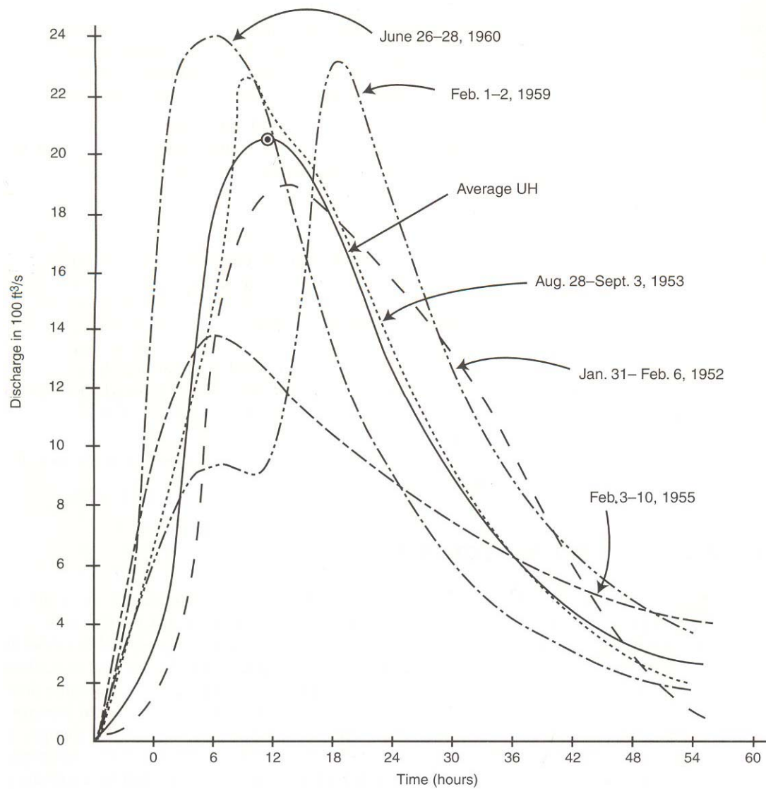
Figure 1.3. Five fitted unit hydrographs from five storm events and watershed-average UH on White Oak Bayou, Texas (from McCuen, 1998).
