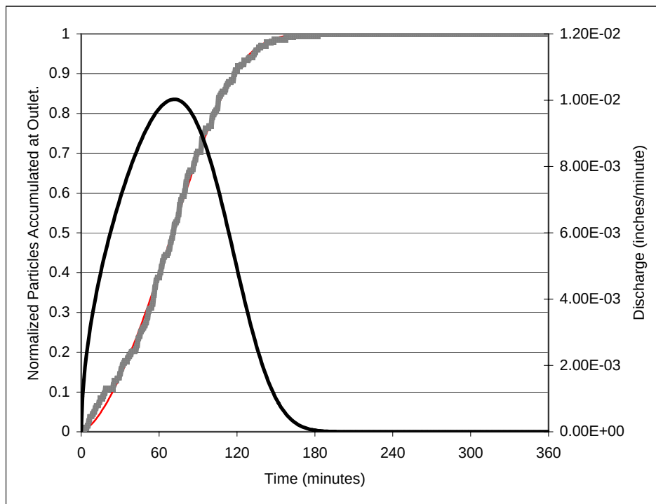
Figure A.12. Empirical and fitted IUH for Ash Creek.
