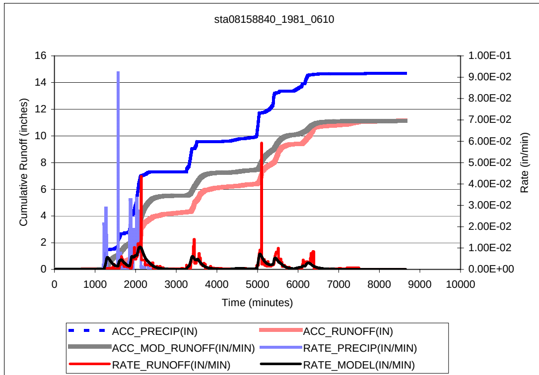
Figure A.18 Slaughter Creek response under rainfall on 06-10-1981.
