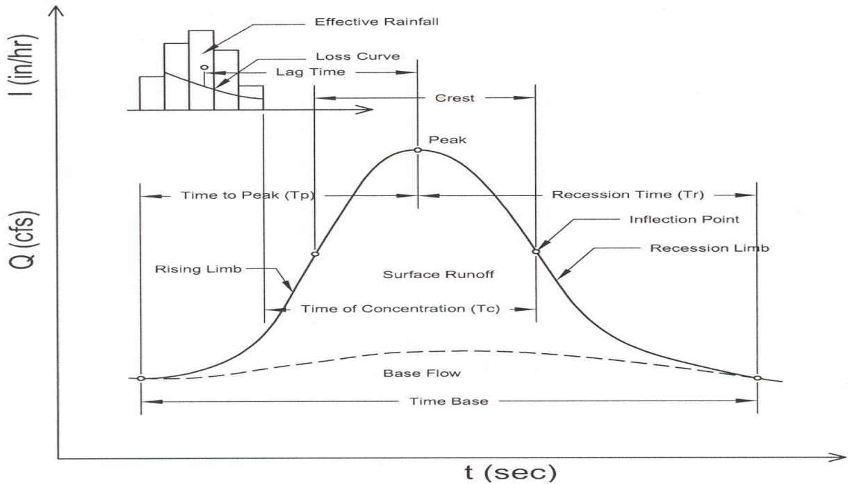
Figure 1.2. Schematic streamflow hydrograph including typical timing parameters and a rainfall hyetograph.
