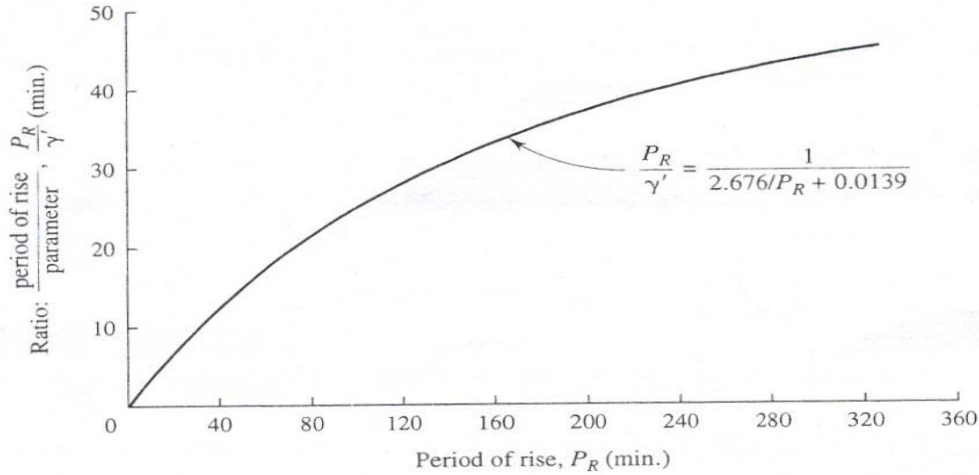
Figure 3.5. Relation for storage factor, P_R / \gamma' , and period of rise P_R (after Gray, 1961).
