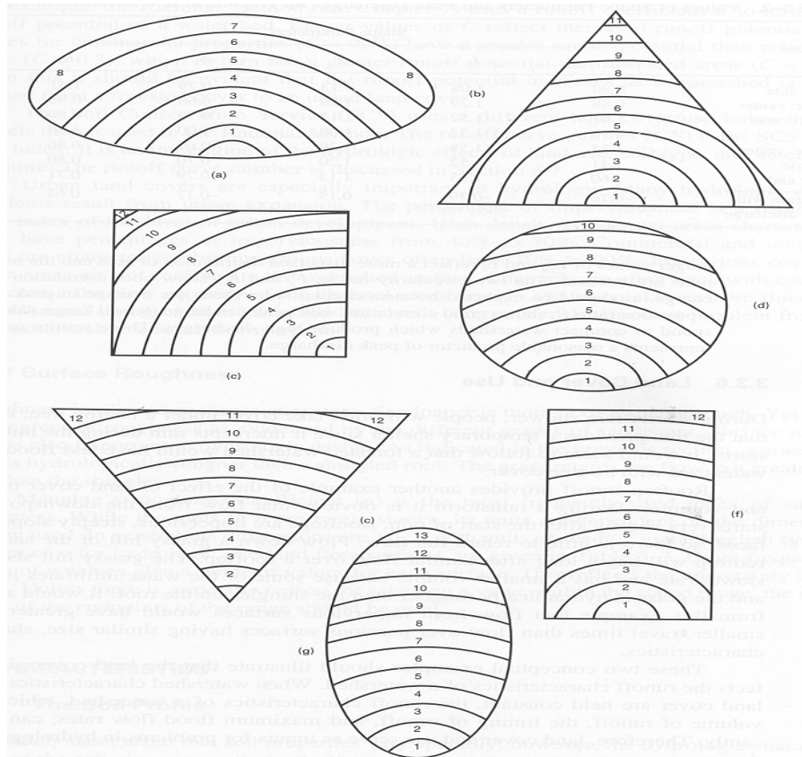
Figure 4.3. Hypothetical watersheds (a) ellipse: side; (b) triangle: center; (c) square: corner; (d) circle; (e) triangle: vertex; (f) rectangle; (g) ellipse: end (McCuen, 1998).
