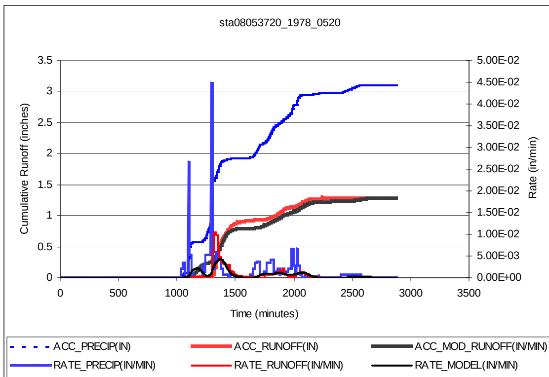
Figure A.14 Ash Creek response under rainfall on 05-20-1978.
