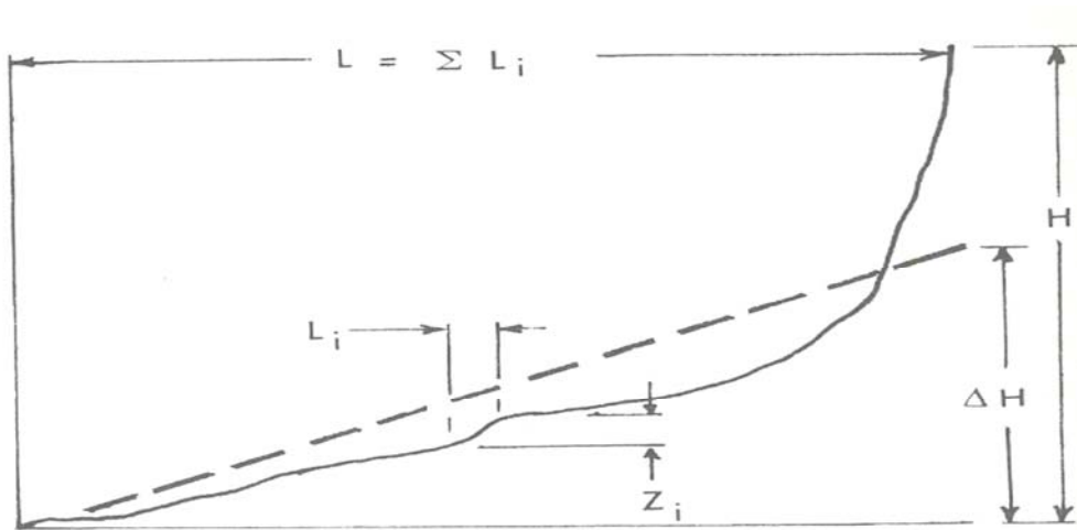
Figure 4.2. Definition of average main channel slope (from Schulz and Lopez, 1974).
