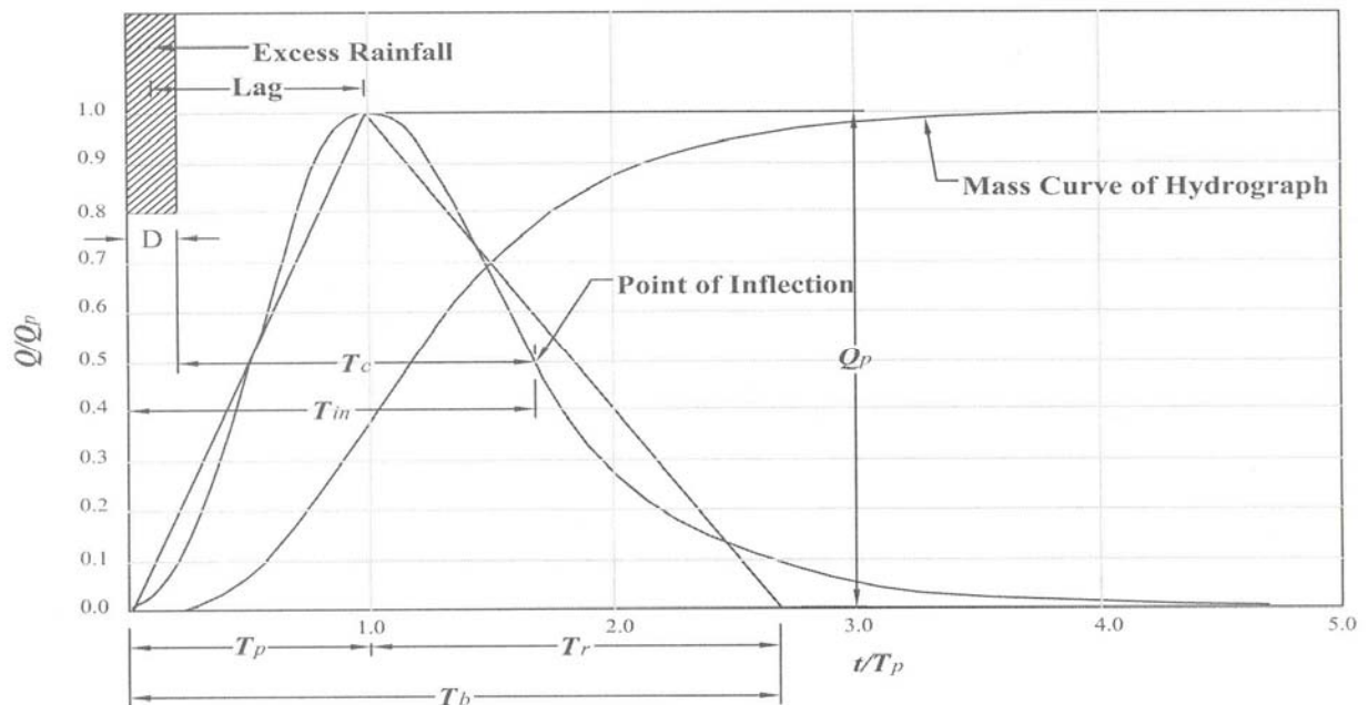
Figure 1.1. NRCS synthetic unit hydrographs including dimensionless unit hydrograph and triangular unit hydrograph.
