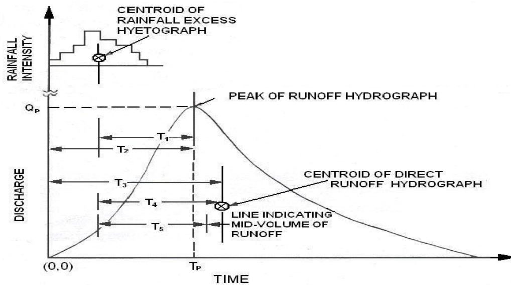
Figure 2.3. Different lag time definitions (after Rao and Delleur, 1973).
