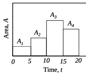
Figure A.2 Time-area diagram.
