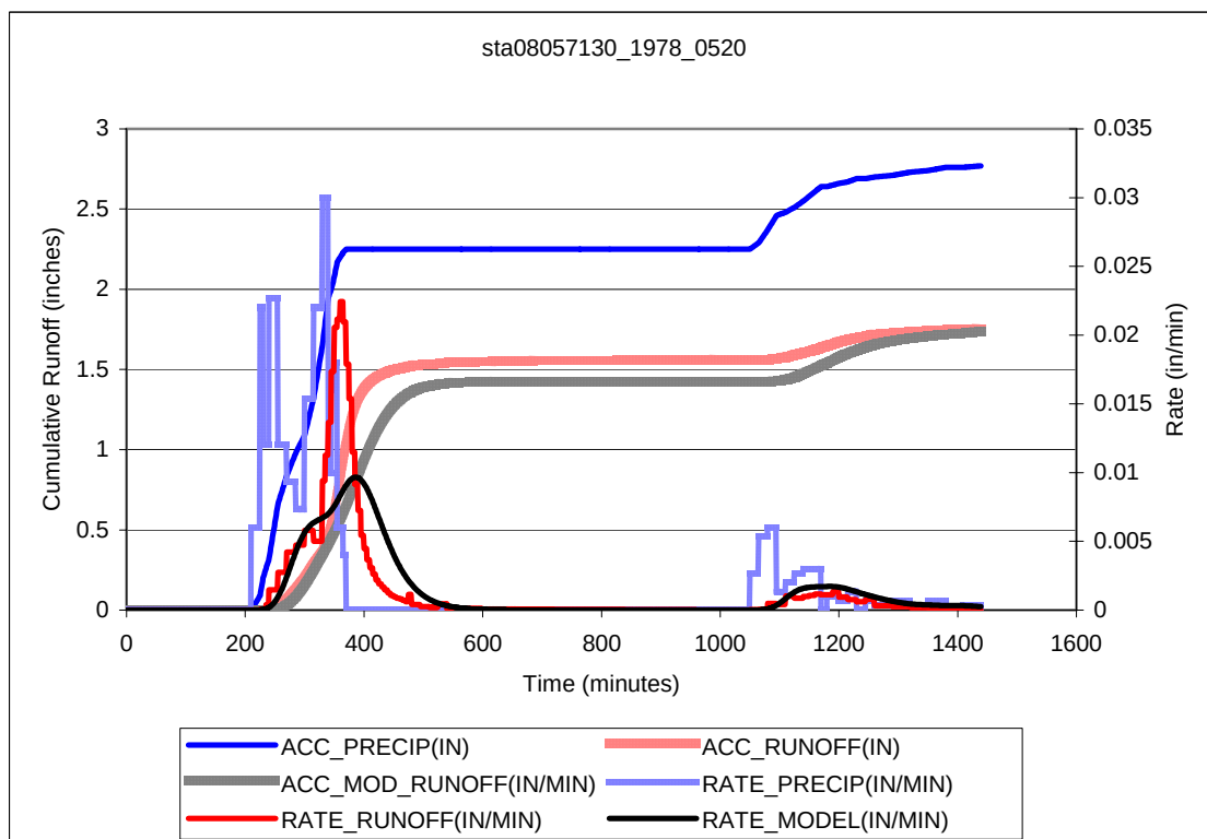
Figure A.11 Rush Branch response under rainfall on 05-20-1978.
