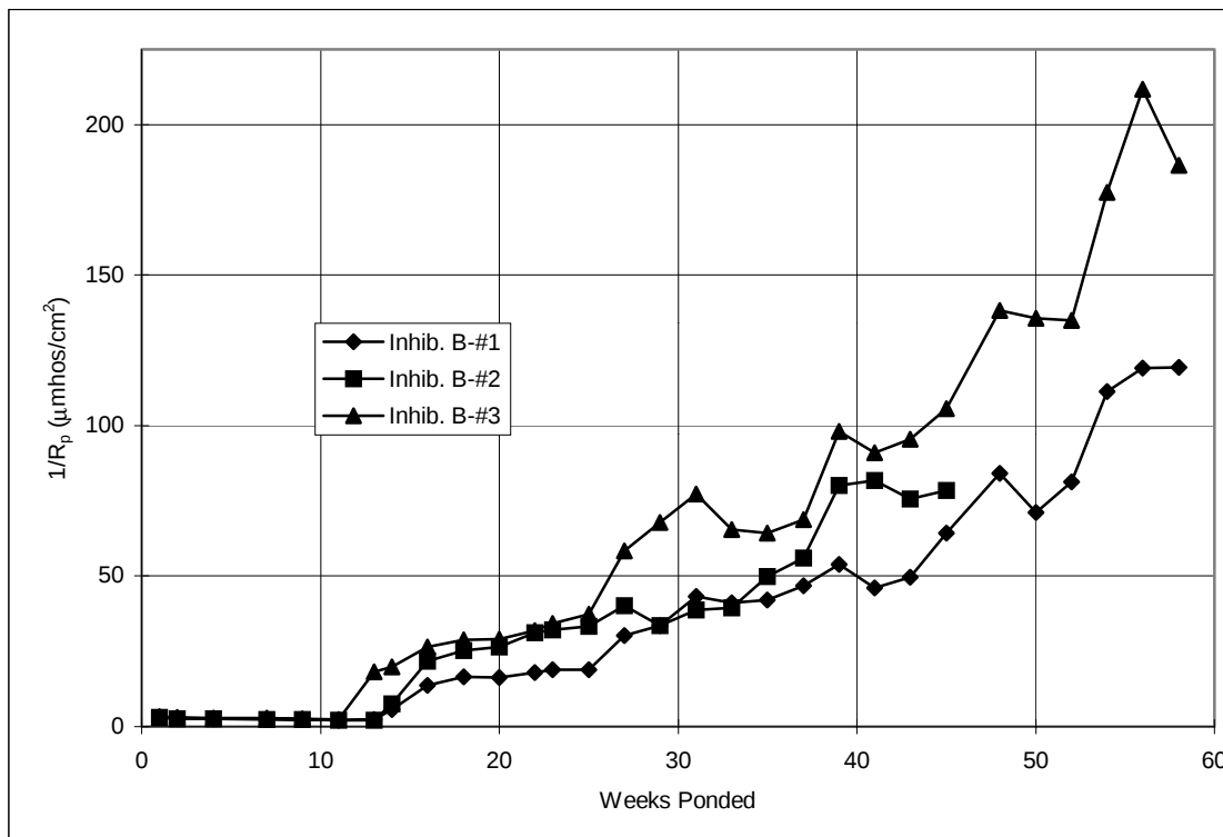
Figure A.39 Corrosion rate, 2-inch diameter lollipops: Inhibitor B.
