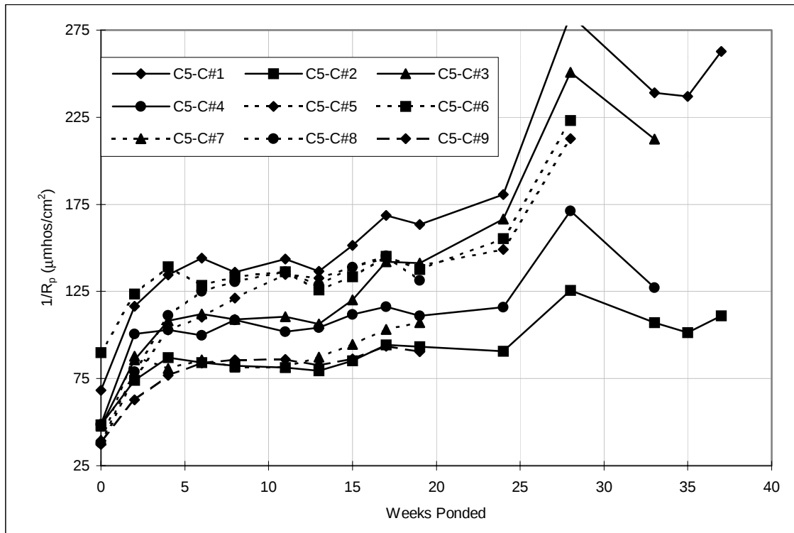
Figure A.63 Corrosion rate, pre-cracked lollipops: Control, specimens 1-9.
