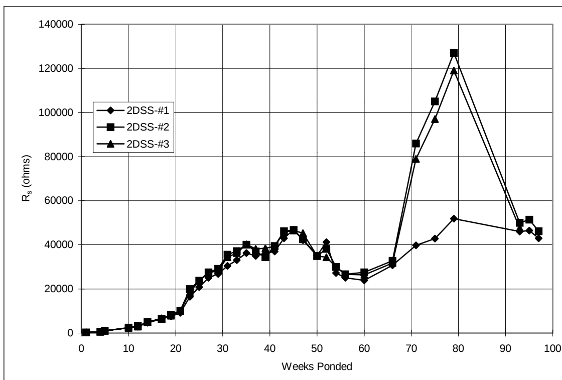
Figure A.15 Solution resistance, 3-inch diameter lollipops: 2%DSS.
