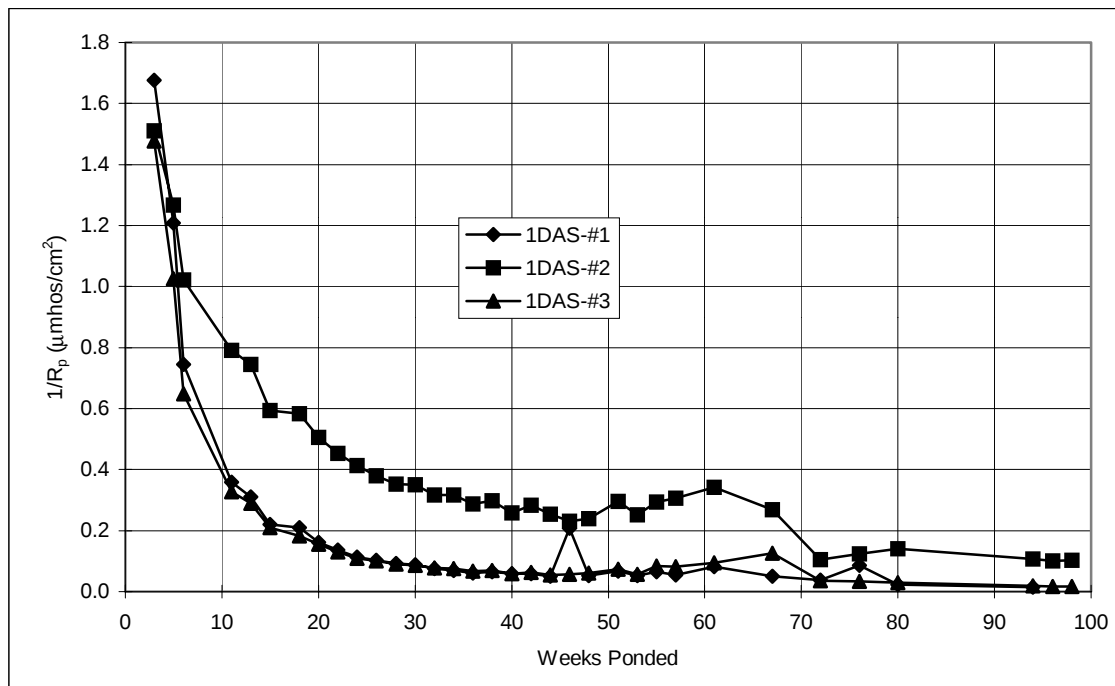
Figure A.49 Corrosion rate, 3-inch diameter lollipops: 1%DAS.
