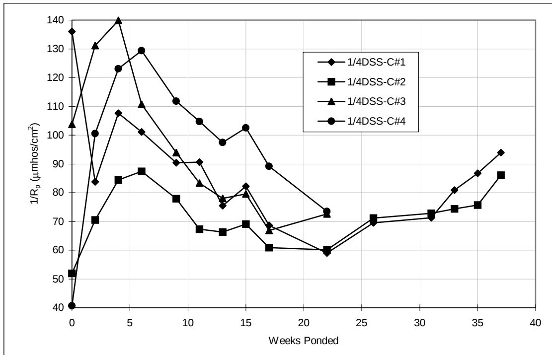
Figure A.71 Corrosion rate, pre-cracked lollipops: 1/4%DSS.
