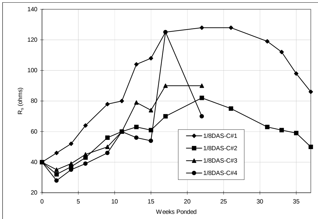
Figure A.33 Solution resistance, pre-cracked lollipops: 1/8%DAS.
