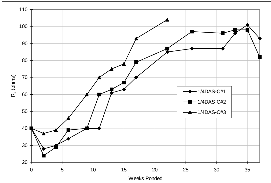
Figure A.32 Solution resistance, pre-cracked lollipops: 1/4%DAS.
