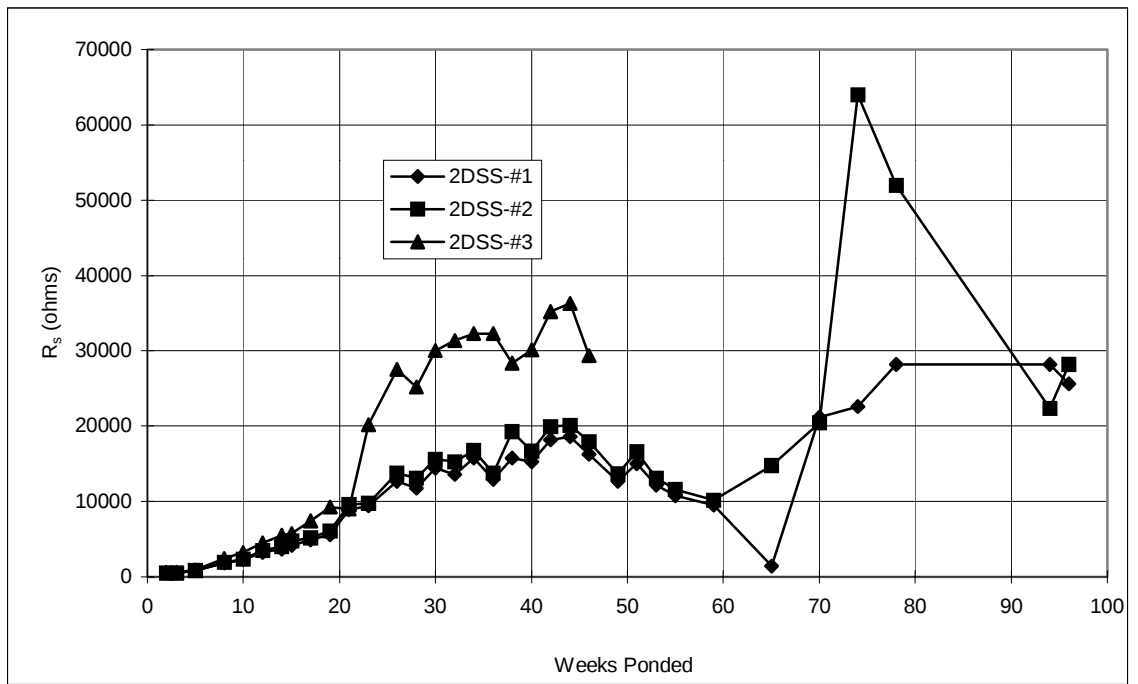
Figure A.7 Solution resistance, 2-inch diameter lollipops: 2%DSS.
