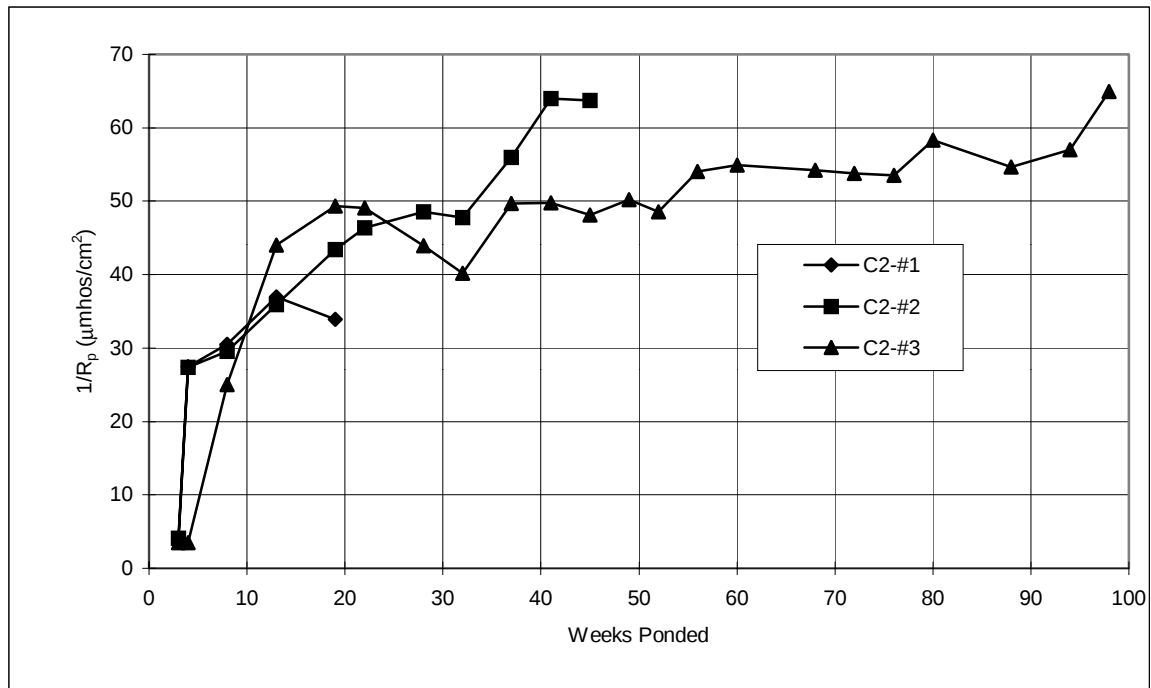
Figure A.54 Corrosion rate, slabs: Control 2-connected.
