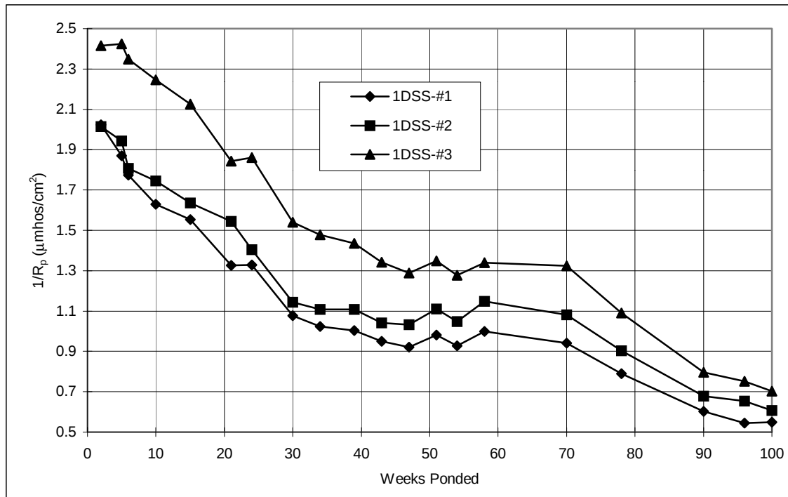
Figure A.62 Corrosion rate, slabs: 1%DSS.
