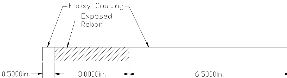
Figure 4.4 No. 4 rebar with 3" long area of exposure.
