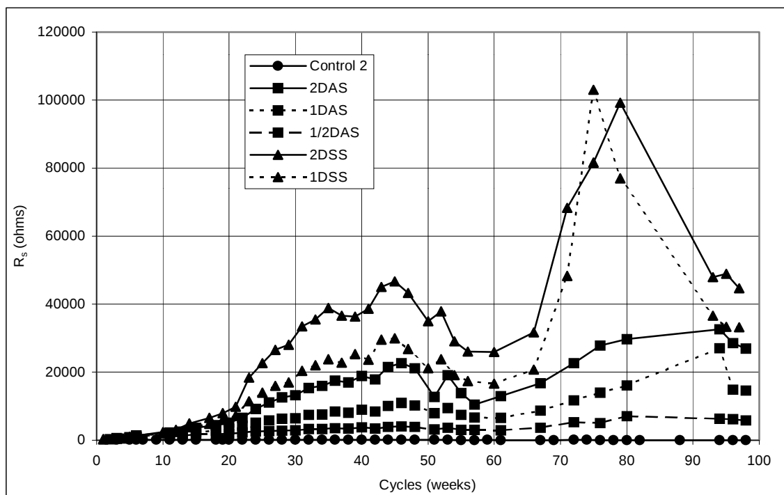
Figure 5.10 Solution resistance, 3-inch cylinders: Control, DAS, and DSS.
