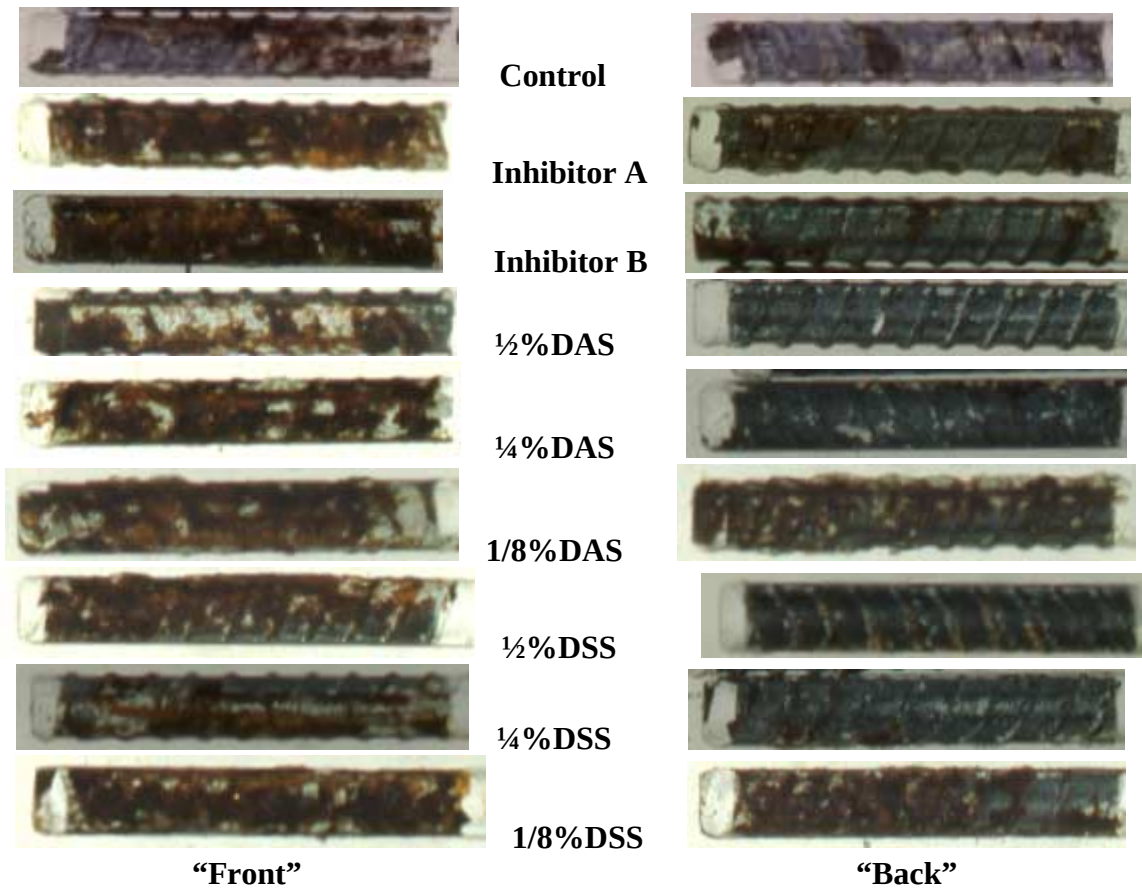
Figure 5.31 No. 4 rebar from the oven-dried pre-cracked specimens.
