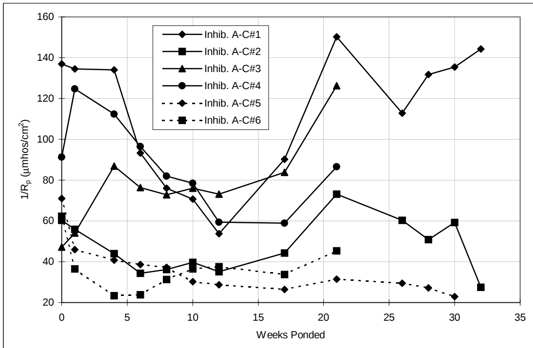
Figure A.65 Corrosion rate, pre-cracked lollipops: Inhibitor A.
