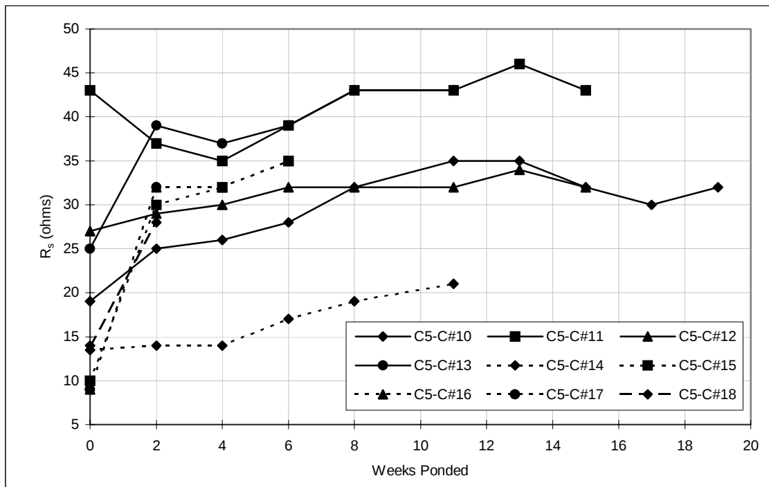
Figure A.28 Solution resistance, pre-cracked lollipops: Control, specimens 10-18.
