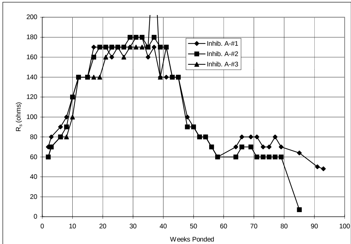
Figure A.10 Solution resistance, 3-inch diameter lollipops: Inhibitor A.
