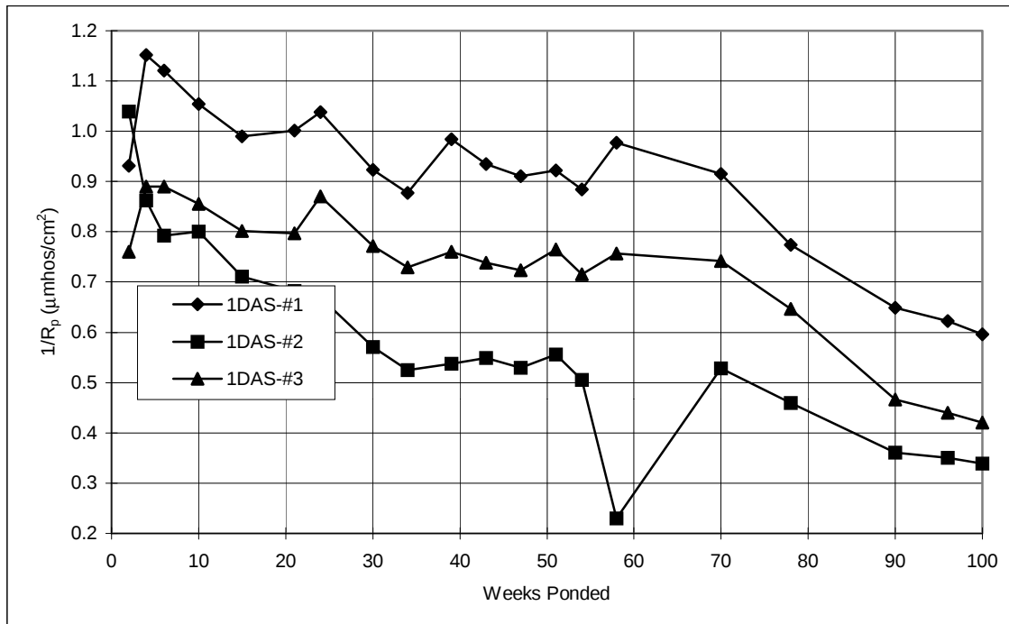
Figure A.59 Corrosion rate, slabs: 1%DAS.
