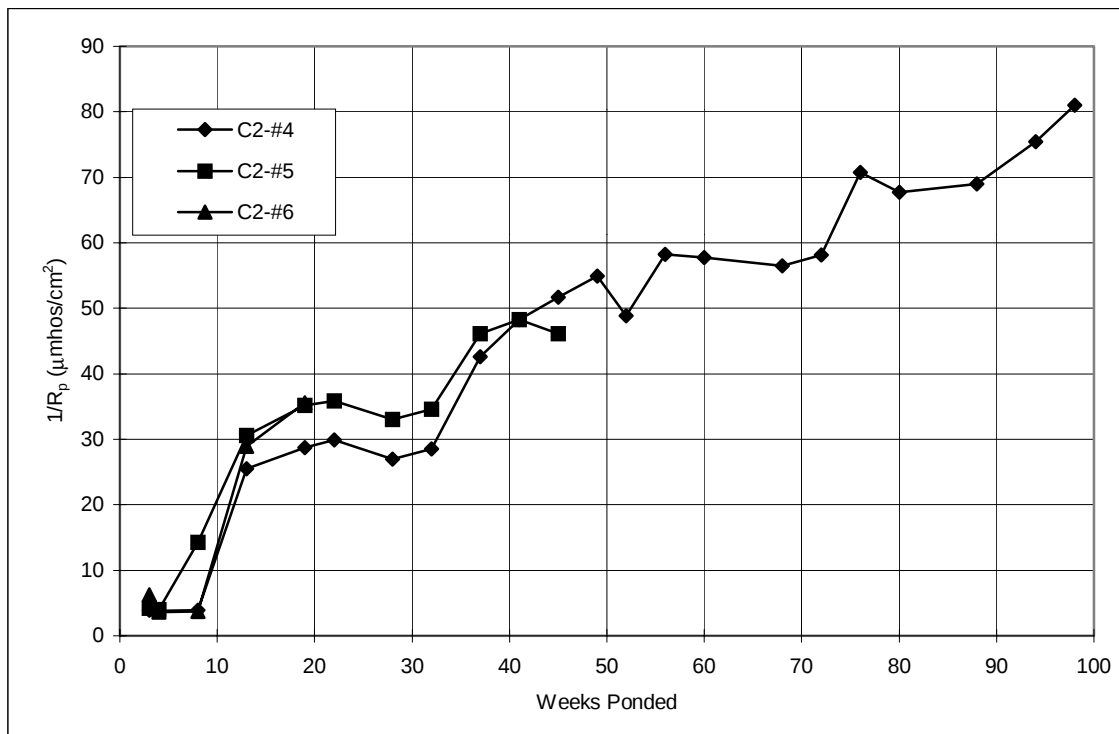
Figure A.55 Corrosion rate, slabs: Control 2-unconnected.
