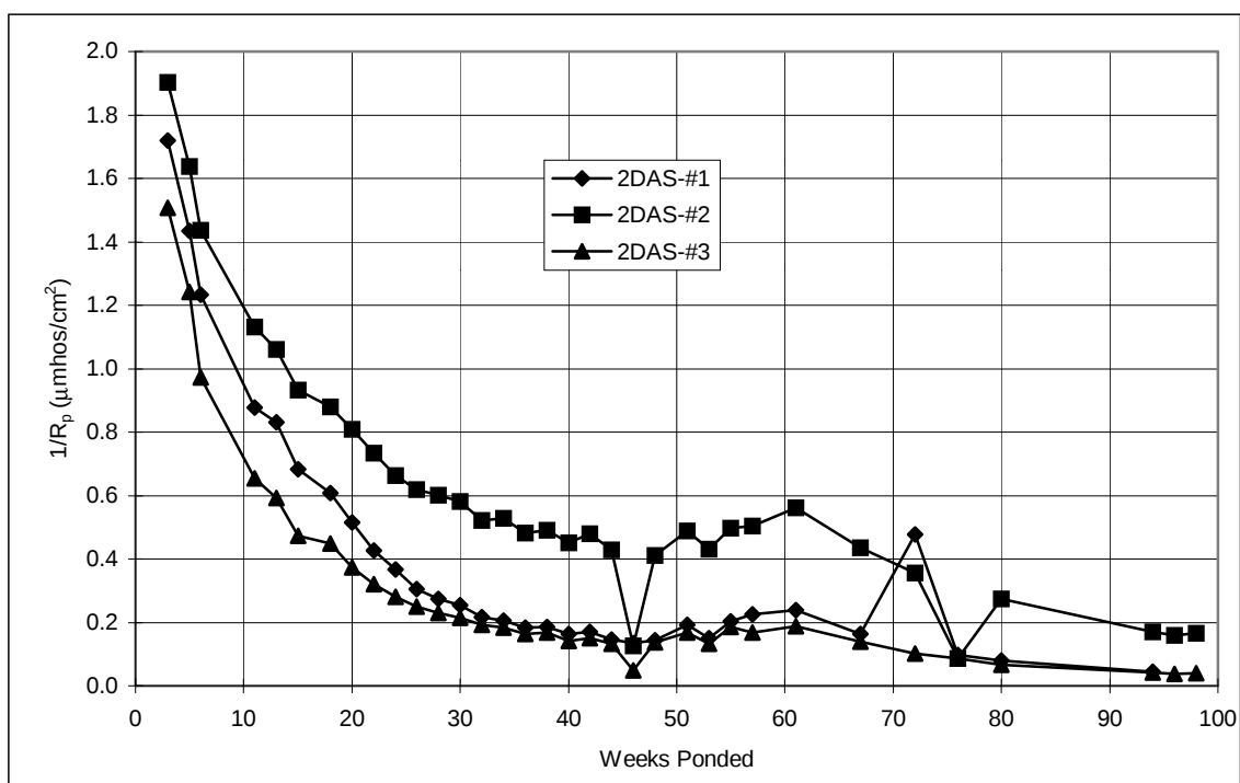
Figure A.48 Corrosion rate, 3-inch diameter lollipops: 2%DAS.
