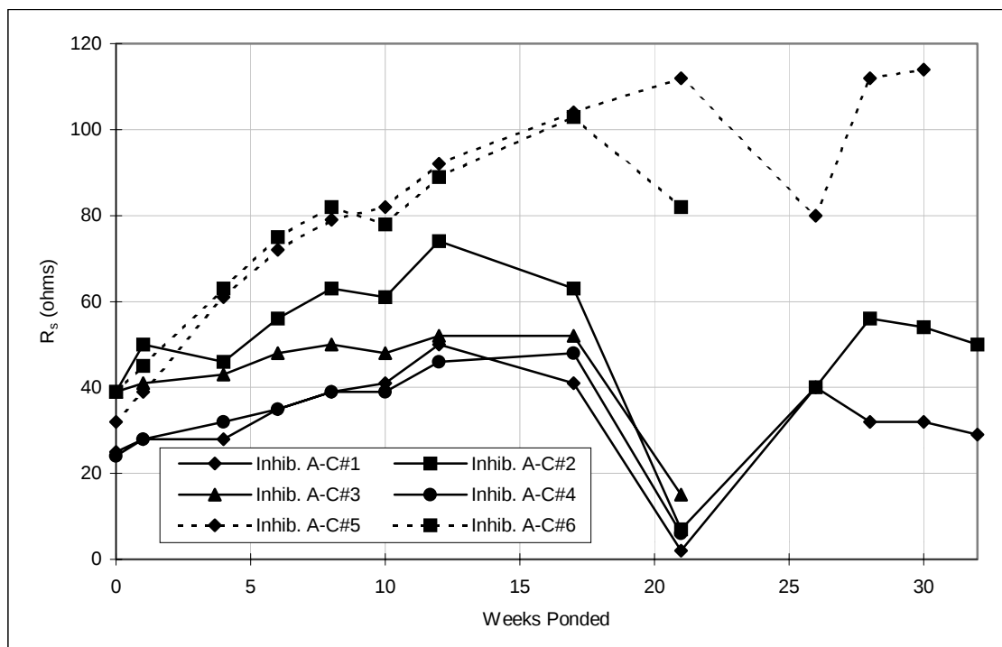
Figure A.29 Solution resistance, pre-cracked lollipops: Inhibitor A.
