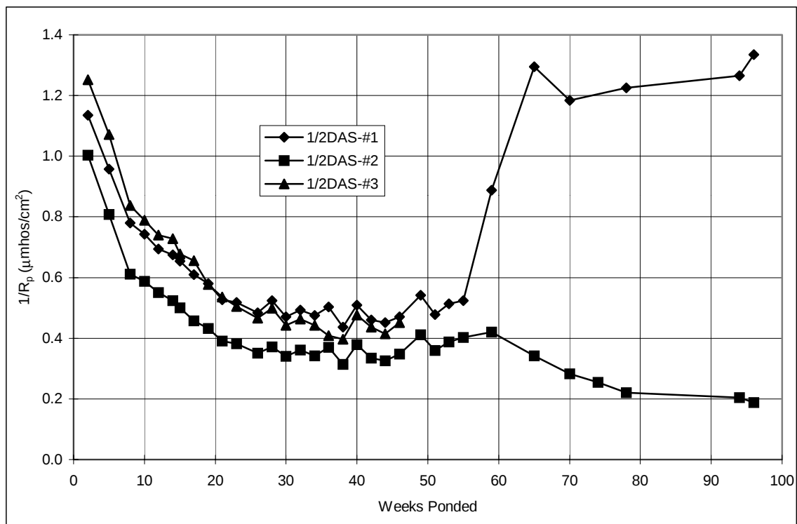
Figure A.42 Corrosion rate, 2-inch diameter lollipops: 1/2%DAS.
