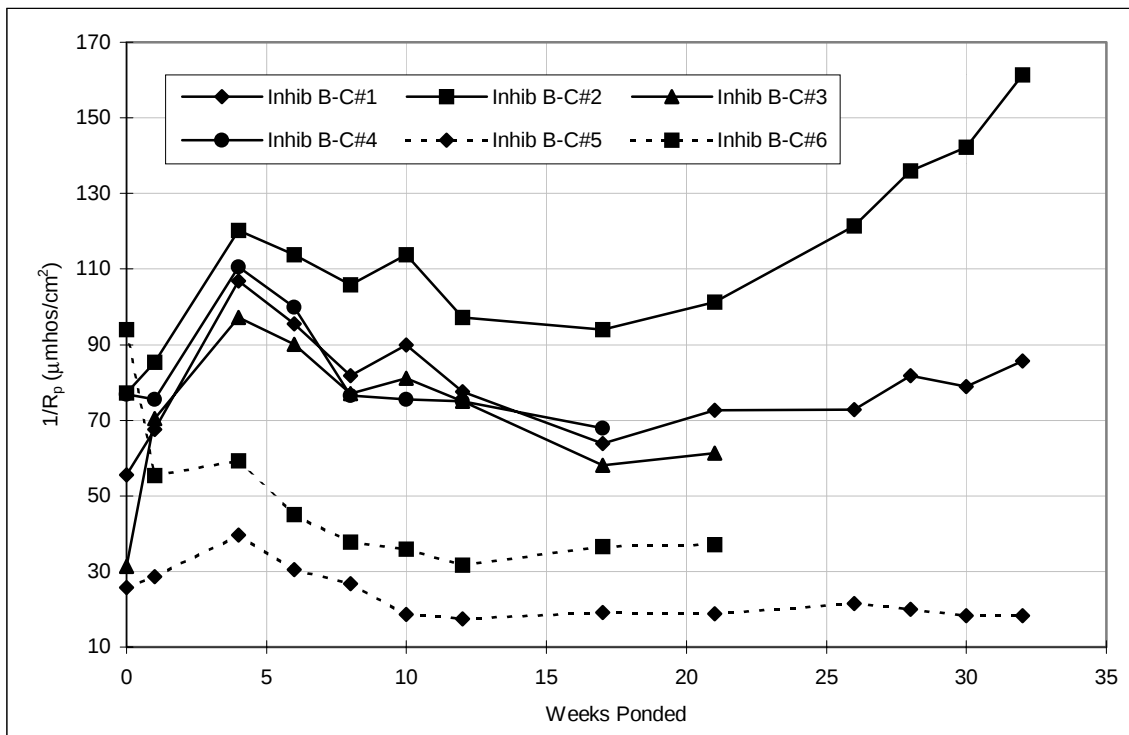
Figure A.66 Corrosion rate, pre-cracked lollipops: Inhibitor B.
