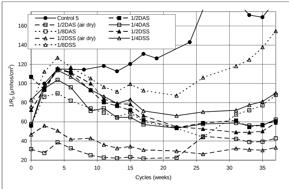
Figure 5.22 Corrosion rates, pre-cracked cylinders: Control, DAS, and DSS.
