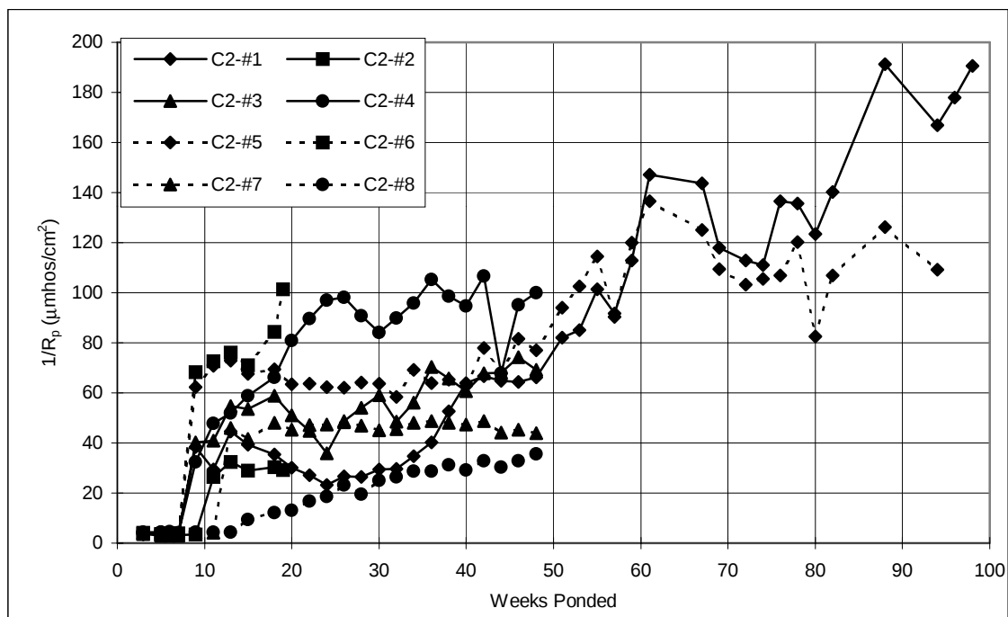
Figure A.45 Corrosion rate, 3-inch diameter lollipops: Control.
