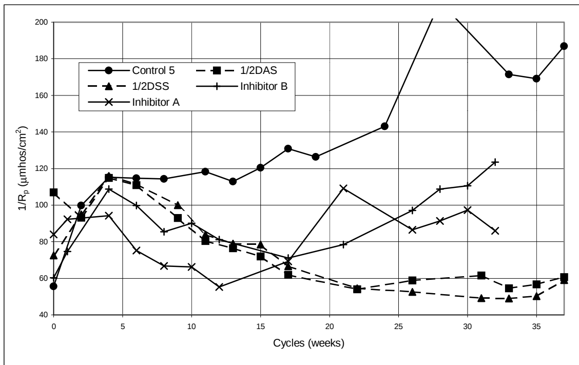
Figure 5.23 Corrosion rates, pre-cracked cylinders: Control, ½%DAS and DSS, and Inhibitors A and B.
