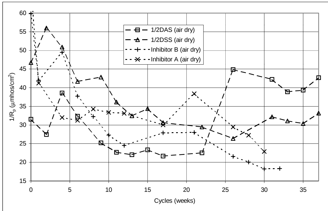
Figure 5.24 Corrosion rates, pre-cracked cylinders (air-dried): ½%DAS and DSS, Inhibitors A and B.
