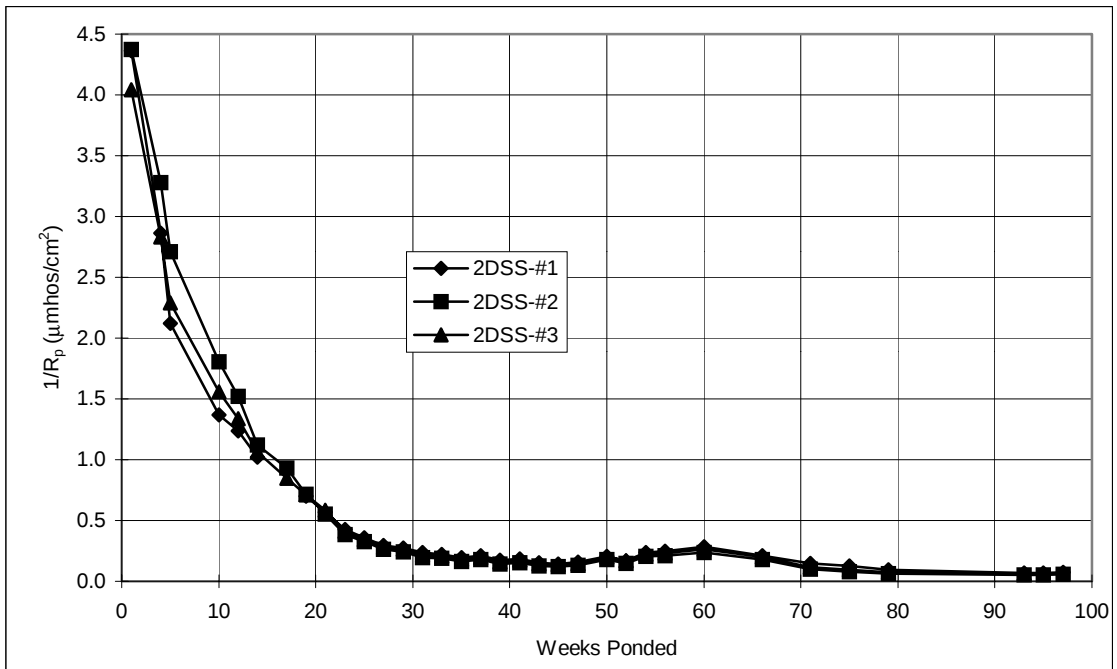
Figure A.51 Corrosion rate, 3-inch diameter lollipops: 2%DSS.
