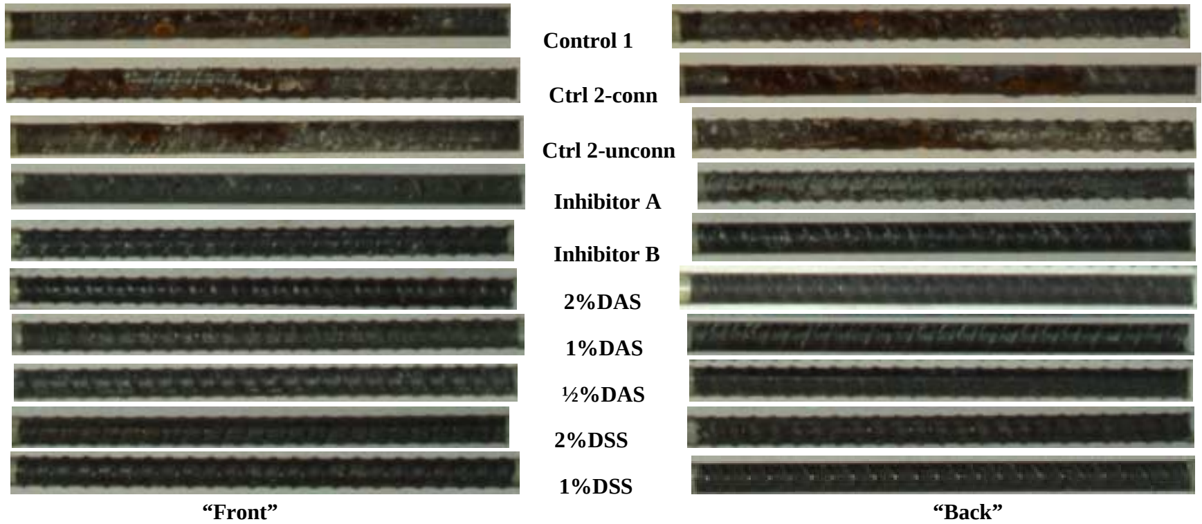
Figure 5.29 No. 4 rebar from the slab specimens.
