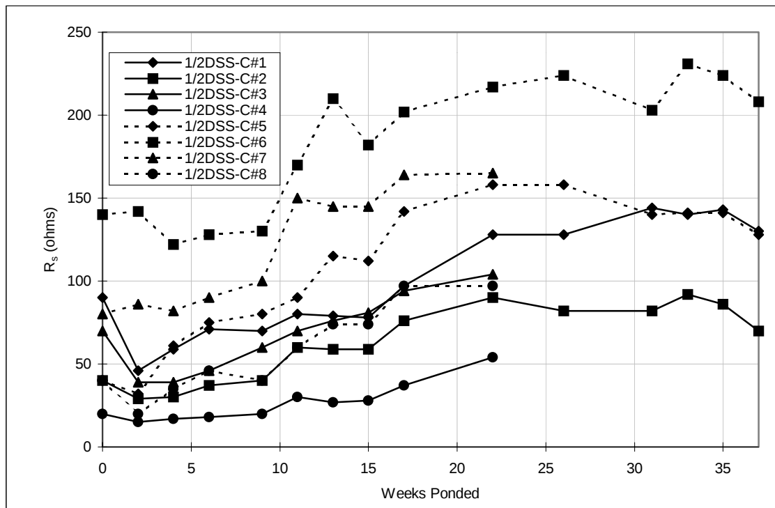
Figure A.34 Solution resistance, pre-cracked lollipops: 1/2%DSS.
