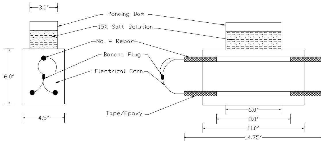
Figure 4.7 Slab Specimen, from Reference 48.
