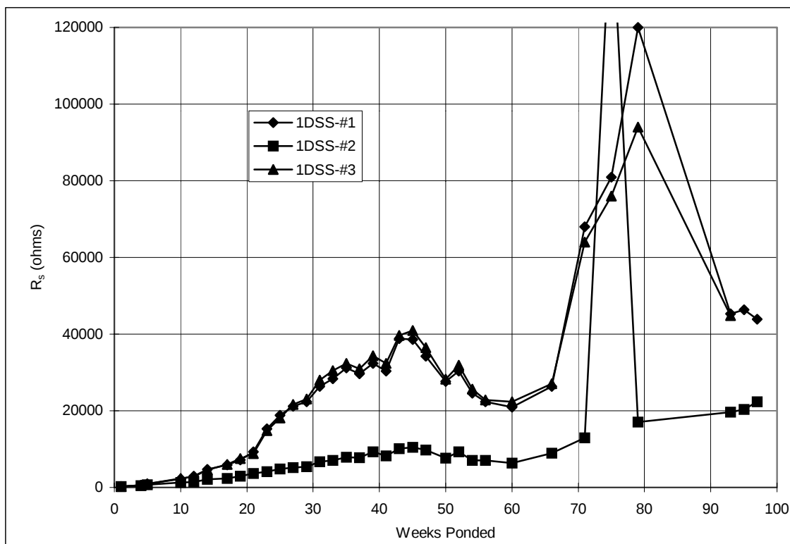
Figure A.16 Solution resistance, 3-inch diameter lollipops: 1%DSS.
