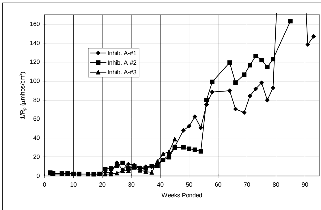
Figure A.46 Corrosion rate, 3-inch diameter lollipops: Inhibitor A.
