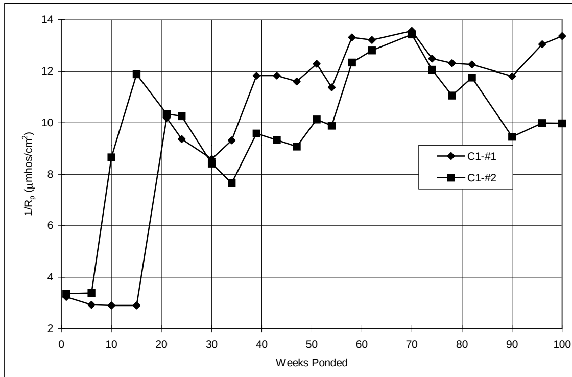
Figure A.53 Corrosion rate, slabs: Control 1.
