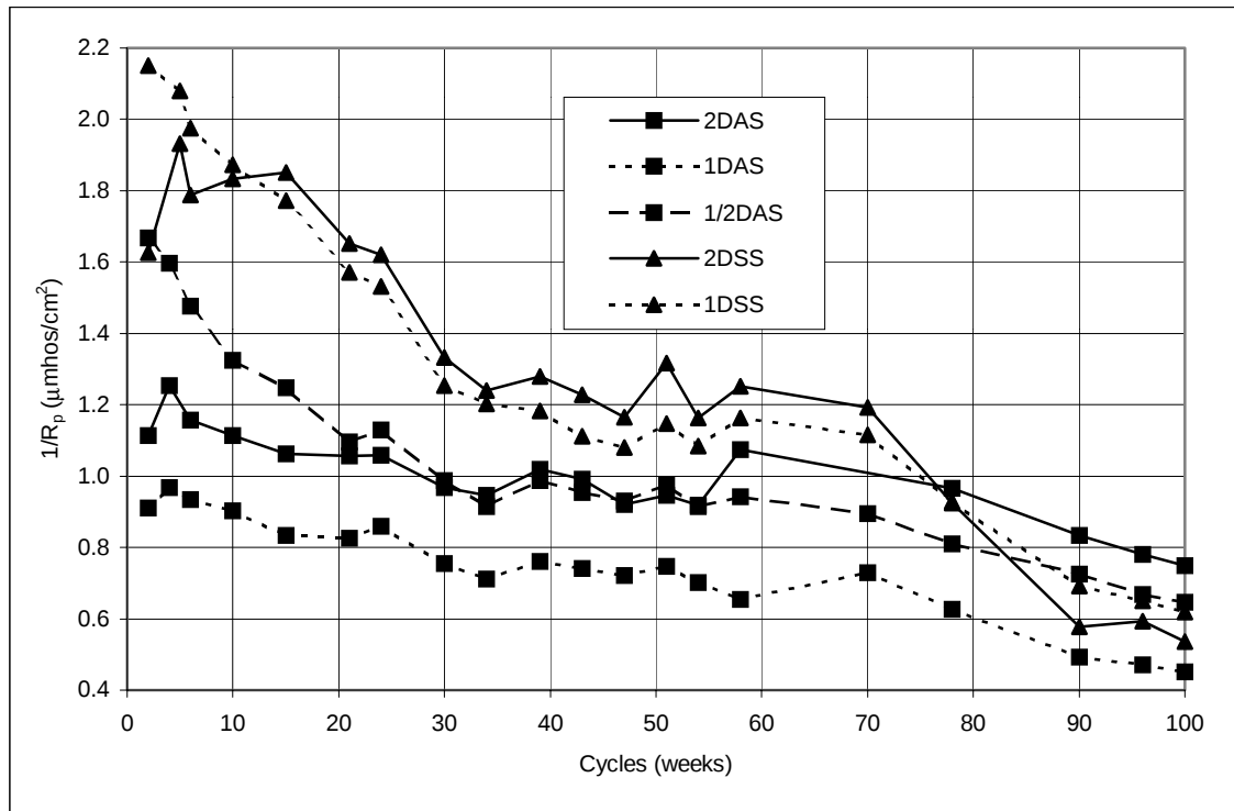
Figure 5.20 Corrosion rates, slabs: DAS and DSS.
