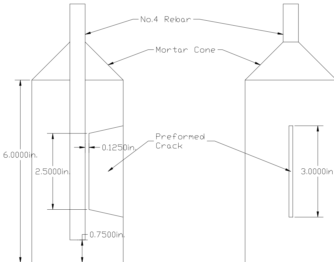
Figure 4.1 Pre-cracked cylinder.
