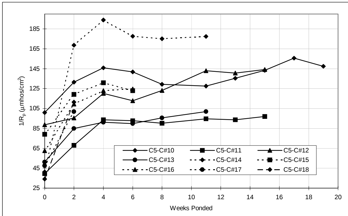
Figure A.64 Corrosion rate, pre-cracked lollipops: Control, specimens 10-18.
