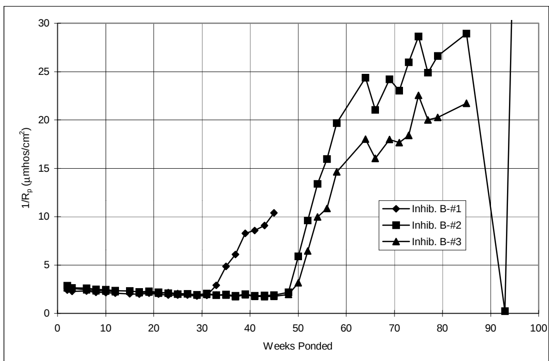
Figure A.47 Corrosion rate, 3-inch diameter lollipops: Inhibitor B.
