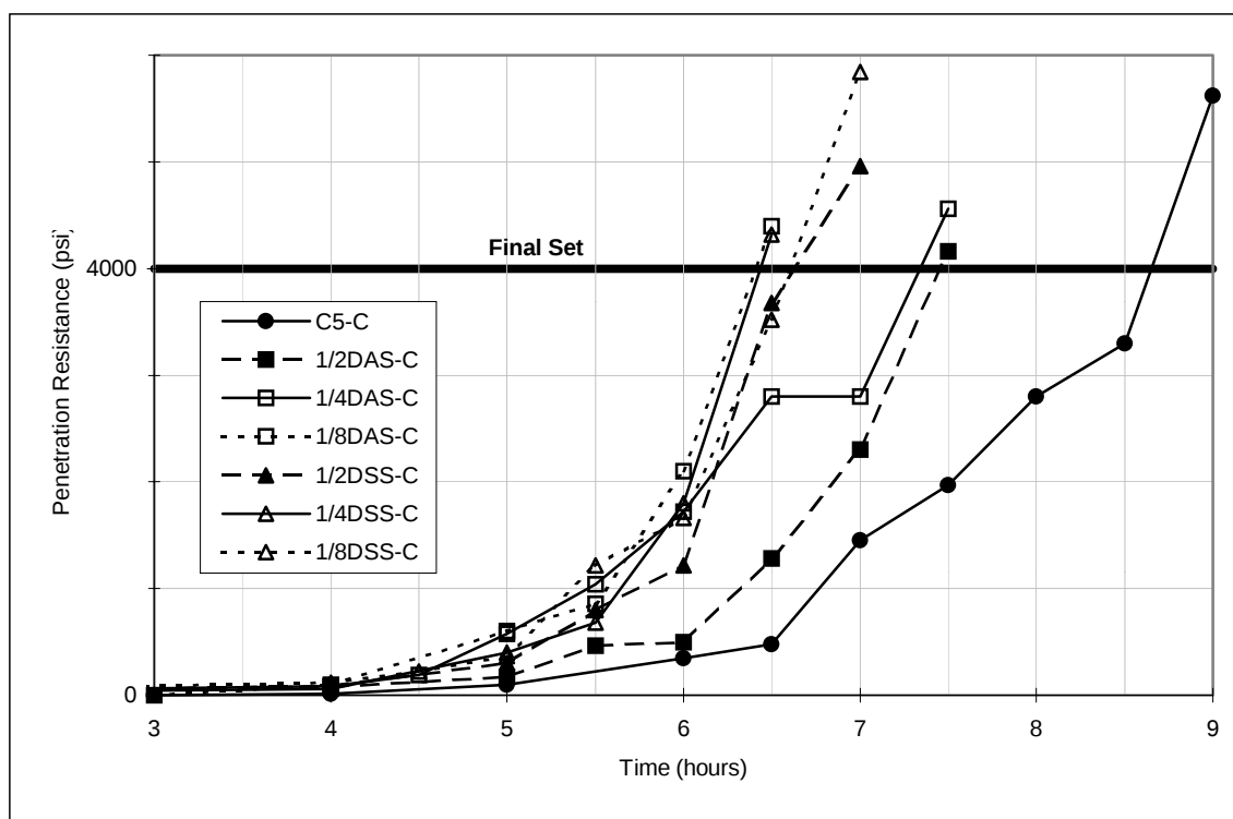
Figure 5.4 Setting times for Phase II specimens.
