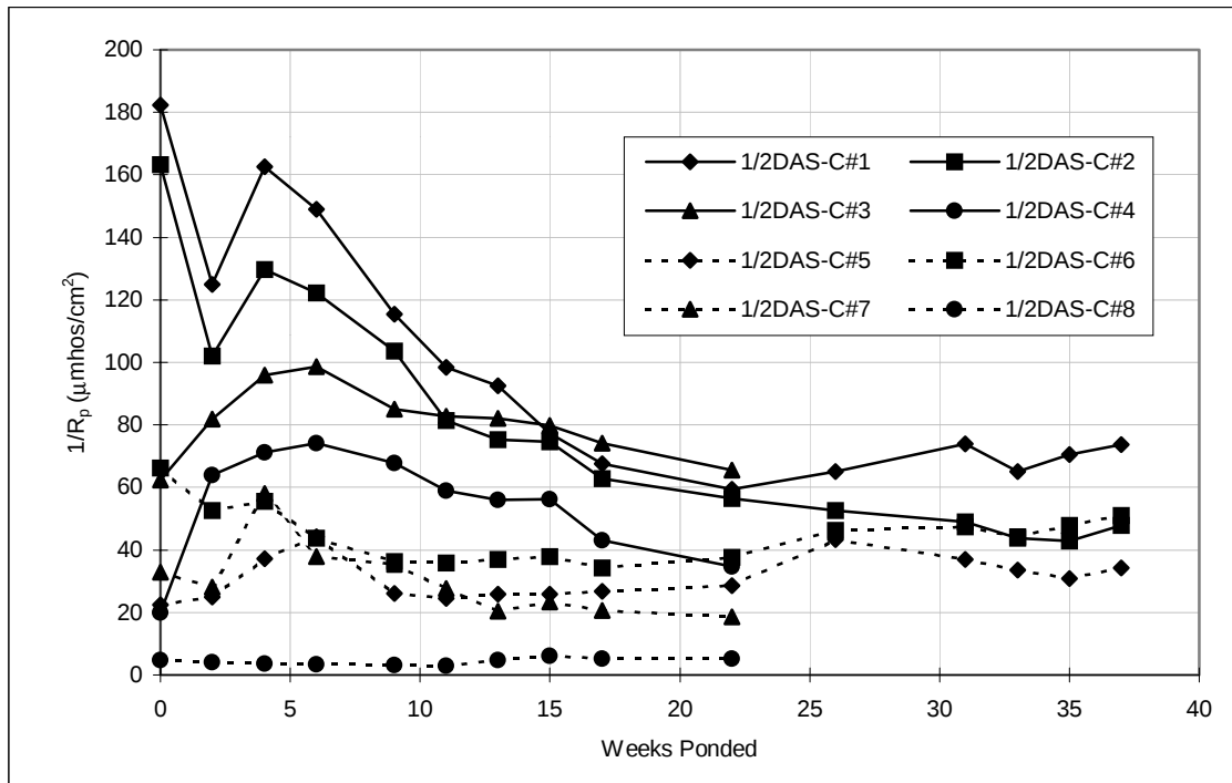
Figure A.67 Corrosion rate, pre-cracked lollipops: 1/2%DAS.
