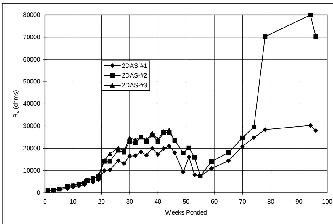
Figure A.4 Solution resistance, 2-inch diameter lollipops: 2%DAS.
