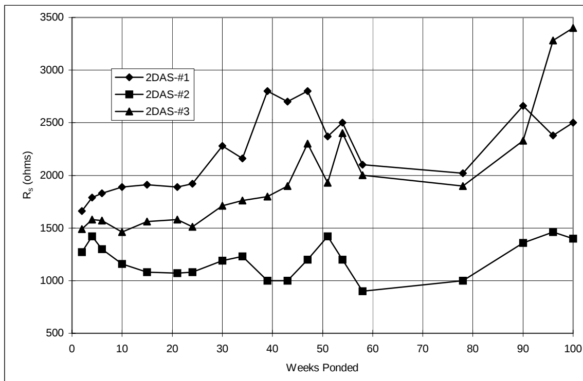
Figure A.22 Solution resistance, slabs: 2%DAS.
