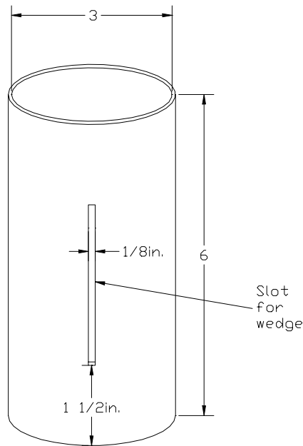
Figure 4.2 Slotted cylinder for casting pre-cracked specimens.
