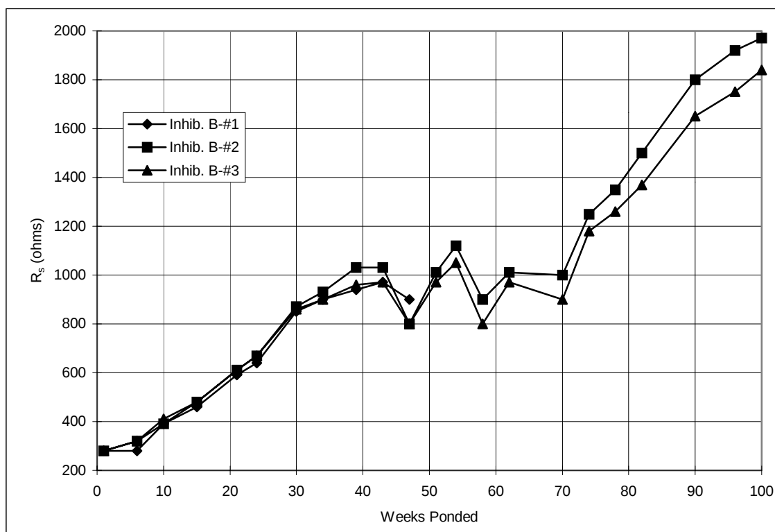
Figure A.21 Solution resistance, slabs: Inhibitor B.
