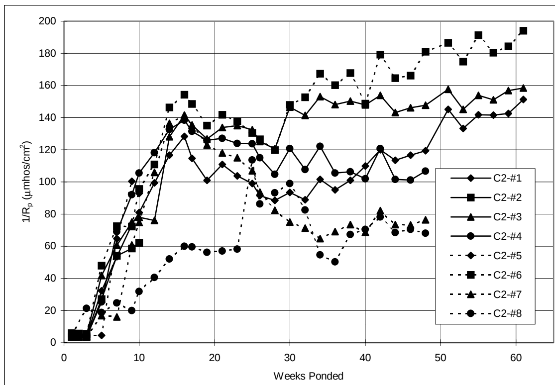
Figure A.37 Corrosion rate, 2-inch diameter lollipops: Control.
