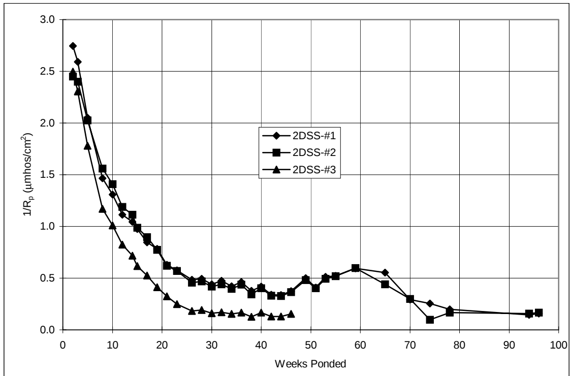
Figure A.43 Corrosion rate, 2-inch diameter lollipops: 2%DSS.
