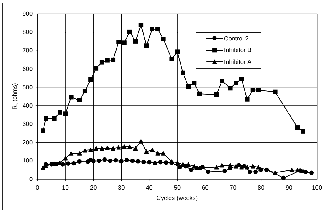
Figure 5.9 Solution resistance, 3-inch cylinders: Control, Inhibitors A and B.
