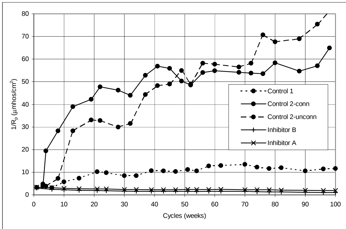
Figure 5.19 Corrosion rates, slabs: Control, Inhibitors A and B.
