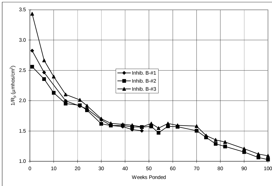
Figure A.57 Corrosion rate, slabs: Inhibitor B.
