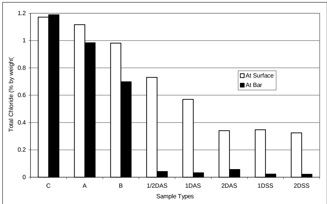
Figure 5.5 Total chlorides (% by weight) present in the concrete at both the surface and rebar.
