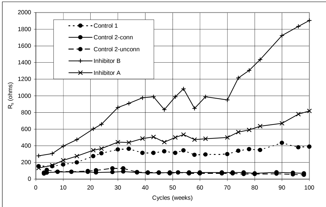
Figure 5.11 Solution resistance, slabs: Controls 1 and 2, Inhibitors A and B.
