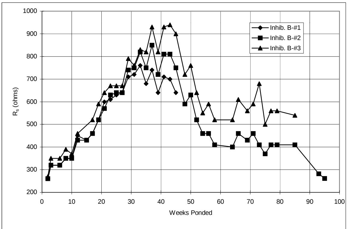
Figure A.11 Solution resistance, 3-inch diameter lollipops: Inhibitor B.
