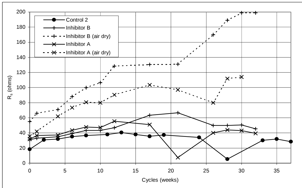
Figure 5.13 Solution resistance, pre-cracked cylinders: Control, Inhibitors A and B.
