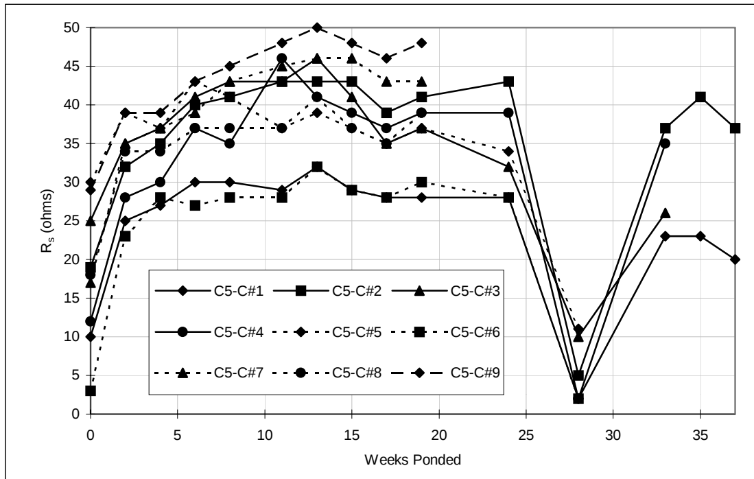
Figure A.27 Solution resistance, pre-cracked lollipops: Control, specimens 1-9.
