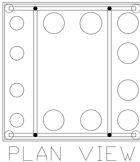
Figure 4.5 Modified (from Phase I) casting form with eight 3-inch diameter openings instead of six, adapted from Reference 48.
