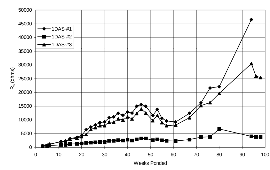
Figure A.13 Solution resistance, 3-inch diameter lollipops: 1%DAS.
