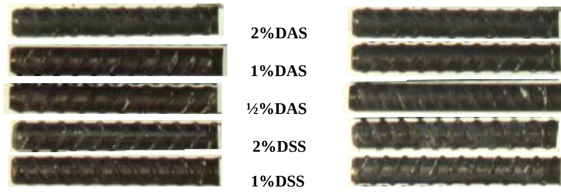
Figure 5.27 No. 4 rebar from the 2-inch DAS and DSS specimens.
