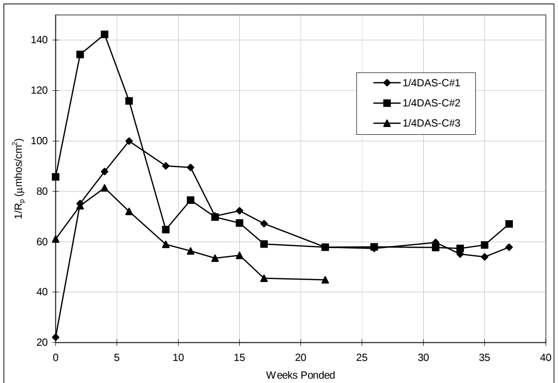
Figure A.68 Corrosion rate, pre-cracked lollipops: 1/4%DAS.
