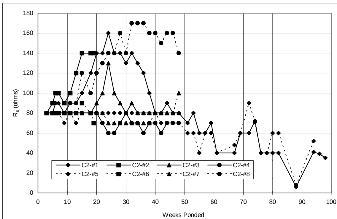
Figure A.9 Solution resistance, 3-inch diameter lollipops: Control.
