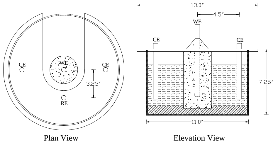
Figure 4.8 Lollipop Test Cell Setup, from Reference 48.
