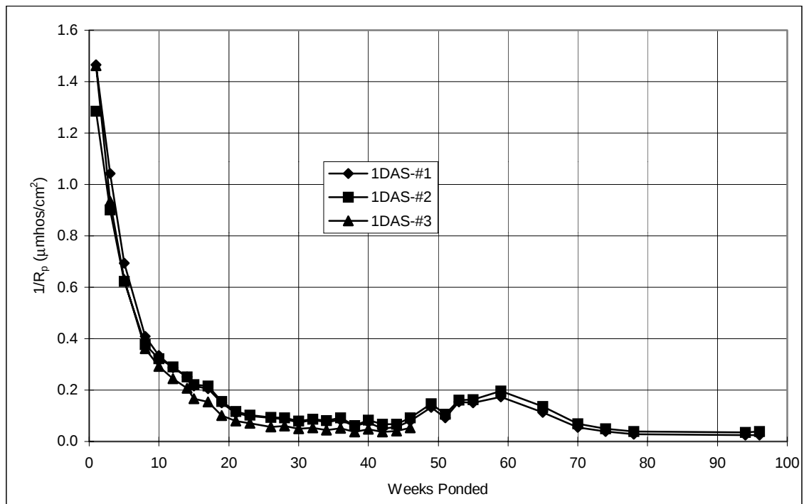
Figure A.41 Corrosion rate, 2-inch diameter lollipop: 1%DAS.
