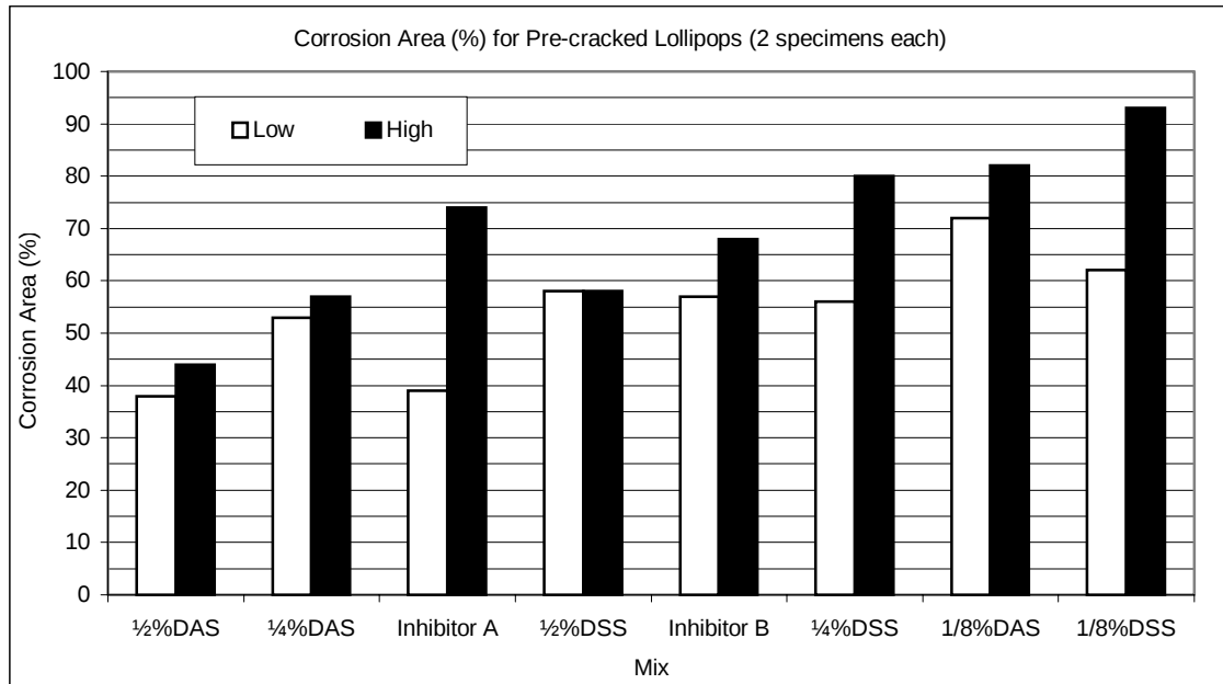
Figure 5.35 Comparison of corroded area for the pre-cracked lollipop specimens.
