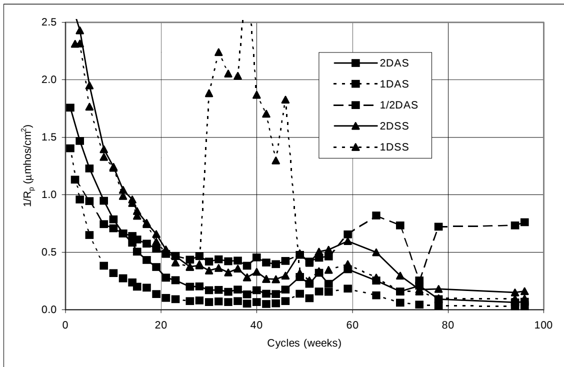
Figure 5.16 Corrosion rates, 2-inch cylinders: DAS and DSS.
