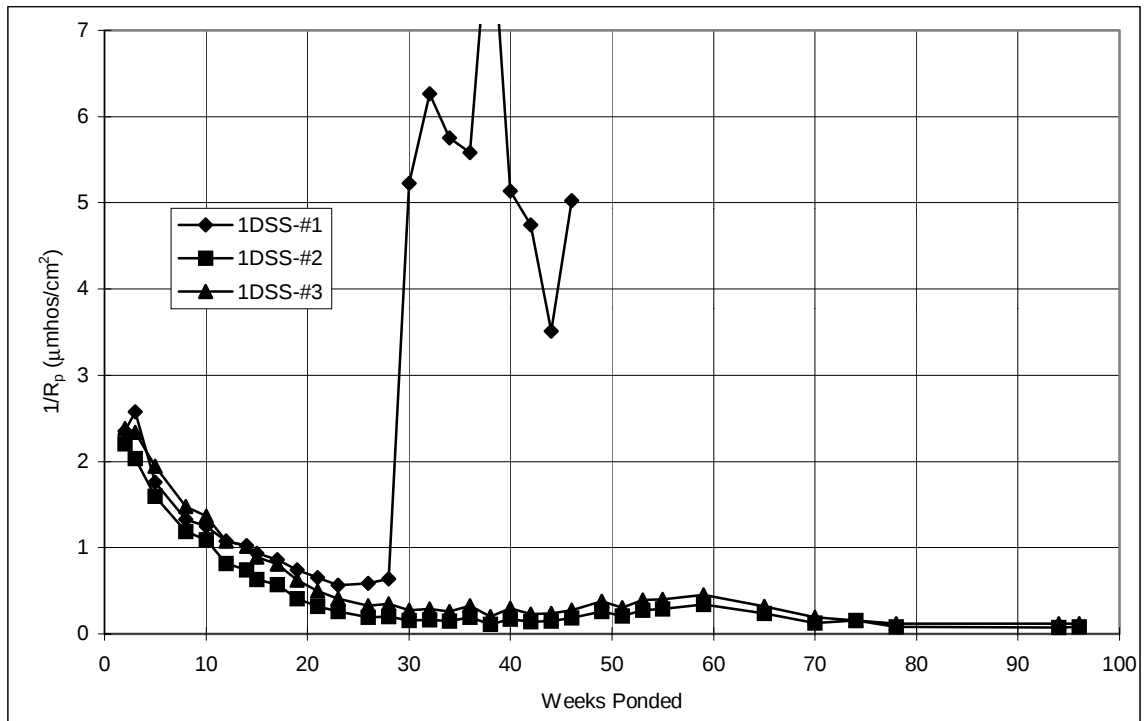
Figure A.44 Corrosion rate, 2-inch diameter lollipops: 1%DSS.
