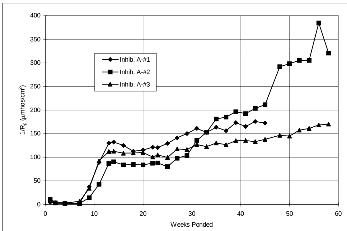
Figure A.38 Corrosion rate, 2-inch diameter lollipops: Inhibitor A.
