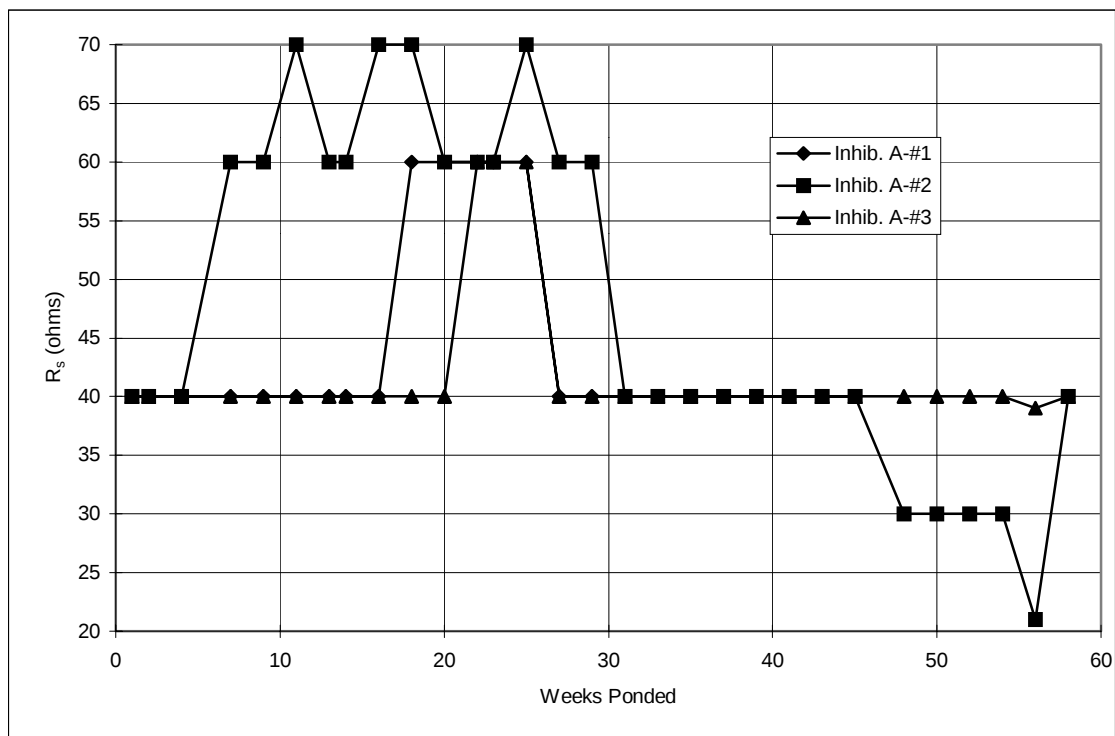
Figure A.2 Solution resistance, 2-inch diameter lollipops: Inhibitor A.
