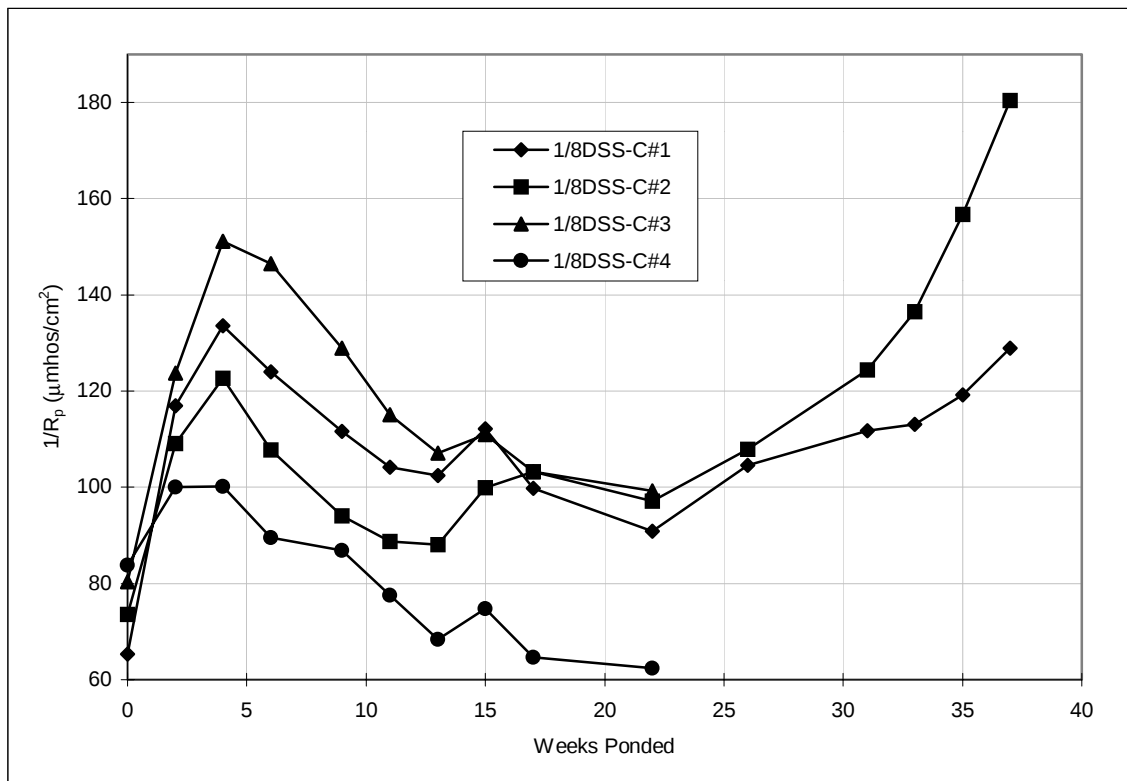
Figure A.72 Corrosion rate, pre-cracked lollipops: 1/8%DSS.
