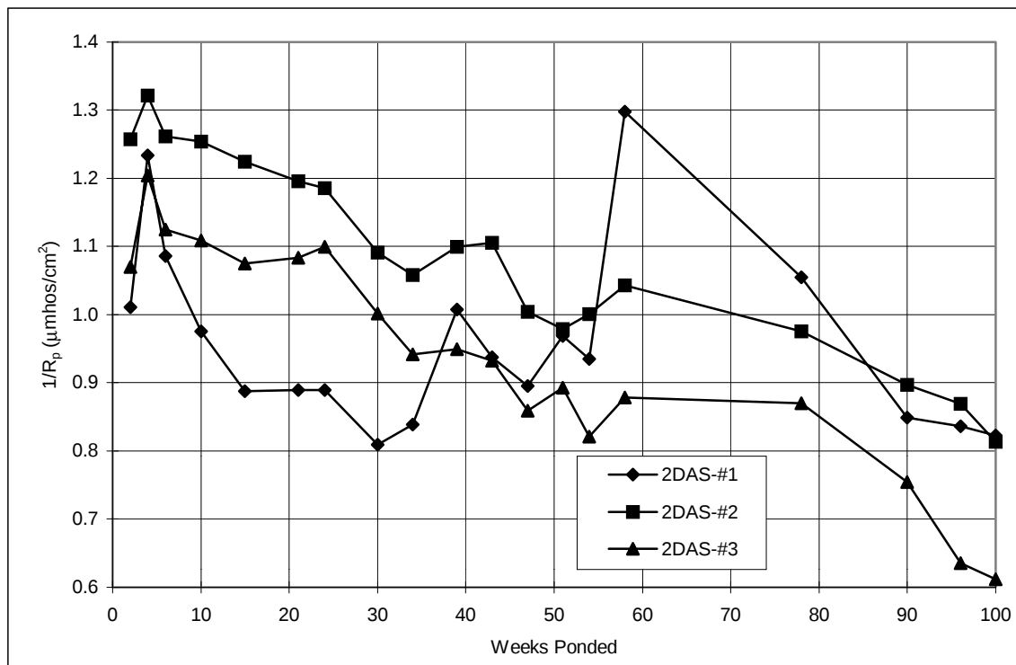
Figure A.58 Corrosion rate, slabs: 2%DAS.
