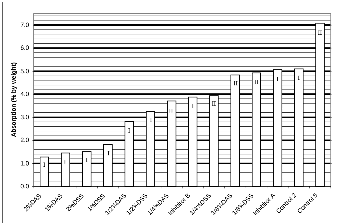
Figure 5.3 Final absorption: all specimens (Phases I and II), dried at 40°C.
