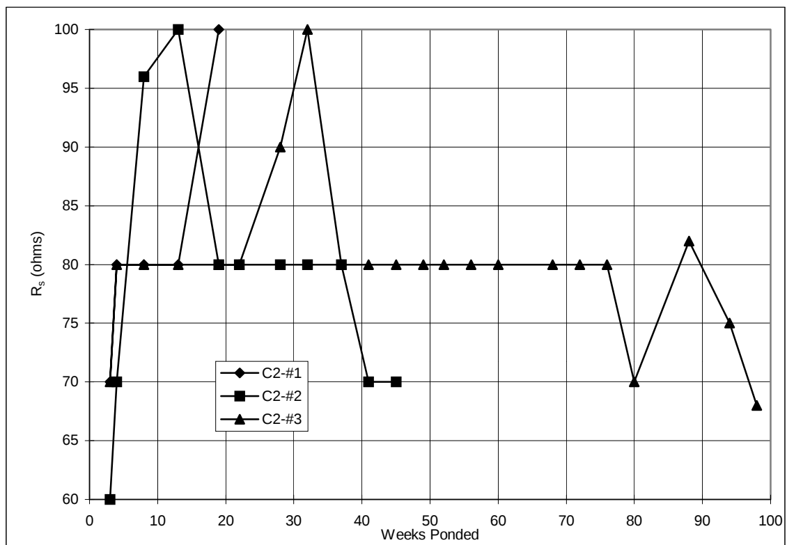
Figure A.18 Solution resistance, slabs: Control 2-connected.
