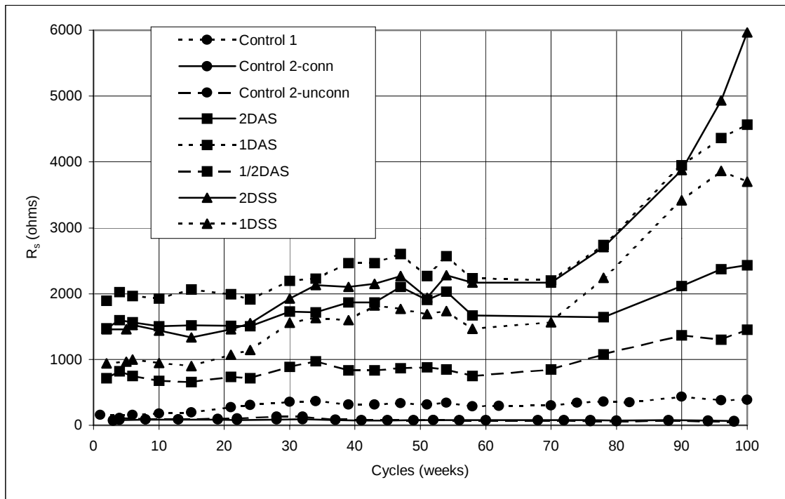
Figure 5.12 Solution resistance, slabs: Controls 1 and 2, DAS, and DSS.
