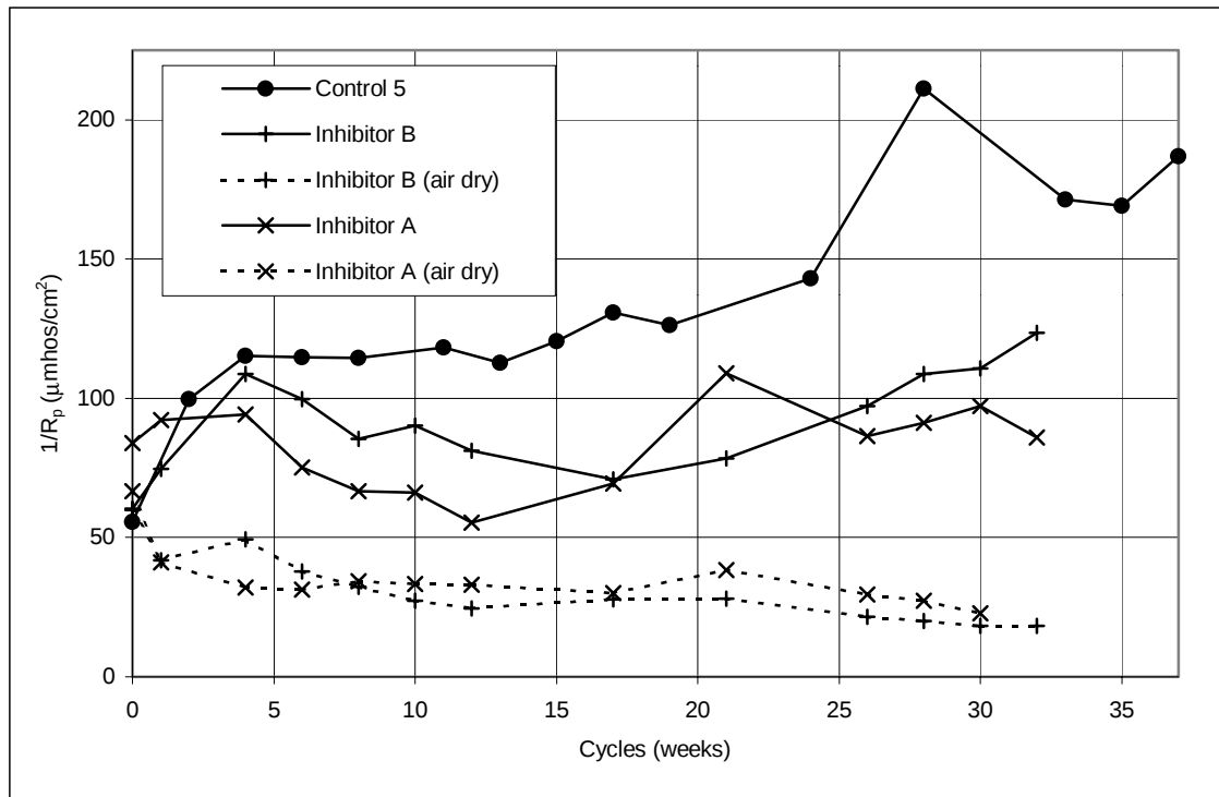
Figure 5.21 Corrosion rates, pre-cracked cylinders: Control, Inhibitors A and B.
