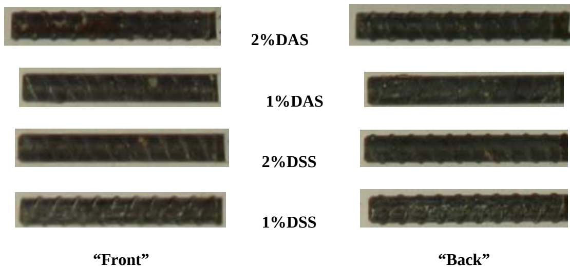
Figure 5.30 No. 4 rebar from the “Saw-Cut” 3-inch DAS and DSS specimens.
