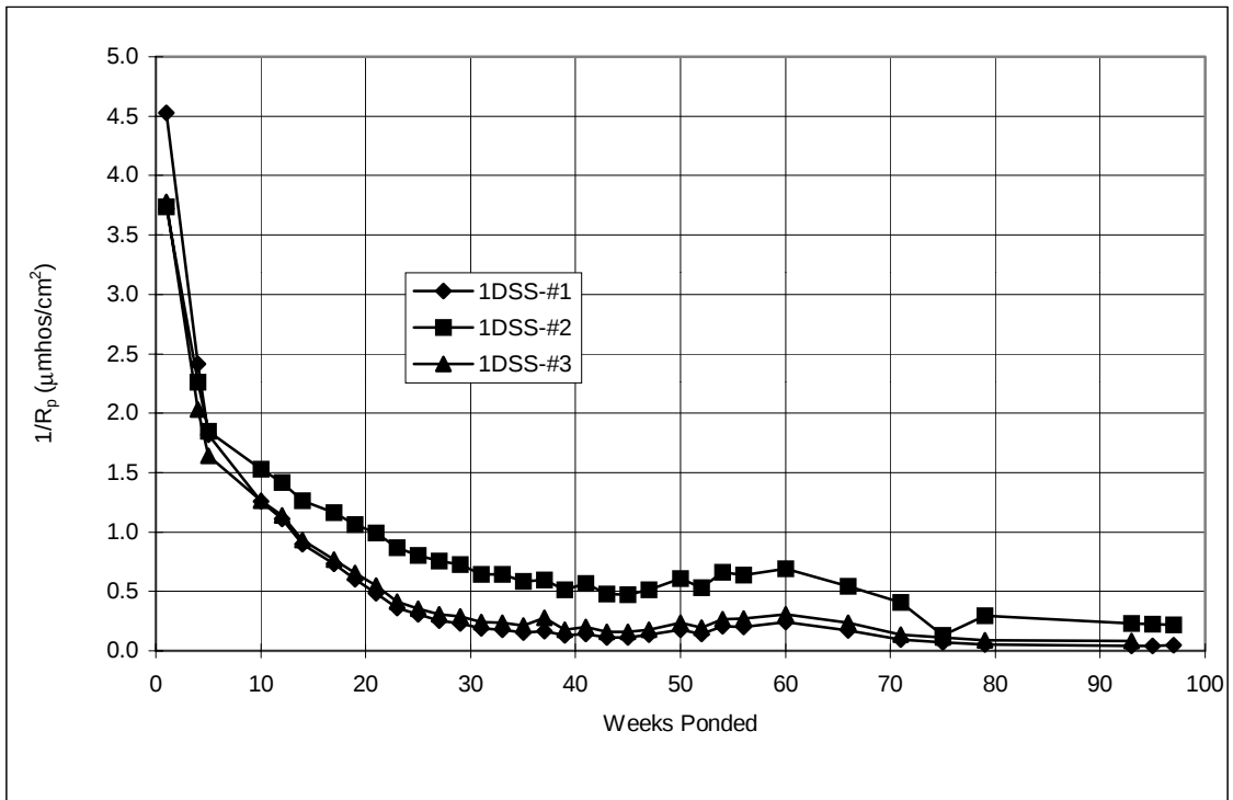
Figure A.52 Corrosion rate, 3-inch diameter lollipops: 1%DSS.
