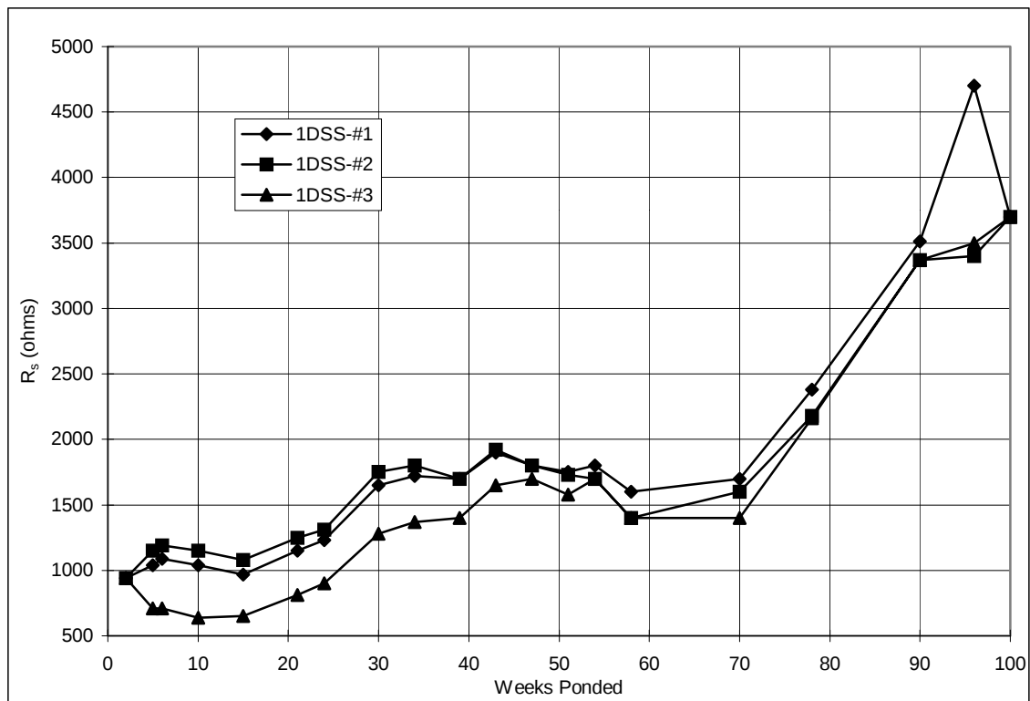
Figure A.26 Solution resistance, slabs: 1%DSS.
