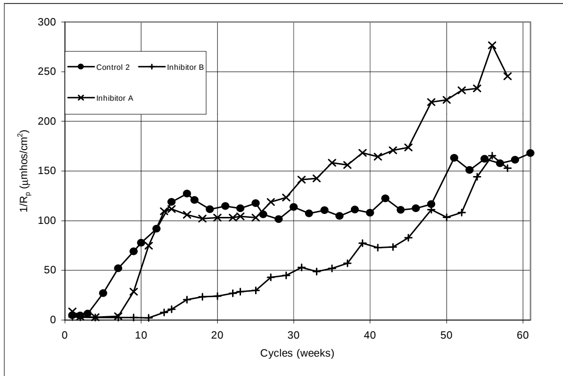
Figure 5.15 Corrosion rates, 2-inch cylinders: Control, Inhibitors A and B.
