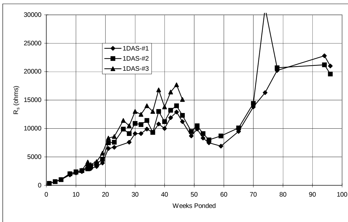
Figure A.5 Solution resistance, 2-inch diameter lollipop: 1%DAS.
