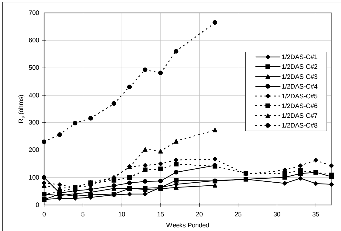
Figure A.31 Solution resistance, pre-cracked lollipops: 1/2%DAS.
