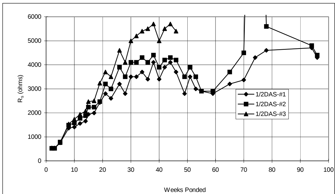
Figure A.6 Solution resistance, 2-inch diameter lollipops: 1/2%DAS.
