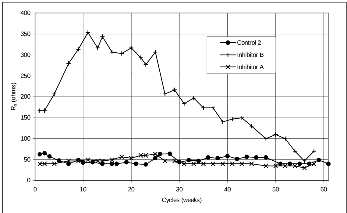
Figure 5.7 Solution resistance, 2-inch cylinders: Control, Inhibitors A and B.
