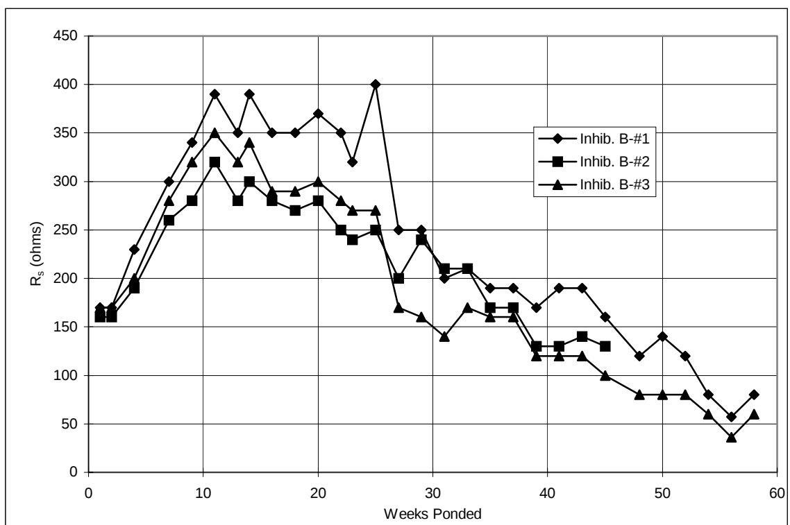
Figure A.3 Solution resistance, 2-inch diameter lollipops: Inhibitor B.
