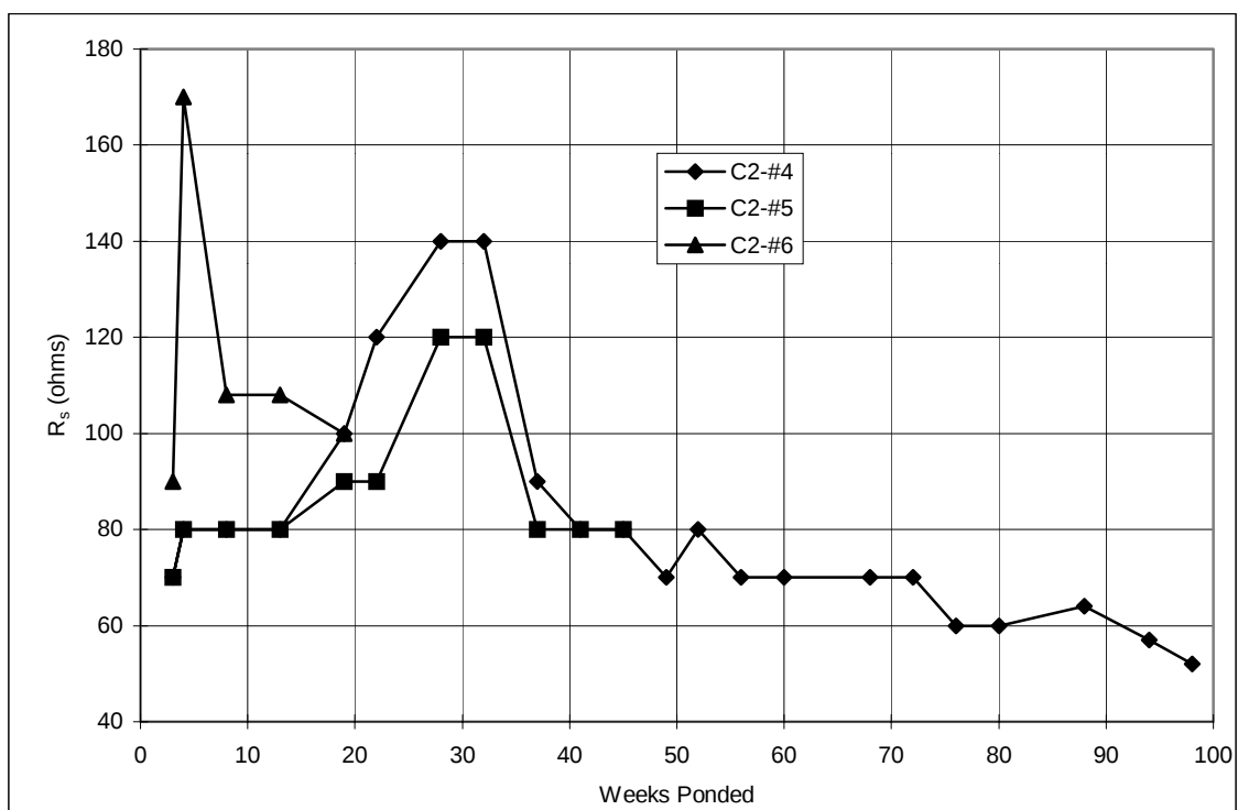
Figure A.19 Solution resistance, slabs: Control 2-unconnected.
