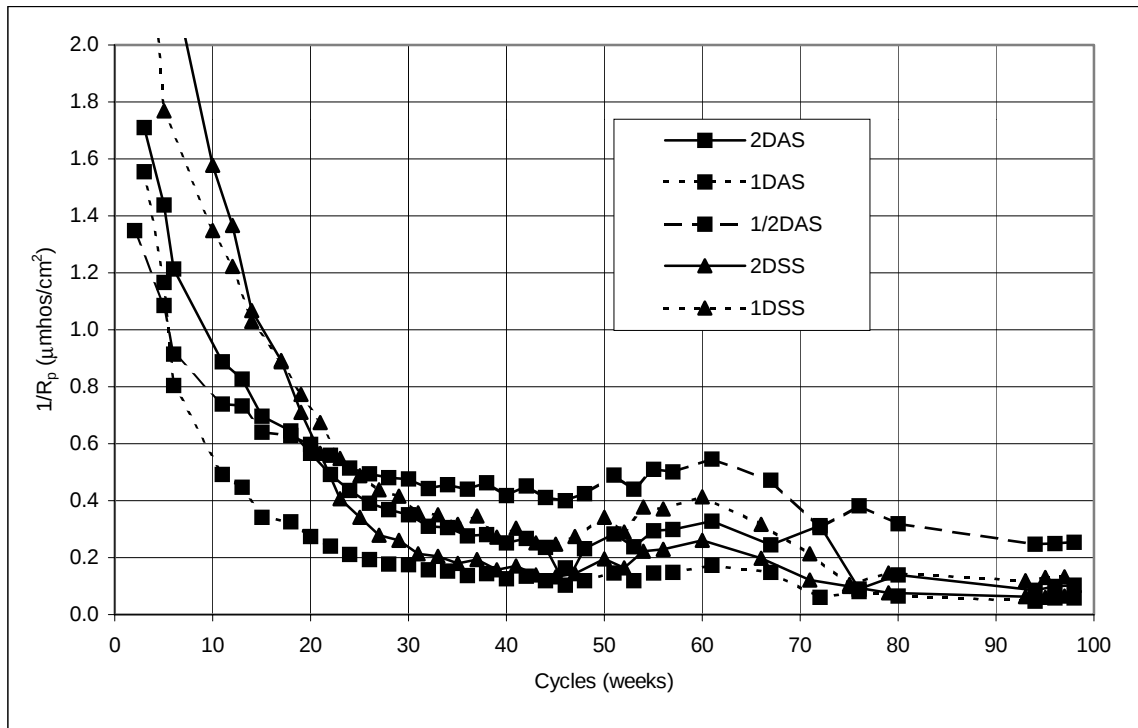
Figure 5.18 Corrosion rates, 3-inch cylinders: DAS and DSS.
