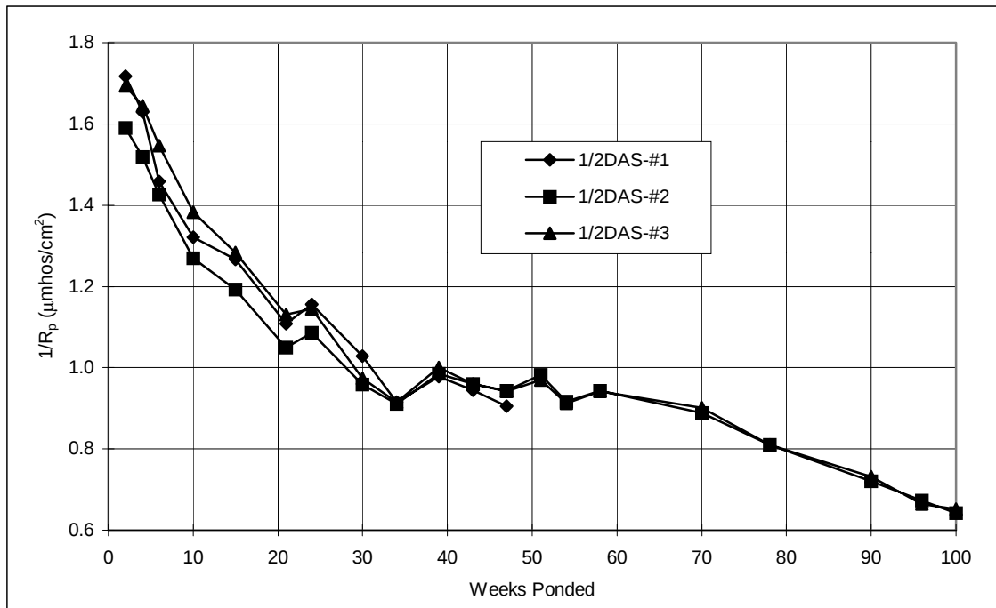
Figure A.60 Corrosion rate, slabs: 1/2%DAS.
