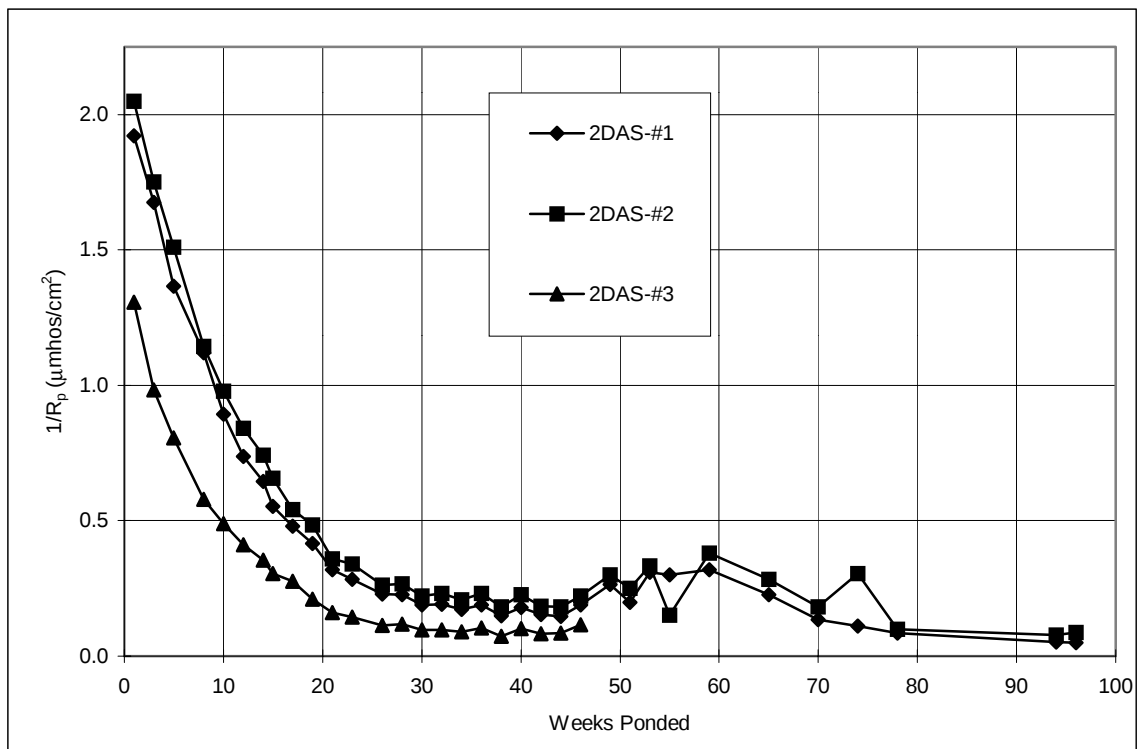
Figure A.40 Corrosion rate, 2-inch diameter lollipops: 2%DAS.
