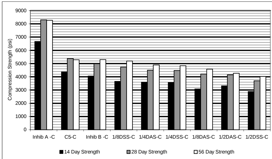
Figure 5.1 Compression Strengths in descending order for 28 day strength.
