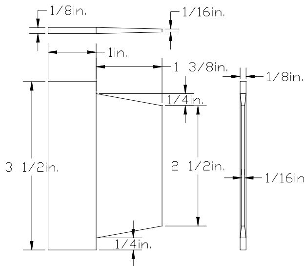
Figure 4.3 Wedge used to cast pre-formed crack.
