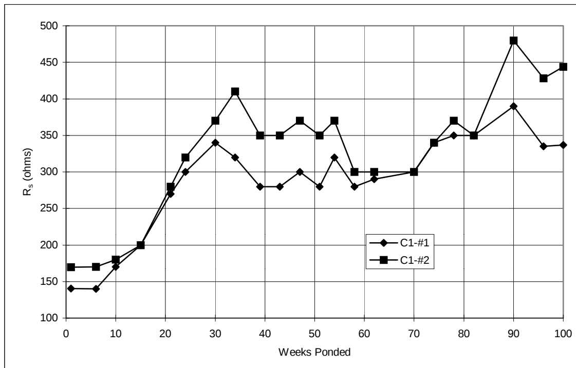
Figure A.17 Solution resistance, slabs: Control 1.
