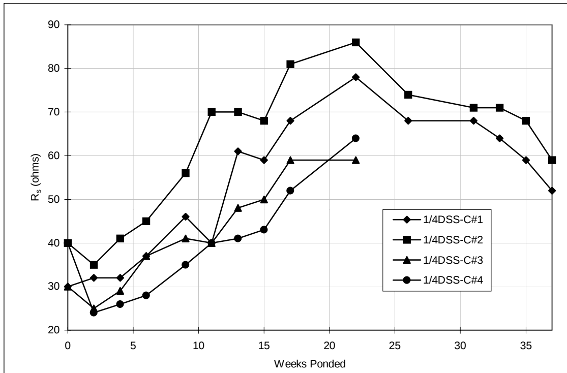
Figure A.35 Solution resistance, pre-cracked lollipops: 1/4%DSS.
