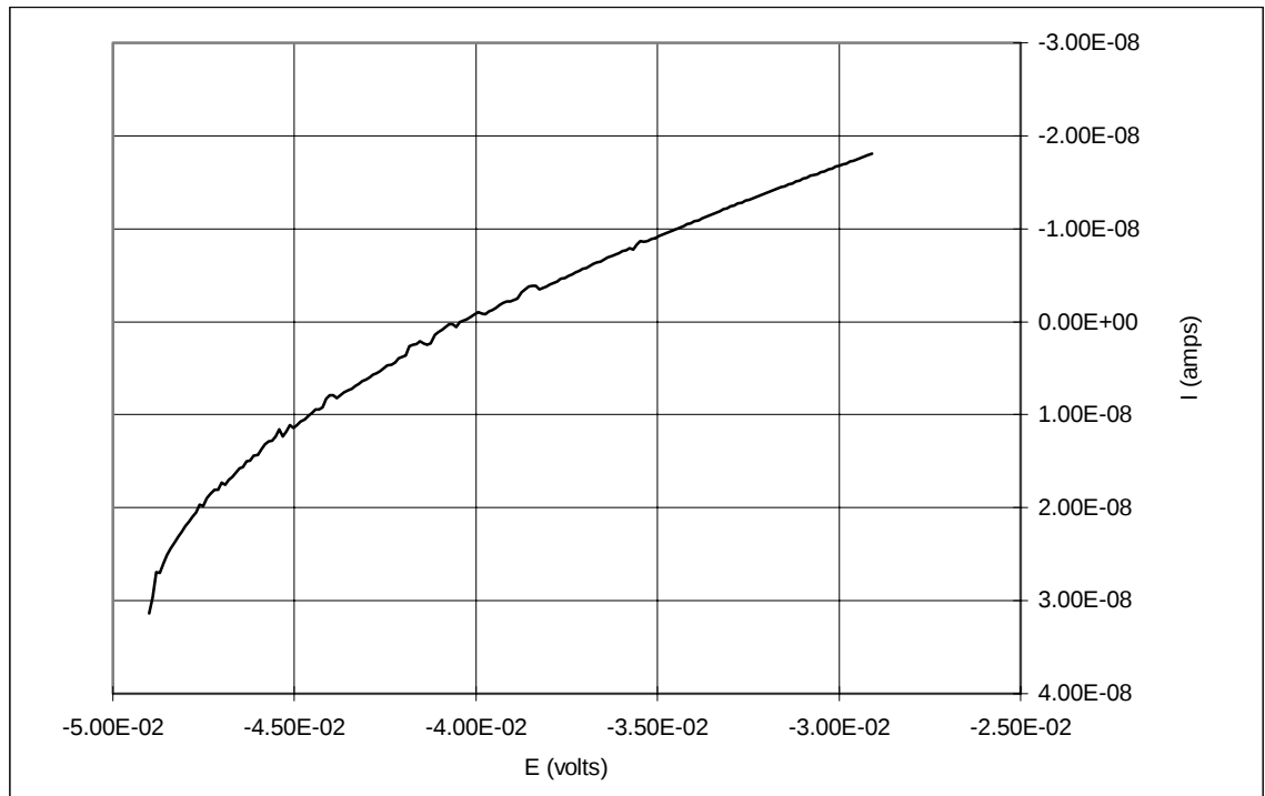
Figure 4.10 Polarization curve for an actively corroding lollipop specimen.
