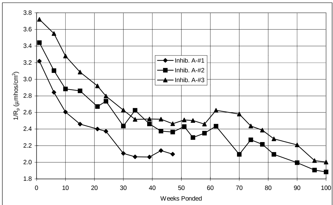
Figure A.56 Corrosion rate, slabs: Inhibitor A.
