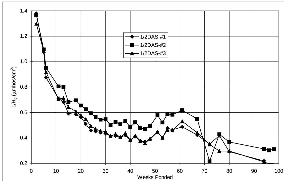
Figure A.50 Corrosion rate, 3-inch diameter lollipops: 1/2%DAS.
