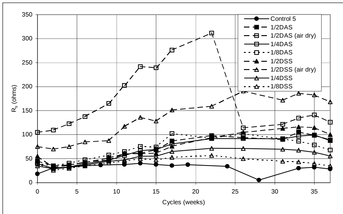
Figure 5.14 Solution resistance, pre-cracked cylinders: Control, DAS, and DSS.
