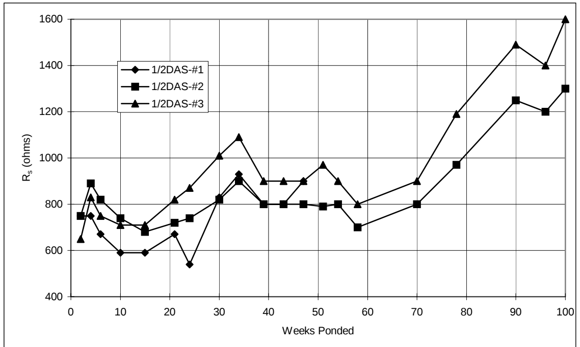
Figure A.24 Solution resistance, slabs: 1/2%DAS.
