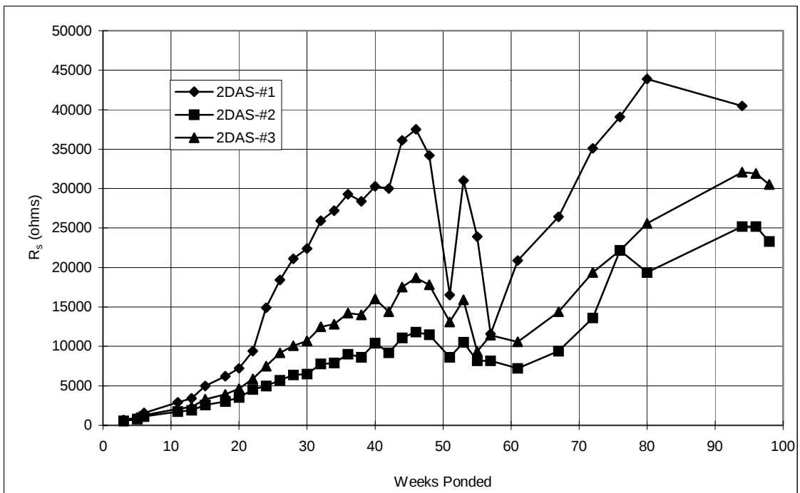
Figure A.12 Solution resistance, 3-inch diameter lollipops: 2%DAS.
