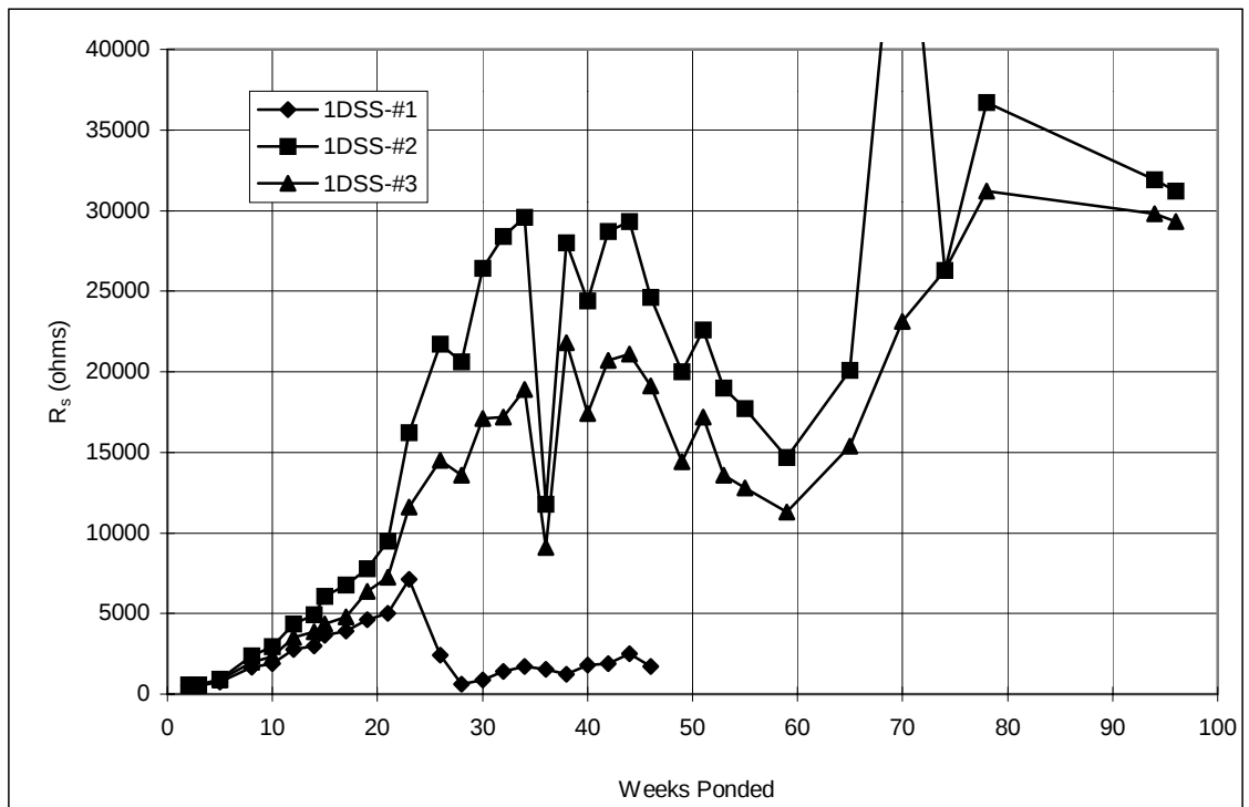
Figure A.8 Solution resistance, 2-inch diameter lollipops: 1%DSS.
