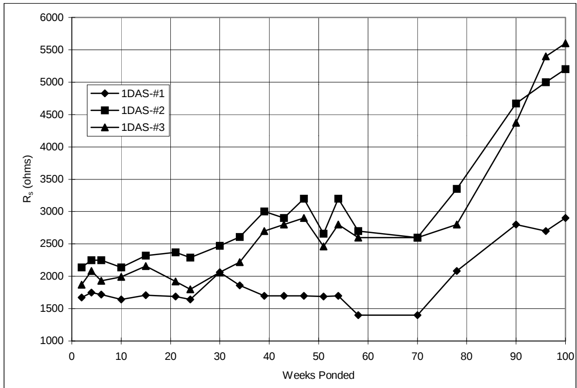
Figure A.23 Solution resistance, slabs: 1%DAS.
