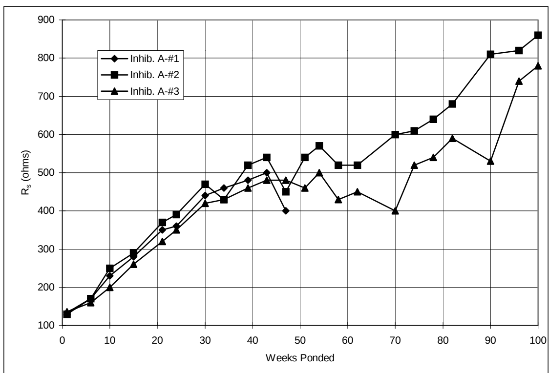
Figure A.20 Solution resistance, slabs: Inhibitor A.
