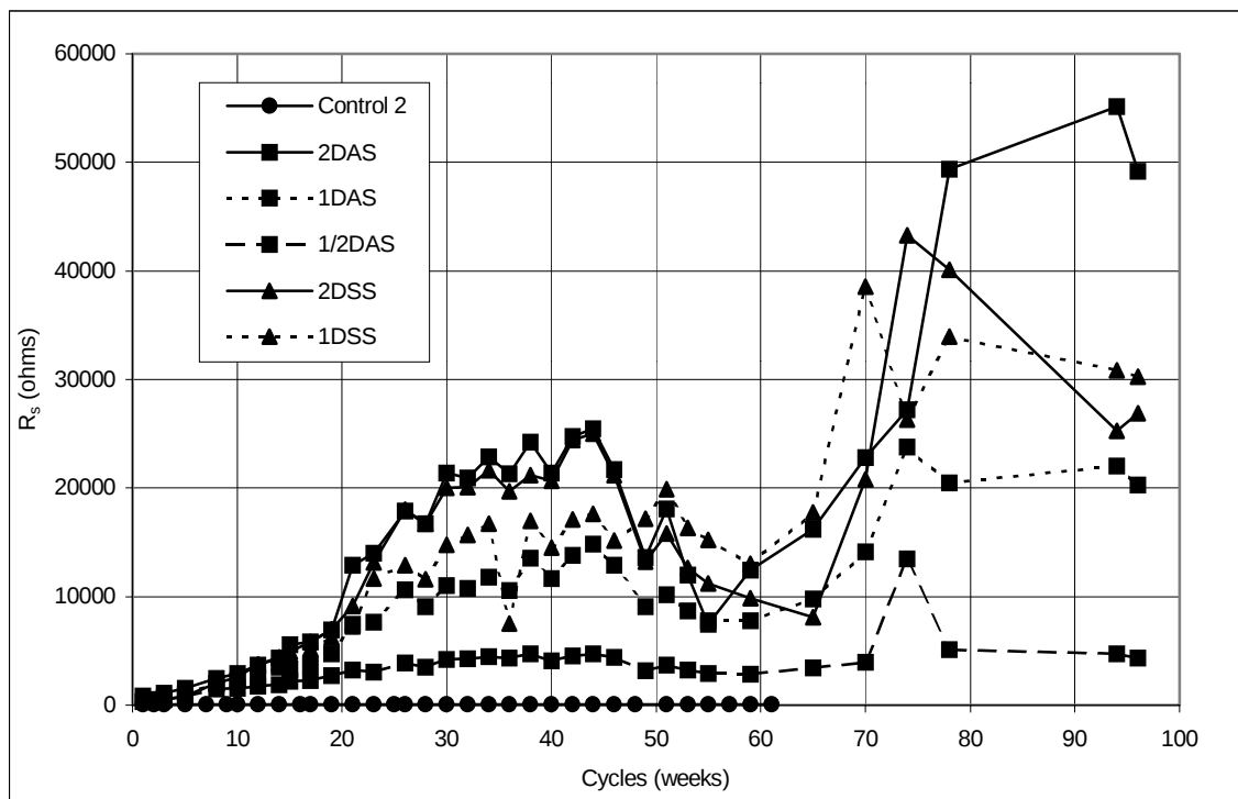
Figure 5.8 Solution Resistance, 2-inch cylinders: Control, DAS, and DSS
