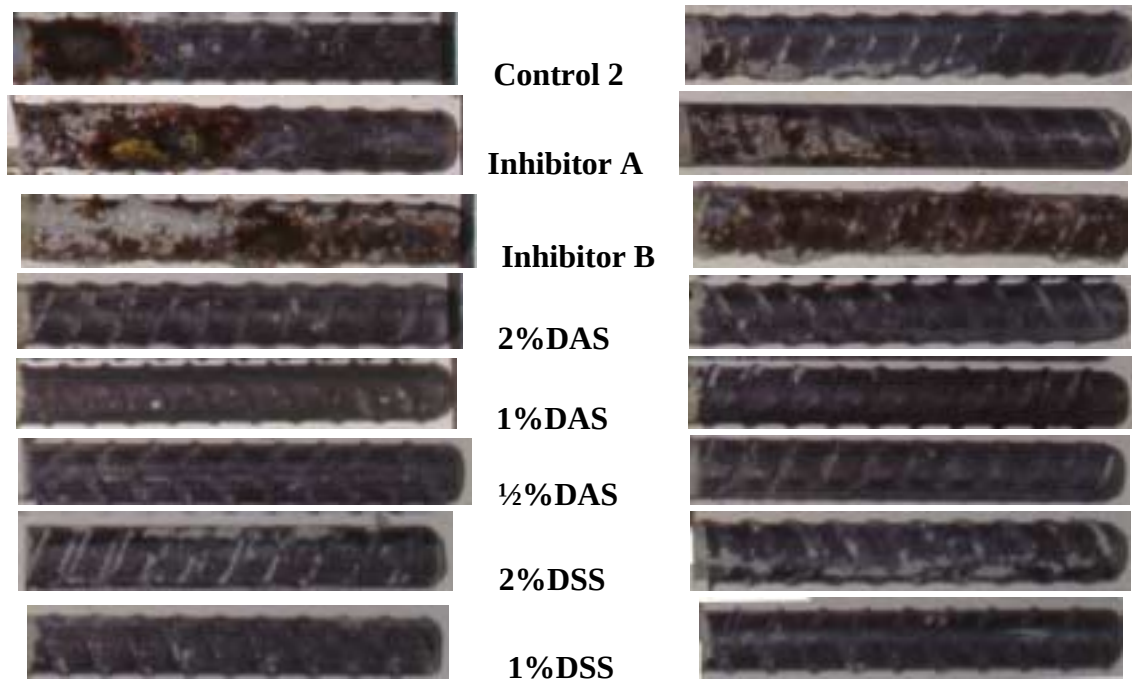
Figure 5.28 No. 4 rebar from the 3-inch specimens.
