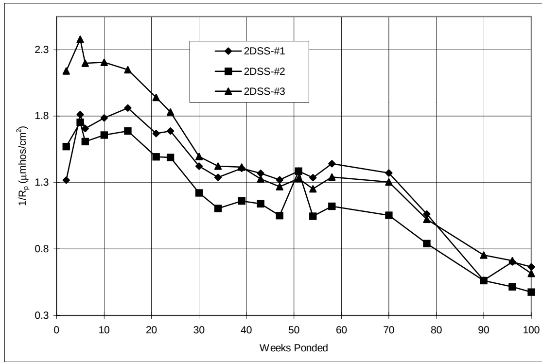
Figure A.61 Corrosion rate, slabs: 2%DSS.
