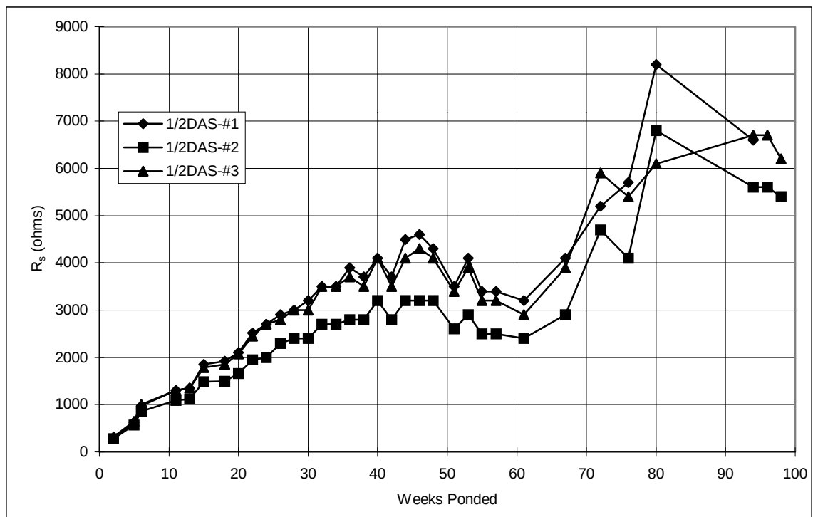
Figure A.14 Solution resistance, 3-inch diameter lollipops: 1/2%DAS.
