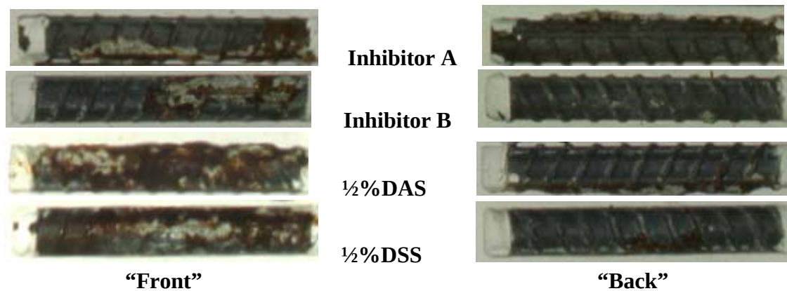
Figure 5.32 No. 4 rebar from the air-dried pre-cracked specimens.
