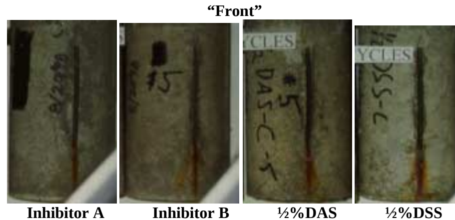
Figure 5.34 Final exterior appearance of the air-dried pre-cracked specimens. Only the “front” side is shown because this is where the corrosion was induced (the camera tripod leg hides the lower-right corner of the Inhibitors A and B specimens).
