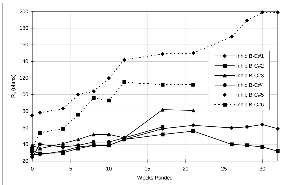
Figure A.30 Solution resistance, pre-cracked lollipops: Inhibitor B.
