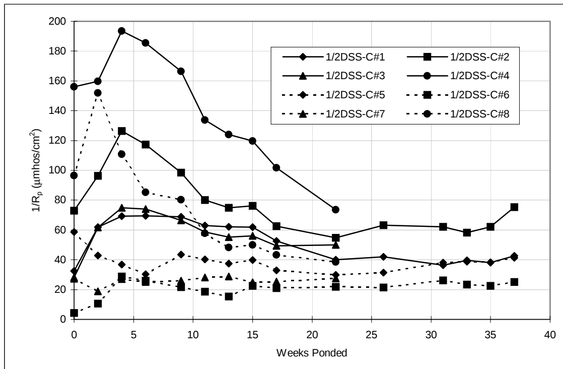
Figure A.70 Corrosion rate, pre-cracked lollipops: 1/2%DSS.
