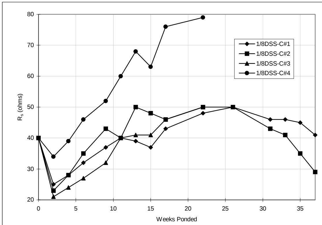
Figure A.36 Solution resistance, pre-cracked lollipops: 1/8%DSS.
