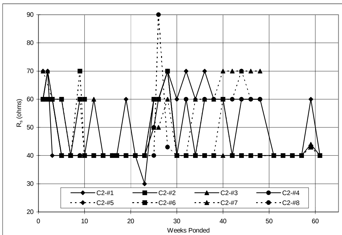
Figure A.1 Solution resistance, 2-inch diameter lollipops: Control.
