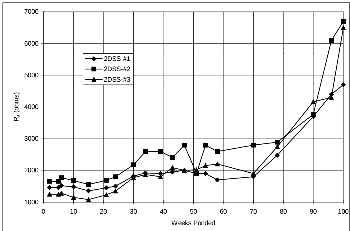
Figure A.25 Solution resistance, slabs: 2%DSS.
