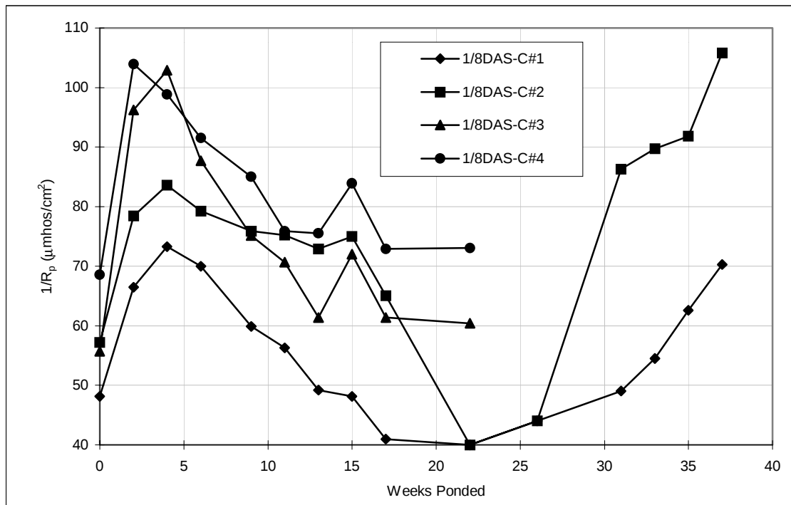
Figure A.69 Corrosion rate, pre-cracked lollipops: 1/8%DAS.
