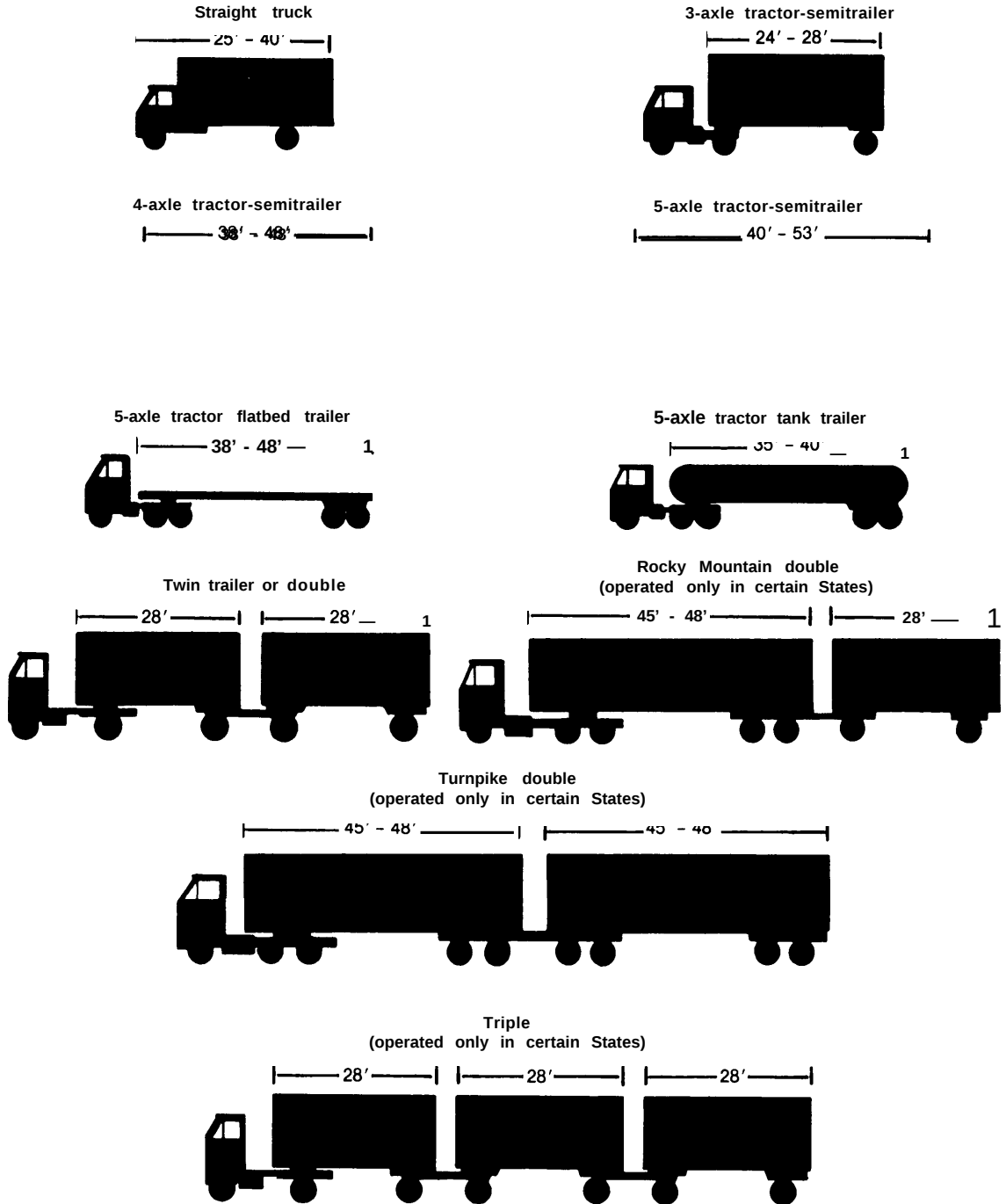
Figure 3-I—Heavy Truck Configurations
