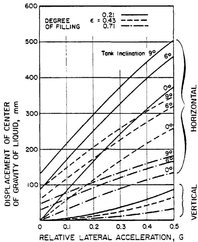
Figure 3a. Horizontal and vertical displacement of center of gravity of liquid in containers with circular cross-section at various tank angles-of-inclination.[12]
