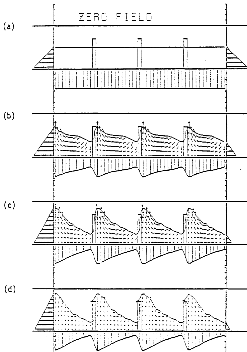
Figure 27. Longitudinal sloshing in a tank with V2 baffle - d=2 ft, a=8.05 ft/s 2 (a) t=0.0 sec (b) t=0.41 sec (c) t=0.71 sec (d) t=0.80 sec [13]
