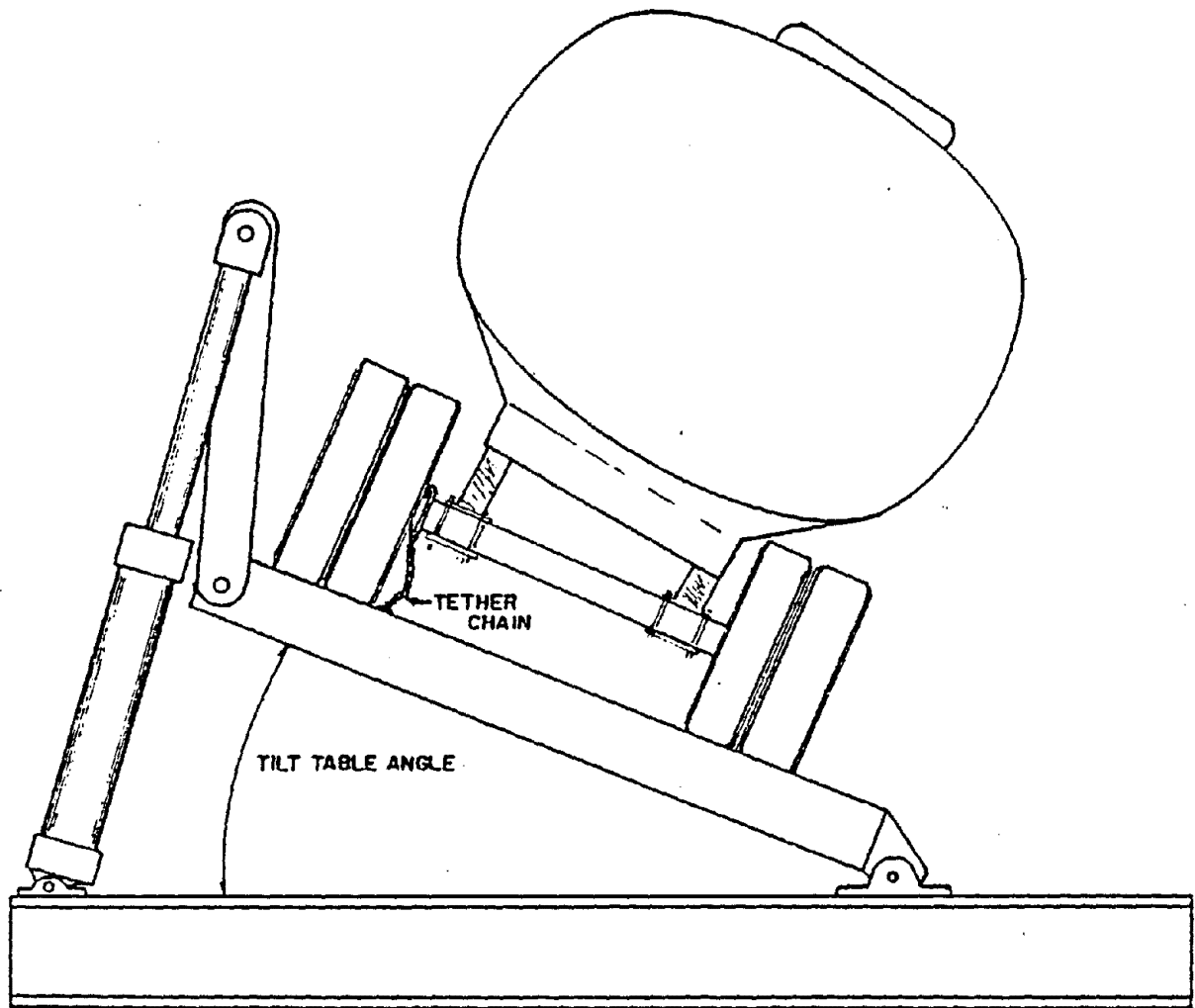
Figure 29. Tilt-table concept for measuring static rollover threshold.
