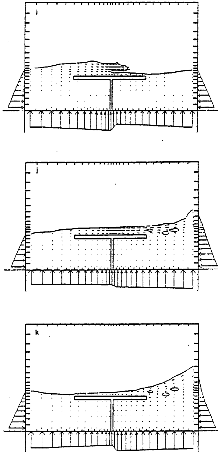
Figure 26. Flow field - tee baffle. [13]
