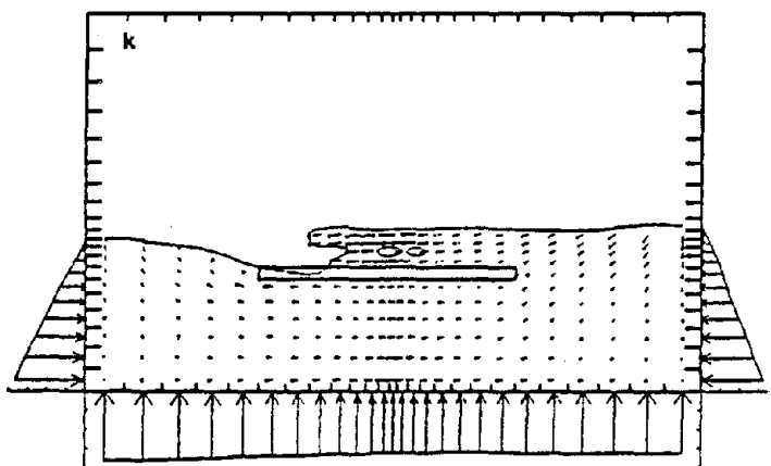
Figure 25. Flow field - partial horizontal baffle. [13]
