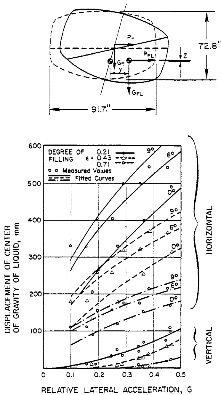
Figure 3b. Horizontal and vertical displacement of center of gravity in container with cross-section as shown above. [12]
