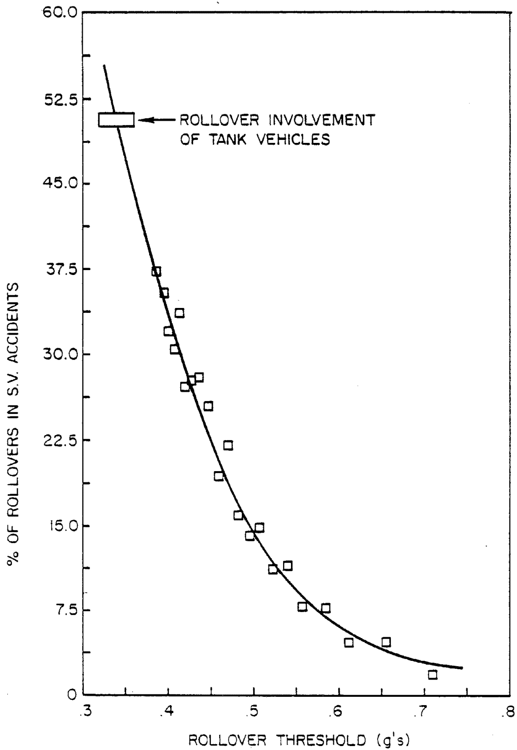
Figure 28. Relationship between rollover threshold and rollover accident involvement. (Based on BMCS accident data for the years 1976-78.) [25]
