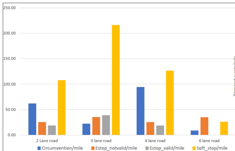
Figure 3-10. Triggered event rates by lane configuration
