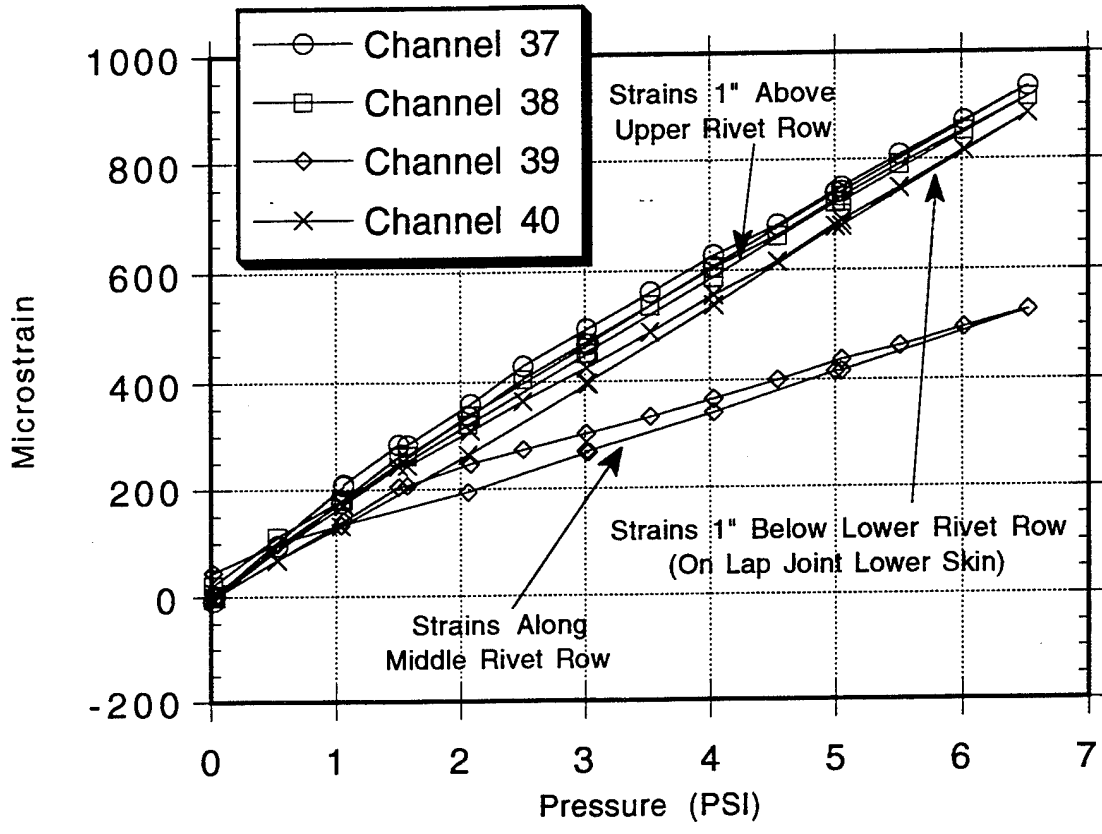
Figure 3.10. External Skin Hoop Strains Along Frame at S-10L, BS480. (Refer to Figure A.5.)
