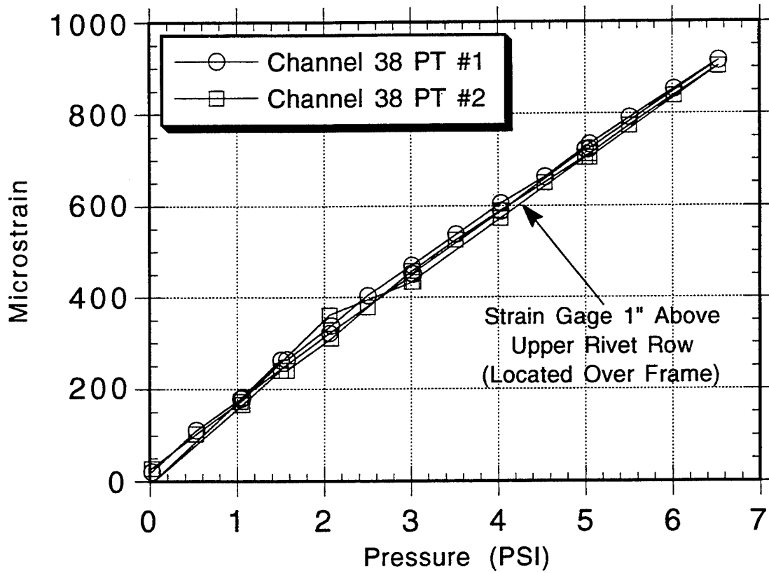
Figure 3.41. Hoop Strains Measured 1 Inch Above Upper Rivet Row at S-10L, BS480 from Tests 1 and 2. (Refer to Figure A.5.)
