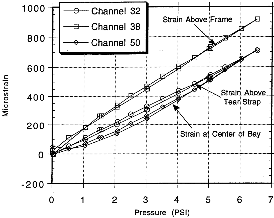
Figure 3.16. External Skin Hoop Strains 1 Inch Above Upper Rivet Row at S-10L Lap Splice Bay Between BS470 and BS480. (Refer to Figure A.5.)
