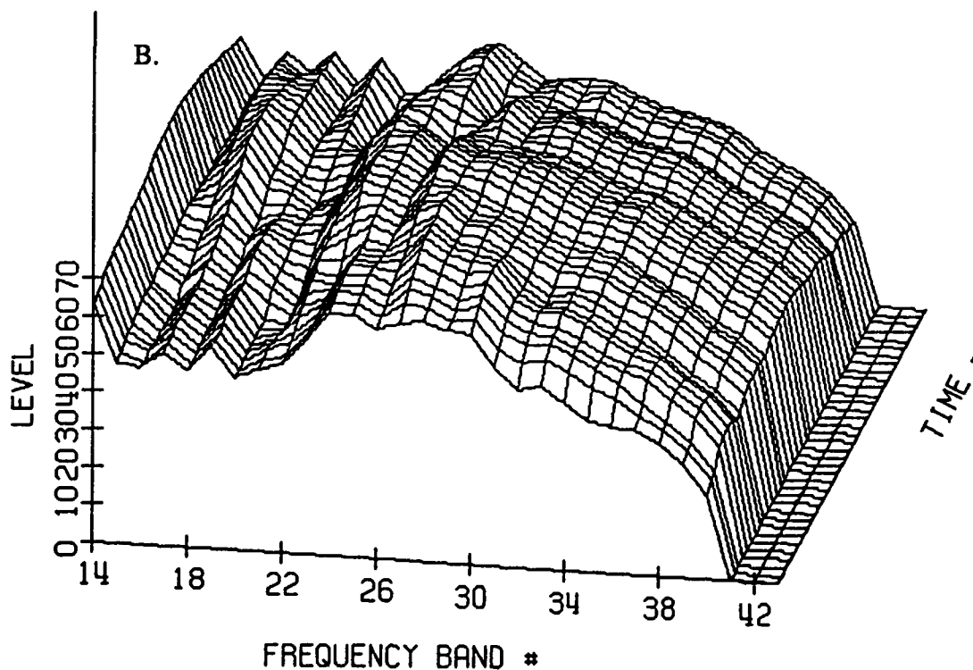
FIGURE C-D-2-1: EVENT B18 - APPROACH - 07/23/91 SCHWEIZER 300 - CONFIGURATION D SIDELINE 150 m WEST - AS MEASURED
