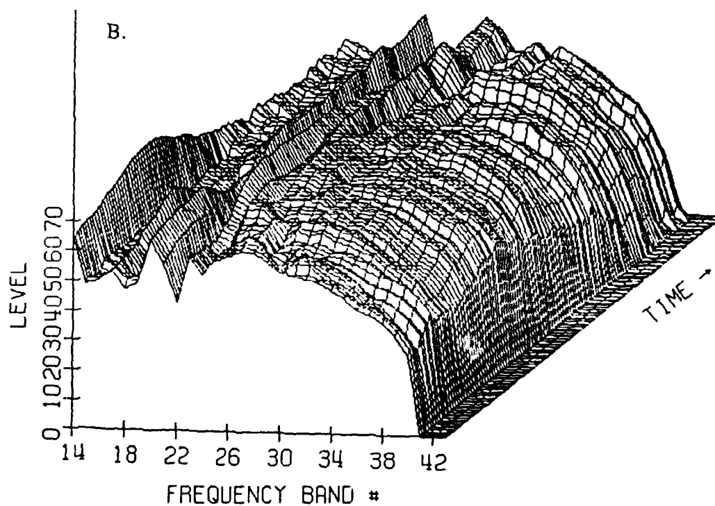
FIGURE C-A-2-2: EVENT C8 - TAKEOFF - 07/22/91 SCHWEIZER 300 - CONFIGURATION A SIDELINE 150 m WEST - AS MEASURED
