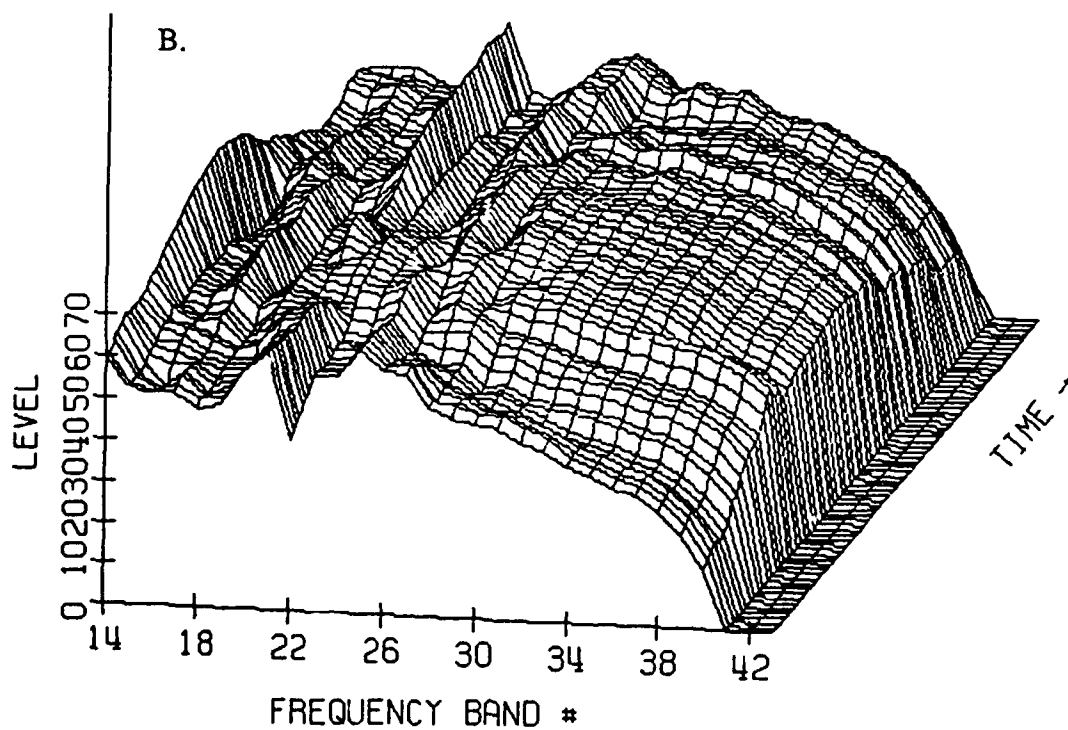
FIGURE C-A-2-3: EVENT A1 - LEVEL FLYOVER - 07/22/91 SCHWEIZER 300 - CONFIGURATION A SIDELINE 150 m WEST - AS MEASURED
