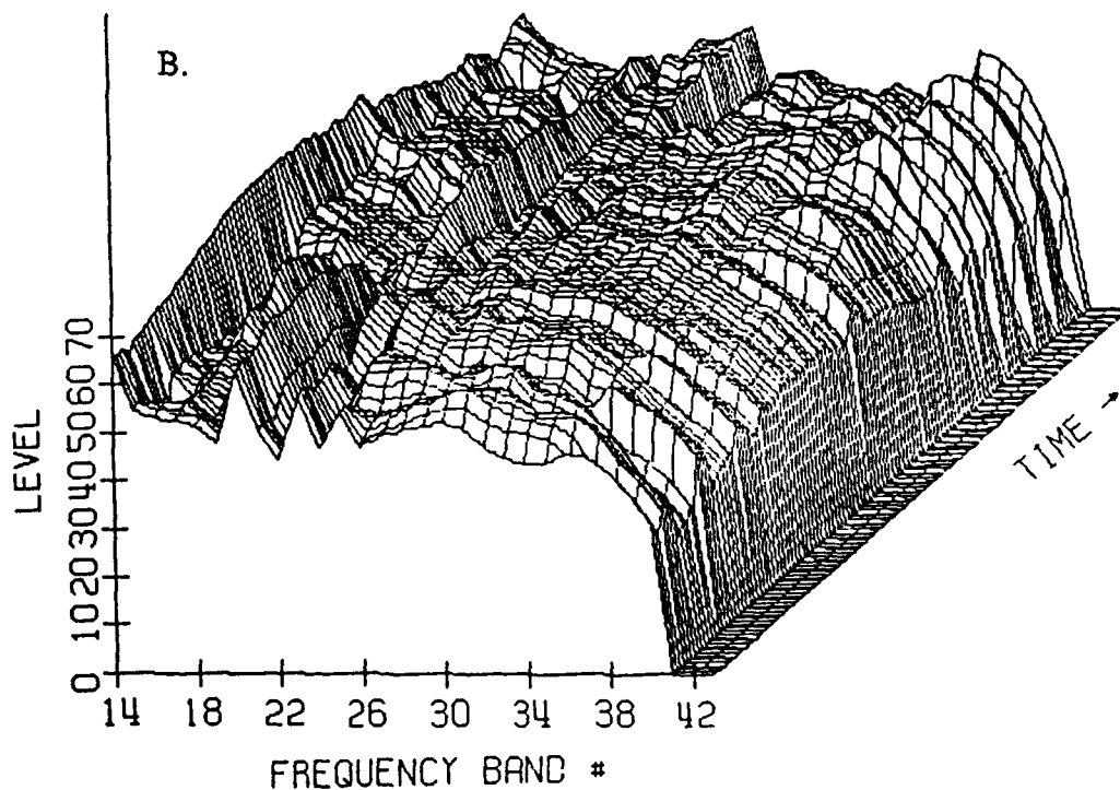
FIGURE C-B-2-2: EVENT C27 - TAKEOFF - 07/22/91 SCHWEIZER 300 - CONFIGURATION B SIDELINE 150 m WEST - AS MEASURED
