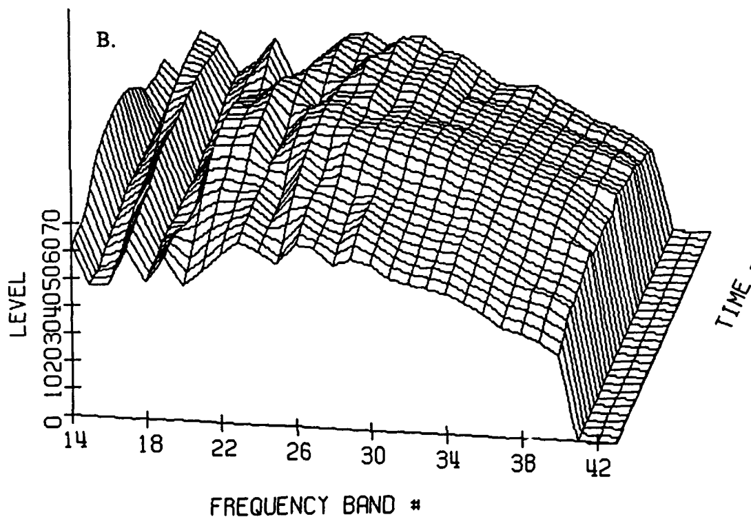
FIGURE C-E-1-1: EVENT B15 - APPROACH - 07/24/91 SCHWEIZER 300 - CONFIGURATION E CENTERLINE CENTER - AS MEASURED
