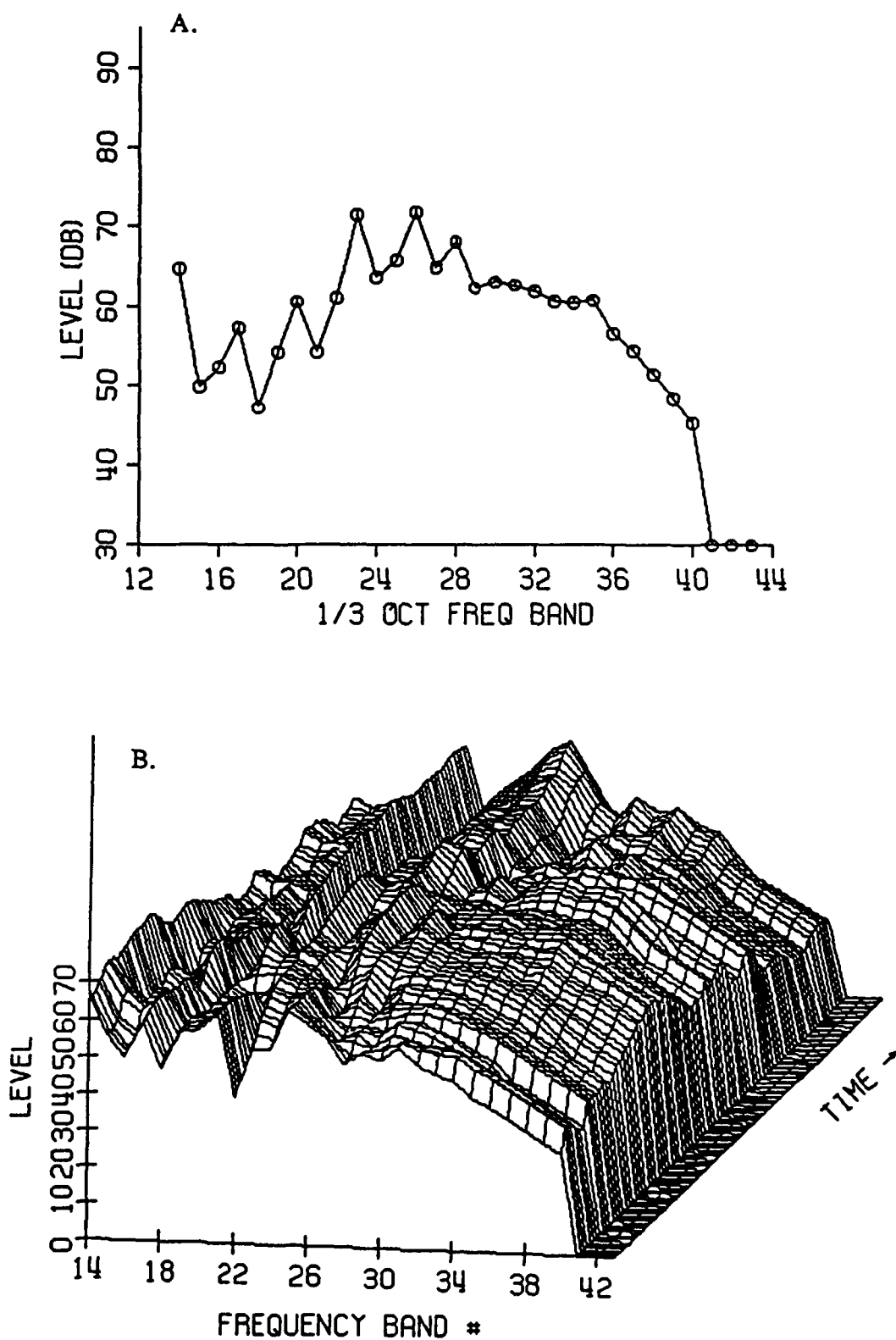
FIGURE C-A-3-3: EVENT A1 - LEVEL FLYOVER - 07/22/91 SCHWEIZER 300 - CONFIGURATION A SIDELINE 150 m EAST - AS MEASURED
