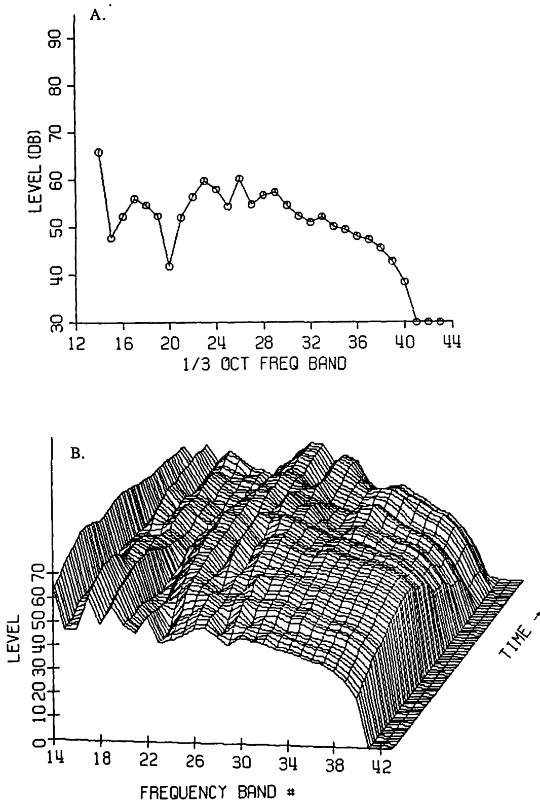
FIGURE C-I-3-2: EVENT C24 - TAKEOFF - 07/24/91 SCHWEIZER 330 - CONFIGURATION I SIDELINE 150 m EAST - AS MEASURED
