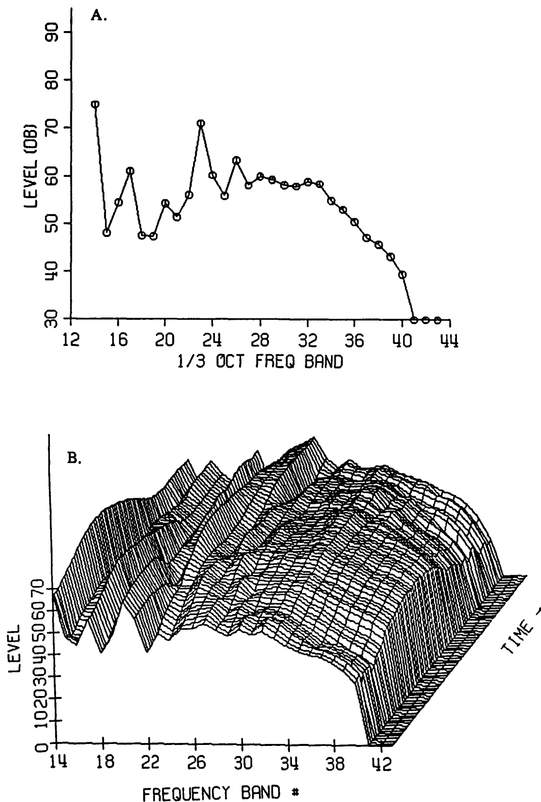
FIGURE C-E-2-2: EVENT E7 - TAKEOFF - 07/24/91 SCHWEIZER 300 - CONFIGURATION E SIDELINE 150 m WEST - AS MEASURED
