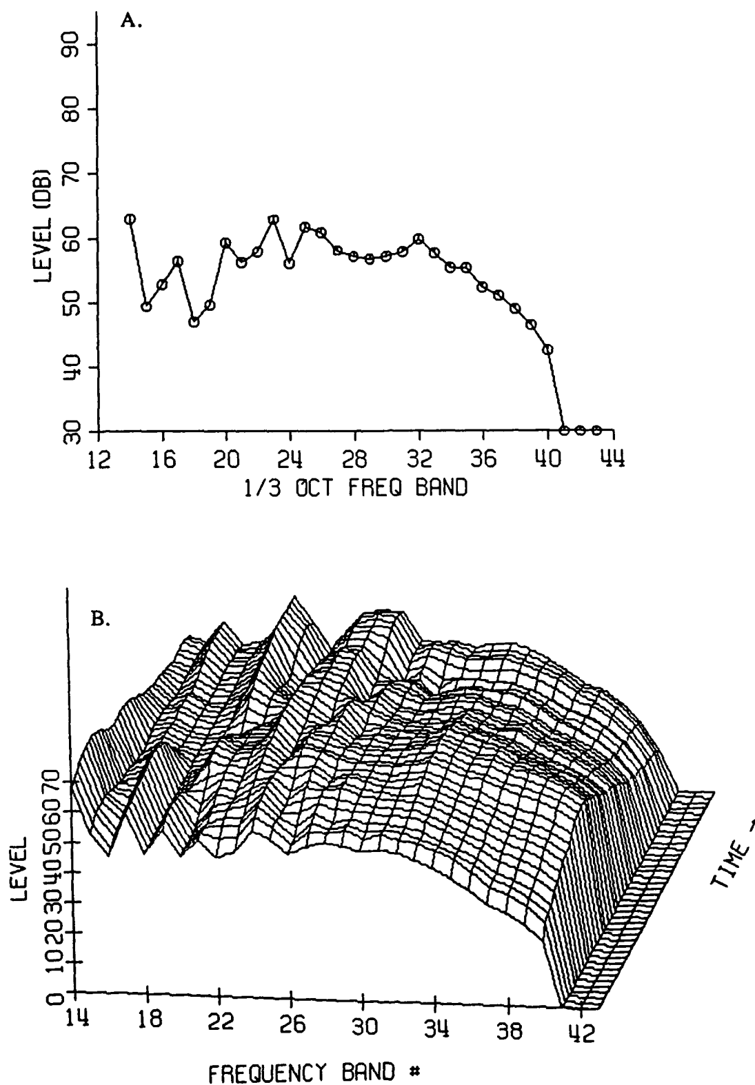
FIGURE C-C-3-3: EVENT A1 - LEVEL FLYOVER - 07/23/91 SCHWEIZER 300 - CONFIGURATION C SIDELINE 150 m EAST - AS MEASURED
