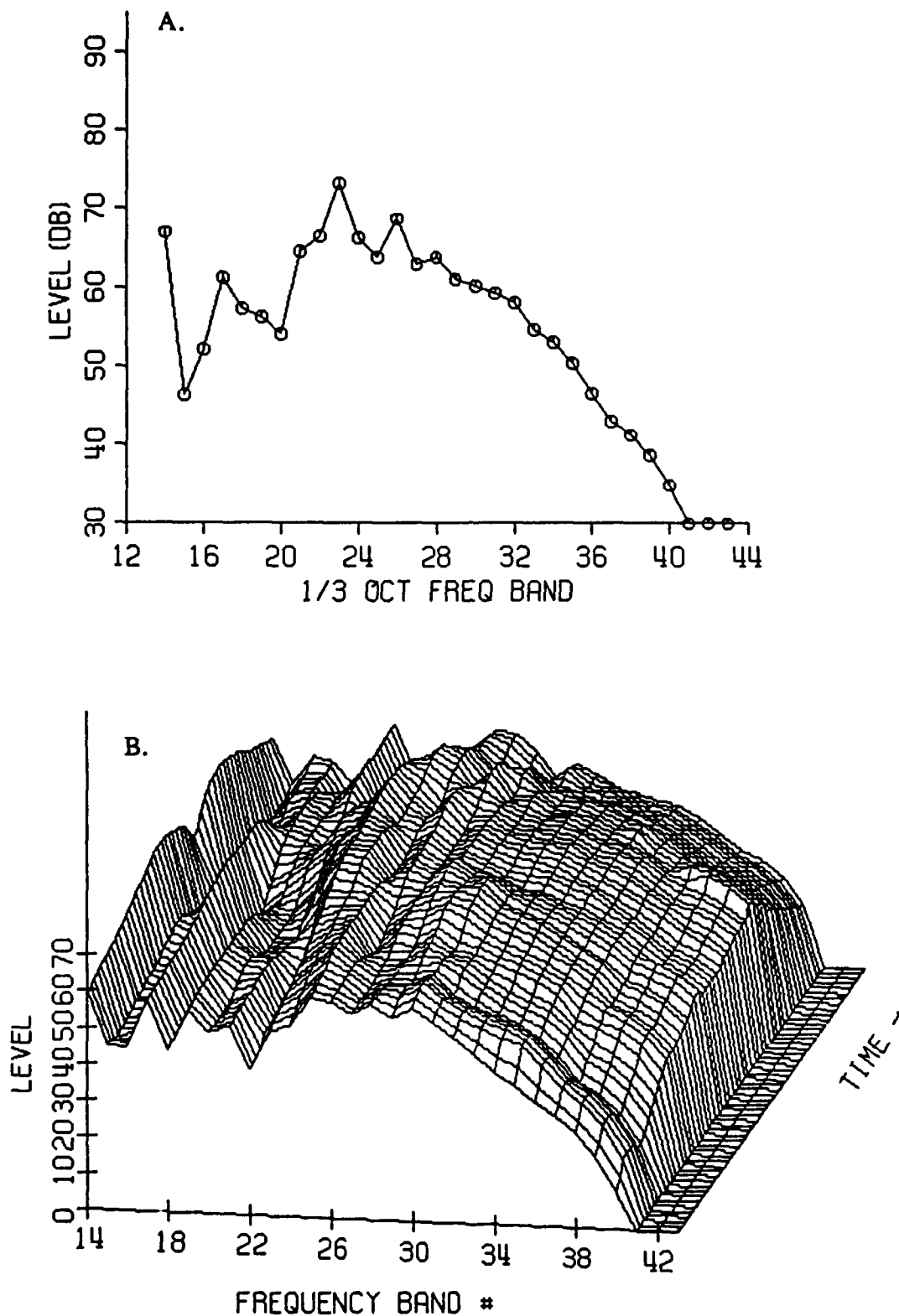
FIGURE C-E-3-1: EVENT B15 - APPROACH - 07/24/91 SCHWEIZER 300 - CONFIGURATION E SIDELINE 150 m EAST - AS MEASURED
