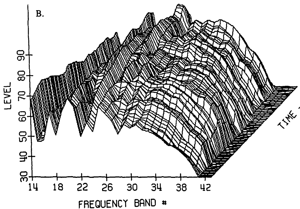
FIGURE C-A-3-2: EVENT C8 - TAKEOFF - 07/22/91 SCHWEIZER 300 - CONFIGURATION A SIDELINE 150 m EAST - AS MEASURED
