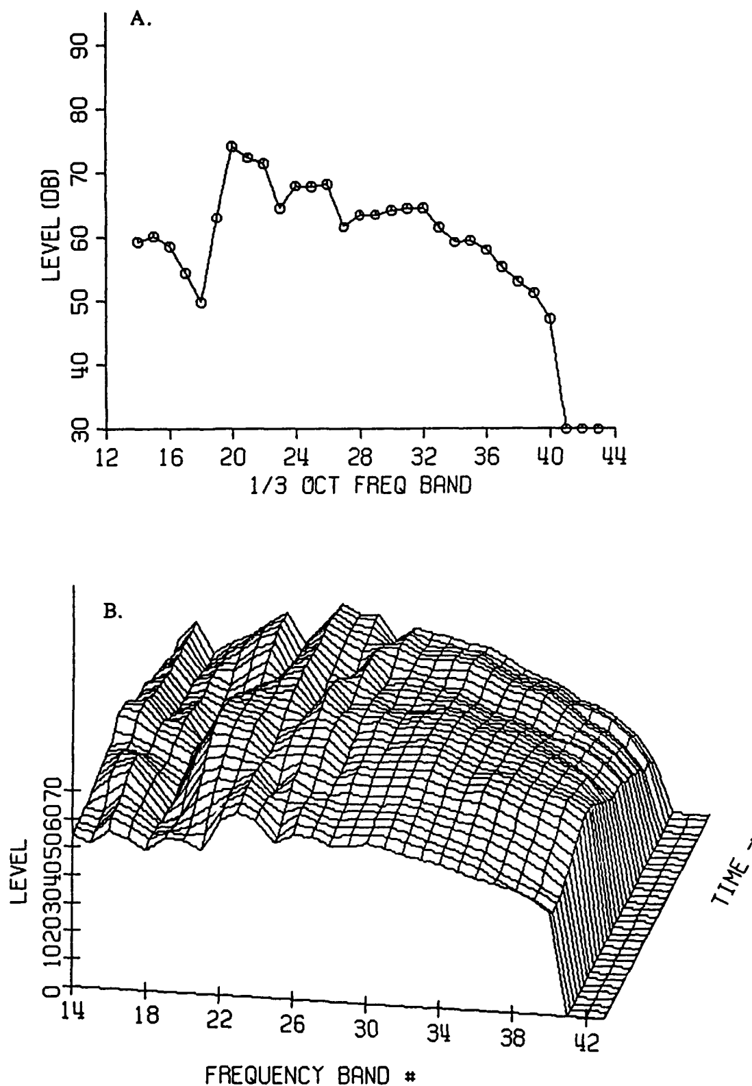
FIGURE C-J-1-2: EVENT CP22 - TAKEOFF - 07/26/91 ENSTROM 280 FX CENTERLINE CENTER - AS MEASURED
