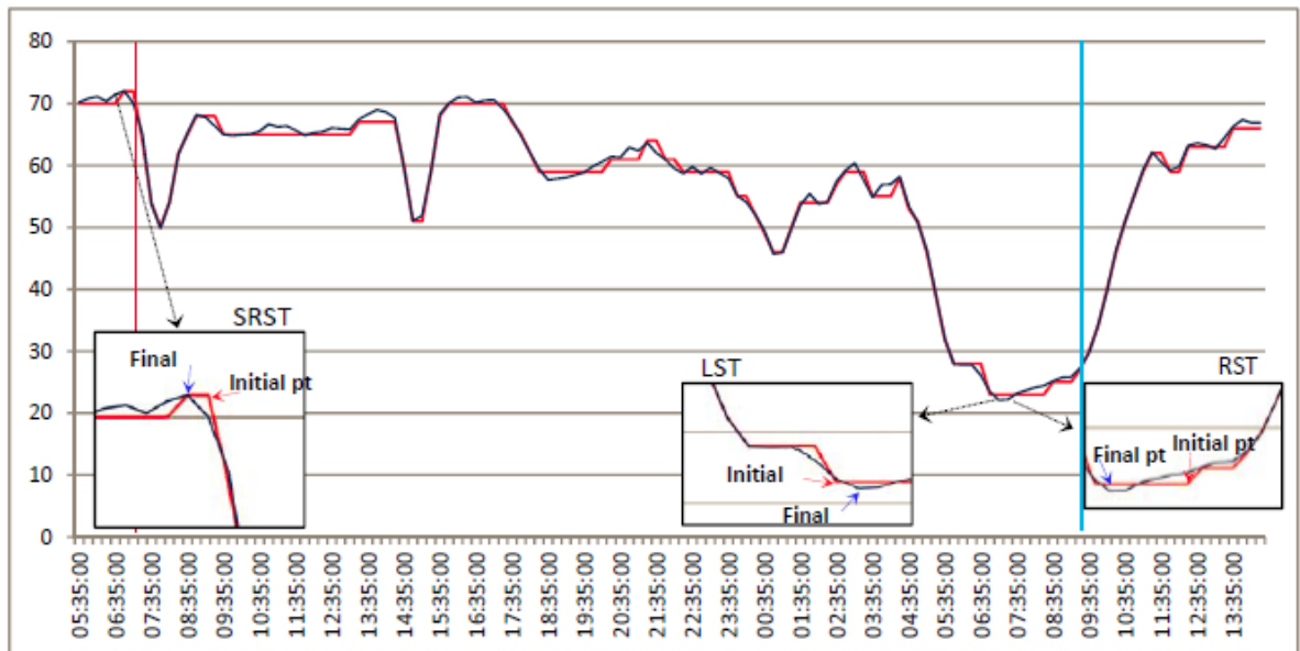
Figure 0.5 Identification of SRST, LST, RST of Speed Variation During Snow Event (Kwon et al., 2012)
