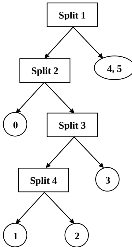
Figure 0.7 Calibrated Classification Tree for Site 00-0
