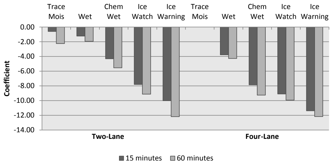
Figure 0.6 Effect of Road Surface Condition
