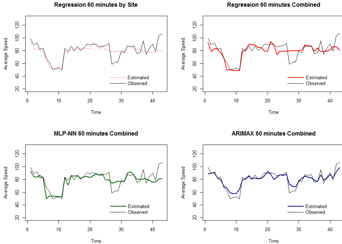
Figure 0.15 Estimation on Two-Lane Highways (Site 01-0 on Dec. 11th.-12th., 2010)
