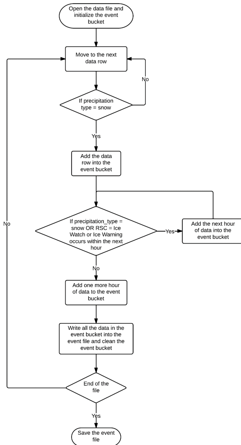
Figure 0.3 Snow Event Extraction Algorithm
