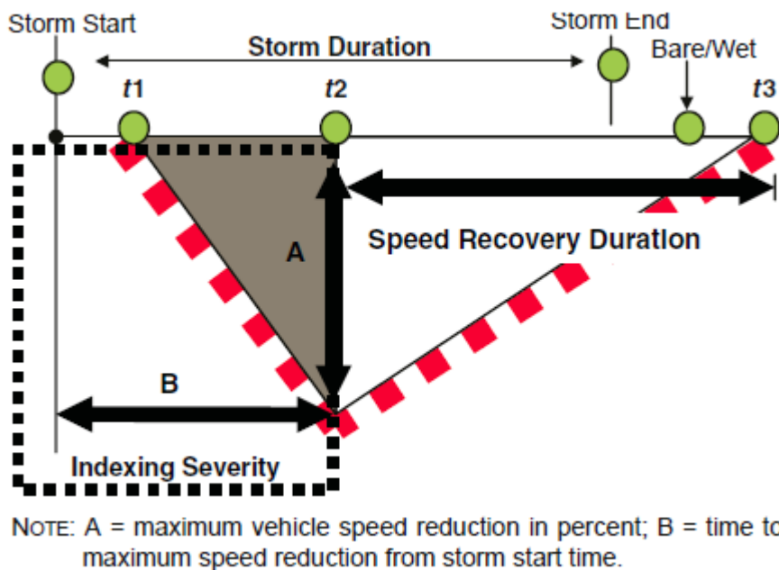
Figure 0.3 Speed Recovery Duration as a Performance Measure (Lee et al., 2008)
