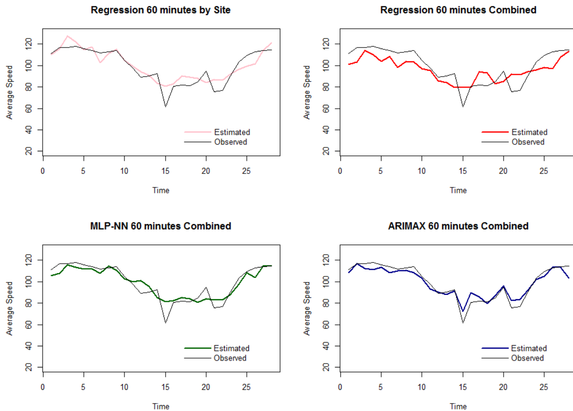
Figure 0.16 Estimation on Four-Lane Highways (Site 00-0 on Jan 10th., 2009)
