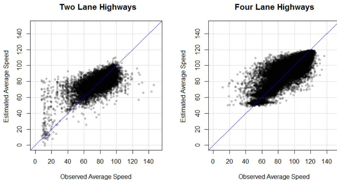
Figure 0.11 Observed vs. Estimated by MLP-NN 60 minutes Combined
