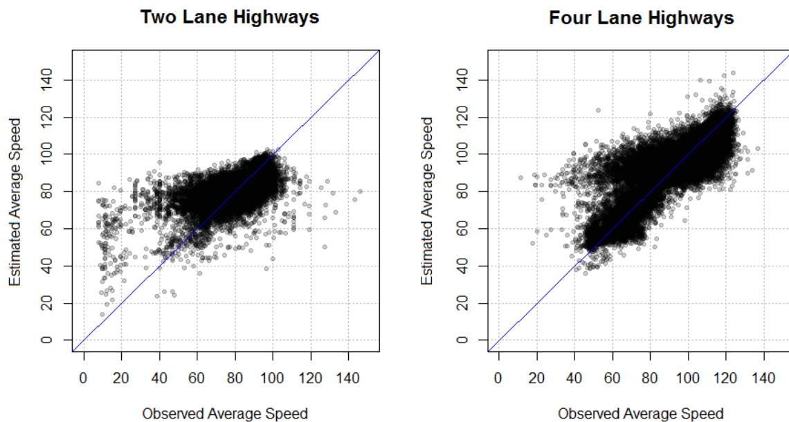
Figure 0.10 Observed vs. Estimated by Regression 60 minutes Combined
