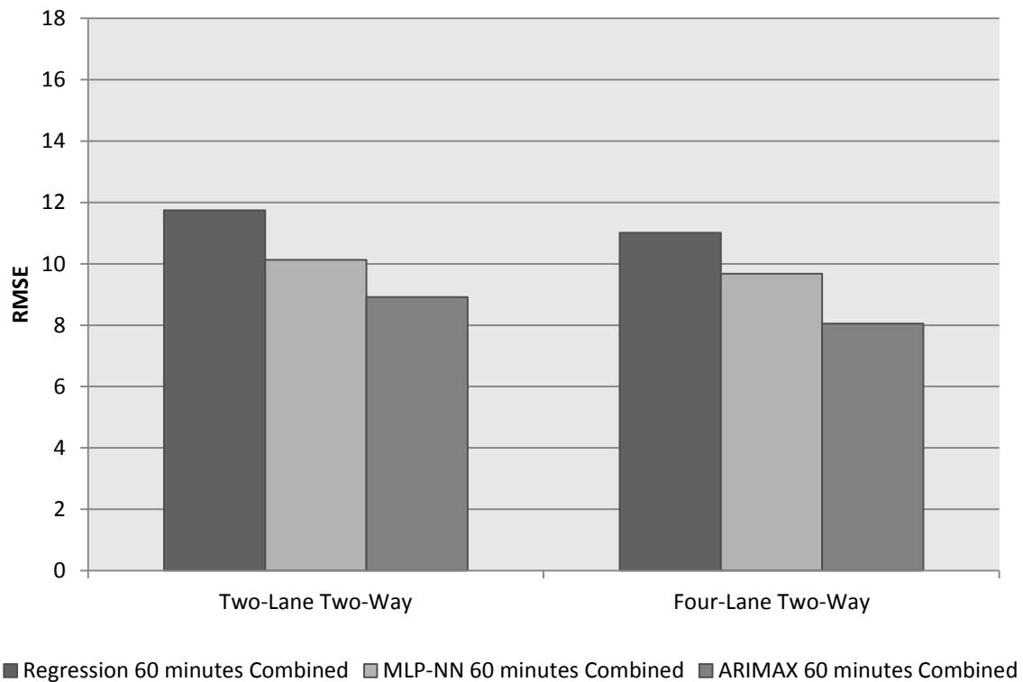
Figure 0.9 Overall RMSE Comparison for Combined Models
