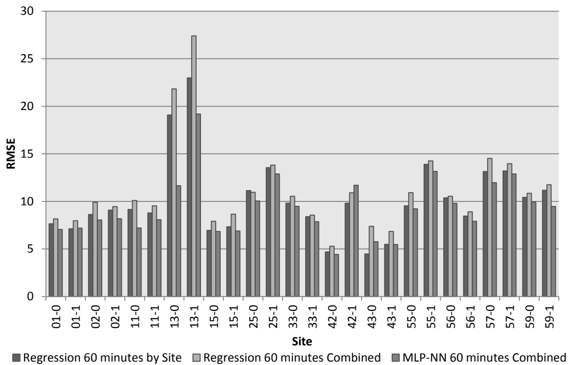
Figure 0.13 RMSE Comparison for Two-Lane Highways 10% Holdout Data
