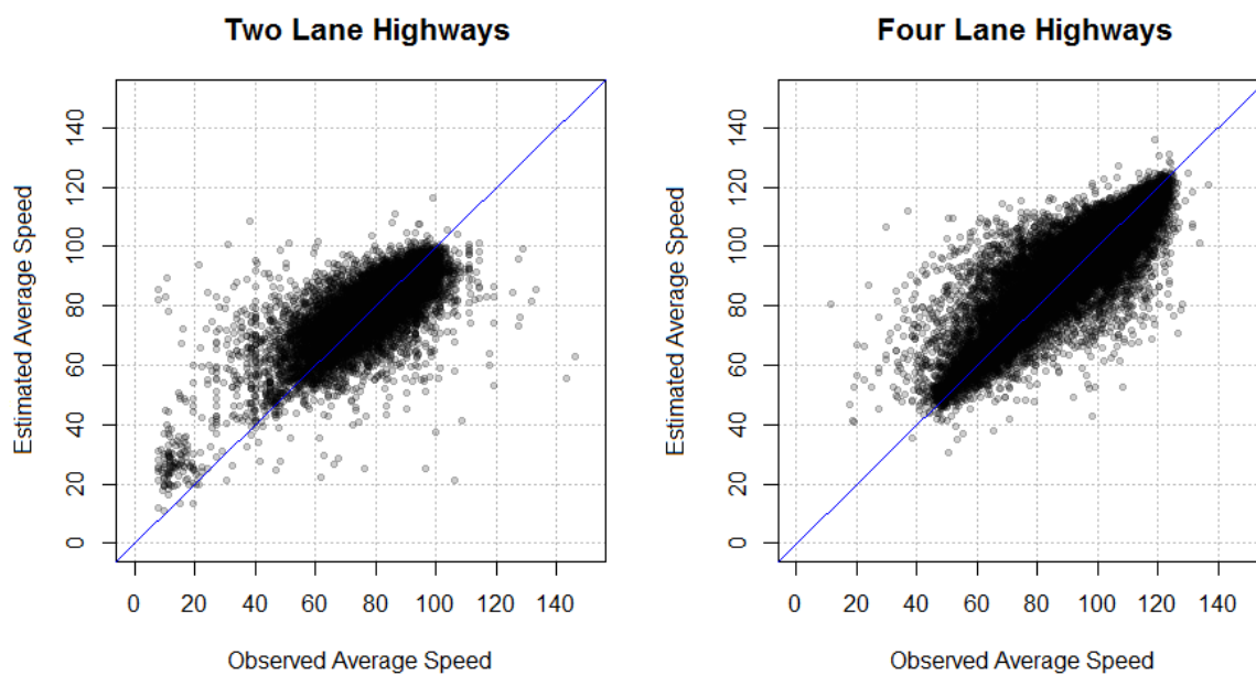
Figure 0.12 Observed vs. Estimated by ARIMAX 60 minutes Combined
