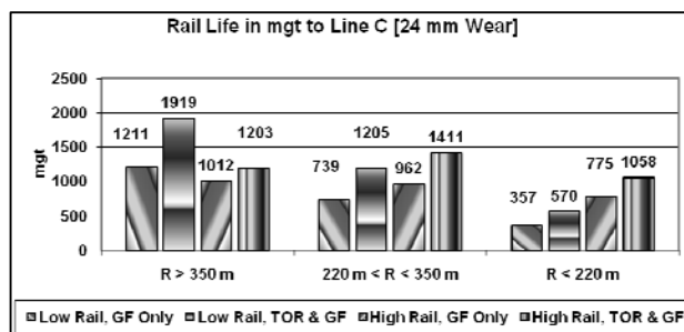
Figure 2 rail life in mgt for the high and low rail in 3 curvature ranges with 2 friction management strategies.
