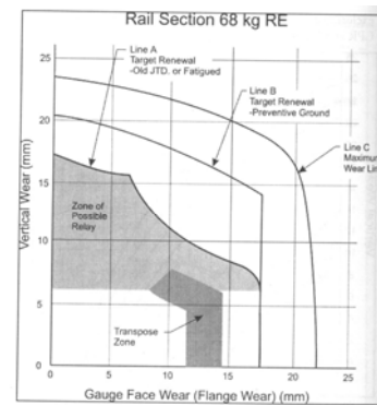
Figure 5.76: Rail Management Decision Zones for 68 kg/m (136 lb. RE)
