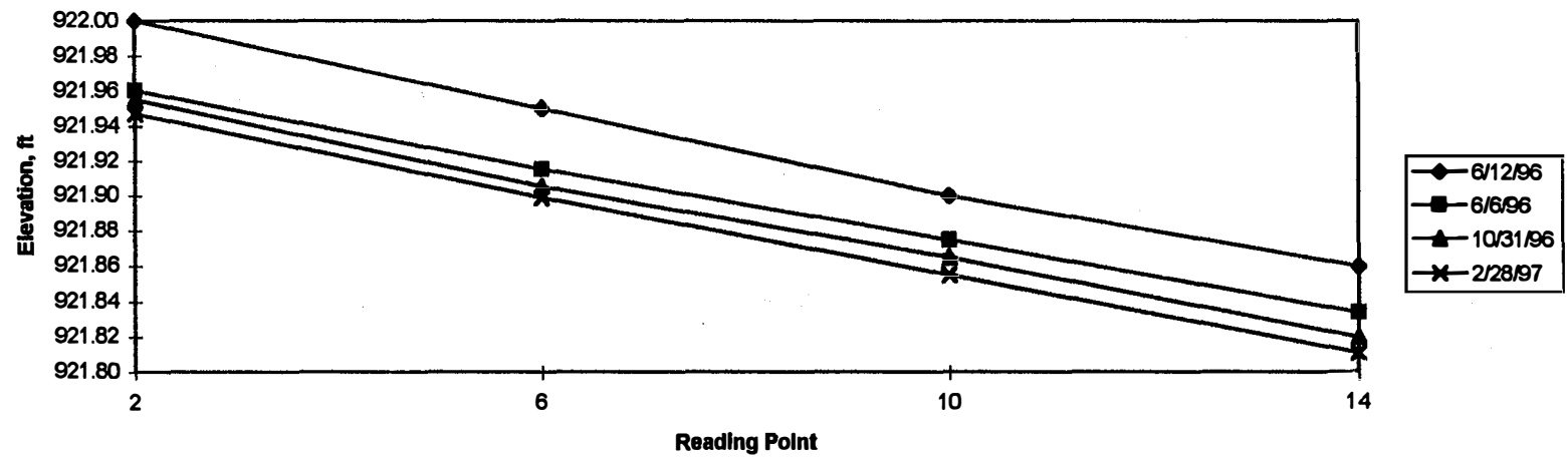
Surface Settlement Point Data, North Abutment Wall, Bridge C
