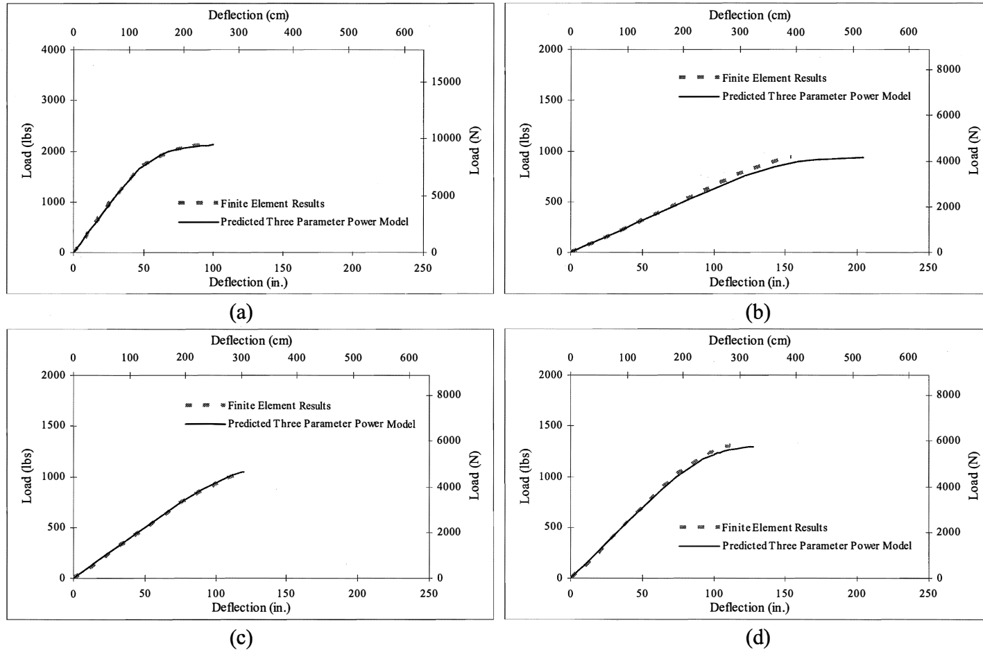
Figure C-4 Comparison of FEM model and predicted equation model for FRP poles:
