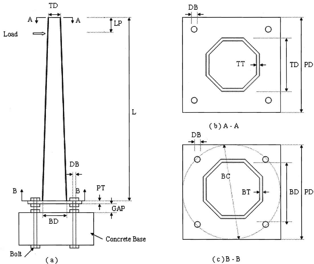
Figure 2.1 Dimensions of steel pole tested: (a) Front view; (b) Section A-A; (c) Section B-B
