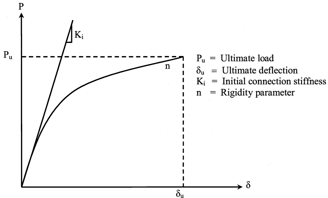
Figure 4.1 Typical load-deflection curve for poles
