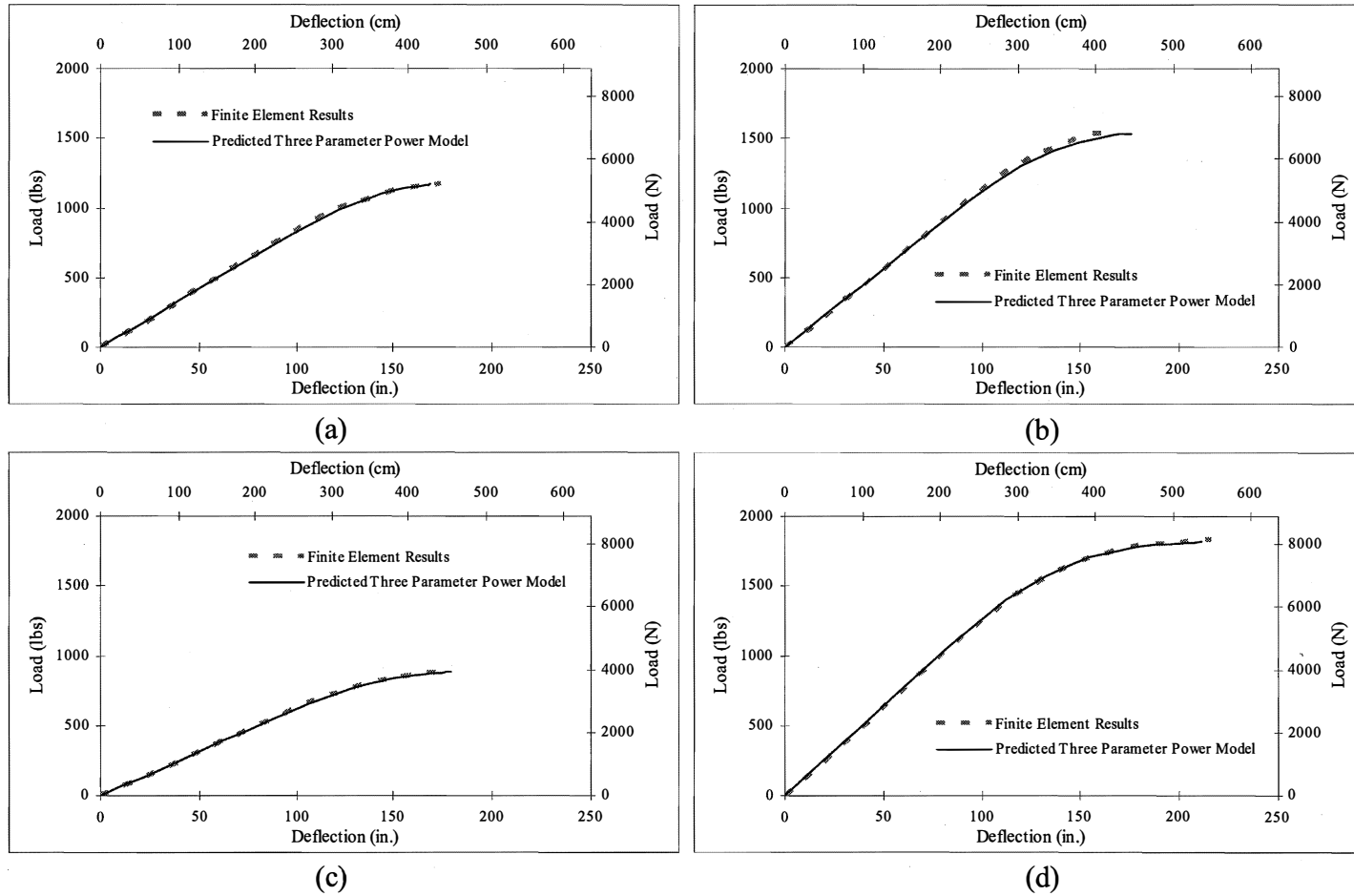
Figure C-8 Comparison of FEM model and predicted equation model for FRP poles: (a) F40-1-0.275-0.3-1.125-11-5.5-2.75-14.5-13-50-4; (b) F40-1-0.3-0.325-1.25-12.5-6-3-16.5-15-60-3.5; (c) F40-1-0.325-0.325-1-9-4.5-2.25-12-10.5-45-5; (d) F40-1-0.35-0.325-1.5-12-6.5-3.25-16.5-15-95-4
