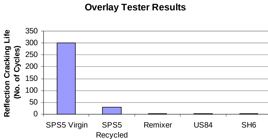
Figure 10. Overlay Tester Results from TxDOT Projects.
