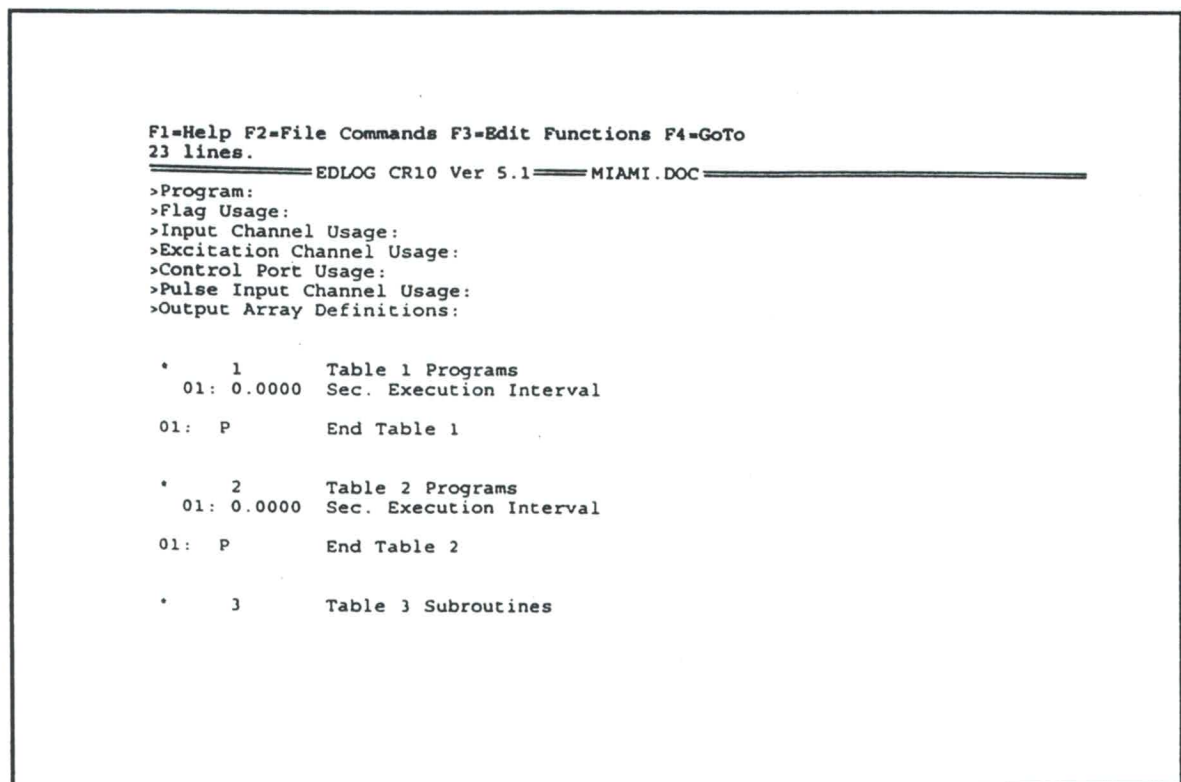
Fig. C-7 View of file newly created and opened with EDLOG
