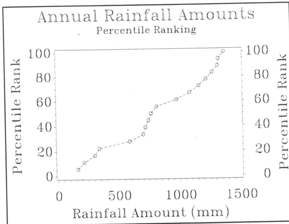
Fig. 5.32 Percentile distribution of annual rainfall amounts
