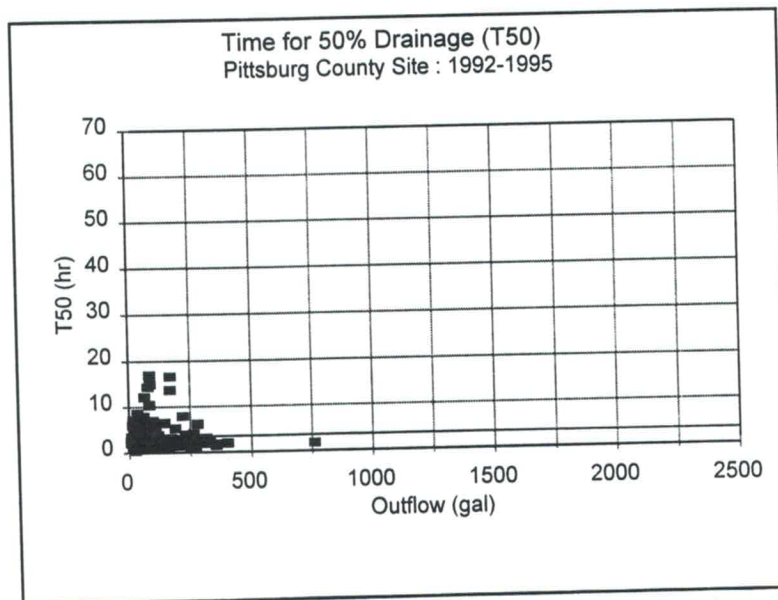
Fig. 6.22 Time required for 50% drainage - Pittsburg county site, 1992-1995
