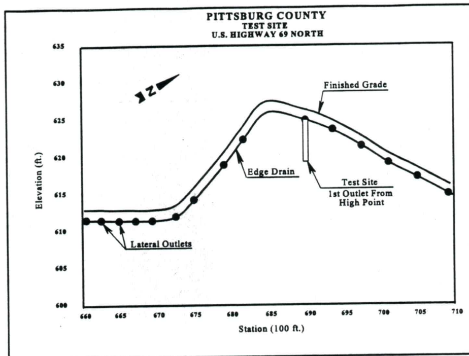
Fig. 2.5 Longitudinal slope of the roadway at the Pittsburg county site
