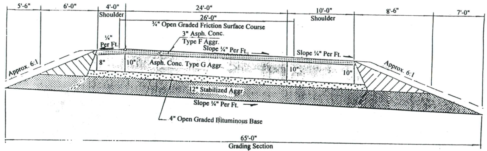
TYPICAL SURFACING AND GRADING SECTION
