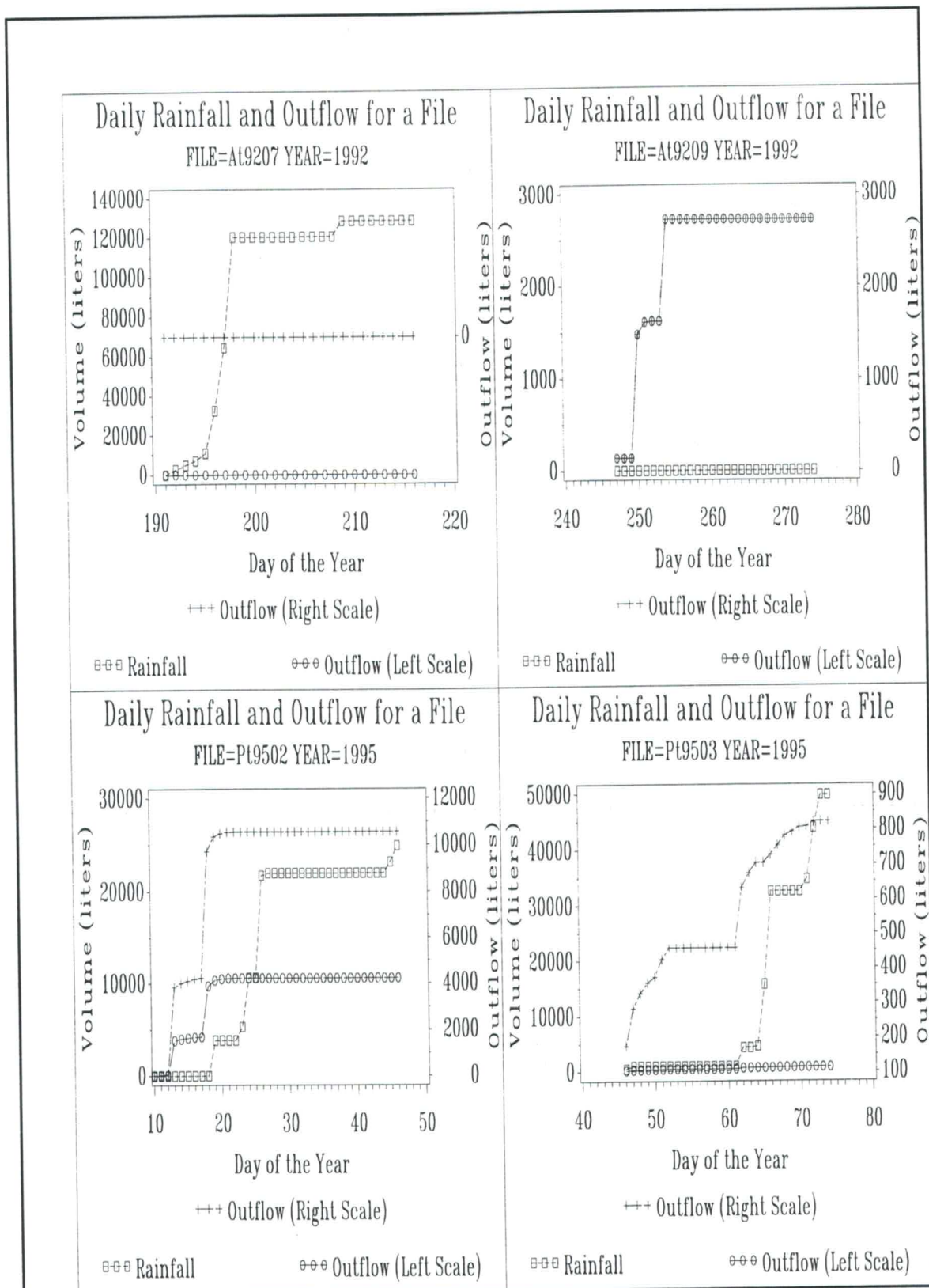
Fig. 5.35 Some files with inconsistent values of daily rainfall and outflow
