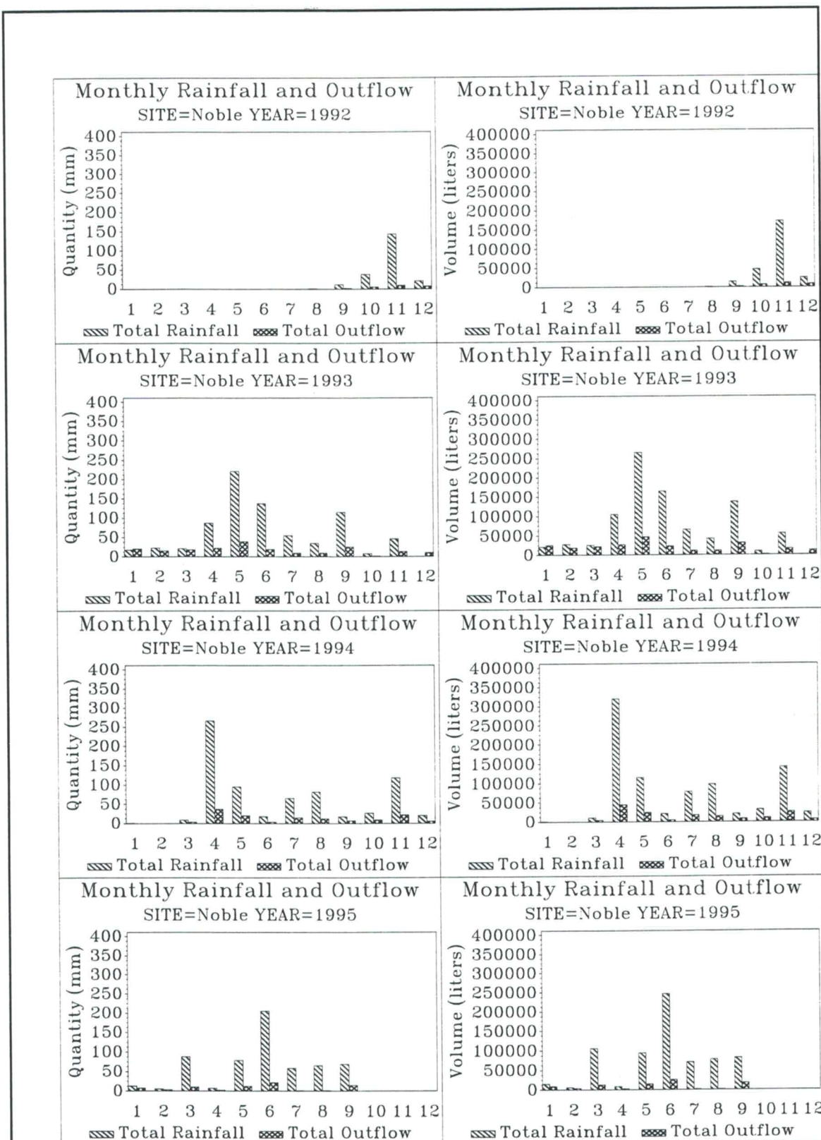
Fig. 5.20 Monthly rainfall and outflow for the Noble county site
