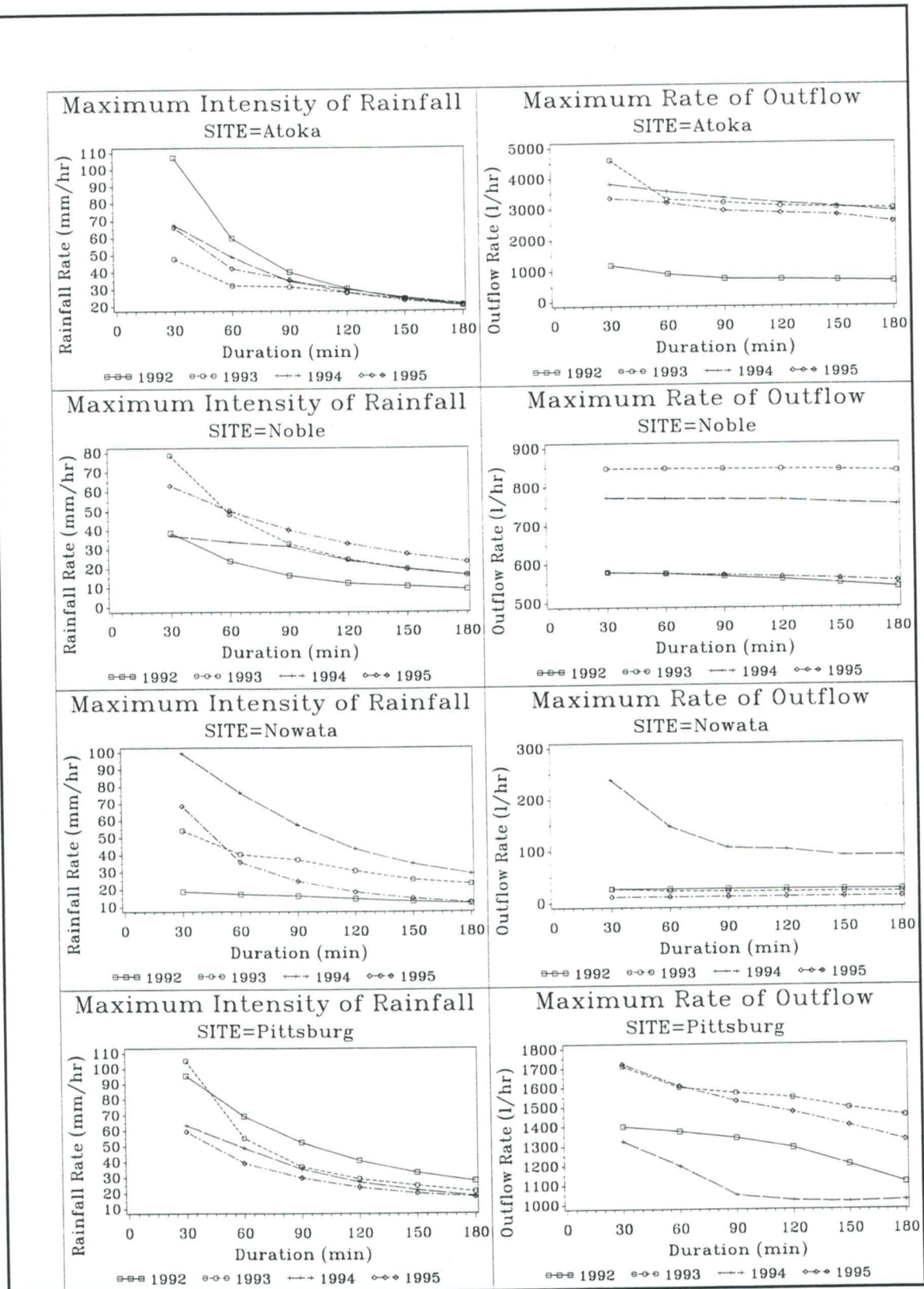
Fig. 5.28 Maximum rates of rainfall and outflow based on different time durations
