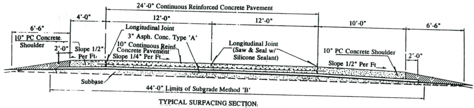
Fig. 2.12 Pavement construction drawing for the Logan county site
