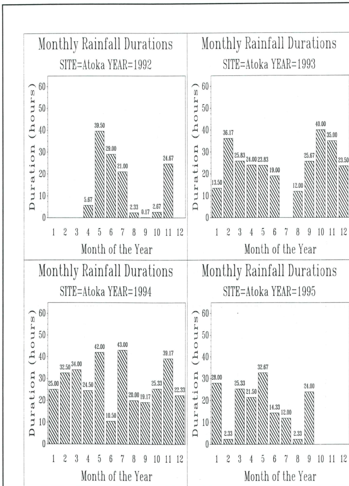
Fig. 5.15 Total duration of measured rainfall at the Atoka county site
