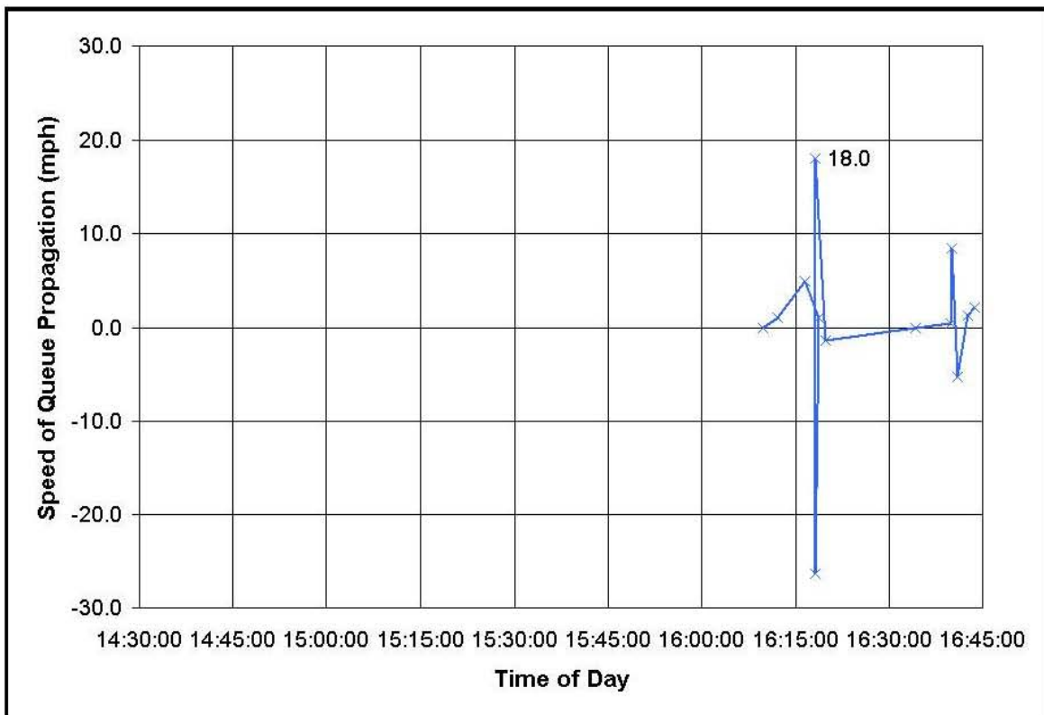
Figure A-14. US 75 Queue Propagation Data for April 24, 2002 – Lane 4 of 4.
