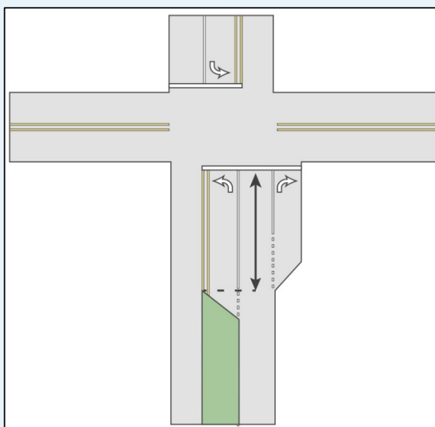
Figure 59. Graphic. Illustration of exclusive left-turn lane length.
