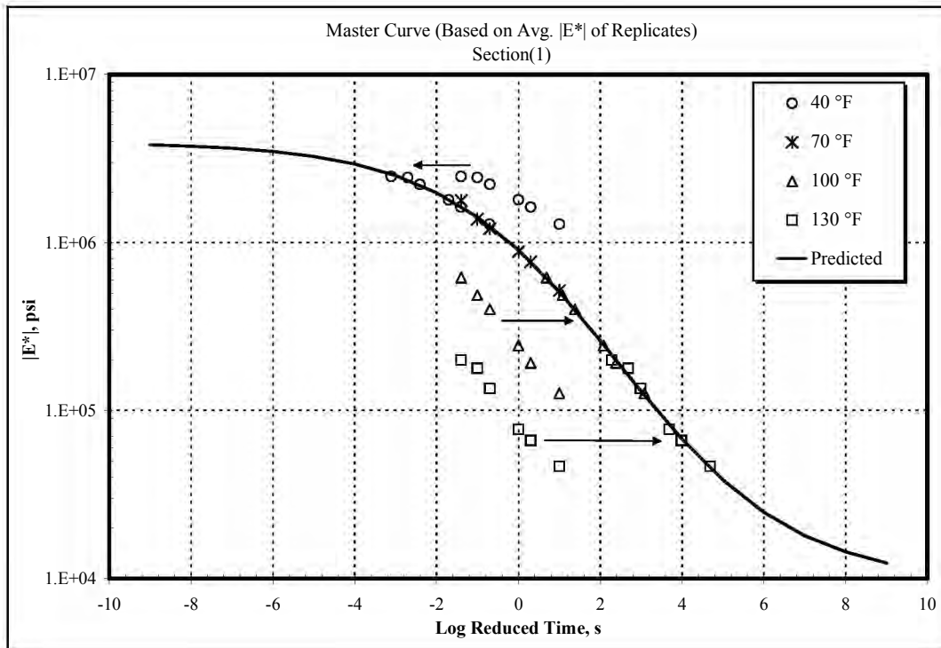
Figure B1. Dynamic Modulus Master Curve for Section 1.
