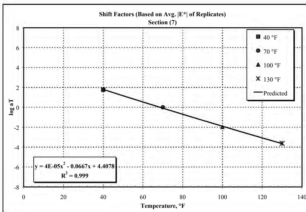
Figure B14. Dynamic Modulus Shift Factors for Section 7.
