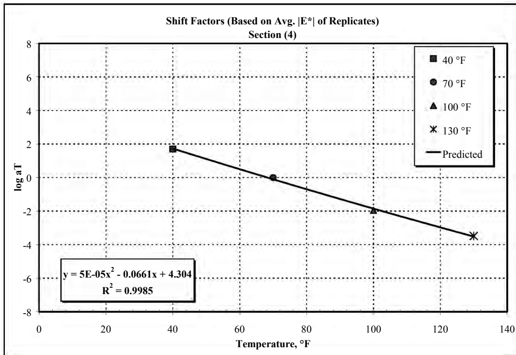
Figure B8. Dynamic Modulus Shift Factors for Section 4.
