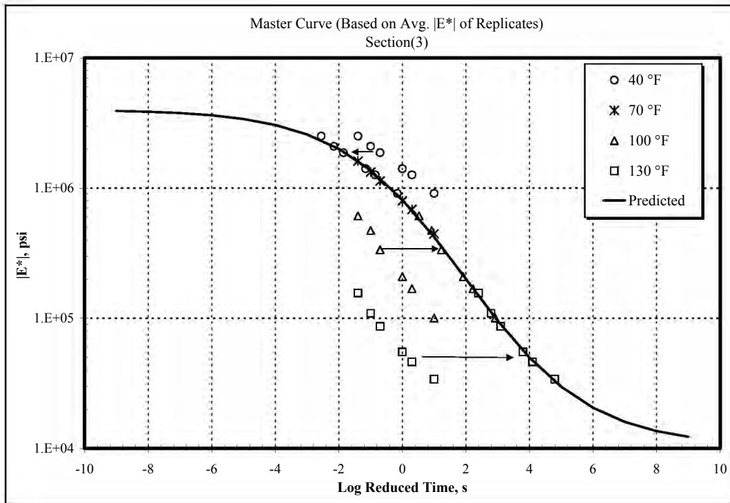
Figure B5. Dynamic Modulus Master Curve for Section 3.
