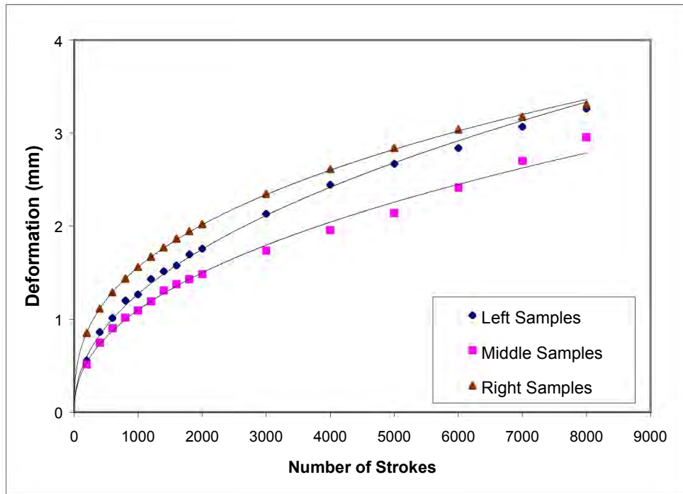
Figure B23. Section 3 APA Rut Test on Field Cores.
