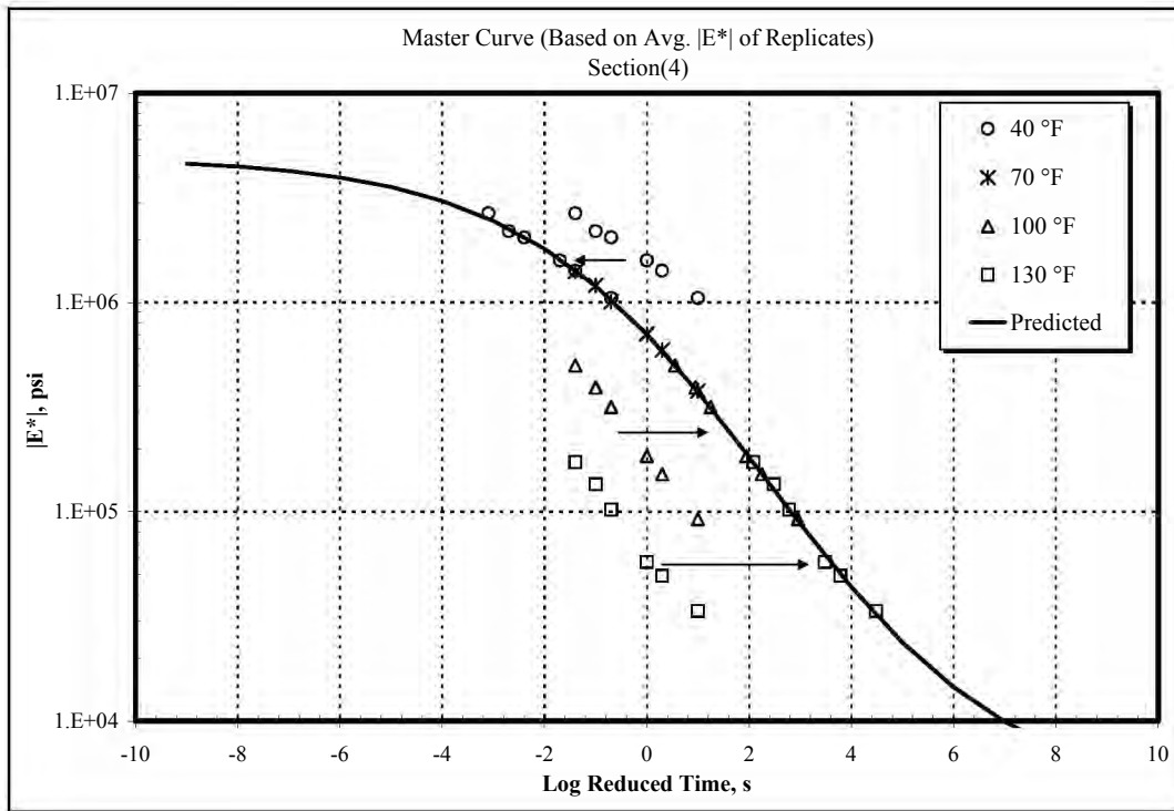
Figure B7. Dynamic Modulus Master Curve for Section 4.
