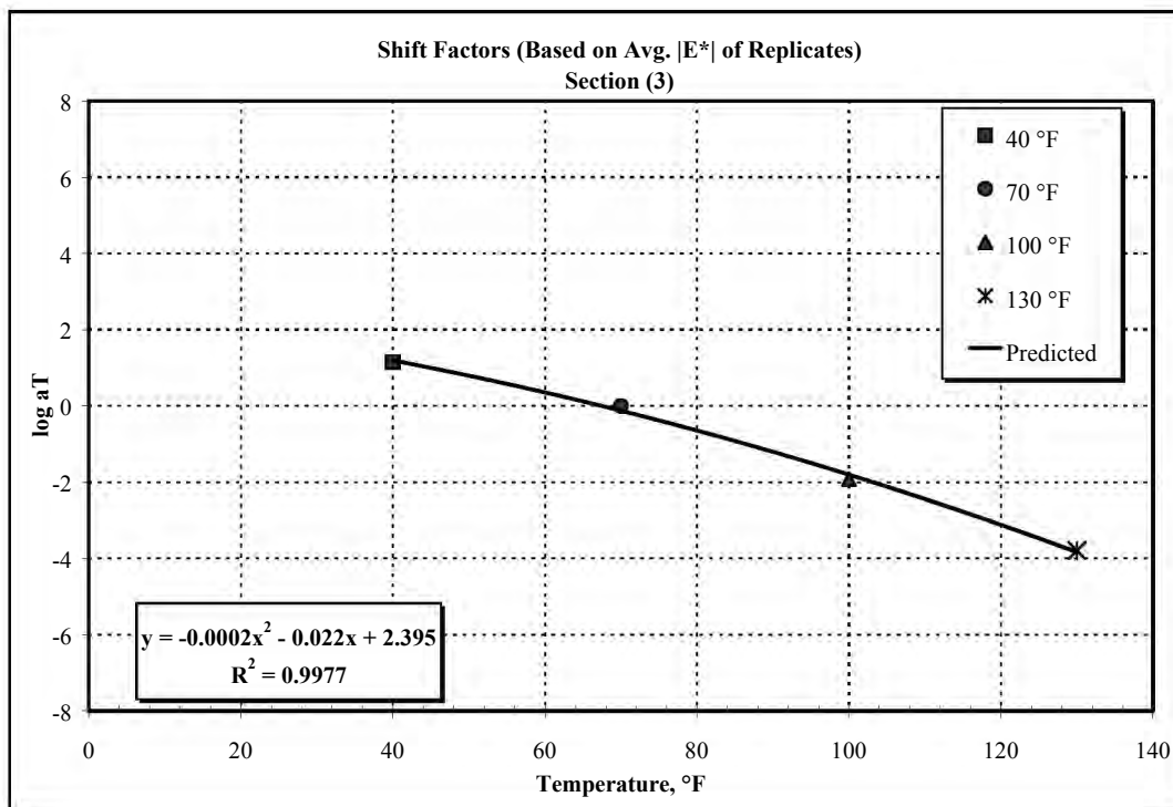
Figure B6. Dynamic Modulus Shift Factors for Section 3.
