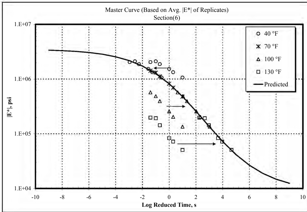
Figure B11. Dynamic Modulus Master Curve for Section 6.
