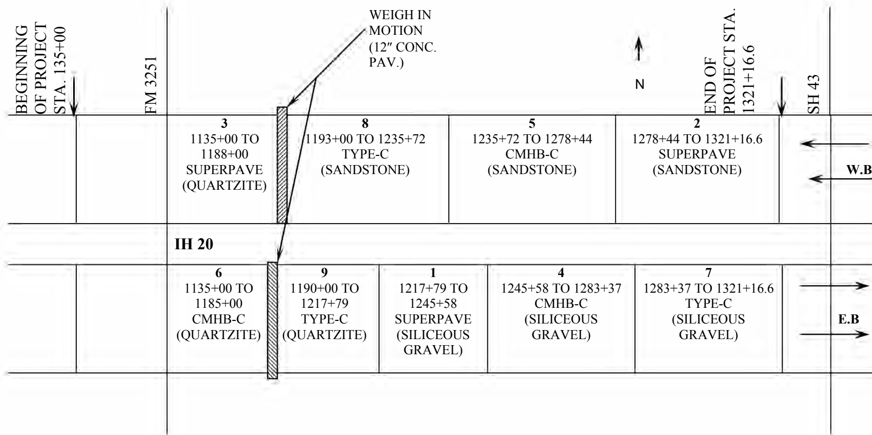
Figure 1. IH-20 Test Section Layout.
