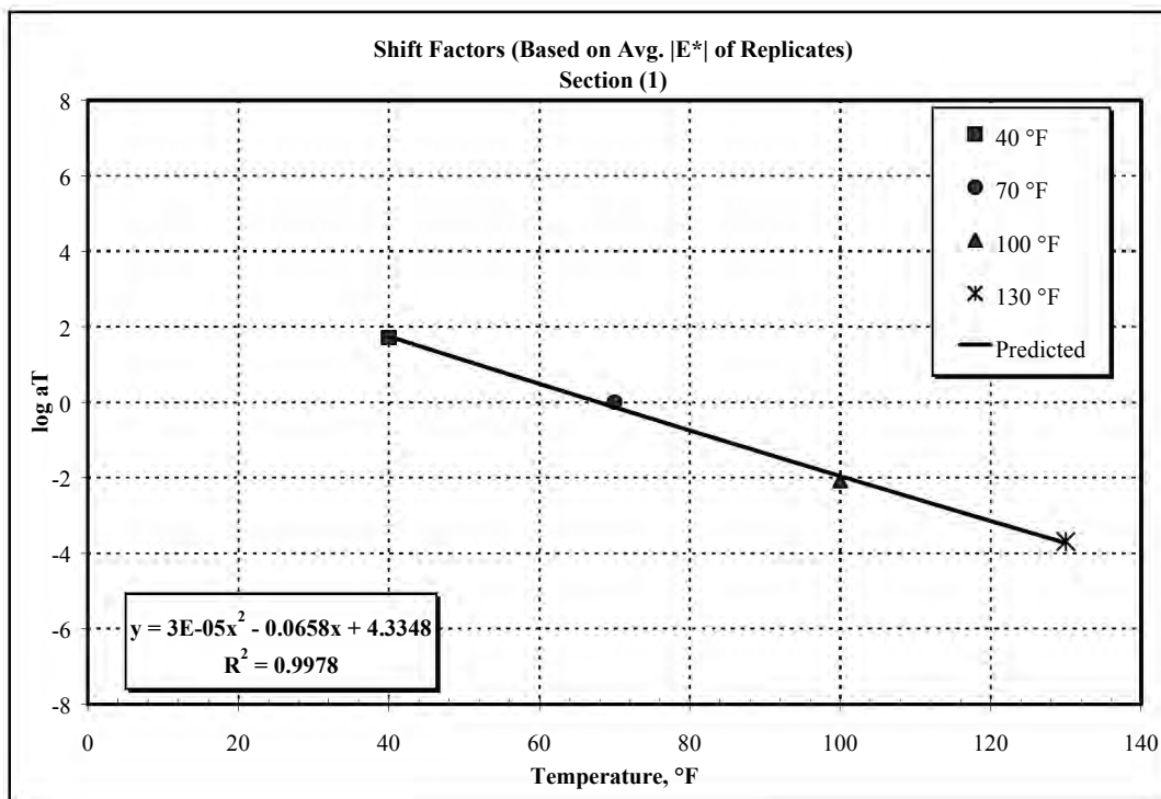
Figure B2. Dynamic Modulus Shift Factors for Section 1.
