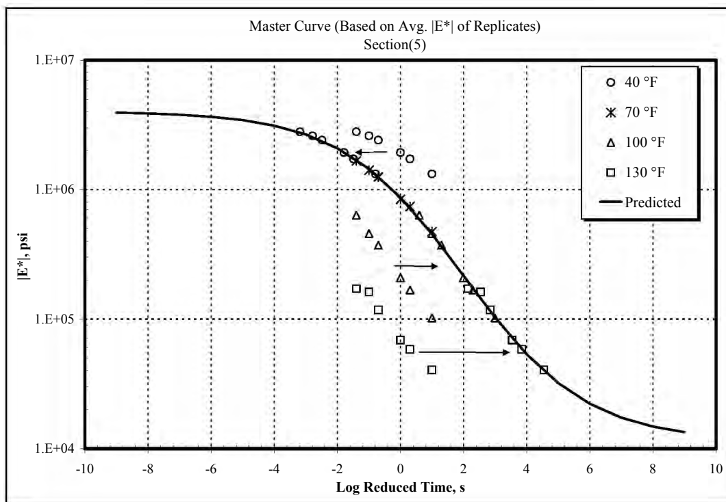
Figure B9. Dynamic Modulus Master Curve for Section 5.
