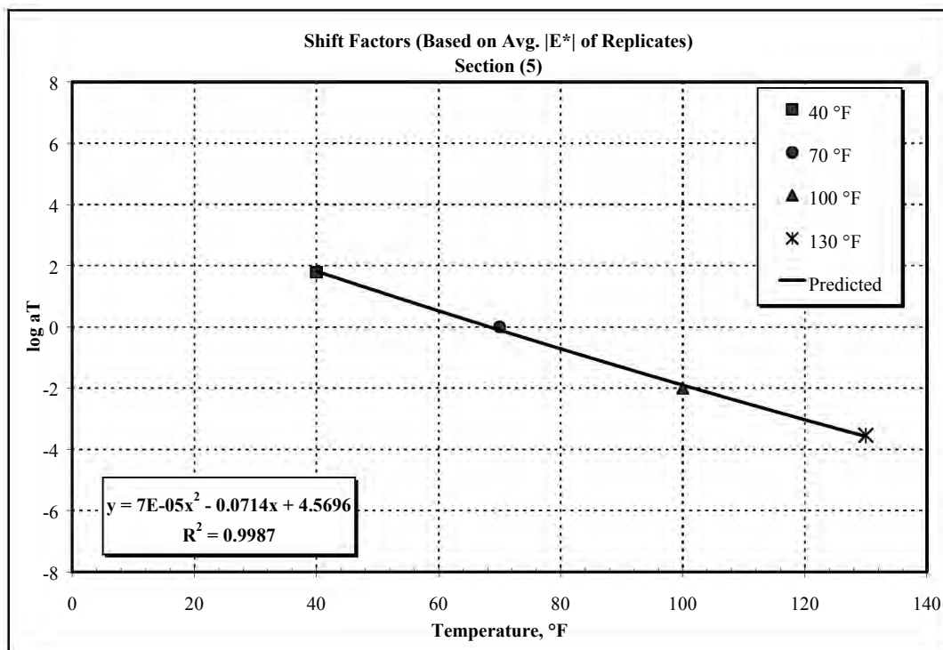
Figure B10. Dynamic Modulus Shift Factors for Section 5.
