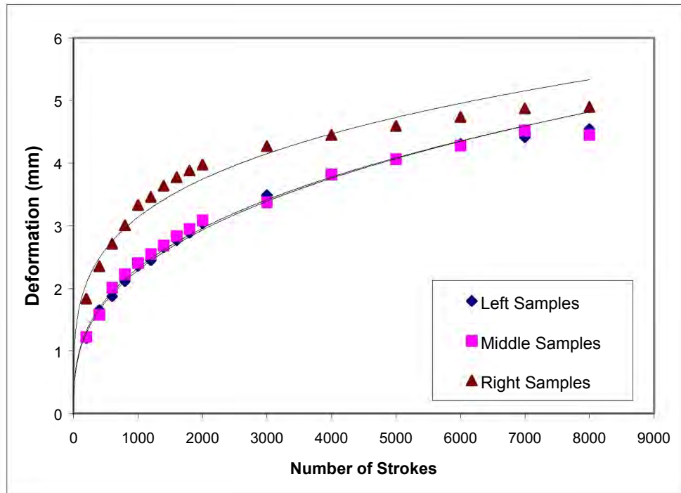
Figure B25. Section 5 APA Rut Test on Field Cores.
