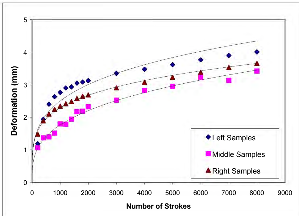
Figure B26. Section 6 APA Rut Test on Field Cores.
