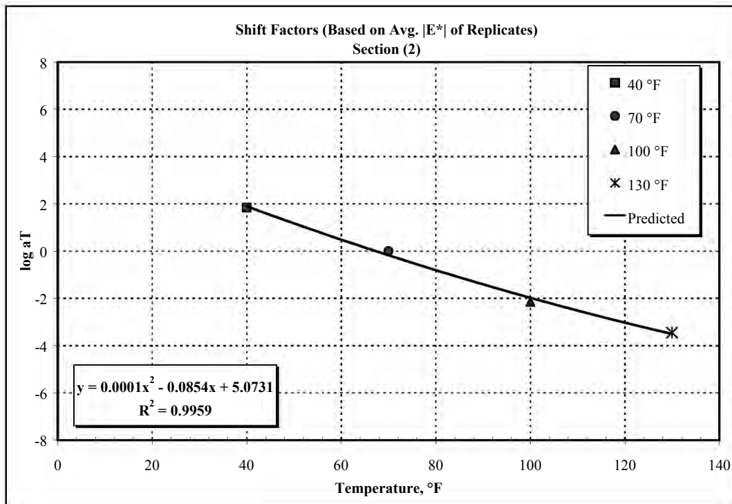
Figure B4. Dynamic Modulus Shift Factors for Section 2.
