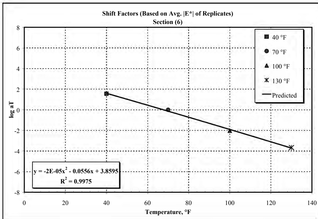
Figure B12. Dynamic Modulus Shift Factors for Section 6.
