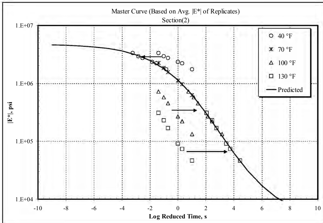
Figure B3. Dynamic Modulus Master Curve for Section 2.
