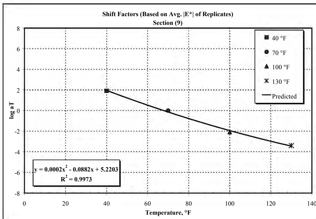
Figure B18. Dynamic Modulus Shift Factors for Section 9.
