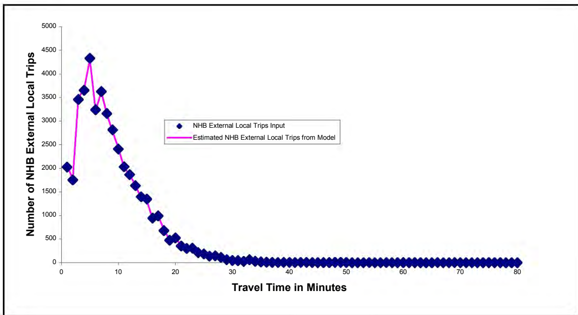
Figure 26. NHB External Local TLFD Results from Trip Distribution.
