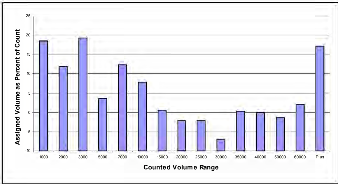
Figure 33. Assigned Volume as Percent of Count Volume for Links Grouped by Count Volume.
