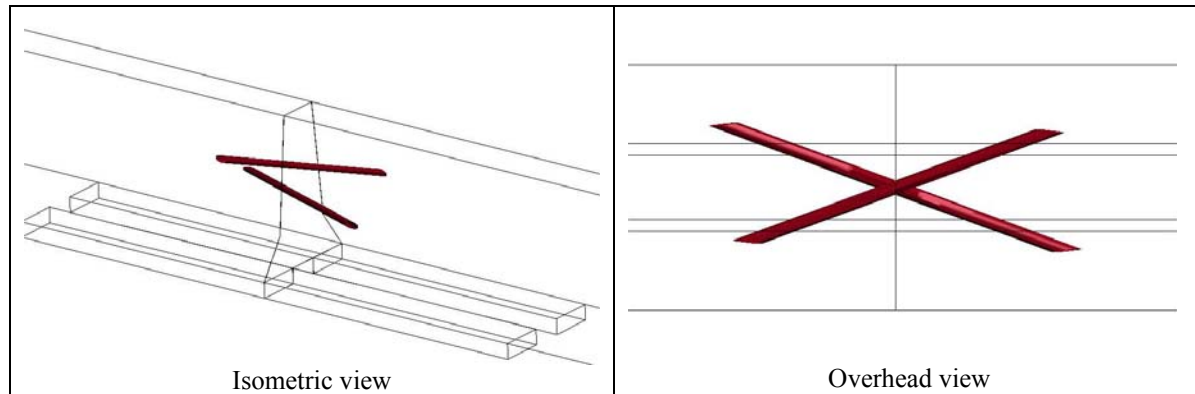
Figure 3. Cross-Bolt Connection.
