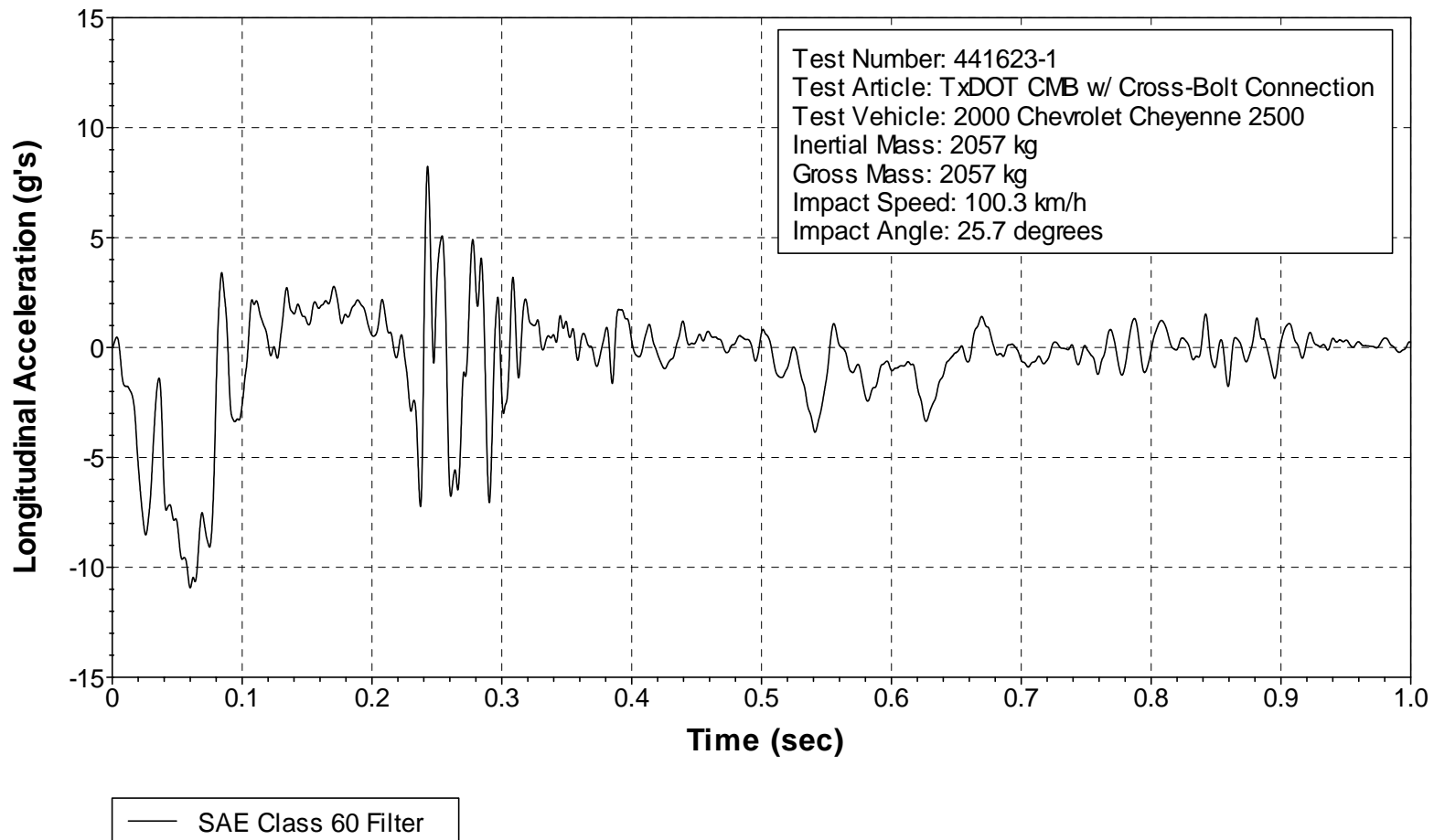
Figure 25. Vehicle Longitudinal Accelerometer Trace for Test 441623-1 (Accelerometer Located over Rear Axle).
