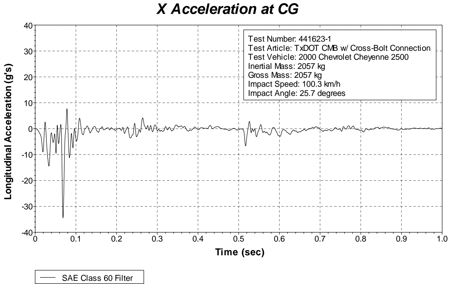
Figure 22. Vehicle Longitudinal Accelerometer Trace for Test 441623-1 (Accelerometer Located at Center of Gravity).
