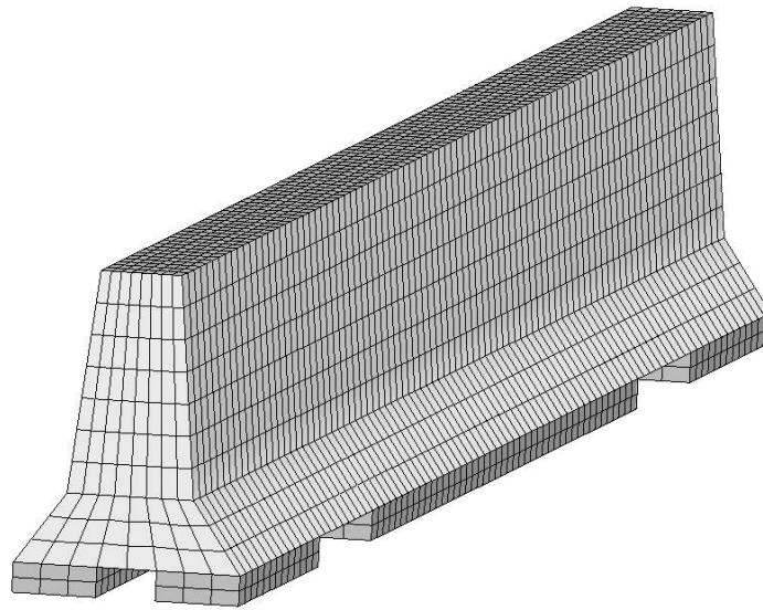
Figure 1. Finite Element Representation of F-Shape Portable Concrete Barrier.
