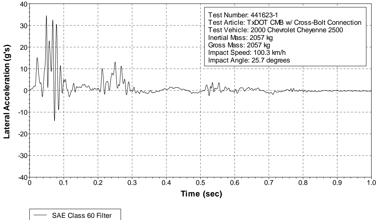
Figure 23. Vehicle Lateral Accelerometer Trace for Test 441623-1 (Accelerometer Located at Center of Gravity).
