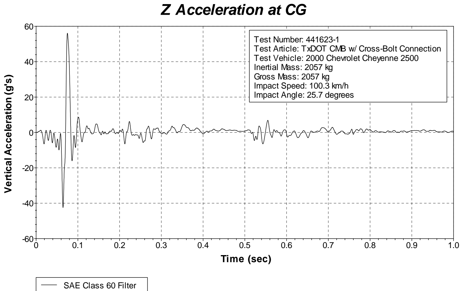
Figure 24. Vehicle Vertical Accelerometer Trace for Test 441623-1 (Accelerometer Located at Center of Gravity).
