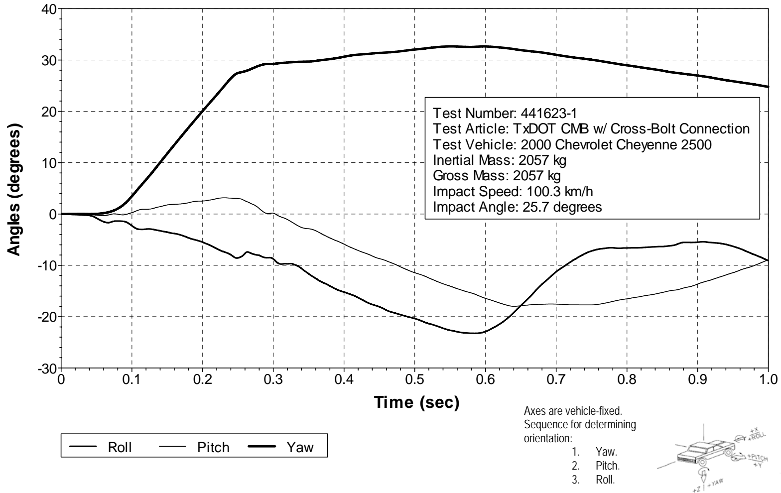
Figure 21. Vehicular Angular Displacements for Test 441623-1.
