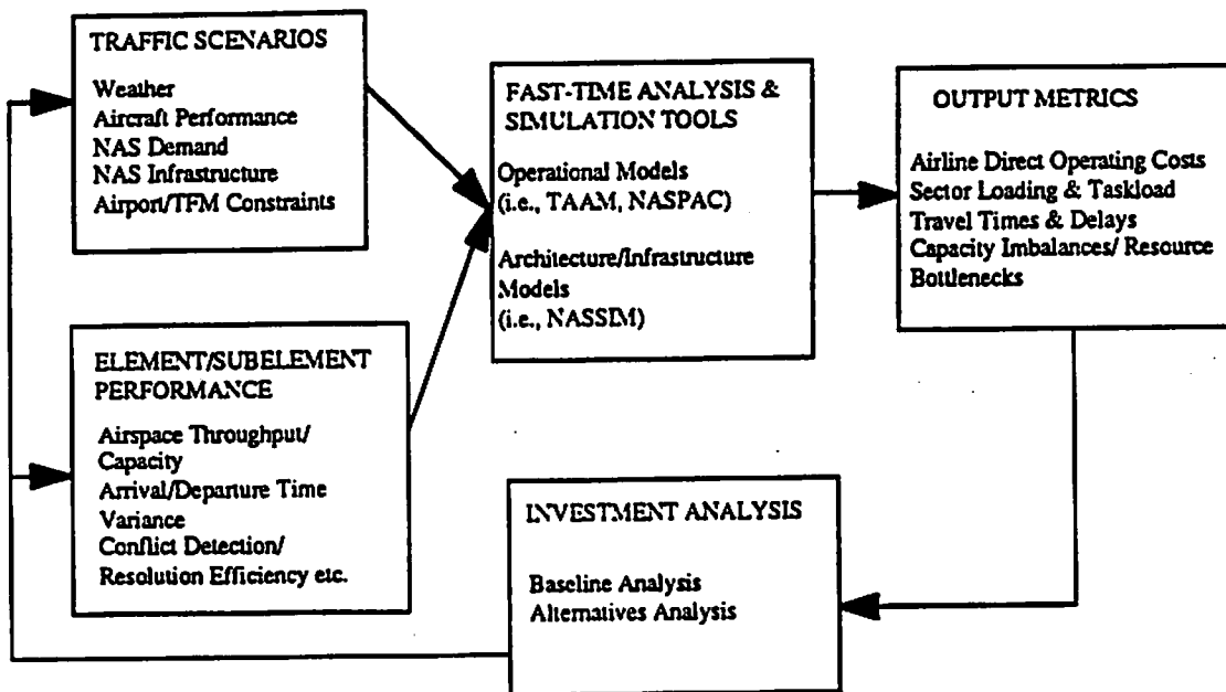
Figure 5.1 - NARIM Functional Flow Diagram
