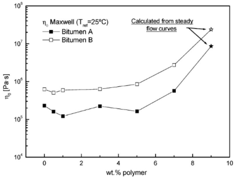
Figure 3- 8 Zero-shear-limiting viscosity as a function of the EVA content (125)
