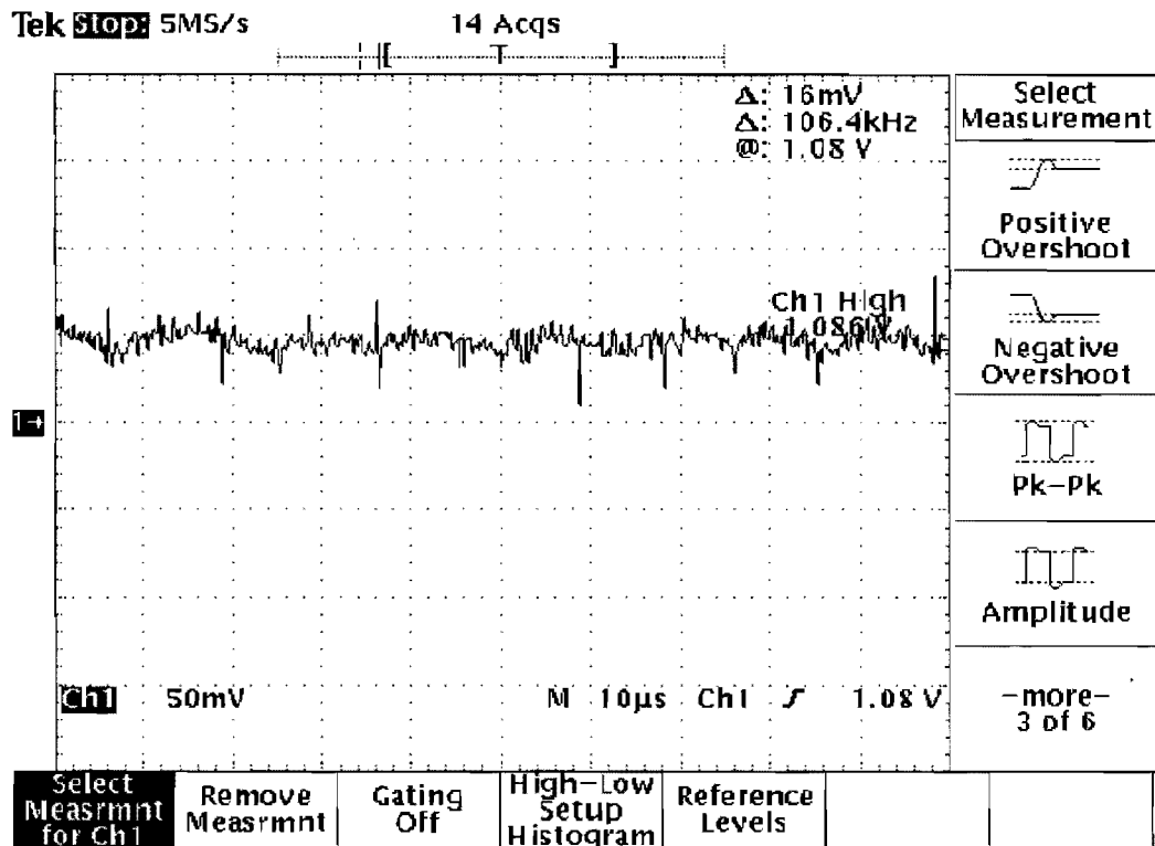
Figure 4.11 Signal after the sample/hod and switching. Note that the system conversion is 8 \mu\text{m/mv} .
