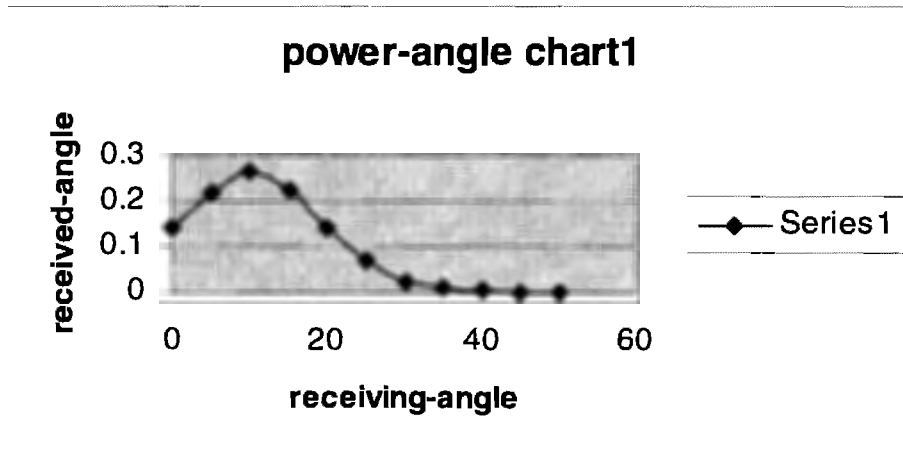
Figure 6.3 Received scattering power versus receiver angle when the incident angle is 10 degrees when the surface is smooth.
