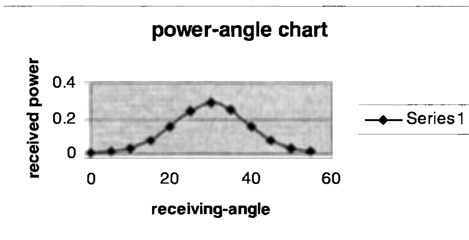
Figure 6.5 Received scattering power versus receiver angle when the incident angle is 30 degrees when the surface is smooth.
