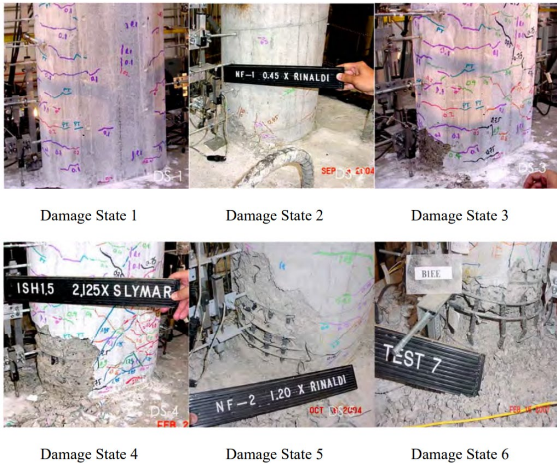
Figure 10. Damage states visualization (DS1 to DS6)
