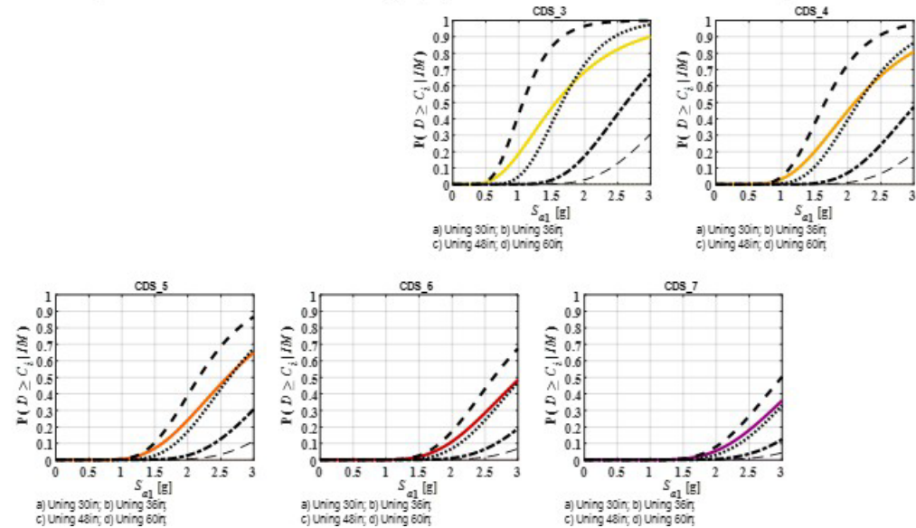
Figure F.67: Stage-B.1: Abutment average unseating damage.
