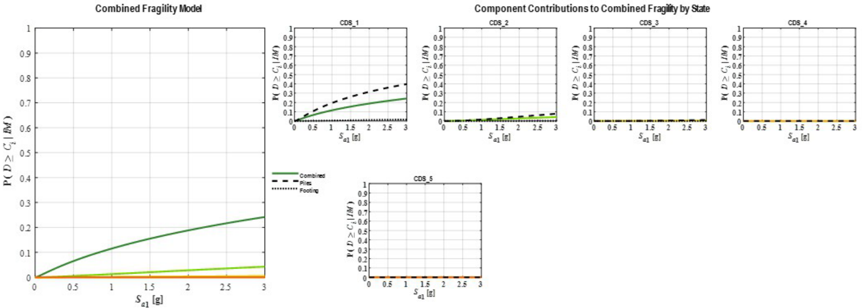
Figure F.95: Stage-B.1: Abutment foundation translational damage (Same as Stage-C roll-up for abutment wall damage).
