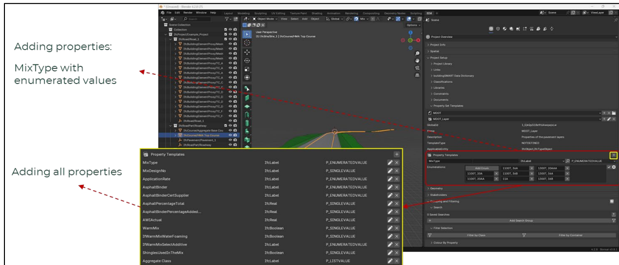
Figure 43. Adding properties
