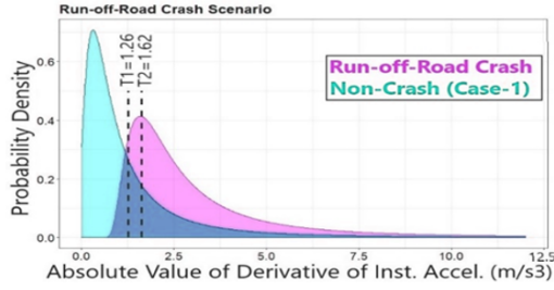
A- GEV Distributions of Absolute Value of Derivative of Instantaneous Acceleration in the Run-off-Road Scenario
