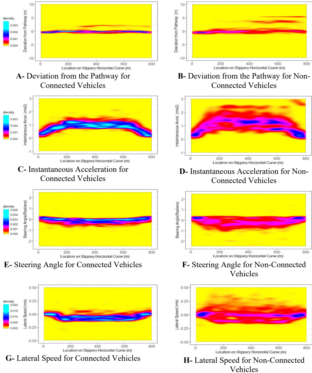
Figure 7.3 Density Distributions of CV and Non-CV Trajectories on the Slippery Horizontal Curve
