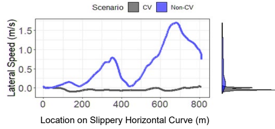
H- Lateral Speed on Regular Slippery Curve
