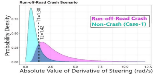
B- GEV Distributions of Absolute Value of Derivative of Steering in the Run-off-Road Scenario
