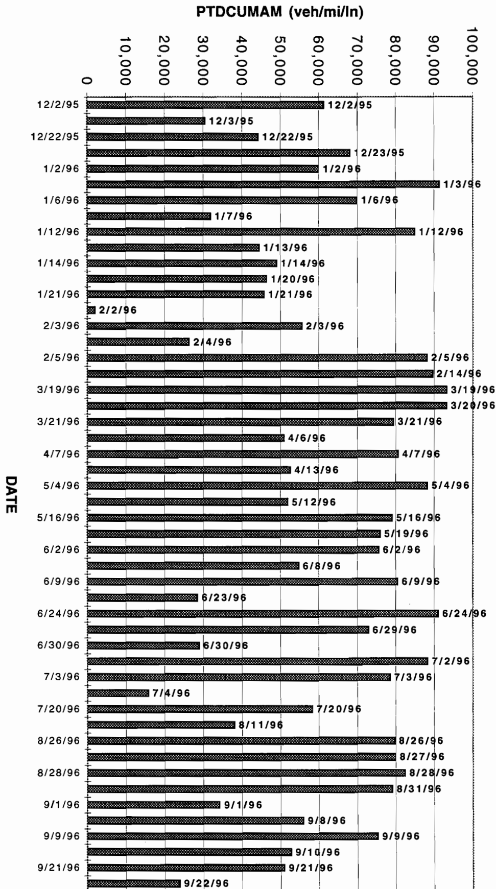
Figure 159. SAN ANTONIO DEC'95-SEP'96 MODEL T10.3.1 DATA CONTROLLED FOR DAYS DURING OZONE EPISODES GT 1-DAY AND DAYS WITH TRAFFIC CONGESTION PARAMETER LT 50th PERCENTILE DAILY CUMULATIVE TRANSGUIDE NETWORK TRAFFIC DENSITY 6AM to 2 HOURS BEFORE TIME of MAX OZONE
