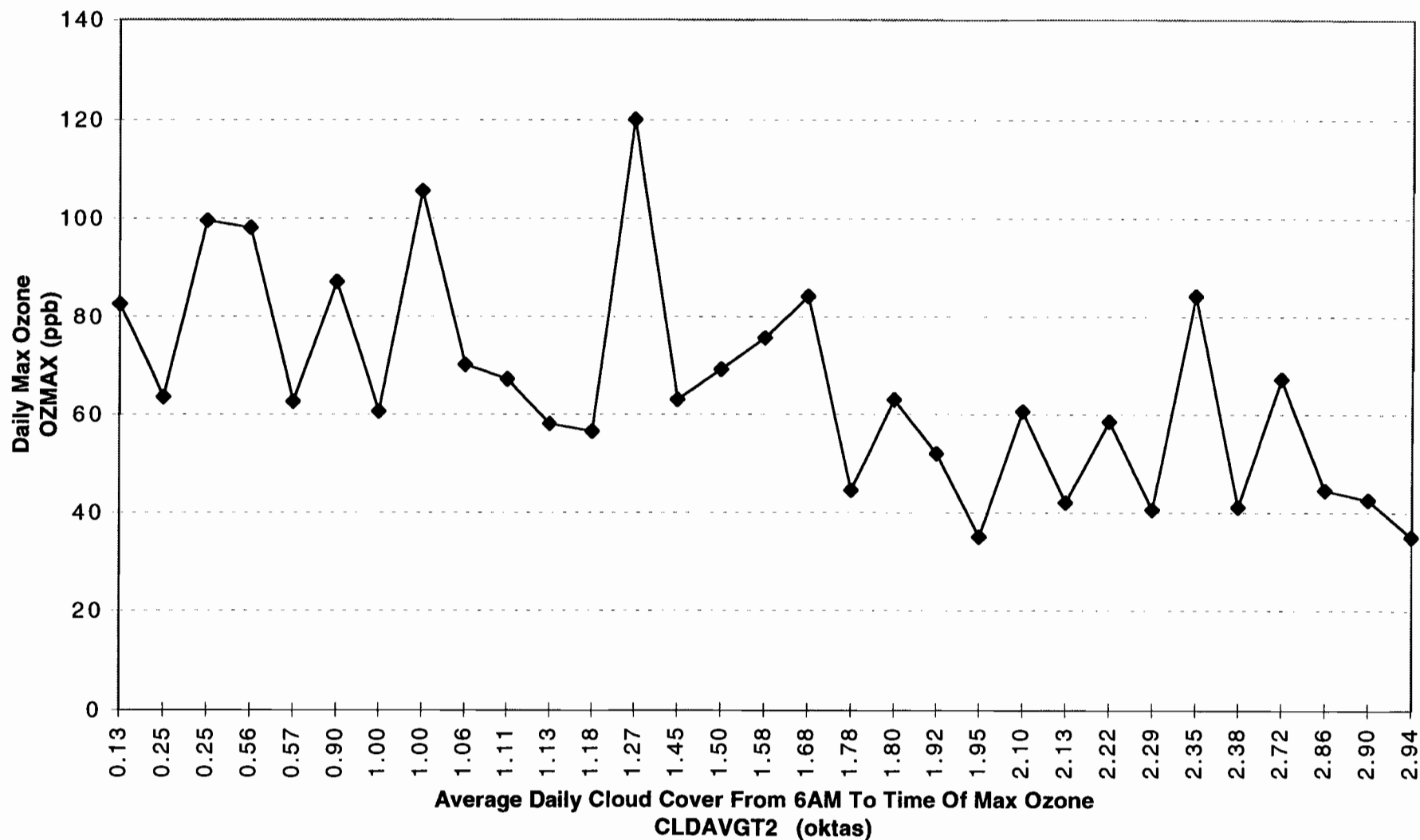
Figure 27. SAN ANTONIO APR'96-SEP'96 MODEL T2.3 Daily Max Ozone As A Function Of Average Daily Cloud Cover From 6AM To Time Of Max Ozone DATA CONTROLLED FOR DAILY AVERAGE CLOUD COVER 6AM TO TIME OF MAX OZONE LE 3 OKTAS AND DAILY AVERAGE WIND SPEED 6AM TO TIME OF MAX OZONE LE 9.2 MPH
