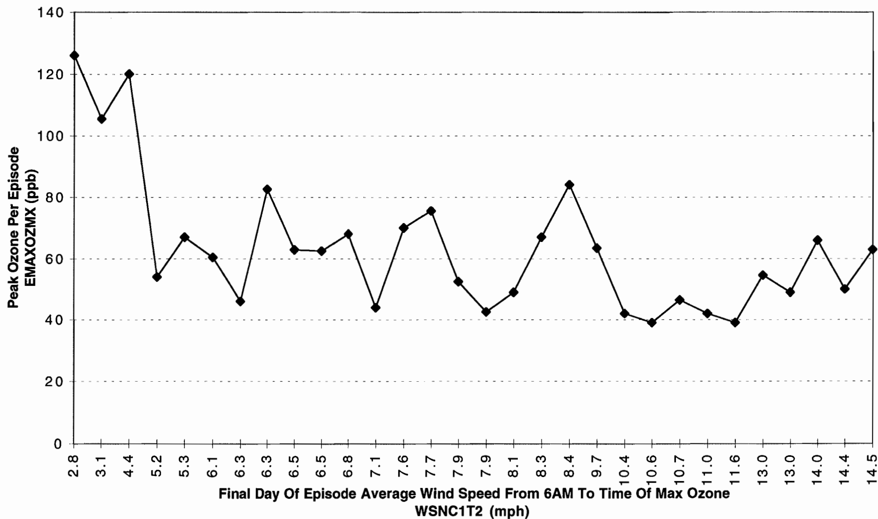
Figure 231. SAN ANTONIO APR'96-SEP'96 MODEL T44 Episodic Max Ozone As A Function Of Final Day Of Episode Average Wind Speed From 6AM To Time Of Max Ozone Data Controlled For Ozone Episodes - One Observation Of Data Per Episode And Average Episodic Cloud Cover From 6AM To Time Of Max Ozone LE 4 Oktas
