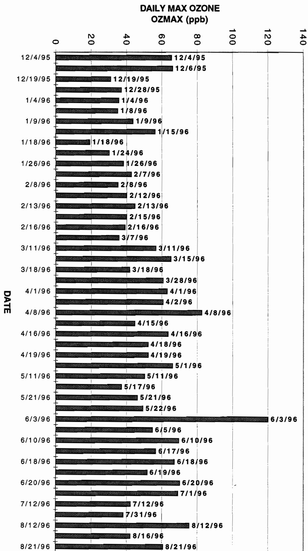
Figure 63. SAN ANTONIO DEC'95-SEP'96 MODEL T10.1 DATA CONTROLLED FOR TRAFFIC CONGESTION PARAMETER GE 50th PERCENTILE AND DAYS WITH CLDAVG12 LE 3 DAILY MAXIMUM OZONE CONCENTRATIONS
