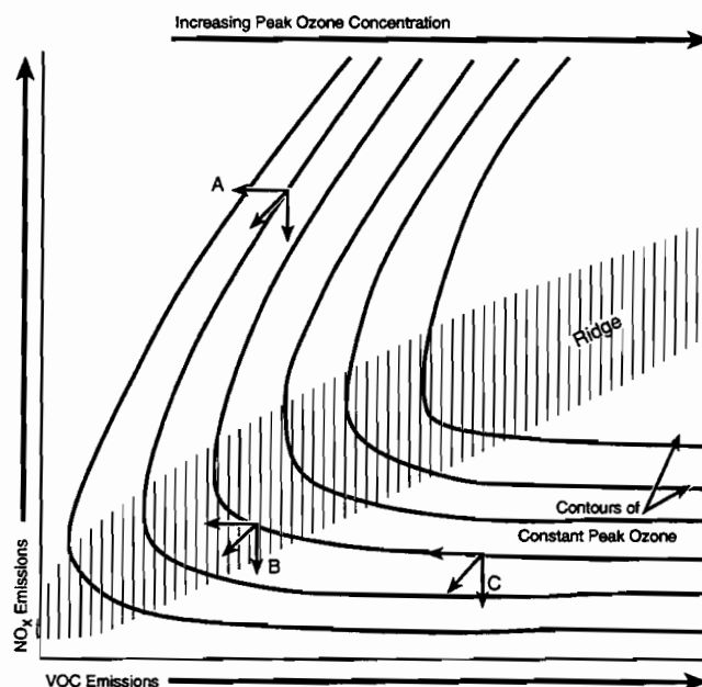
Figure 2. Hypothetical Ozone Isopleths Based on EKMA Modeling for Varying Levels of VOCs and \text{NO}_x (based on Ref 5)
