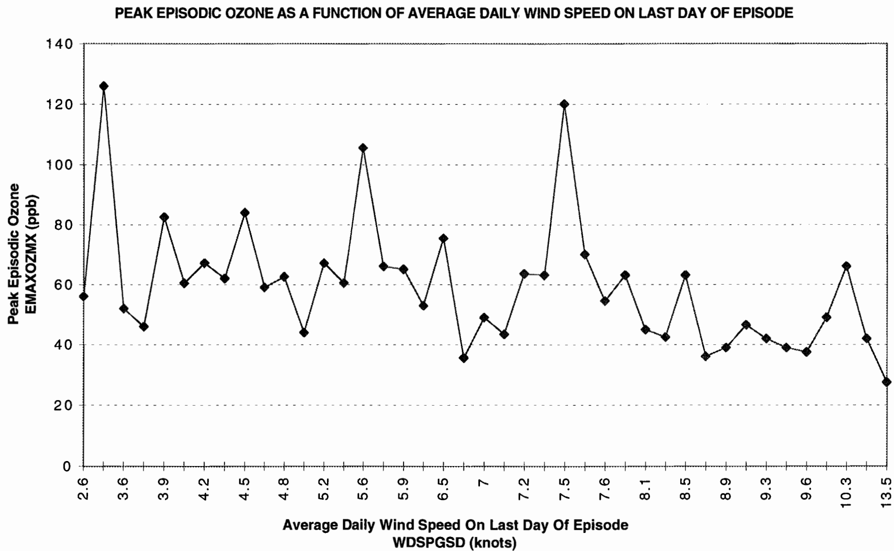
Figure 223. SAN ANTONIO DEC'95-SEP'96 MODEL T51 DATA CONTROLLED FOR OZONE EPISODES - ONE OBSERVATION PER EPISODE AND AVERAGE EPISODIC CLOUD COVER LE 4 OKTAS
