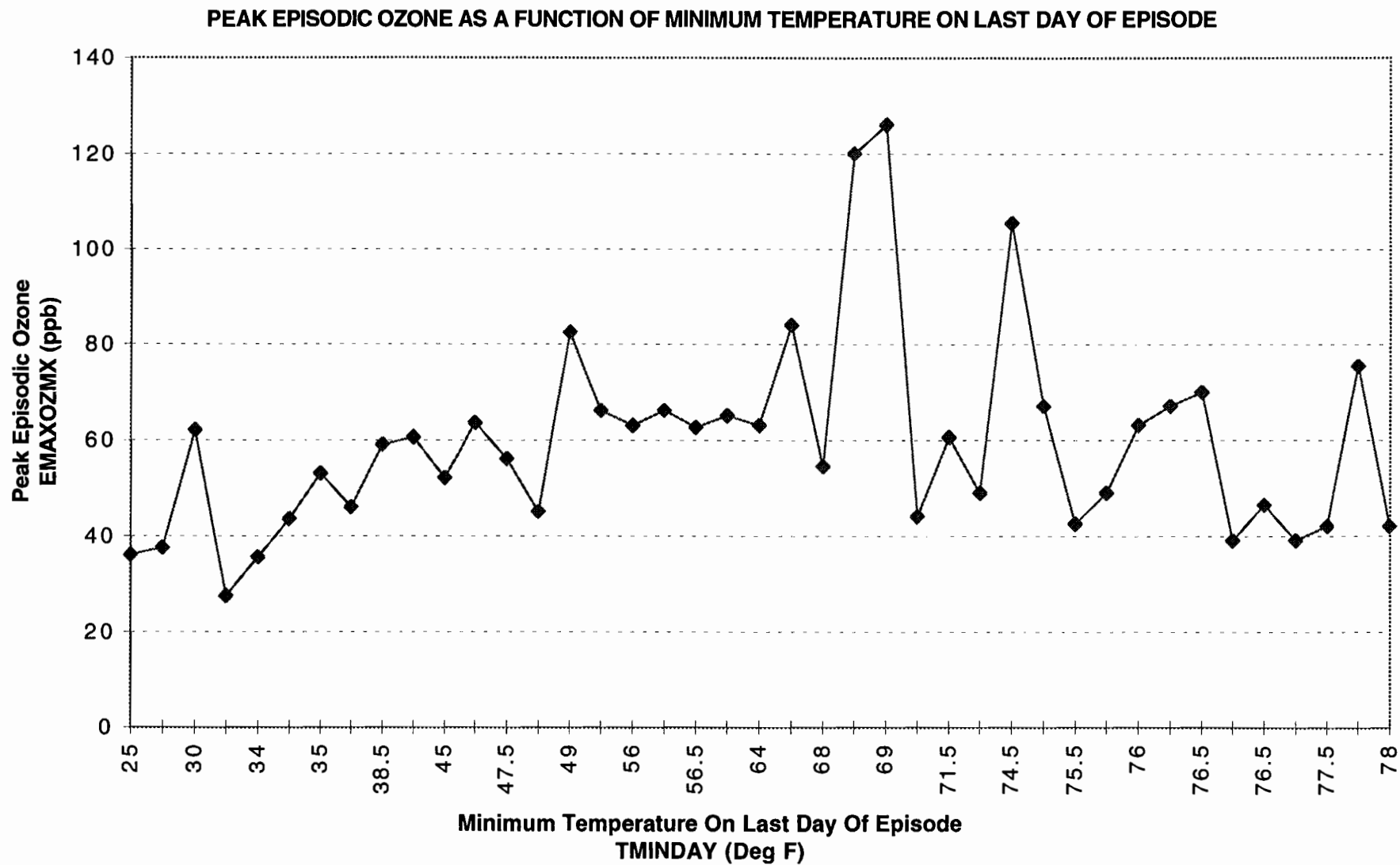
Figure 224. SAN ANTONIO DEC'95-SEP'96 MODEL T51 DATA CONTROLLED FOR OZONE EPISODES - ONE OBSERVATION PER EPISODE AND AVERAGE EPISODIC CLOUD COVER LE 4 OKTAS
