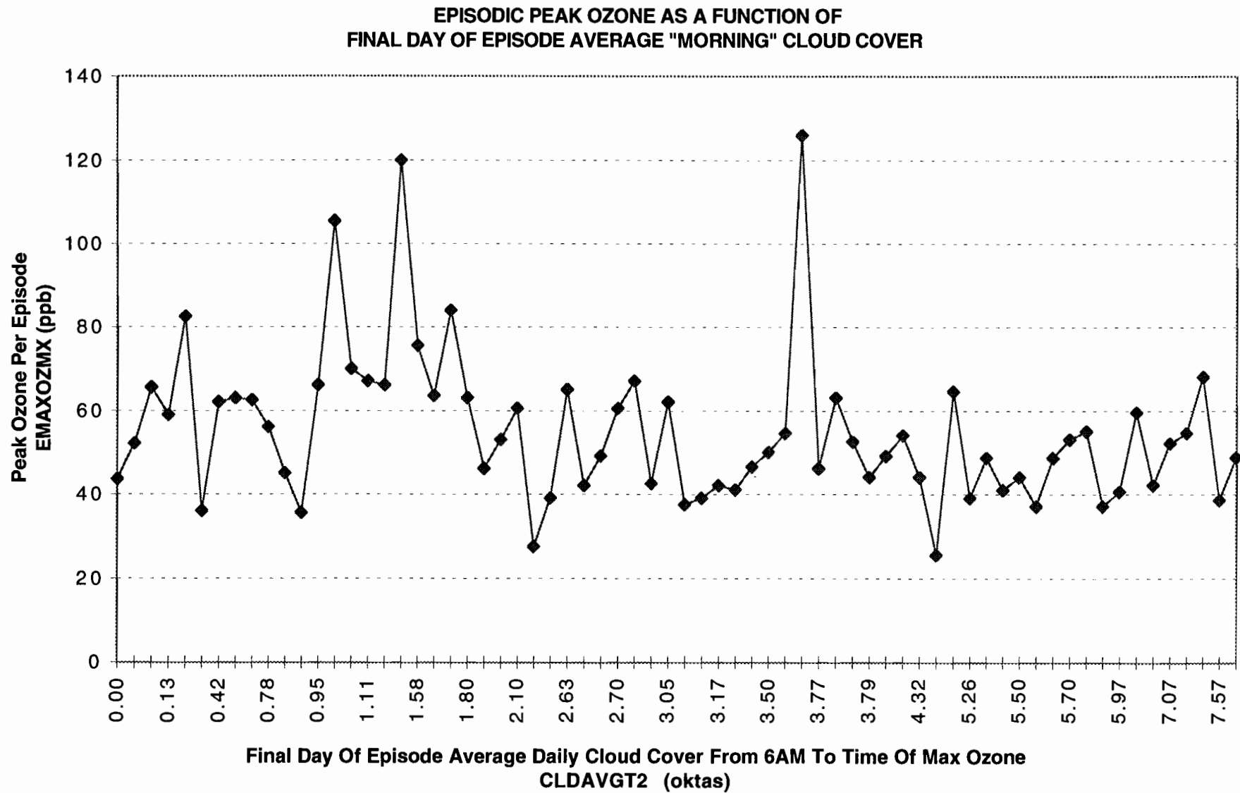
Figure 200. SAN ANTONIO DECEMBER'95 - SEPTEMBER'96 MODEL T43.0 DATA CONTROLLED FOR OZONE EPISODES - ONE OBSERVATION OF DATA PER EPISODE
