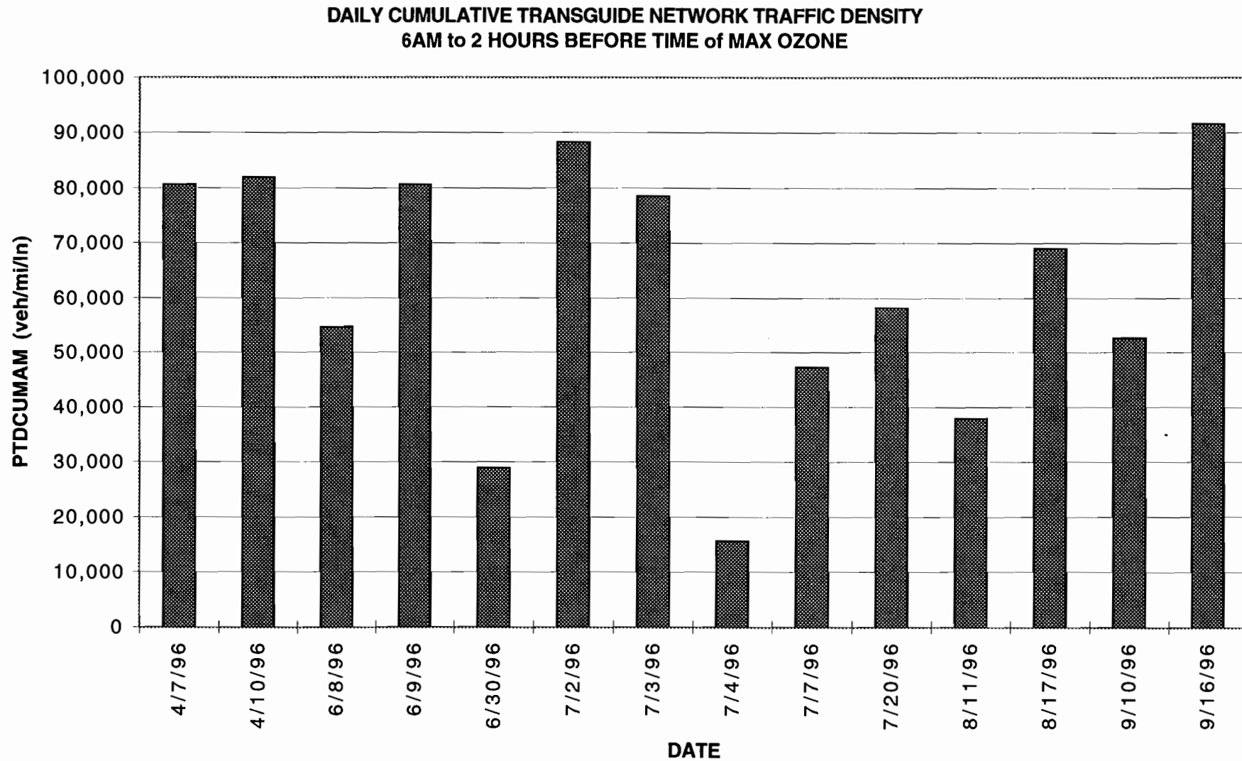
Figure 130. SAN ANTONIO APR'96-SEP'96 MODEL T13.1.0 DATA CONTROLLED FOR DAYS WITH TRAFFIC CONGESTION PARAMETER LT 50th PERCENTILE AND DAYS DURING OZONE EPISODES AND AVERAGE "MORNING" CLOUD COVER LE 3 OKTAS
