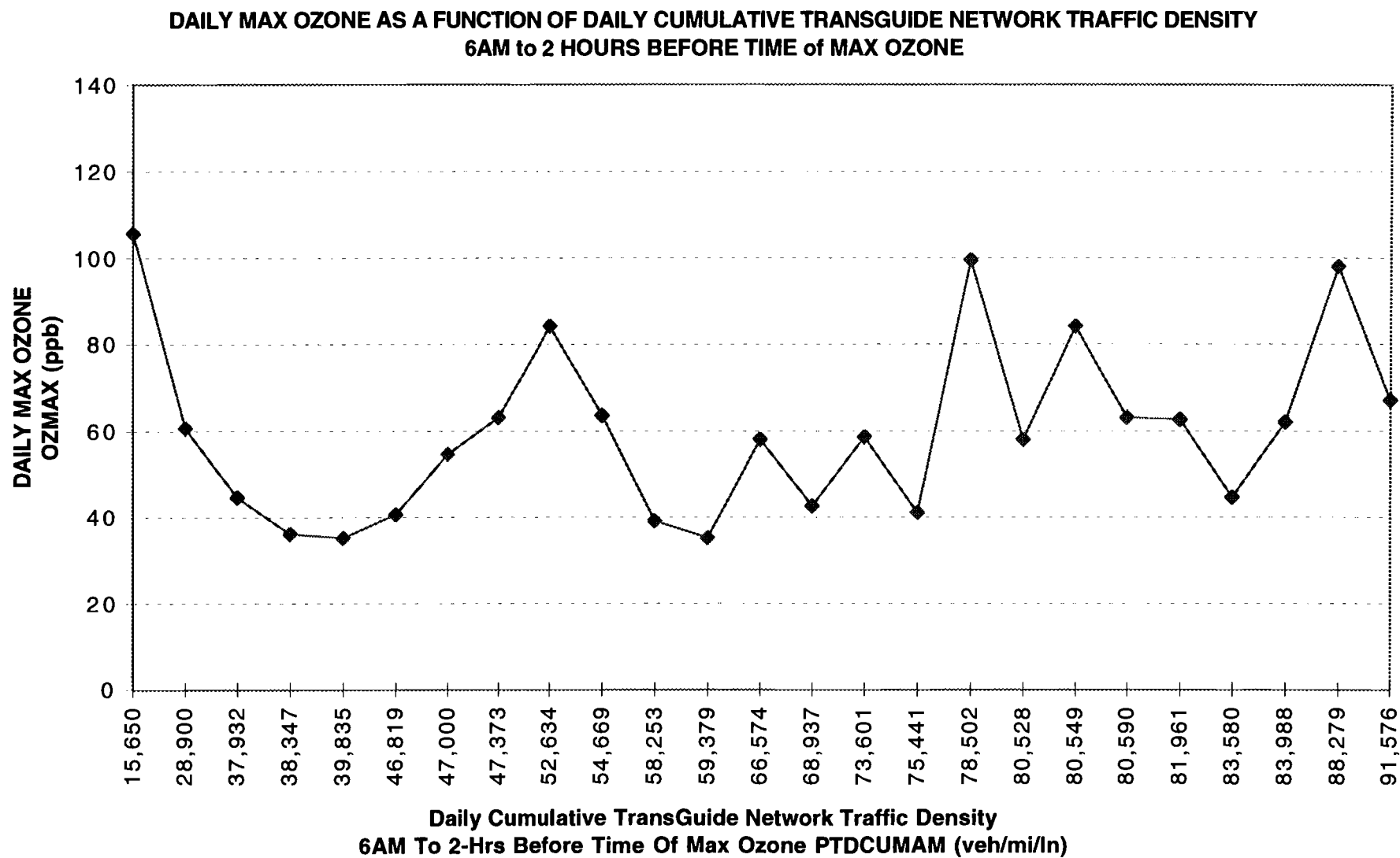
Figure 74. SAN ANTONIO APR'96-SEP'96 MODEL T11.2 DATA CONTROLLED FOR TRAFFIC CONGESTION PARAMETER LT 50th PERCENTILE AND DAYS WITH CLDAVGT2 LE 3
