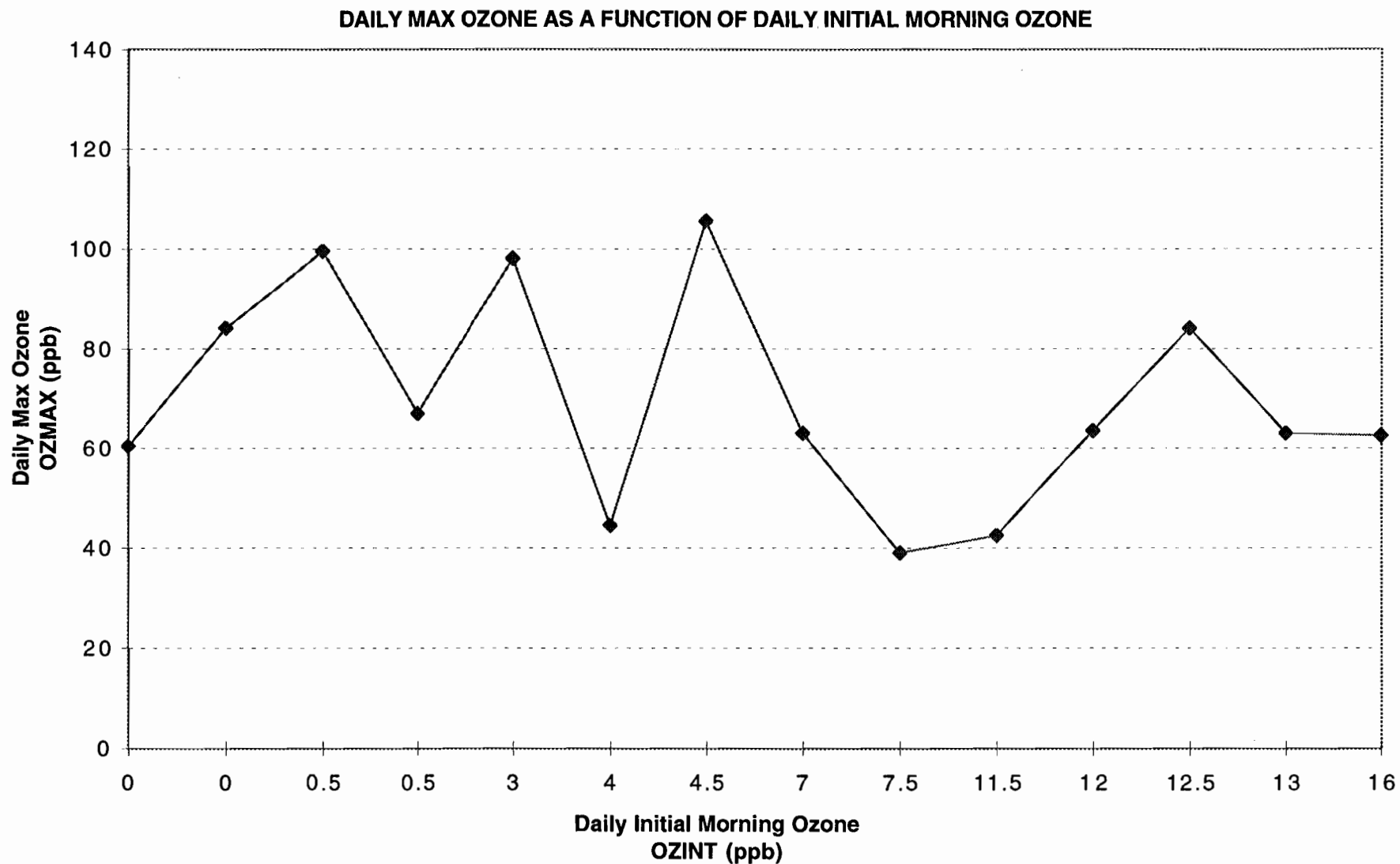
Figure 132. SAN ANTONIO APR'96-SEP'96 MODEL T13.1.0 DATA CONTROLLED FOR DAYS WITH TRAFFIC CONGESTION PARAMETER LT 50th PERCENTILE AND DAYS DURING OZONE EPISODES AND AVERAGE "MORNING" CLOUD COVER LE 3 OKTAS
