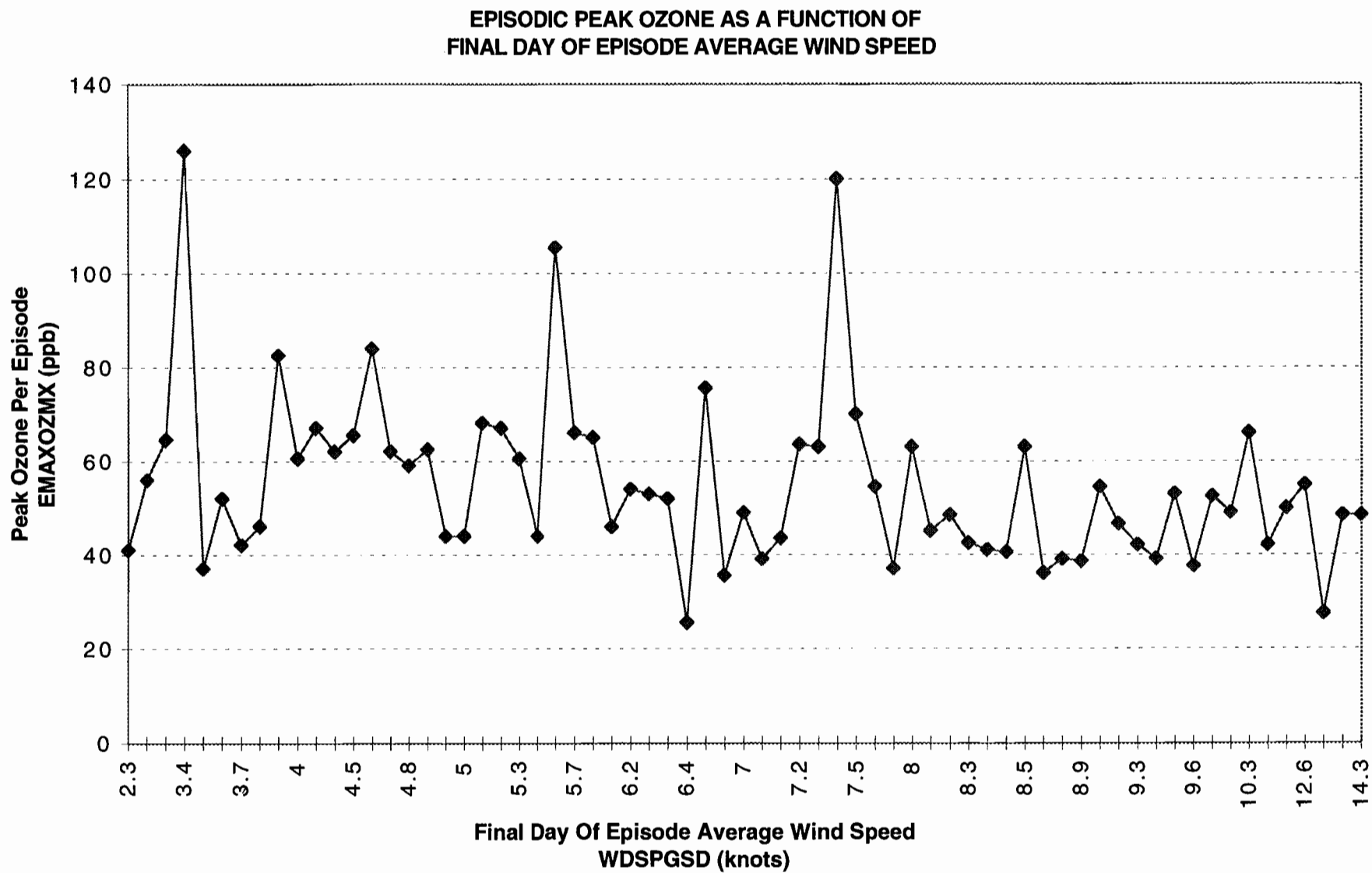
Figure 203. SAN ANTONIO DECEMBER'95 - SEPTEMBER'96 MODEL T43.0 DATA CONTROLLED FOR OZONE EPISODES - ONE OBSERVATION OF DATA PER EPISODE
