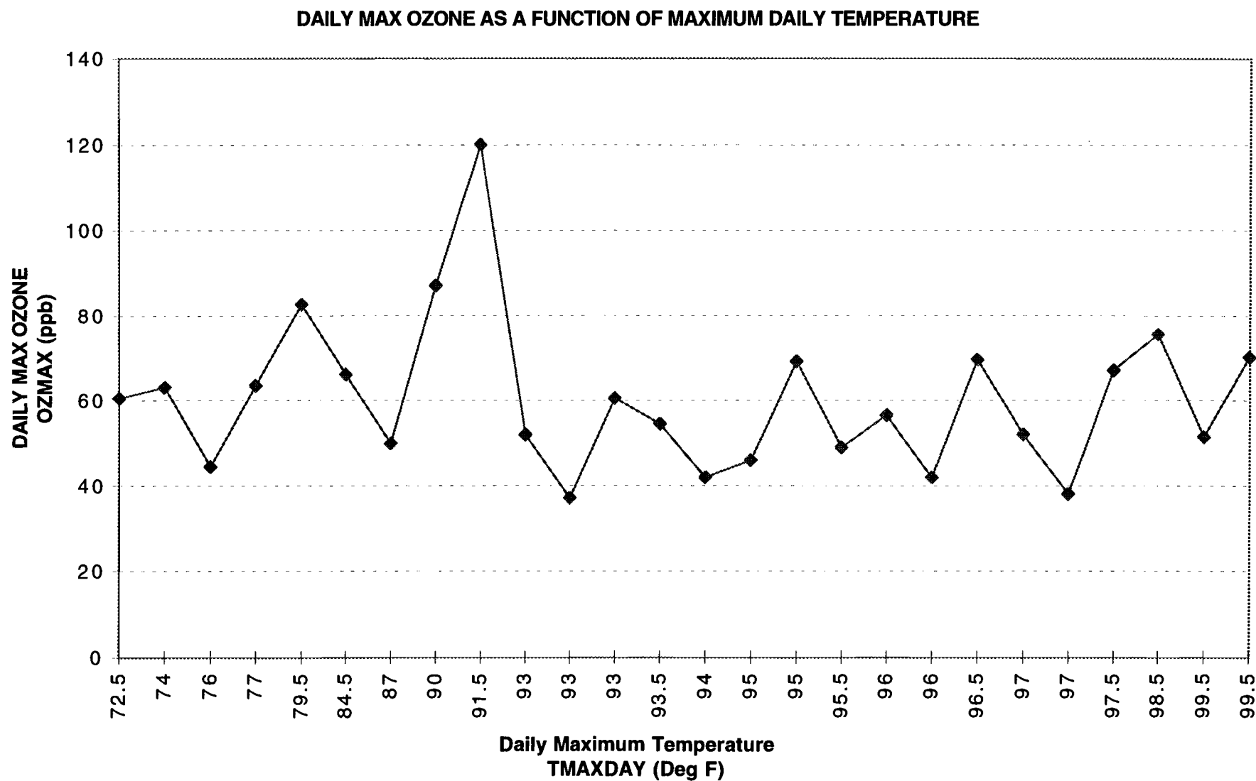
Figure 59. SAN ANTONIO APR'96-SEP'96 MODEL T11.1 DATA CONTROLLED FOR TRAFFIC CONGESTION PARAMETER GE 50th PERCENTILE AND DAYS WITH CLDAVGT2 LE 3
