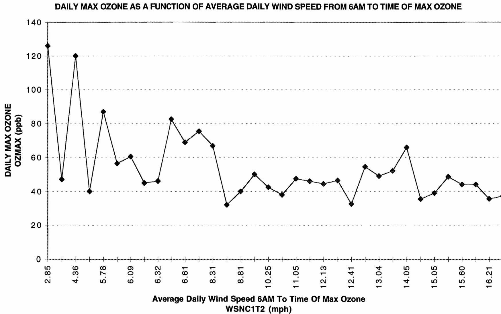
Figure 191. SAN ANTONIO APR'96-SEP'96 MODEL T19.1 DATA CONTROLLED FOR DAYS DURING OZONE EPISODES GT 1-DAY AND DAYS WITH TRAFFIC CONGESTION PARAMETER GE 50th PERCENTILE
