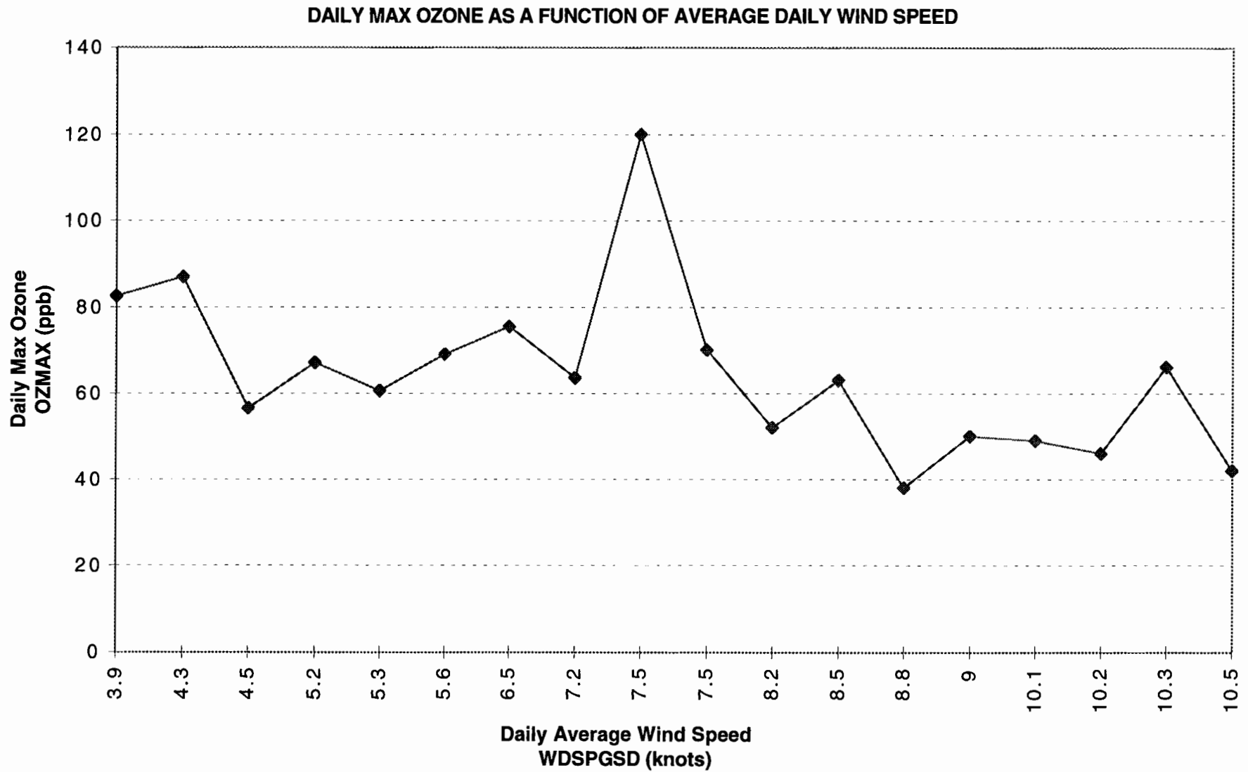
Figure 155. SAN ANTONIO APR'96-SEP'96 MODEL T13.1 DATA CONTROLLED FOR DAYS WITH TRAFFIC CONGESTION PARAMETER GE 50th PERCENTILE AND DAYS DURING OZONE EPISODES AND AVERAGE "MORNING" CLOUD COVER LE 3 OKTAS
