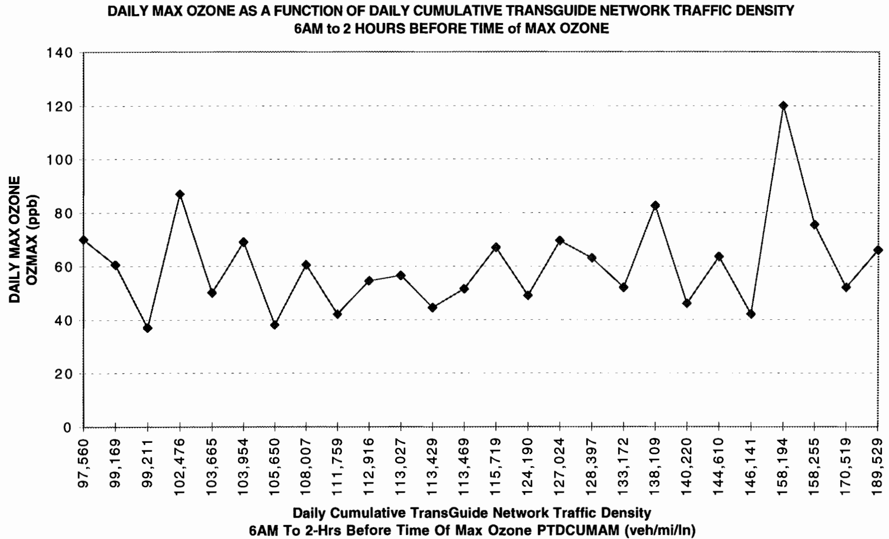
Figure 55. SAN ANTONIO APR'96-SEP'96 MODEL T11.1 DATA CONTROLLED FOR TRAFFIC CONGESTION PARAMETER GE 50th PERCENTILE AND DAYS WITH CLDAVGT2 LE 3
