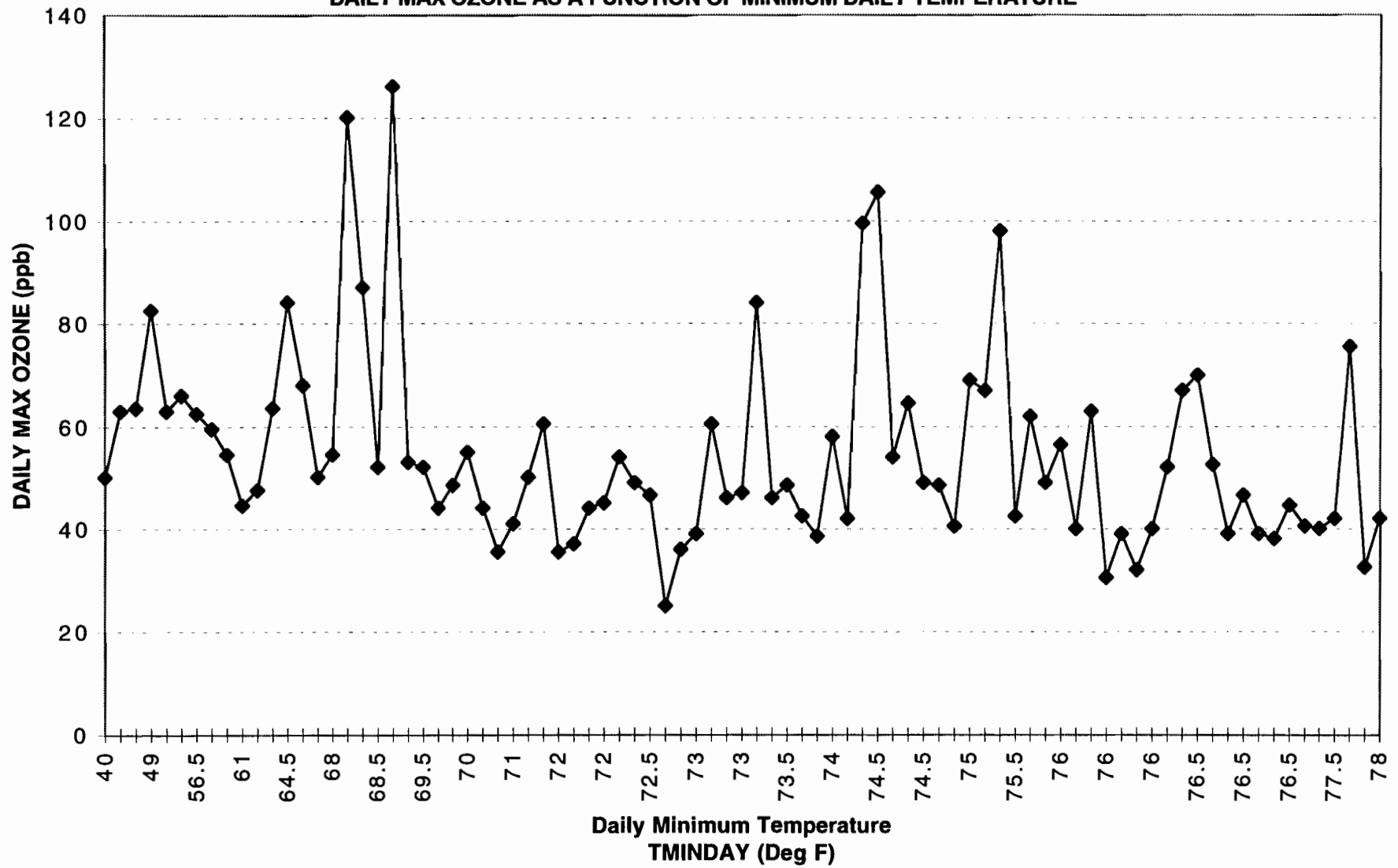
Figure 98. SAN ANTONIO APR'96-SEP'96 MODEL T22 DATA CONTROLLED FOR DAYS DURING OZONE EPISODES DAILY MAX OZONE AS A FUNCTION OF MINIMUM DAILY TEMPERATURE
