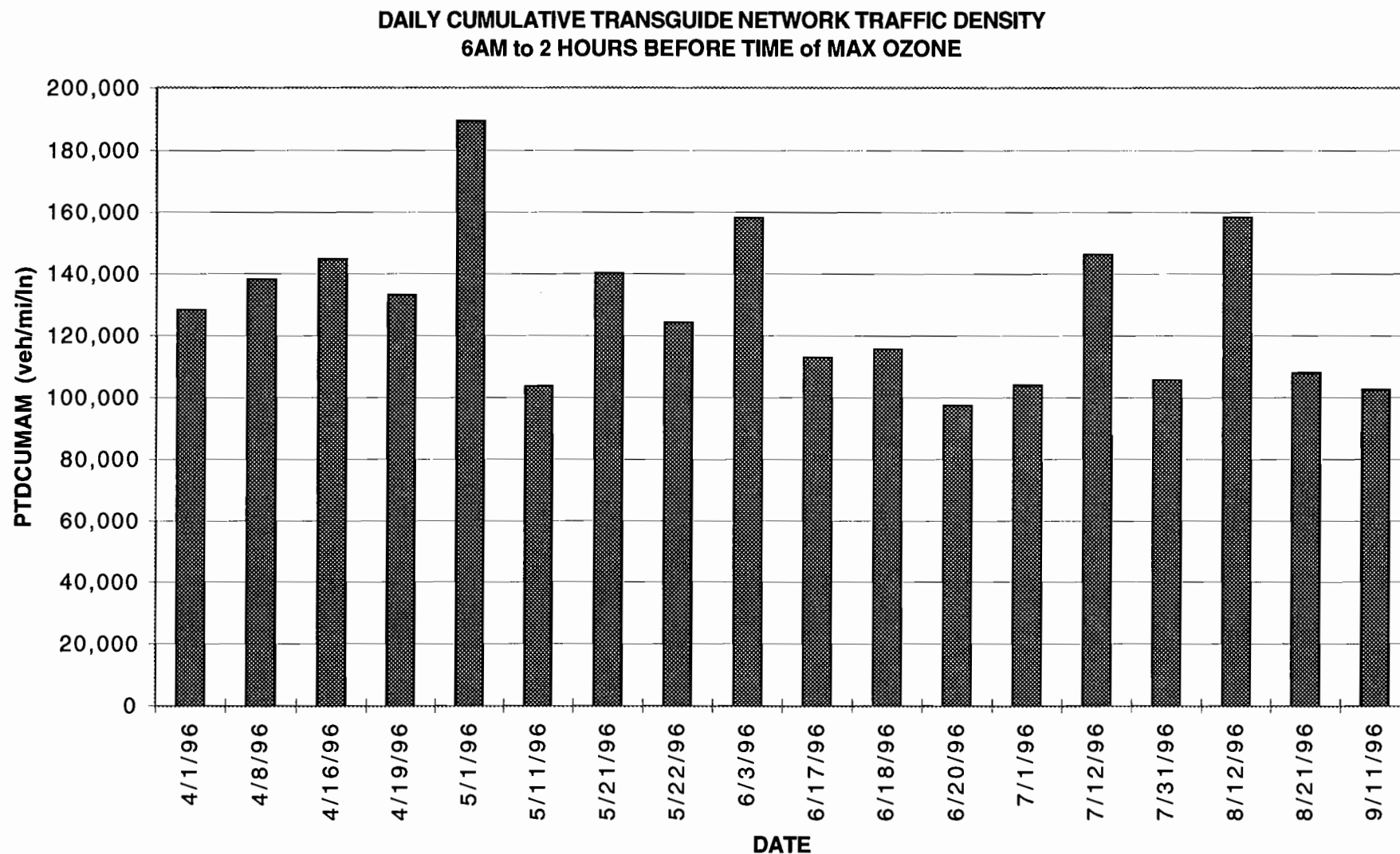
Figure 149. SAN ANTONIO APR'96-SEP'96 MODEL T13.1 DATA CONTROLLED FOR DAYS WITH TRAFFIC CONGESTION PARAMETER GE 50th PERCENTILE AND DAYS DURING OZONE EPISODES AND AVERAGE "MORNING" CLOUD COVER LE 3 OKTAS
