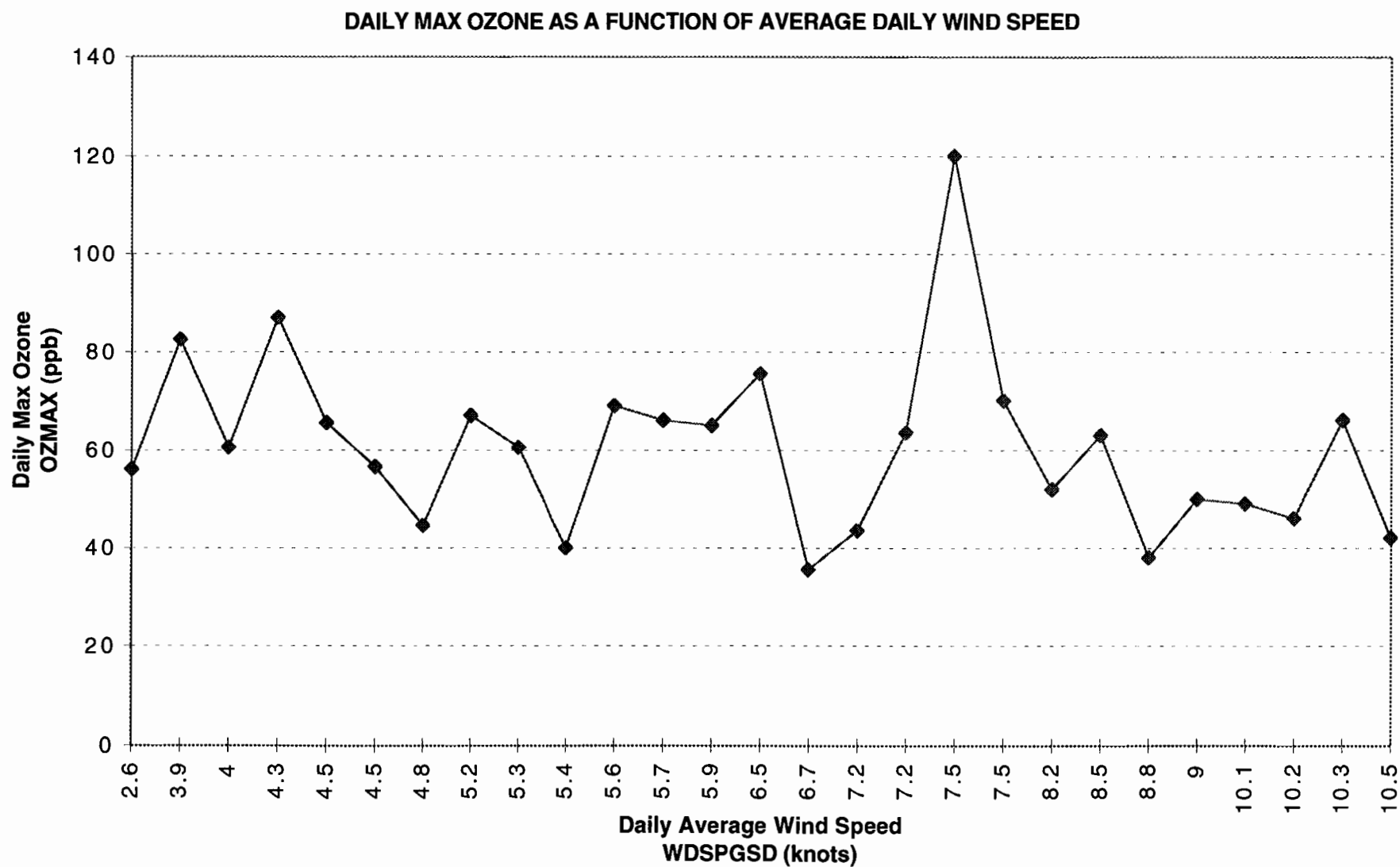
Figure 145. SAN ANTONIO DEC'95-SEP'96 MODEL T14 DATA CONTROLLED FOR DAYS WITH TRAFFIC CONGESTION PARAMETER GE 50th PERCENTILE AND DAYS DURING OZONE EPISODES AND AVERAGE "MORNING" CLOUD COVER LE 3 OKTAS
