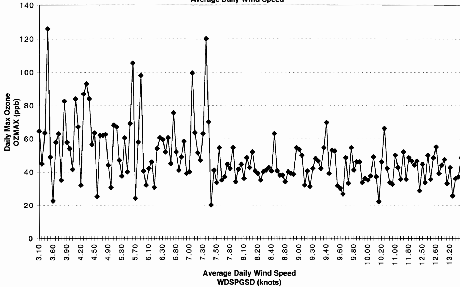
Figure 20. SAN ANTONIO APR'96-SEP'96 MODEL T2.1
