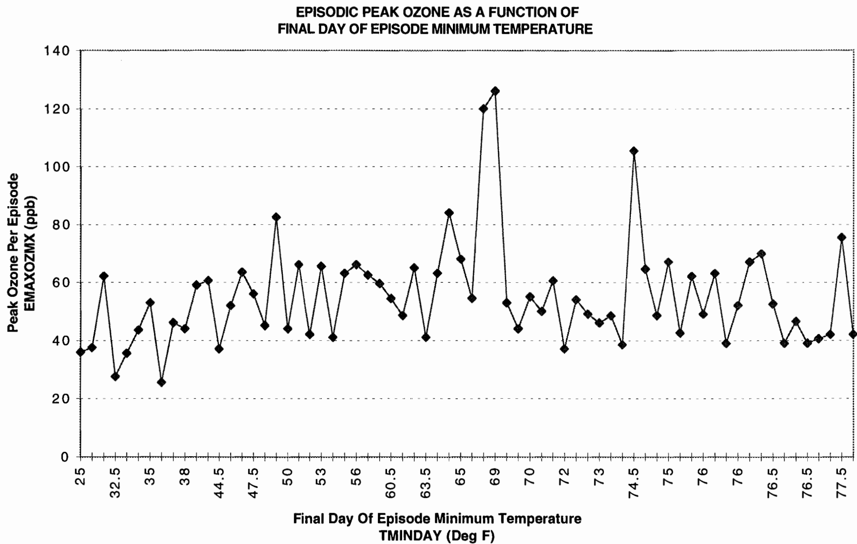
Figure 204. SAN ANTONIO DECEMBER'95 - SEPTEMBER'96 MODEL T43.0 DATA CONTROLLED FOR OZONE EPISODES - ONE OBSERVATION OF DATA PER EPISODE
