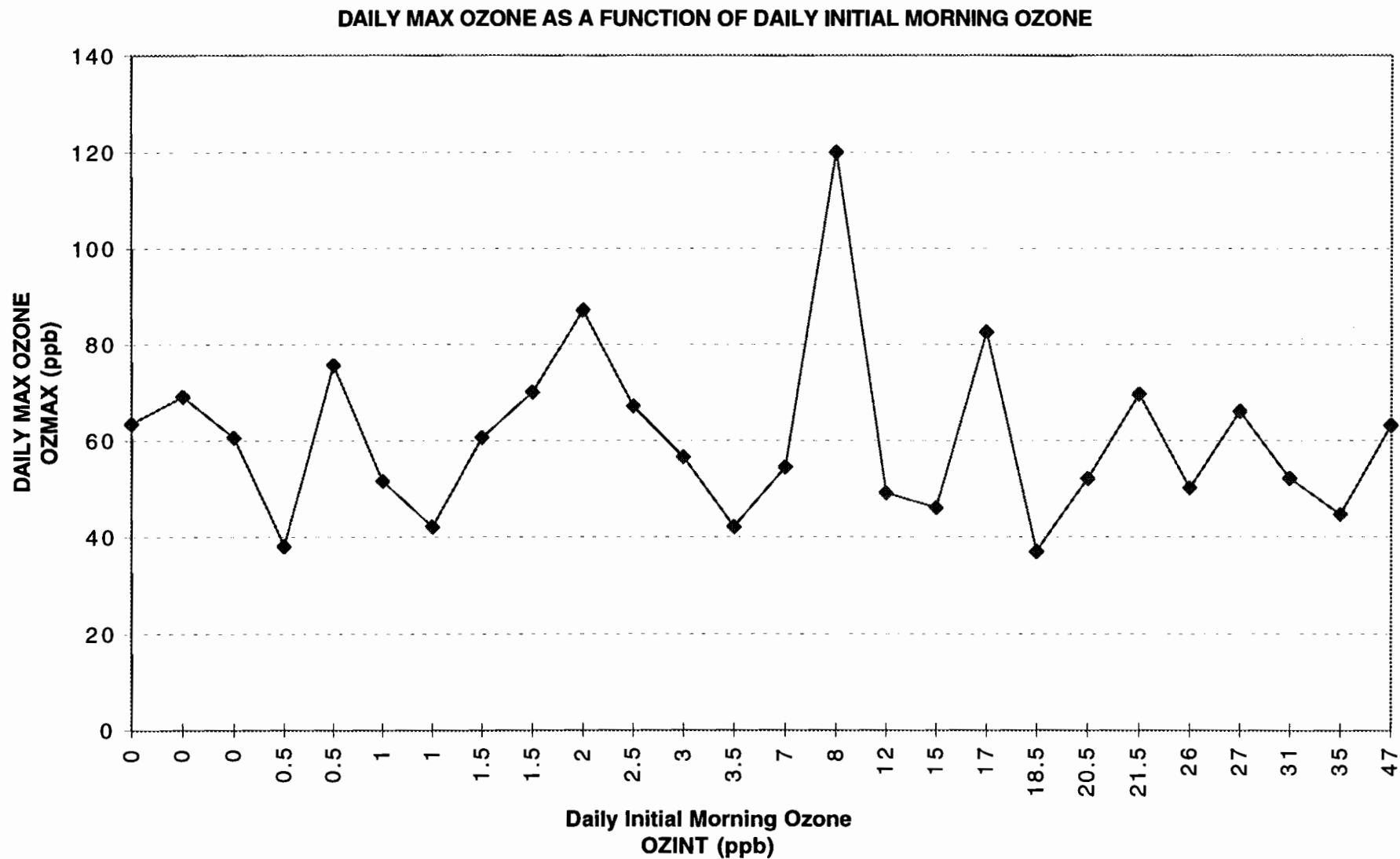
Figure 56. SAN ANTONIO APR'96-SEP'96 MODEL T11.1 DATA CONTROLLED FOR TRAFFIC CONGESTION PARAMETER GE 50th PERCENTILE AND DAYS WITH CLDAVGT2 LE 3
