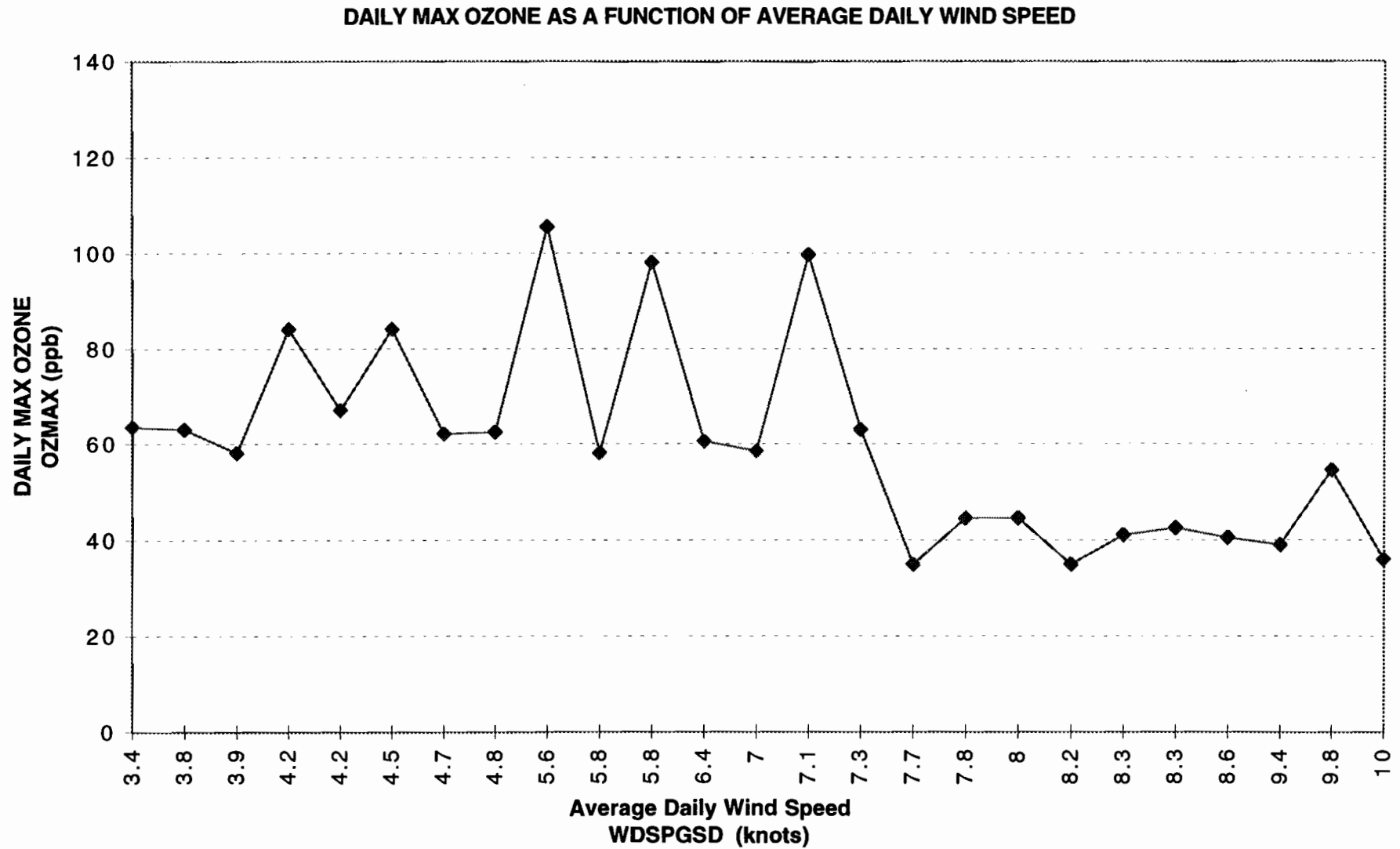
Figure 79. SAN ANTONIO APR'96-SEP'96 MODEL T11.2 DATA CONTROLLED FOR TRAFFIC CONGESTION PARAMETER LT 50th PERCENTILE AND DAYS WITH CLDAVGT2 LE 3
