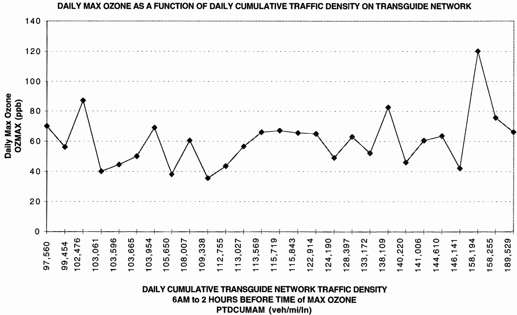
Figure 140. SAN ANTONIO DEC'95-SEP'96 MODEL T14 DATA CONTROLLED FOR DAYS WITH TRAFFIC CONGESTION PARAMETER GE 50th PERCENTILE AND DAYS DURING OZONE EPISODES AND AVERAGE "MORNING" CLOUD COVER LE 3 OKTAS
