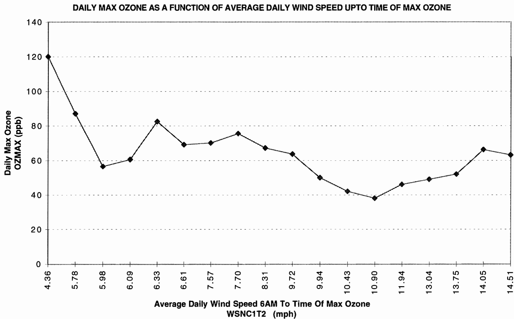
Figure 153. SAN ANTONIO APR'96-SEP'96 MODEL T13.1 DATA CONTROLLED FOR DAYS WITH TRAFFIC CONGESTION PARAMETER GE 50th PERCENTILE AND DAYS DURING OZONE EPISODES AND AVERAGE "MORNING" CLOUD COVER LE 3 OKTAS
