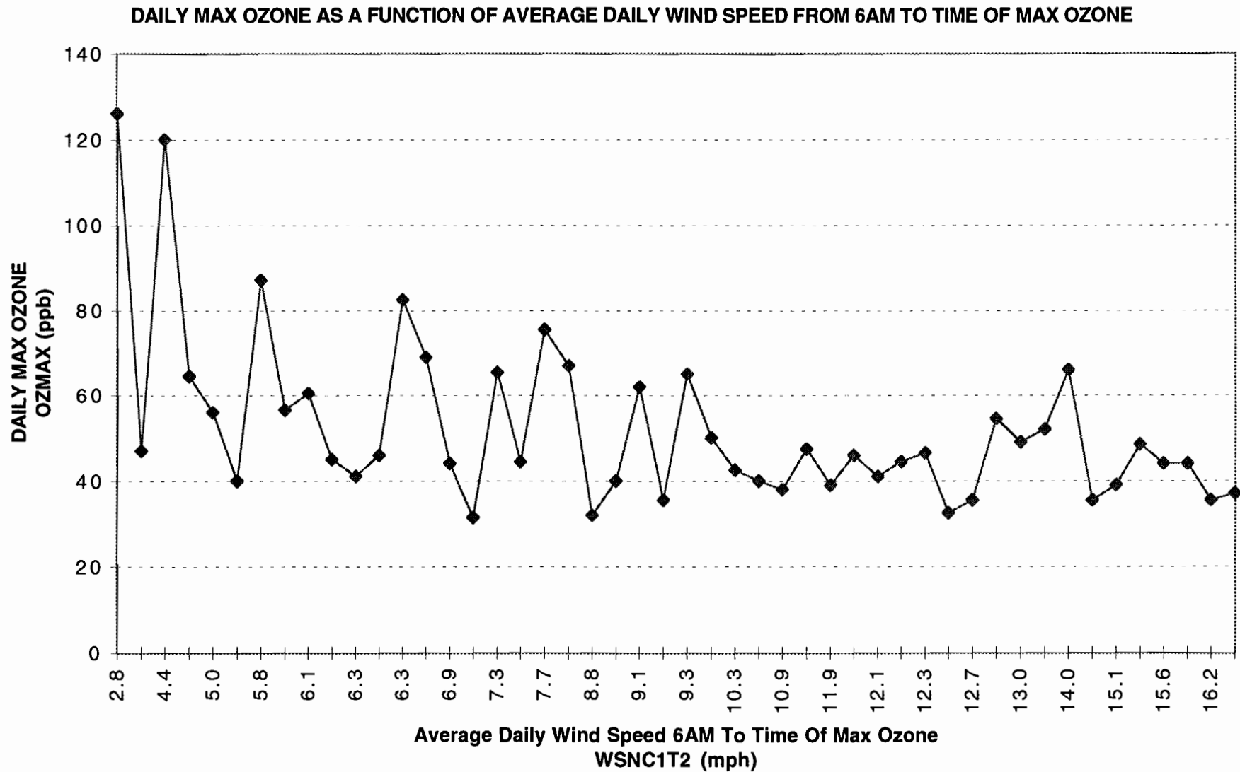
Figure 181. SAN ANTONIO DEC'95-SEP'96 MODEL T10.3 DATA CONTROLLED FOR DAYS DURING OZONE EPISODES GT 1-DAY AND DAYS WITH TRAFFIC CONGESTION PARAMETER GE 50th PERCENTILE
