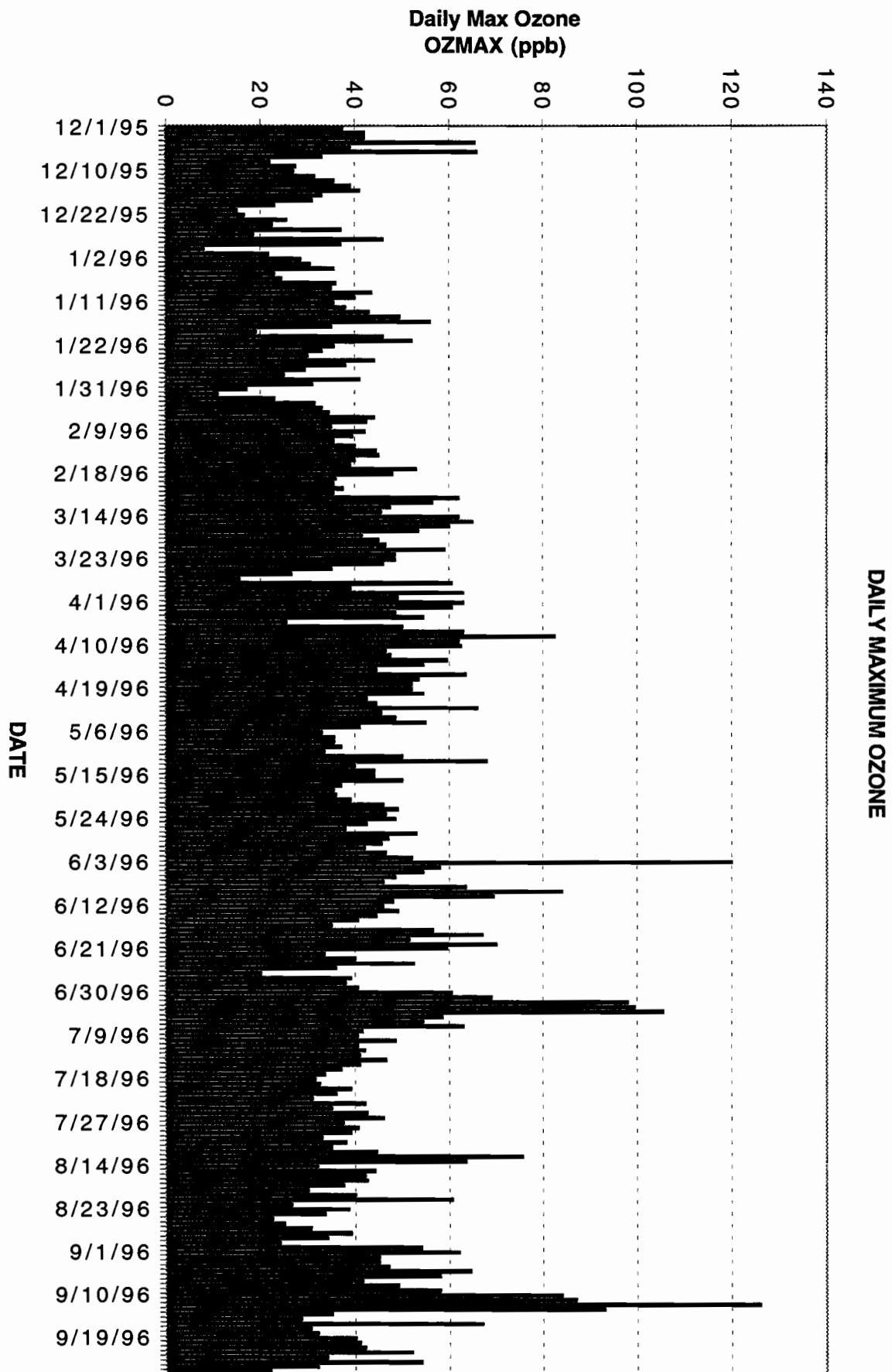
Figure 4. SAN ANTONIO DECEMBER'95-SEPTEMBER'96 MODEL T2.1.0
