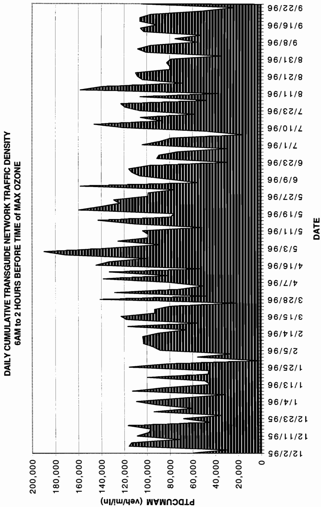
Figure 82. SAN ANTONIO DECEMBER'95 - SEPTEMBER'96 MODEL T22.0 DATA CONTROLLED FOR DAYS DURING OZONE EPISODES
