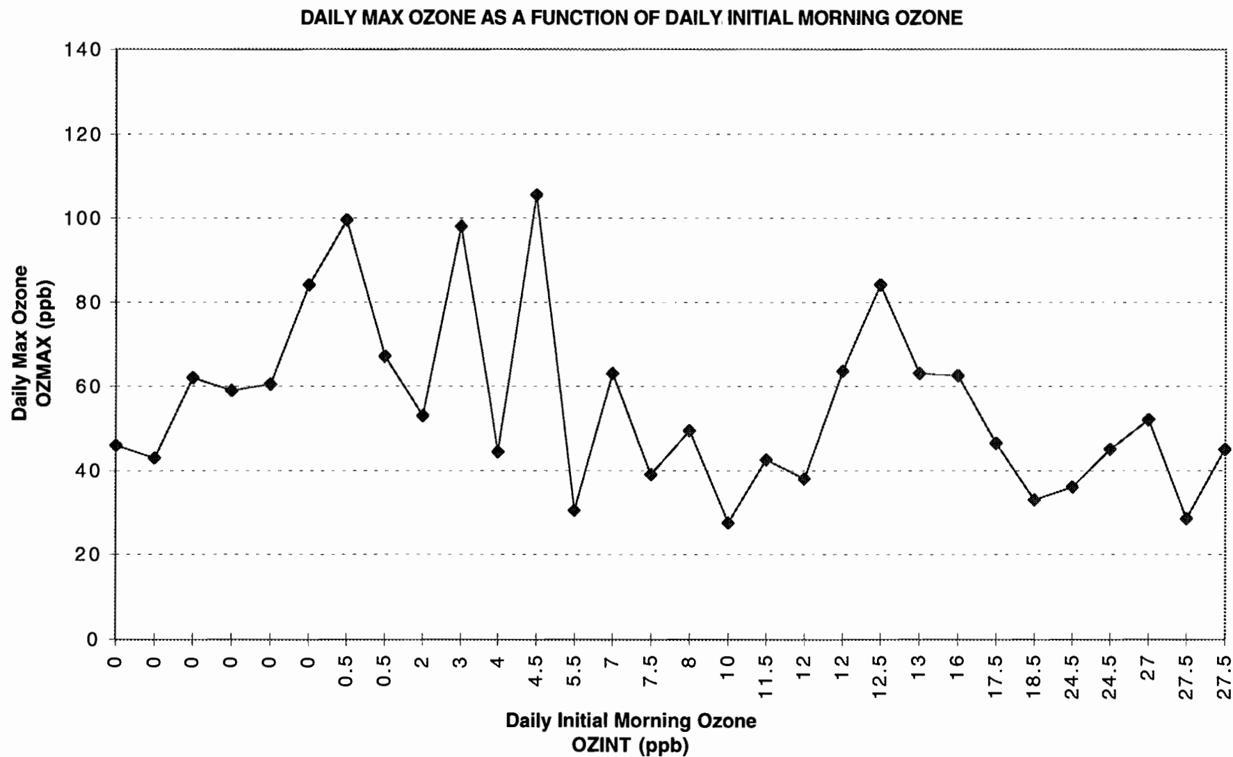
Figure 123. SAN ANTONIO DEC'95-SEP'96 MODEL T14.1 DATA CONTROLLED FOR DAYS WITH TRAFFIC CONGESTION PARAMETER LE 50th PERCENTILE AND DAYS DURING OZONE EPISODES AND AVERAGE "MORNING" CLOUD COVER LE 3 OKTAS
