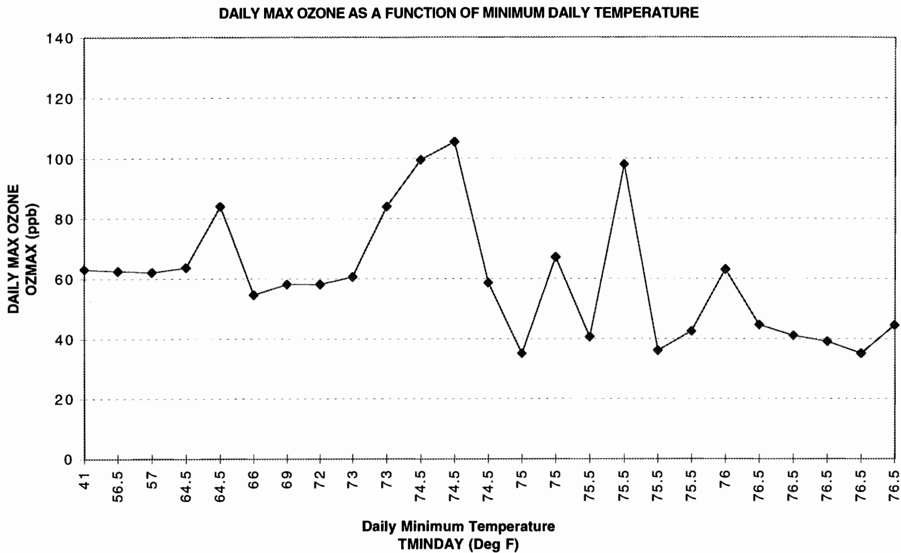
Figure 80. SAN ANTONIO DEC'95-SEP'96 MODEL T11.2 DATA CONTROLLED FOR TRAFFIC CONGESTION PARAMETER LT 50th PERCENTILE AND DAYS WITH CLDAVGT2 LE 3
