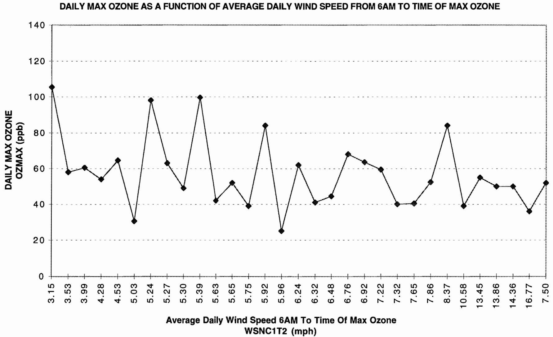
Figure 172. SAN ANTONIO APR'96-SEP'96 MODEL T19.1.1 DATA CONTROLLED FOR DAYS DURING OZONE EPISODES GT 1-DAY AND DAYS WITH TRAFFIC CONGESTION PARAMETER LT 50th PERCENTILE
