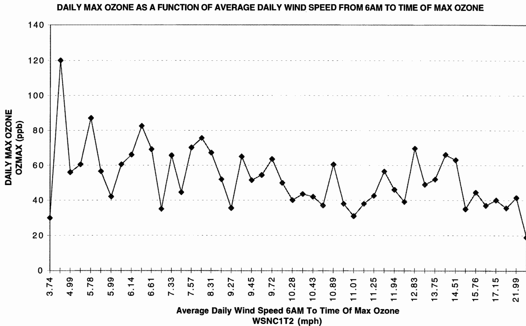
Figure 48. SAN ANTONIO DEC'95-SEP'96 MODEL T10.1 DATA CONTROLLED FOR TRAFFIC CONGESTION PARAMETER GE 50th PERCENTILE AND DAYS WITH CLDAVGT2 LE 3
