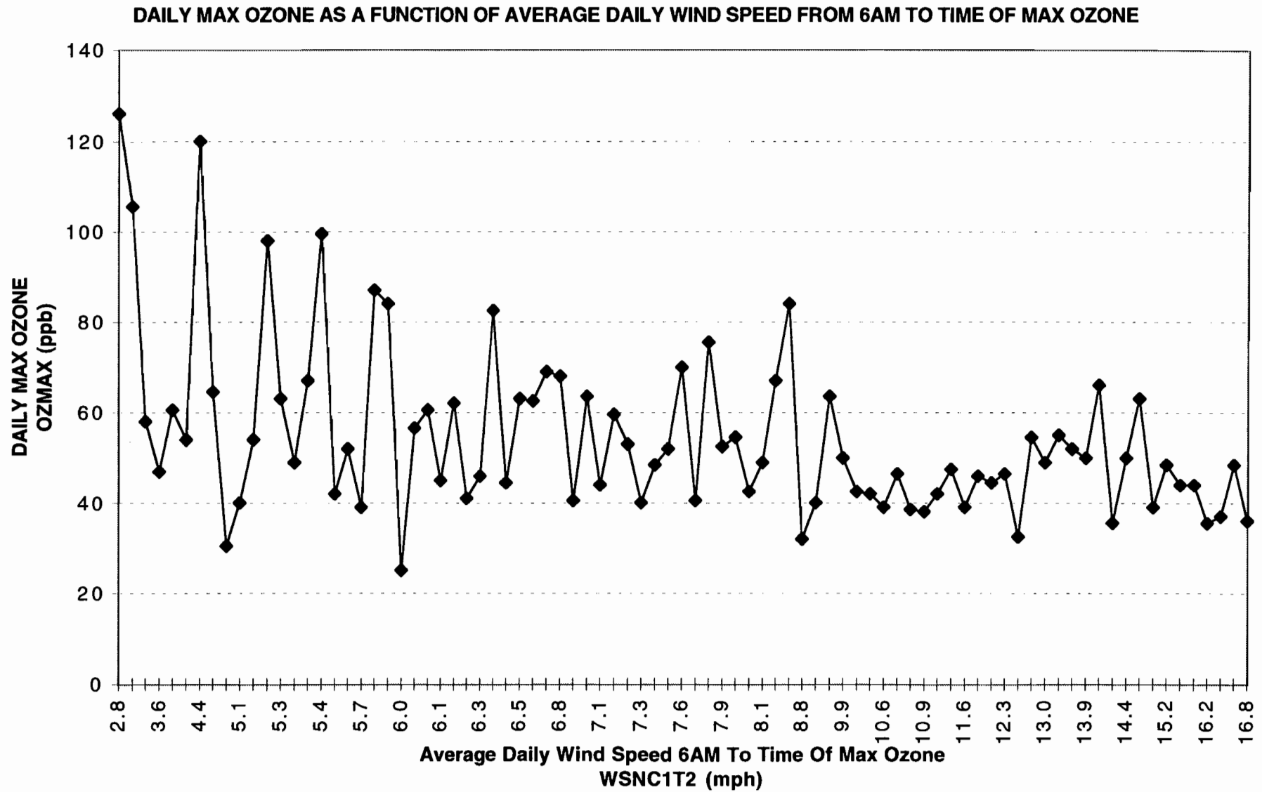
Figure 95. SAN ANTONIO APR'96-SEP'96 MODEL T22 DATA CONTROLLED FOR DAYS DURING OZONE EPISODES
