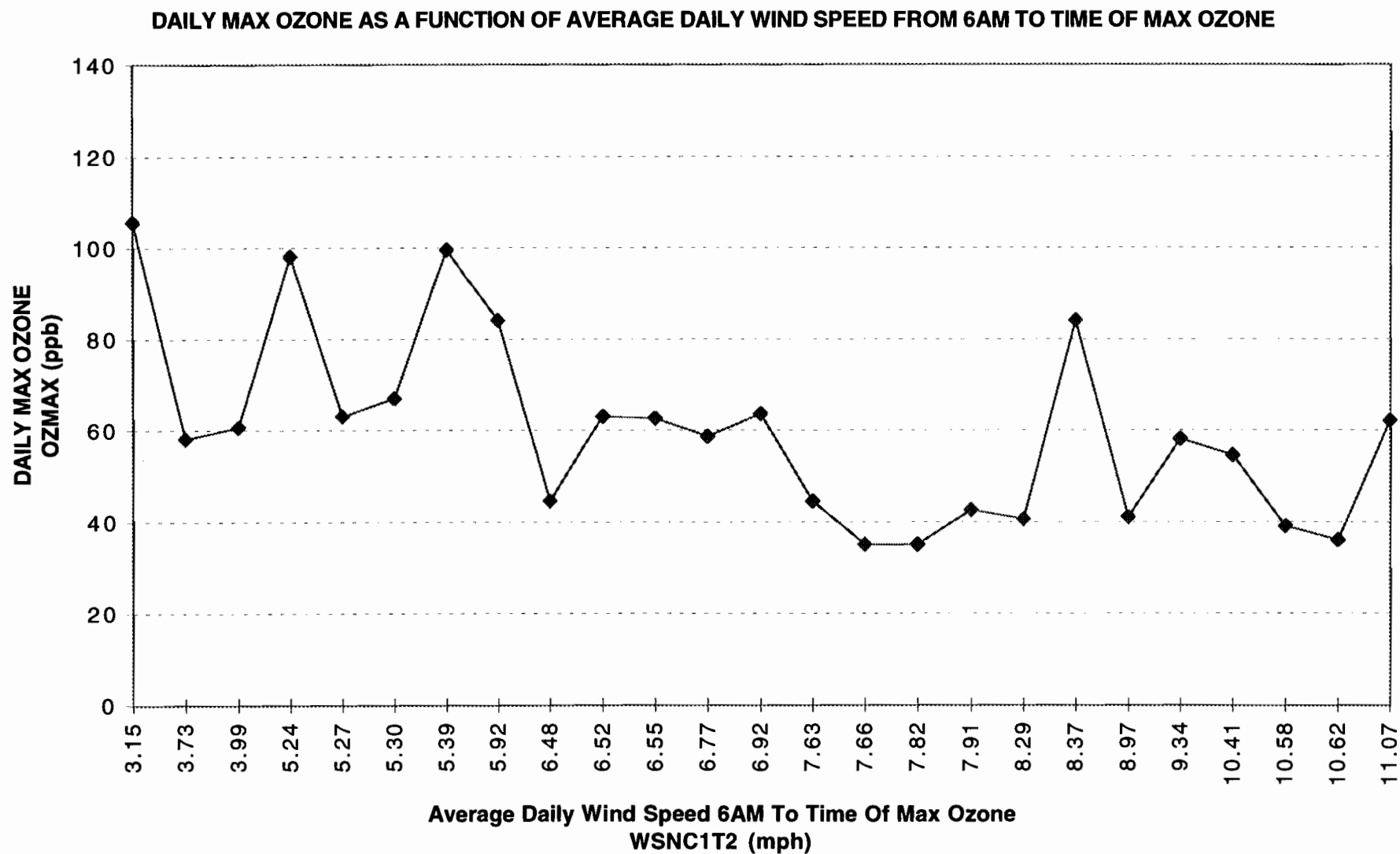
Figure 77. SAN ANTONIO APR'96-SEP'96 MODEL T11.2 DATA CONTROLLED FOR TRAFFIC CONGESTION PARAMETER LT 50th PERCENTILE AND DAYS WITH CLDAVGT2 LE 3
