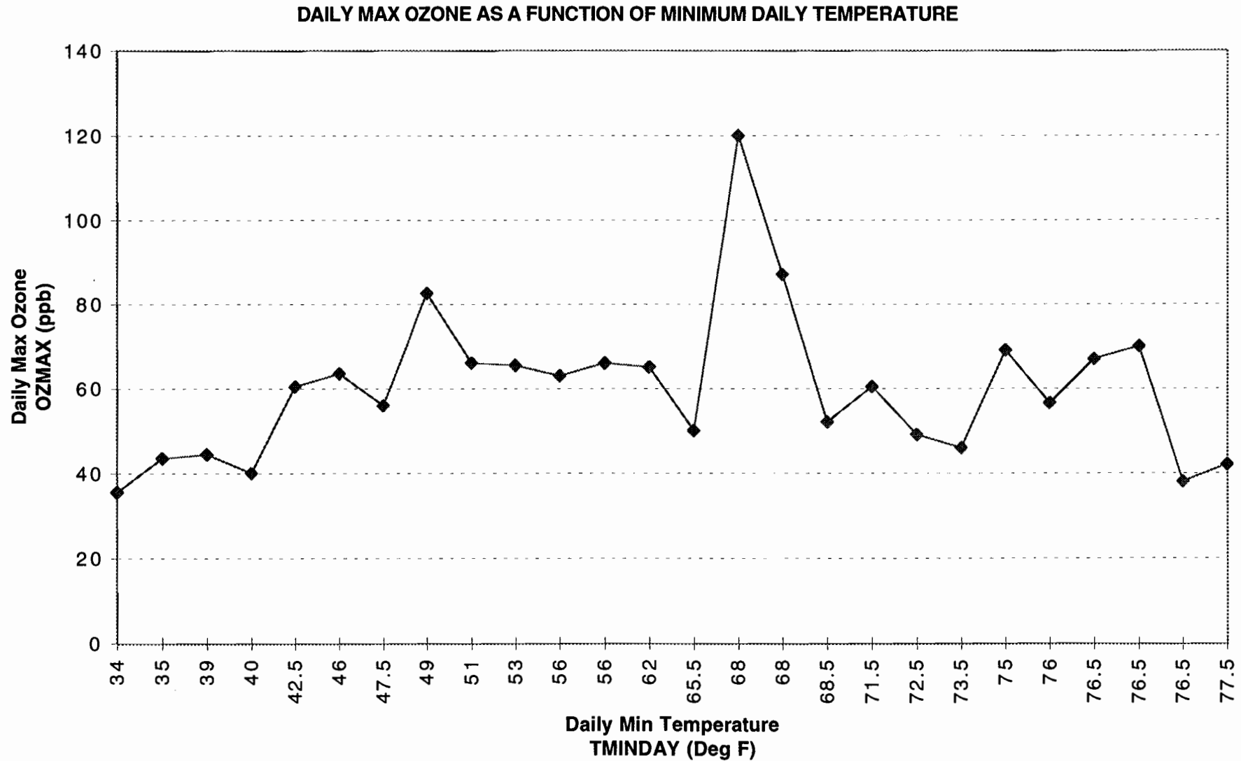
Figure 146. SAN ANTONIO DEC'95-SEP'96 MODEL T14 DATA CONTROLLED FOR DAYS WITH TRAFFIC CONGESTION PARAMETER GE 50th PERCENTILE AND DAYS DURING OZONE EPISODES AND AVERAGE "MORNING" CLOUD COVER LE 3 OKTAS
