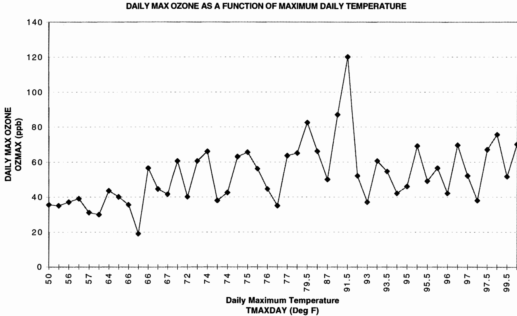
Figure 49. SAN ANTONIO DEC'95-SEP'96 MODEL T10.1 DATA CONTROLLED FOR TRAFFIC CONGESTION PARAMETER GE 50th PERCENTILE AND DAYS WITH CLDAVGT2 LE 3
