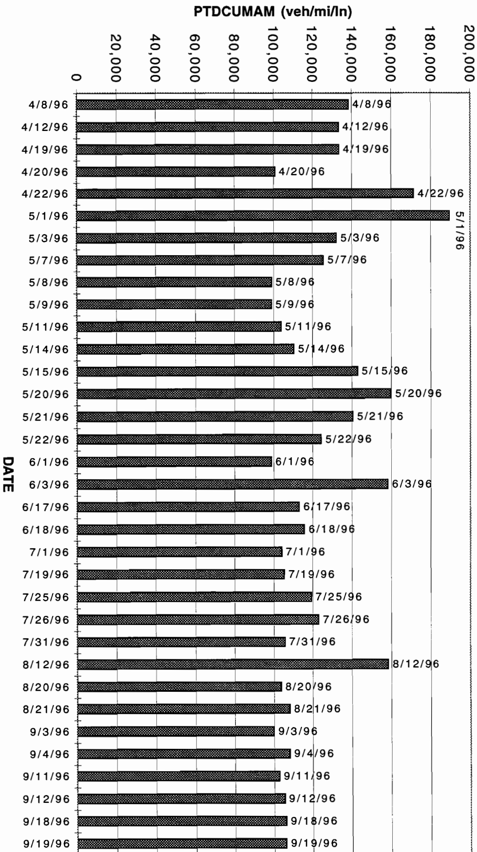
Figure 187. SAN ANTONIO APR'96-SEP'96 MODEL T19.1 DATA CONTROLLED FOR DAYS DURING OZONE EPISODES GT 1-DAY AND DAYS WITH TRAFFIC CONGESTION PARAMETER GE 50th PERCENTILE DAILY CUMULATIVE TRANSGUIDE NETWORK TRAFFIC DENSITY 6AM to 2 HOURS BEFORE TIME of MAX OZONE
