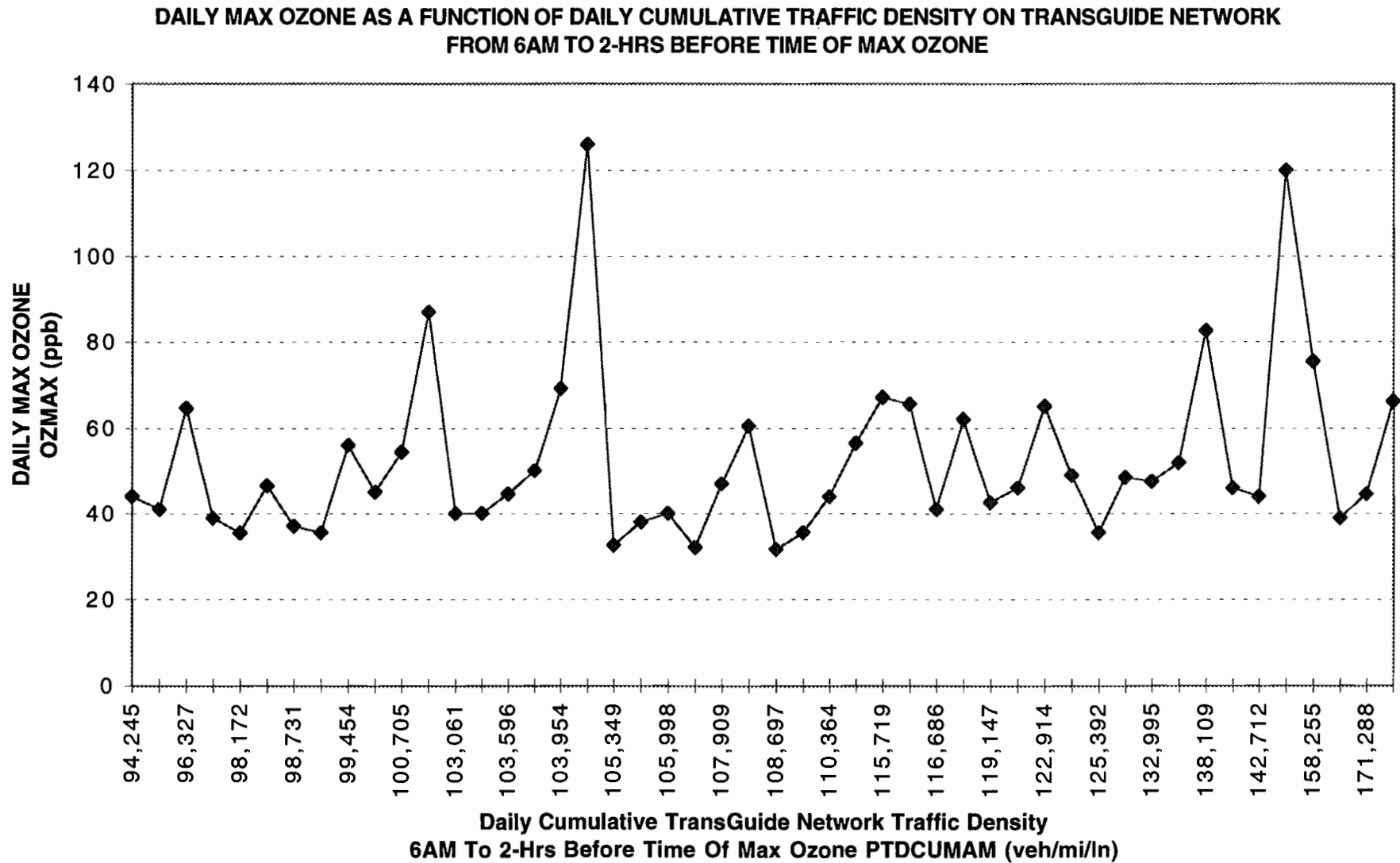
Figure 178. SAN ANTONIO DEC'95-SEP'96 MODEL T10.3 DATA CONTROLLED FOR DAYS DURING OZONE EPISODES GT 1-DAY AND DAYS WITH TRAFFIC CONGESTION PARAMETER GE 50th PERCENTILE
