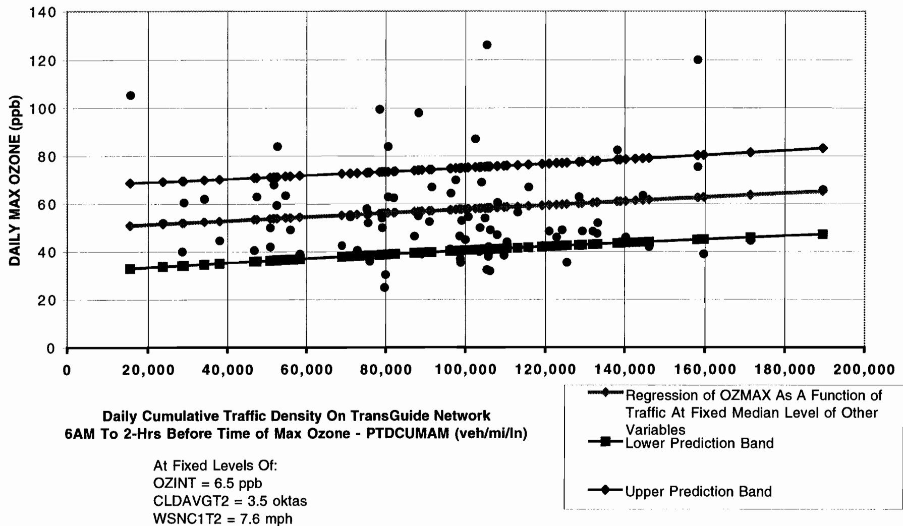
Figure 99. SAN ANTONIO APR'96-SEP'96 MODEL T22 DATA CONTROLLED FOR DAYS DURING OZONE EPISODES 80% CONFIDENCE PREDICTION BAND ON DAILY MAX OZONE AS A FUNCTION OF TRANSGUIDE NETWORK CUMULATIVE TRAFFIC DENSITY AT FIXED LEVELS OF OTHER INDEPENDENT VARIABLES (MEDIAN LEVELS)
