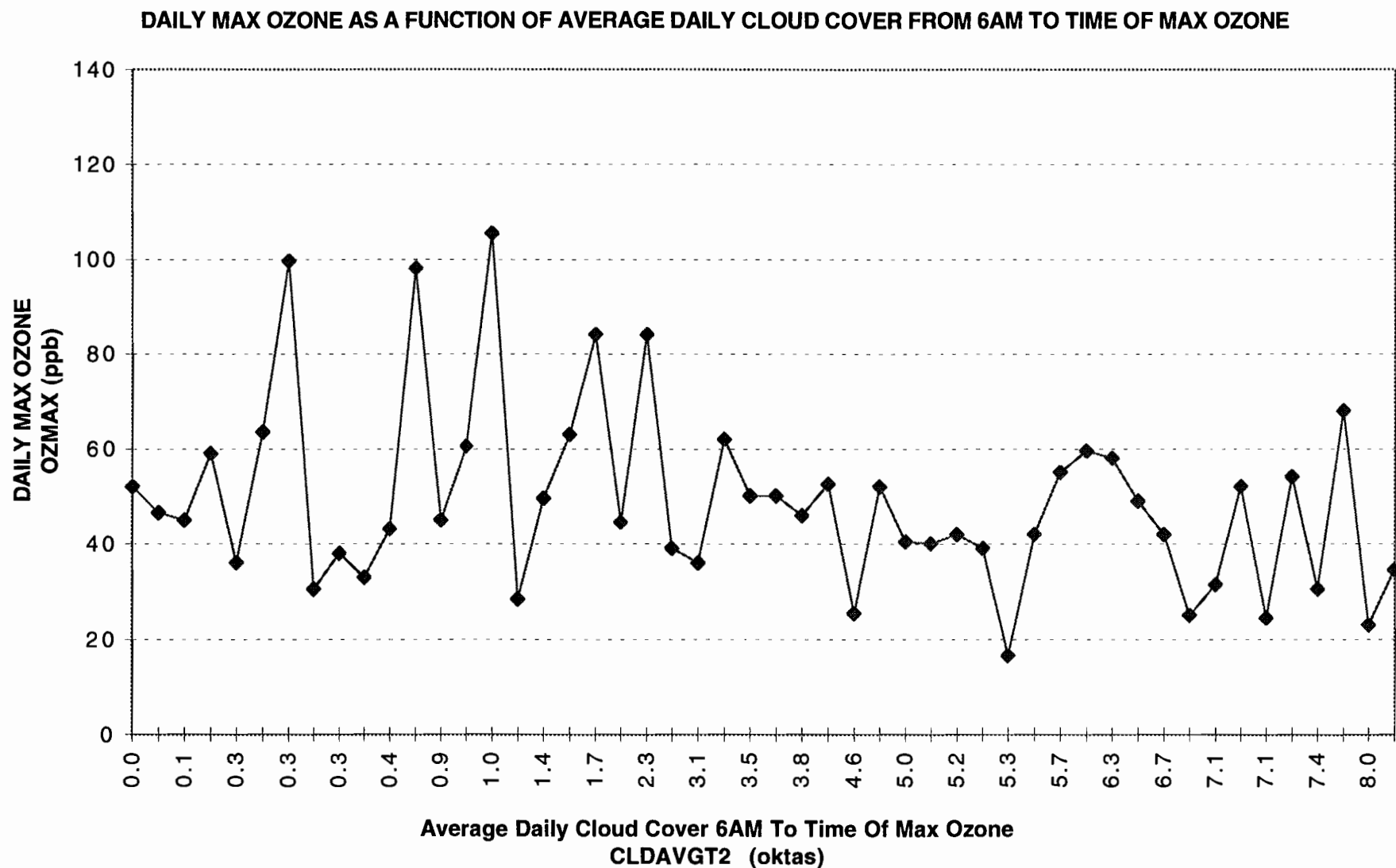
Figure 161. SAN ANTONIO DEC'95-SEP'96 MODEL T10.3.1 DATA CONTROLLED FOR DAYS DURING OZONE EPISODES GT 1-DAY AND DAYS WITH TRAFFIC CONGESTION PARAMETER LT 50th PERCENTILE
