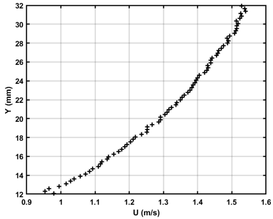
Figure 4.35 Average velocity profile in Test 1
