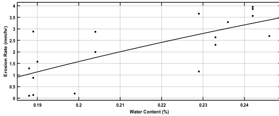
Figure 4.9 Erosion rate vs. water content for \tau_b > 19.5 \text{ N/m}^2
