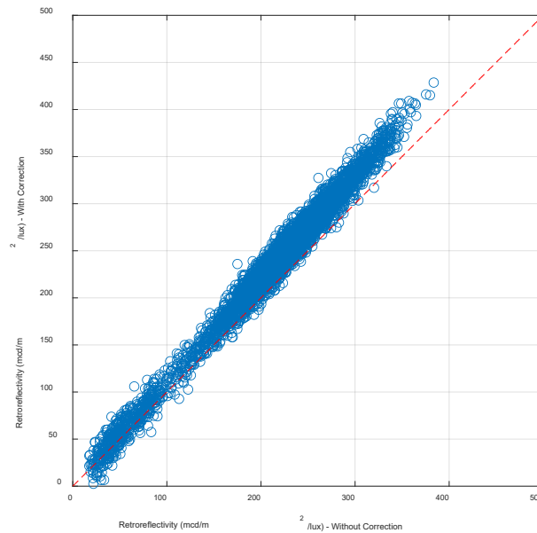
Figure 2.8: Correlation between calculated retroreflectivity with and without wet refraction index correction
