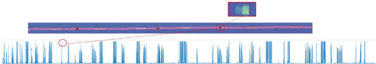
Figure 2.7: Observed RPM peaks in the point cloud data with high retroreflectivity
