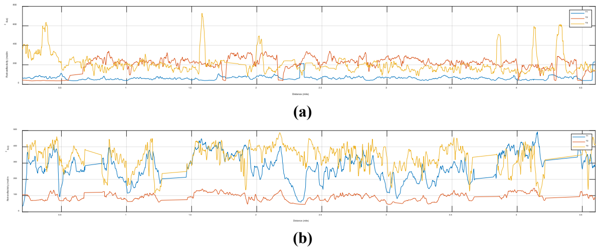
Figure 3.6: Retroreflectivity deterioration results for a sample thermoplastic site
