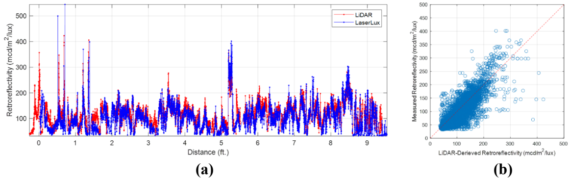
Figure 3.2: Correlation between retroreflectometer measurements and LiDAR-derived retroreflectivity for solid lines (originally reported in Phase 1)
