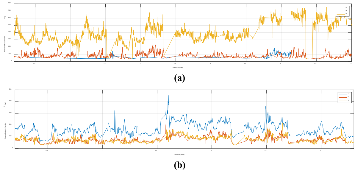
Figure 3.7: Retroreflectivity deterioration results for a sample tape site
