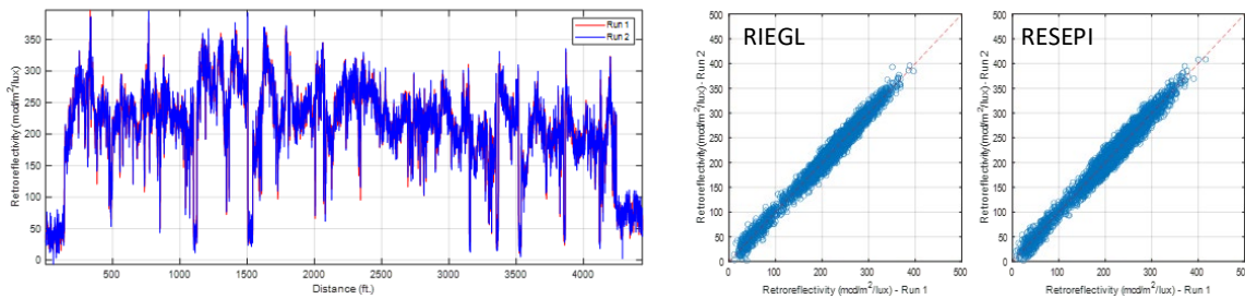
Figure 3.1: Repeatability of retroreflectivity measurements using different LiDAR systems
