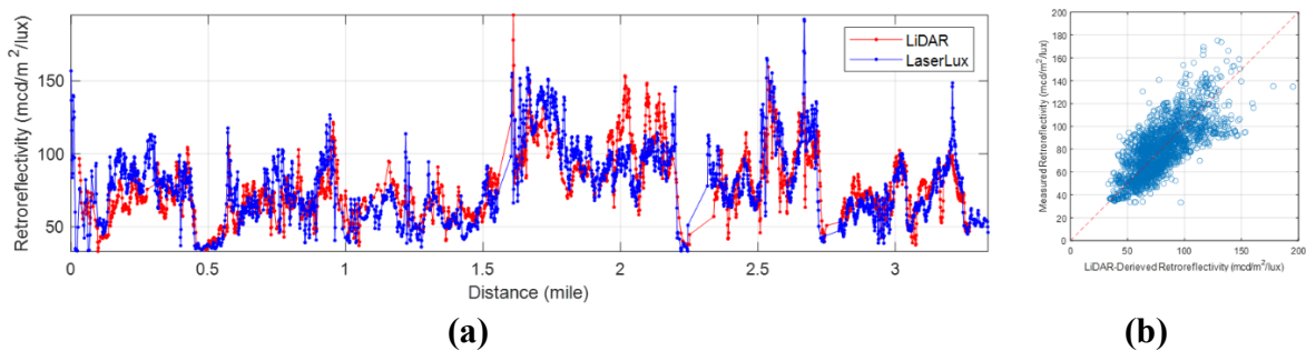
Figure 3.3: Correlation between retroreflectometer measurements and LiDAR-derived retroreflectivity for skip lines
