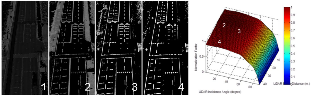
Figure 2.5: Examples of how incidence angle impacts retroreflectivity measurements
