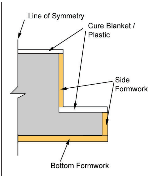
Figure 22 - Construction Summary form T-shaped Bent Cap
