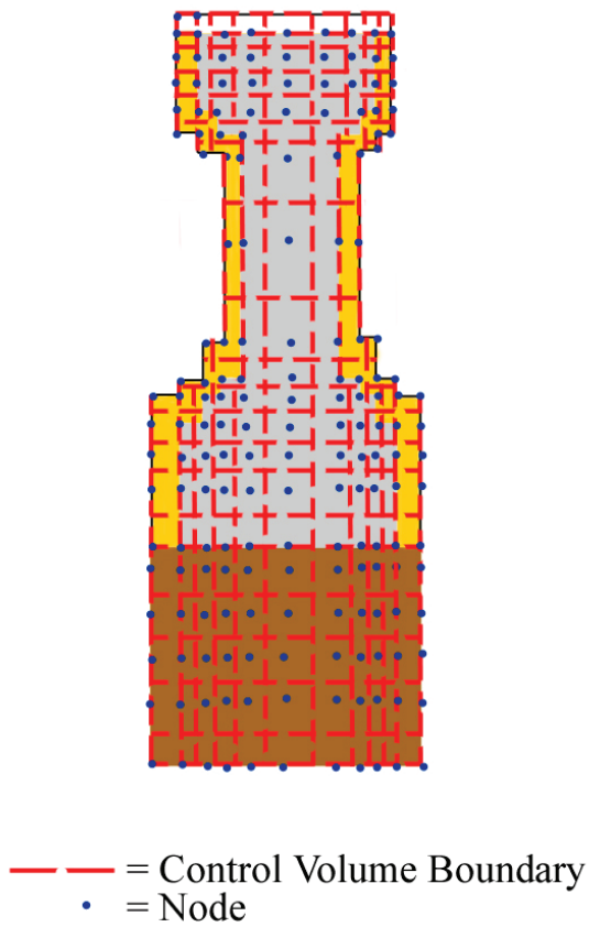
Figure 34 - Precast type IV beam node and control volume boundary layout
