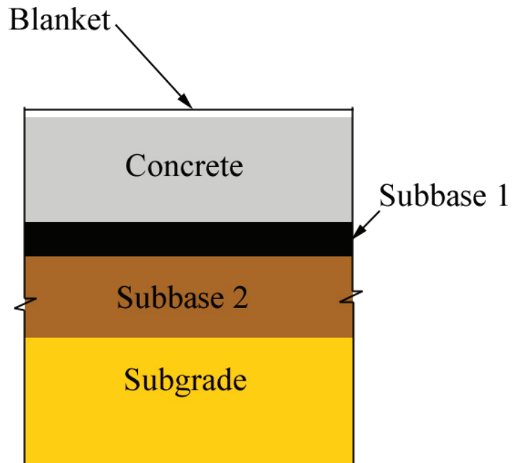
Figure 35 - Pavement layers modeled
