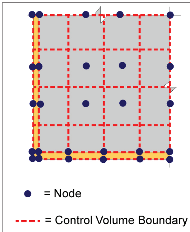
Figure 5 - Example rectangular column node and control volumes
