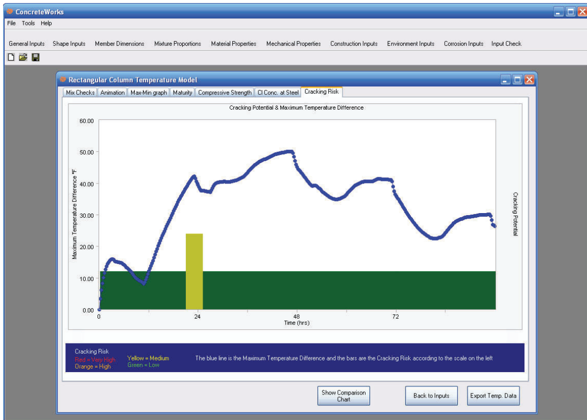
Figure 85 - Cracking Risk Classification Chart
