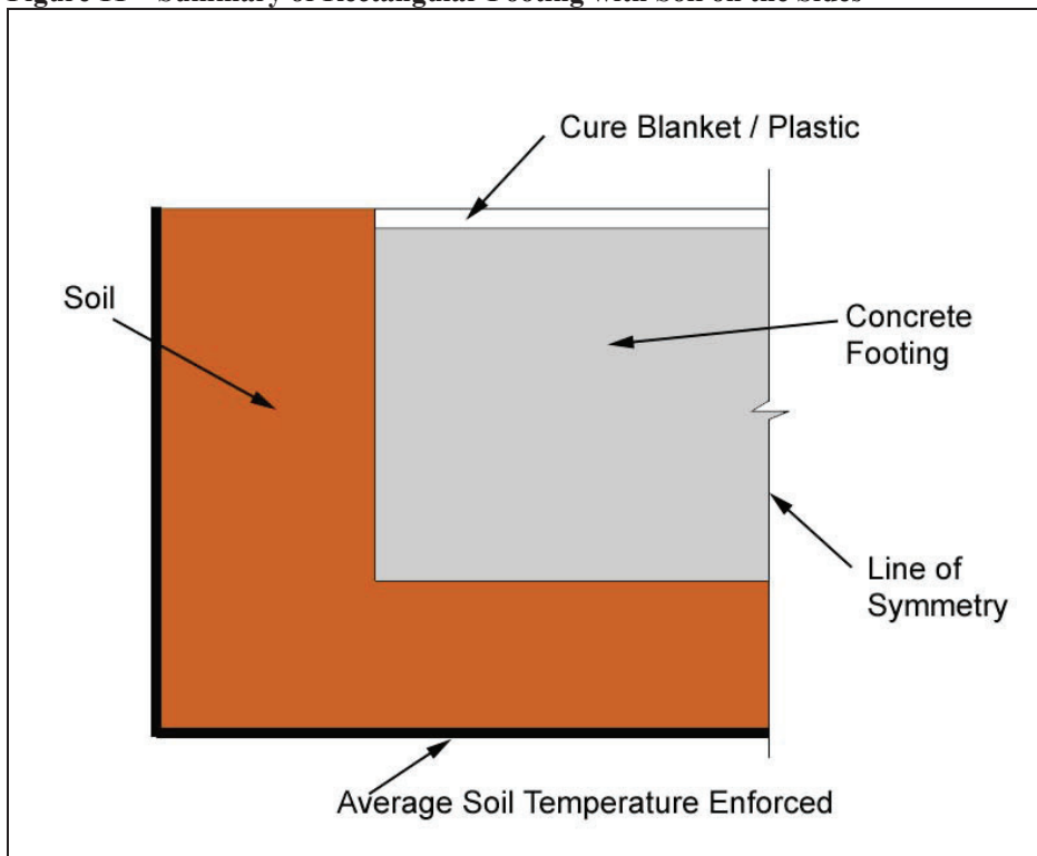
Figure 12 – Rectangular Footing with Soil on Sides Model
