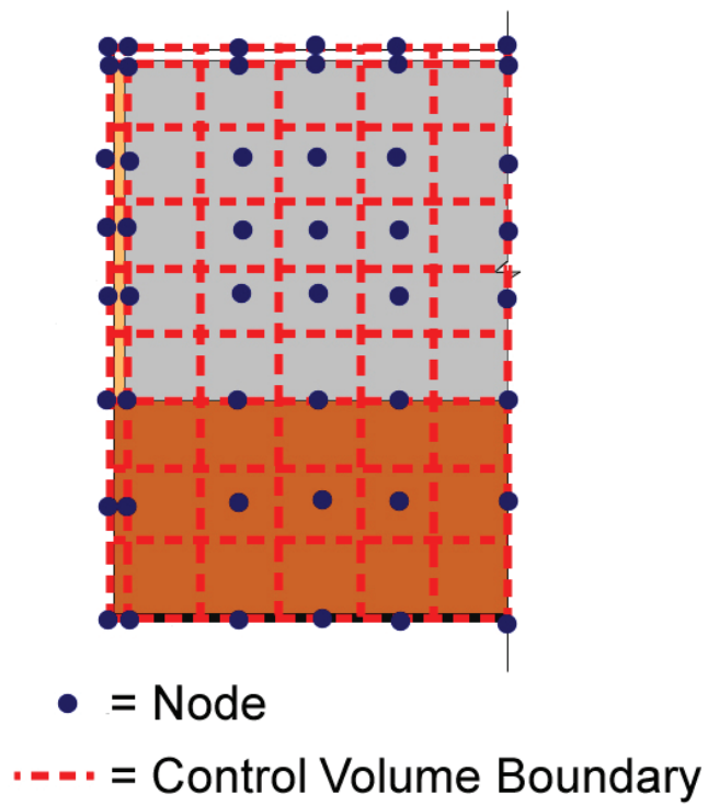
Figure 10 - Node layout for rectangular footing
