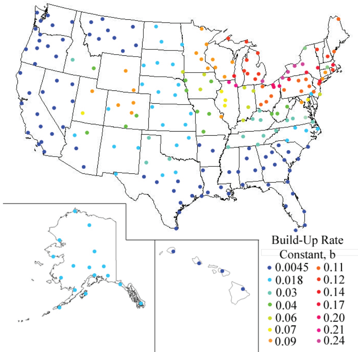
Figure 47- Build-up rate constants used in ConcreteWorks
