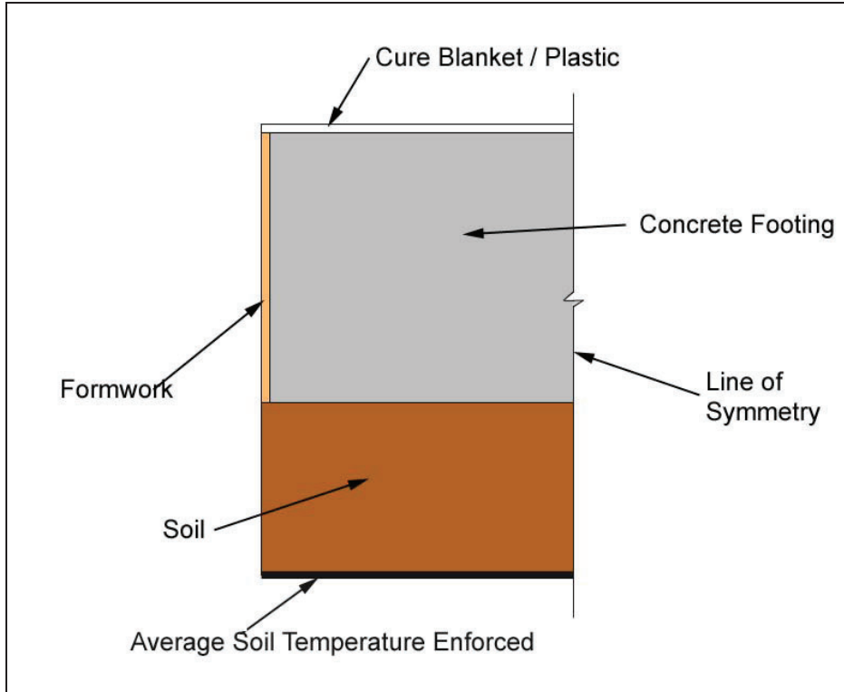
Figure 9 - Rectangular footing model
