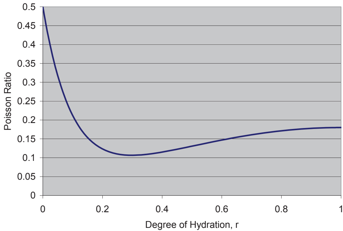
Figure 38 - Poisson ratio development during hydration
