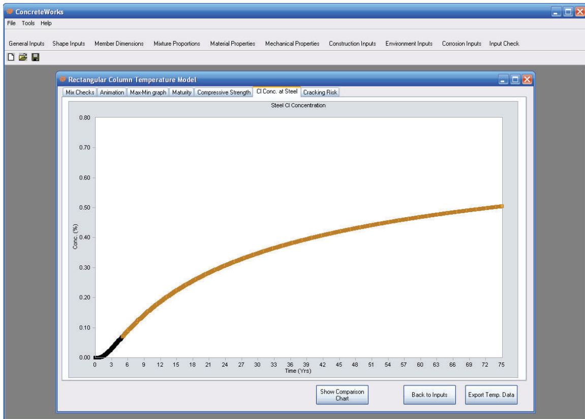
Figure 84 - Graph of Chloride Concentration at Steel
