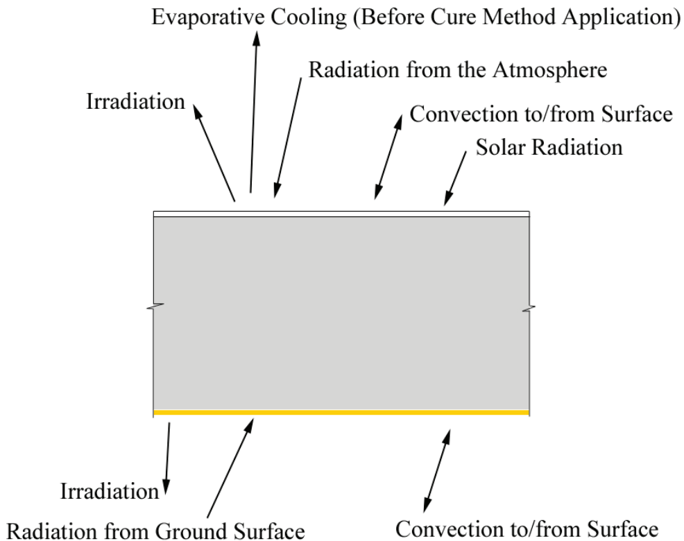
Figure 29 - Bridge deck temperature boundary conditions
