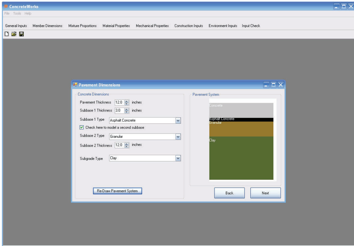
Figure 56 - Pavement Dimensions Input Screen
