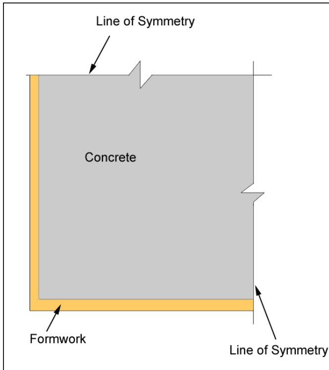
Figure 4 - Simplified rectangular column model used in ConcreteWorks
