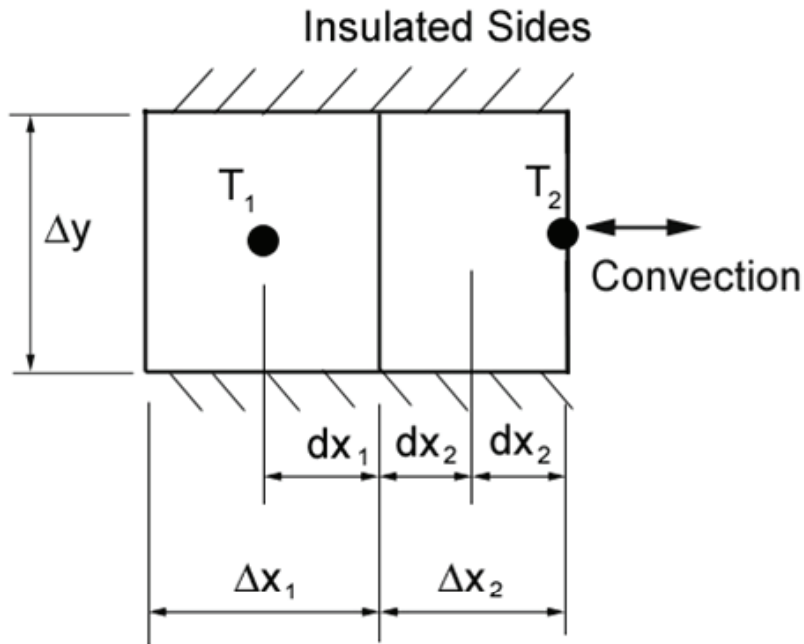
Figure 2 - Example of control volume with a convection boundary condition
