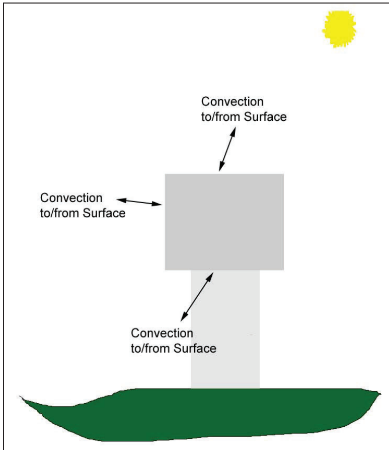
Figure 16 -Rectangular Bent Cap Convection Summary
