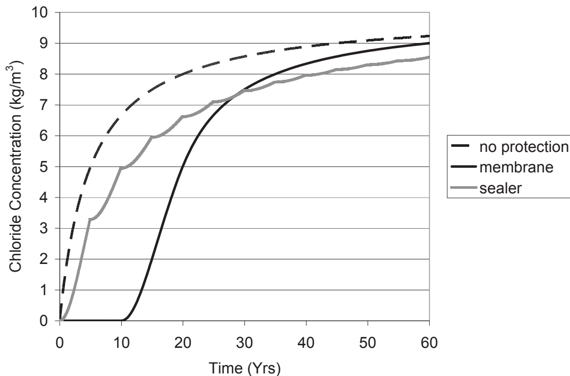
Figure 48 - Chloride surface concentration for cases where no barrier protection method is used, a membrane is used, and a sealer is used
