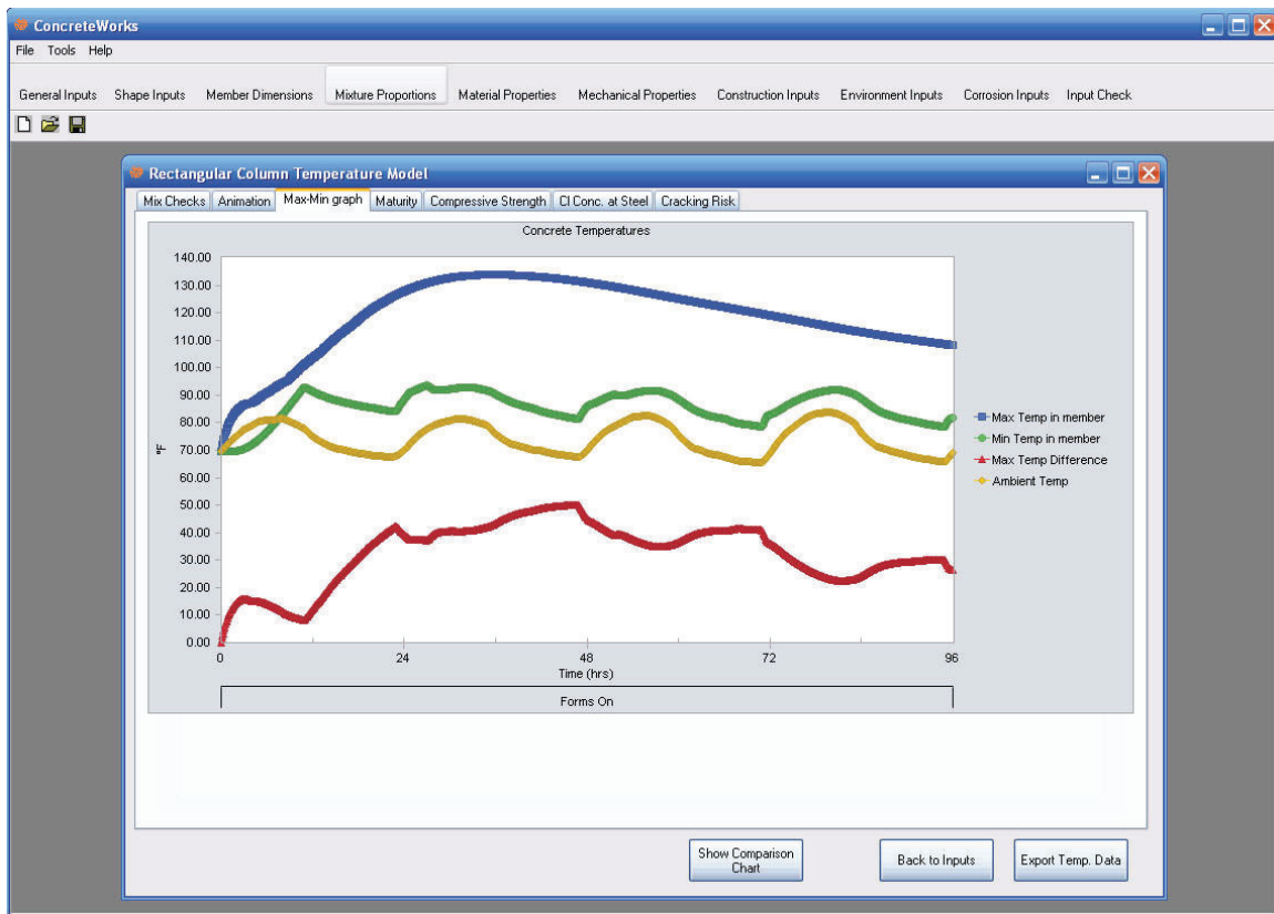
Figure 80 - Max-Min Graph tab as shown on the Rectangular Column Temperature Model screen
