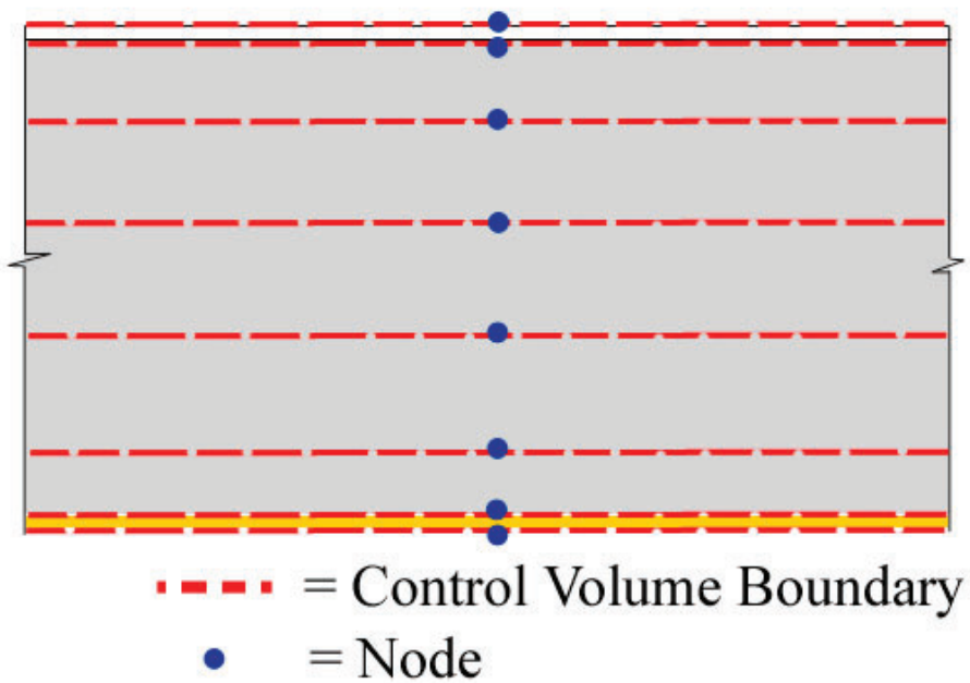
Figure 28 - Bridge deck node and control volume layout
