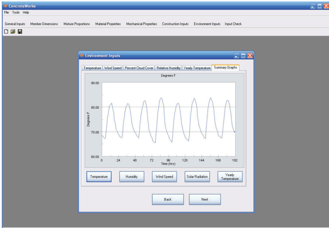
Figure 77 - Summary Graphs tab on the Environment Inputs screen - the temperature graph is currently displayed
