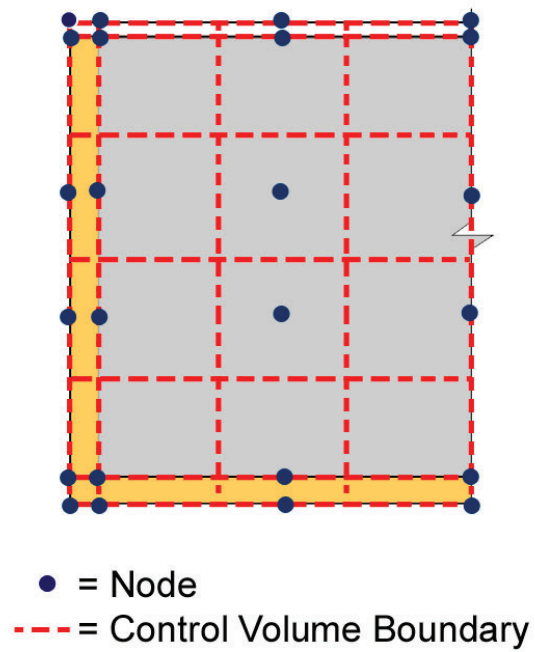
Figure 18 - Node and control volume layout of rectangular bent cap
