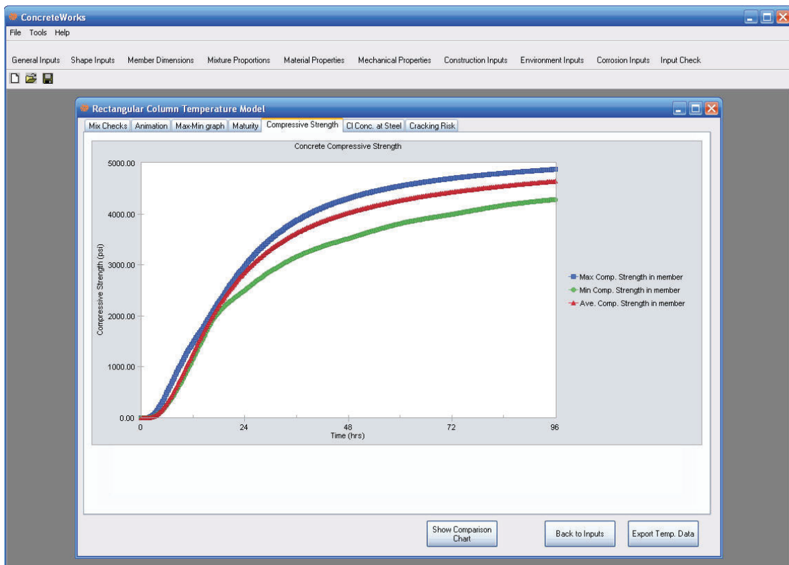
Figure 83 - Compressive Strength tab with compressive strength calculated as shown on the Rectangular Column Temperature Model screen
