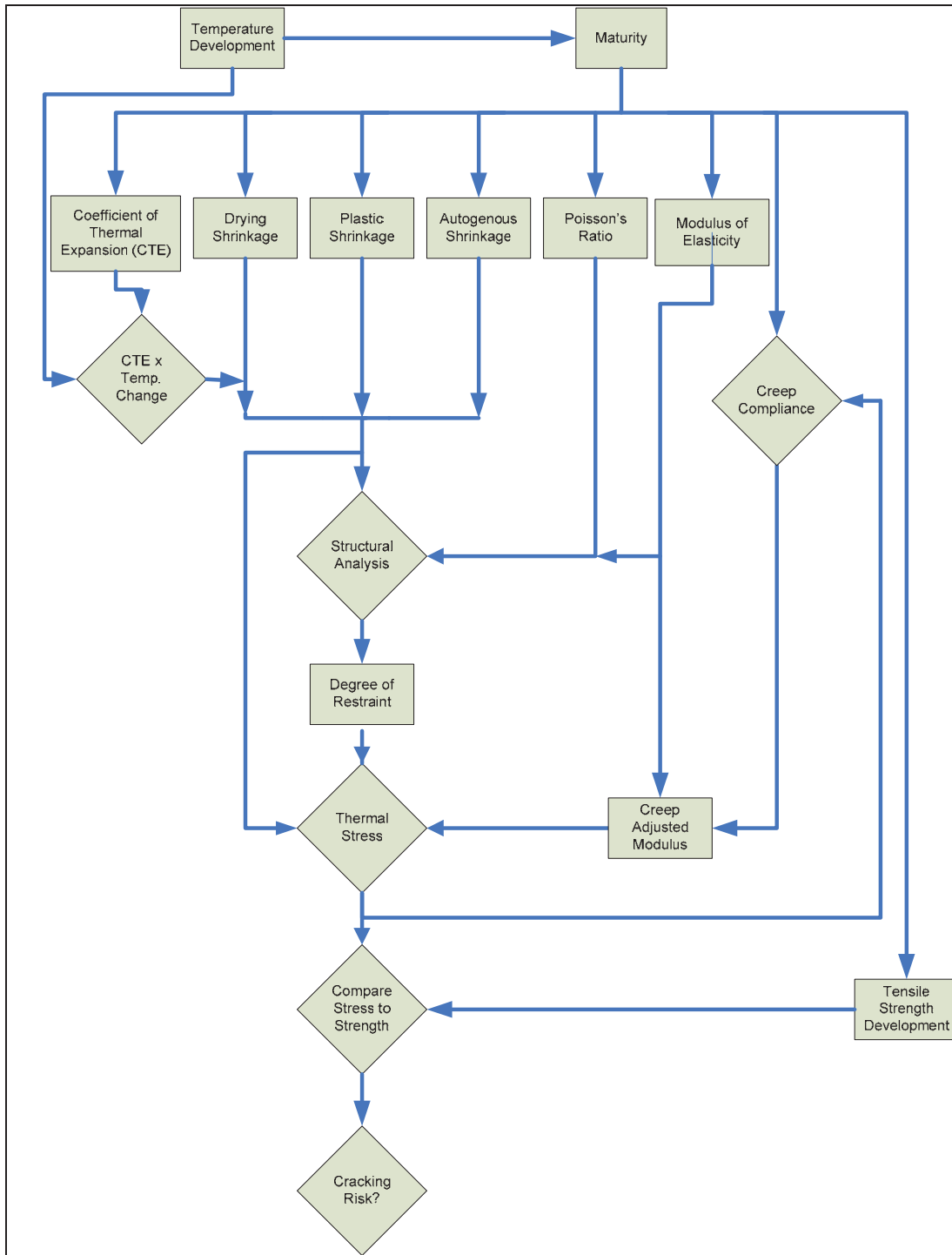
Figure 37 - Flow chart describing the relationship between different parameters in thermal stress modeling of concrete structures
