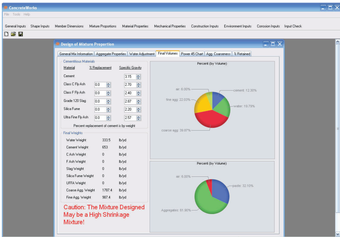
Figure 65 - Final Volume tab of the Design of Mixture Proportion screen
