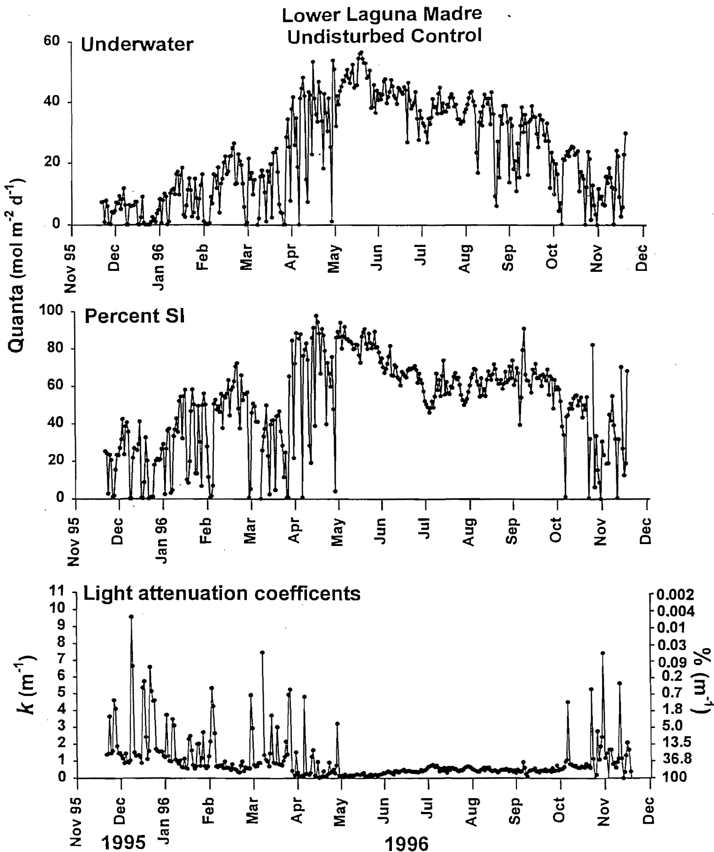
Figure 8. Underwater irradiance, percent surface irradiance (SI) and diffuse attenuation coefficient ( k ) at the Undisturbed Halodule site.
