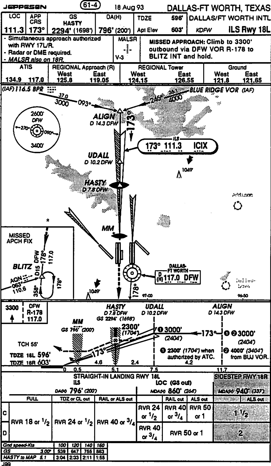
Figure 2. Prototype Volpe/ATA Part 121 IAP Chart for the ILS Approach to Runway 18 Left at Dallas/Fort Worth International Airport
