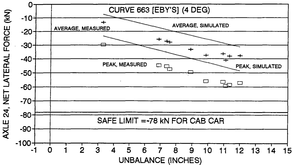
Figure 6.1(b): Measurement vs Prediction, Net Axle Lateral Force
