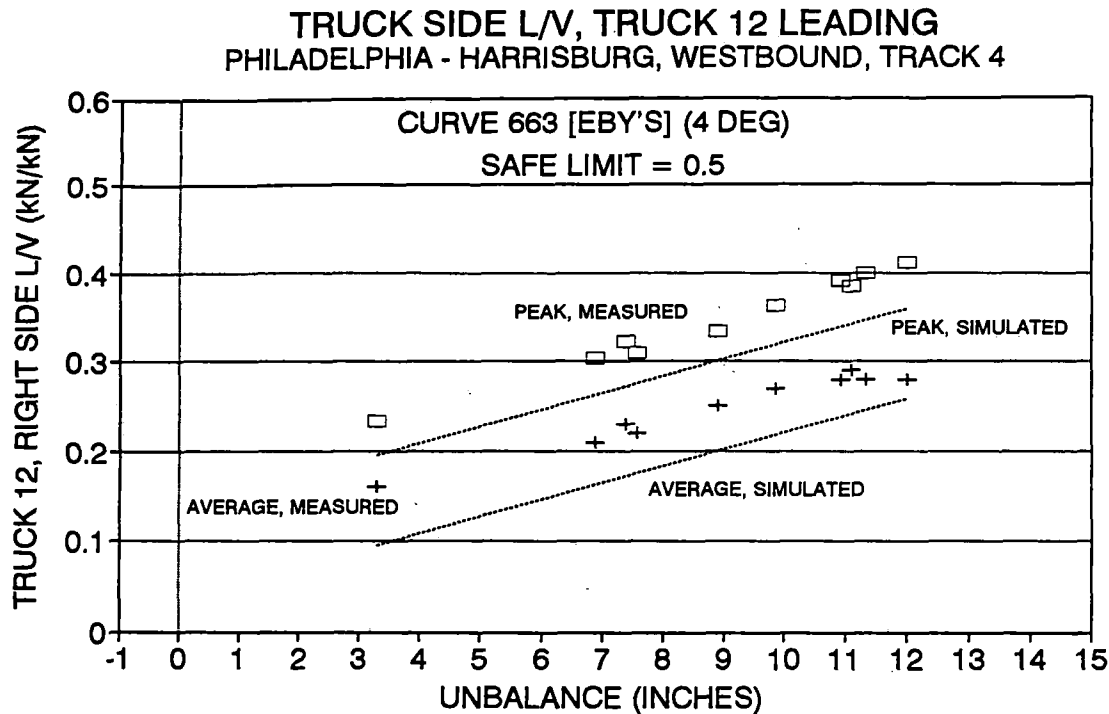
Figure 6.1(d): Measurement vs Prediction, Truck-Side L/V Ratio
