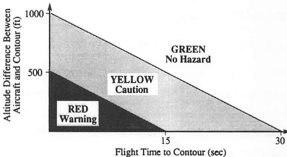
Figure 3.4 Prototypical GGPWS Contour Color Alerting Criteria
