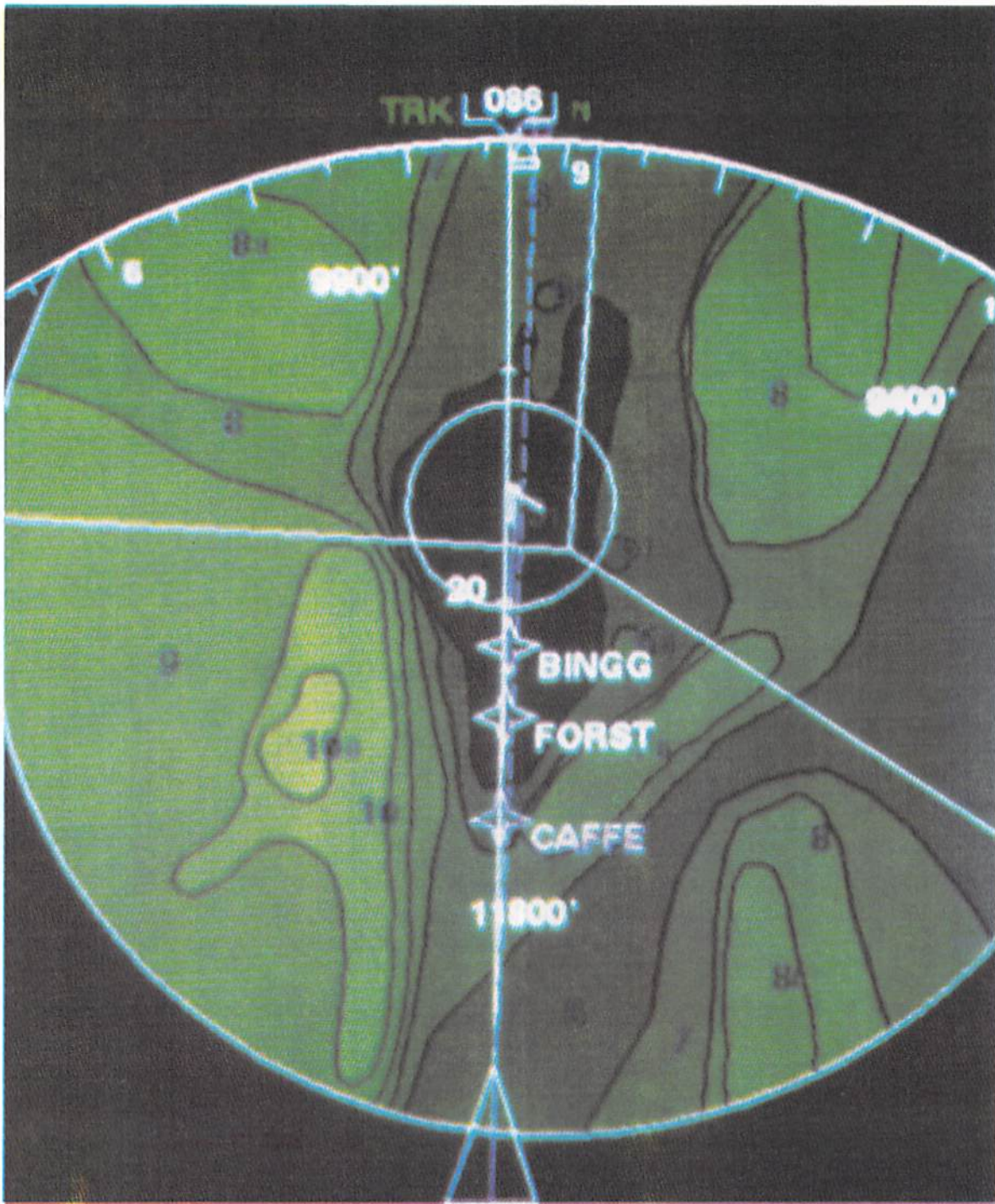
Figure 5.2 Prototypical Smoothed Contour Display
