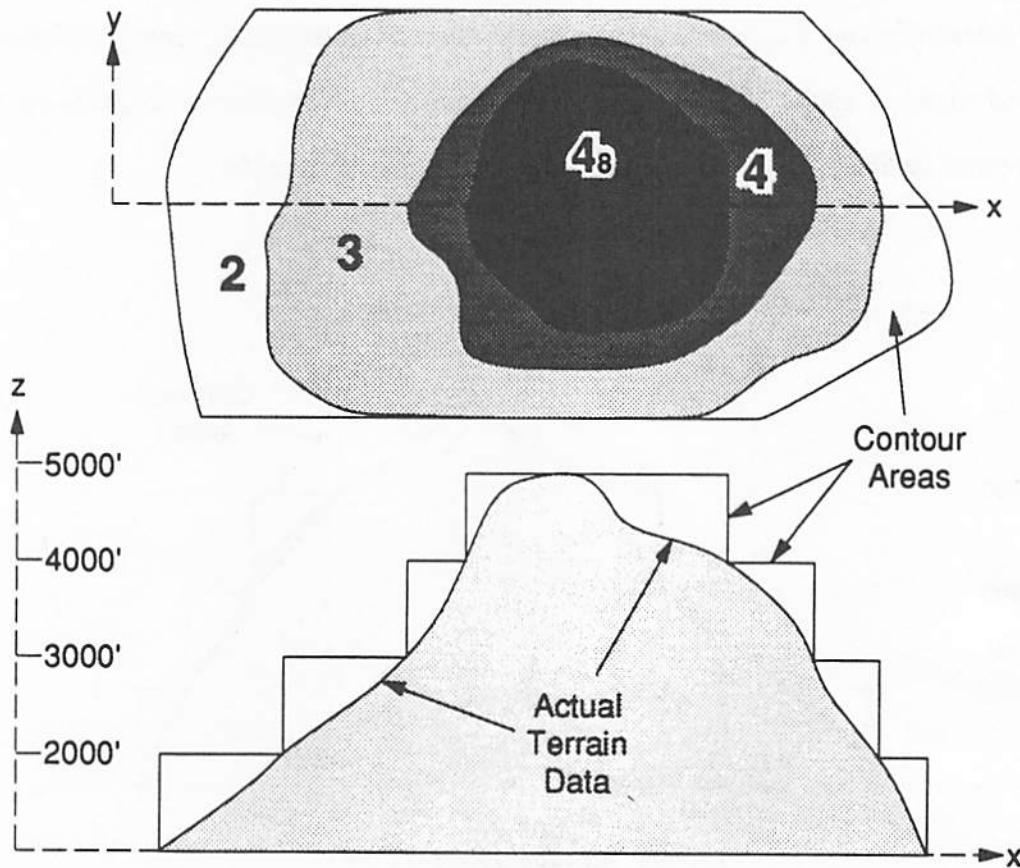
Figure 3.2 Coarse Terrain Model
