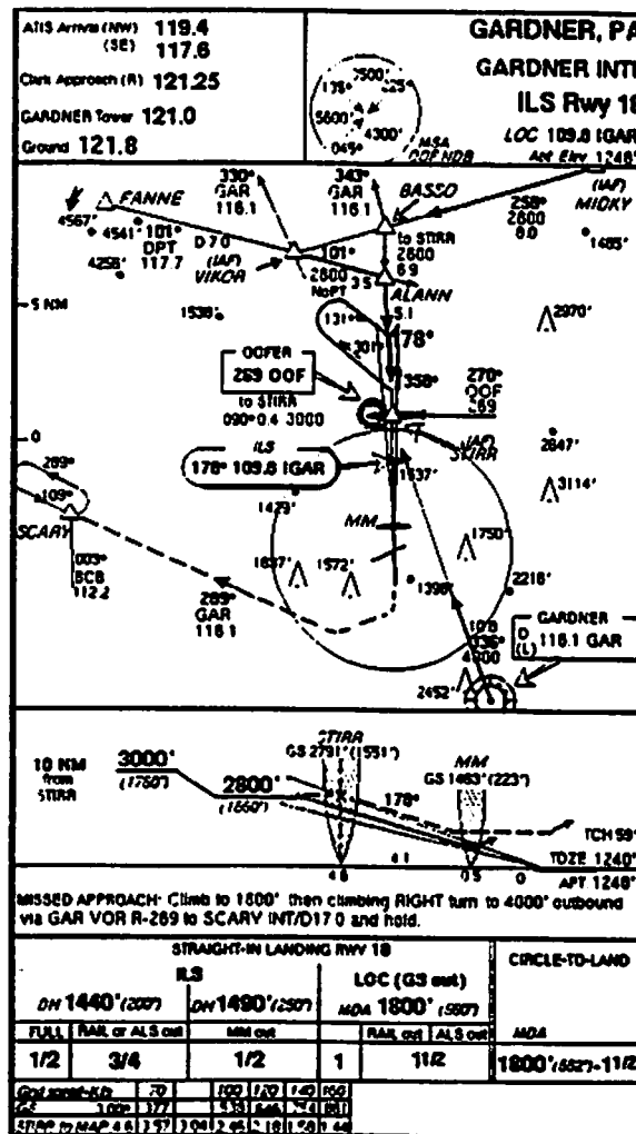
Figure 4.1 Example Format 1 IAP
