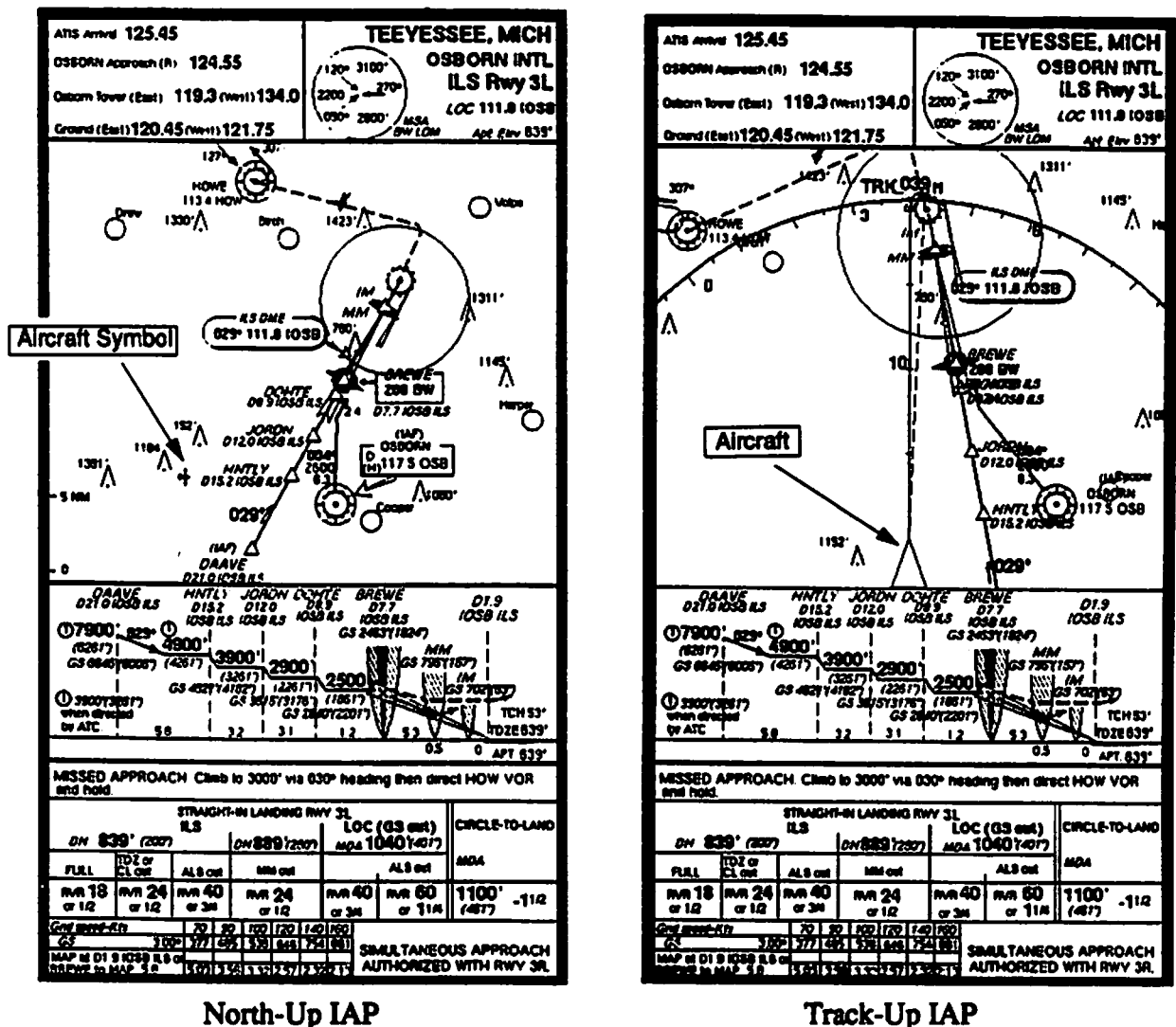
Figure 4.2 Example Format 2 IAPs
