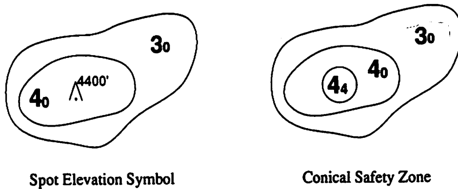
Figure 2.8 Depiction of Point Obstructions in Contour Charts
