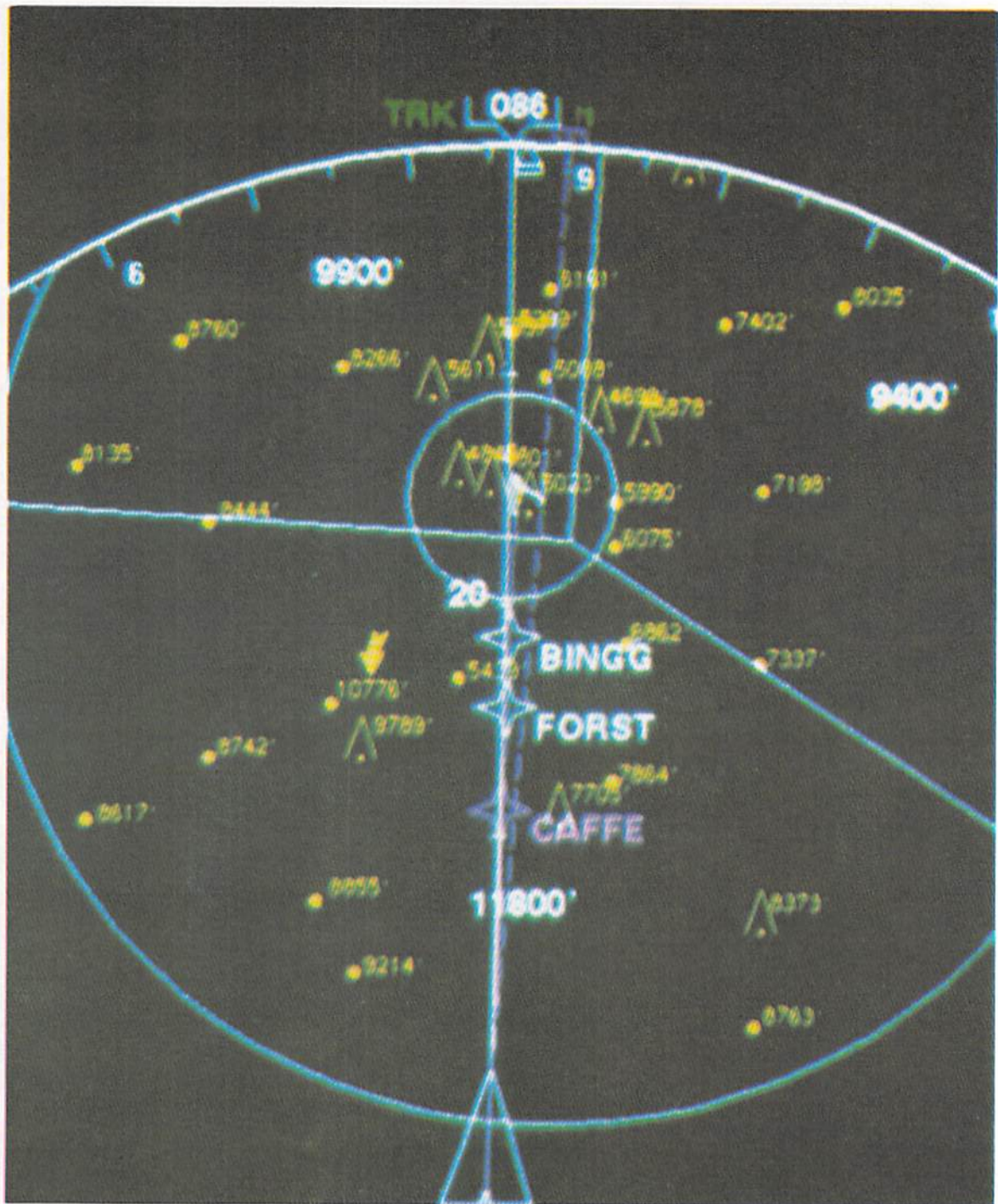
Figure 5.1 Prototypical Spot Elevation Display
