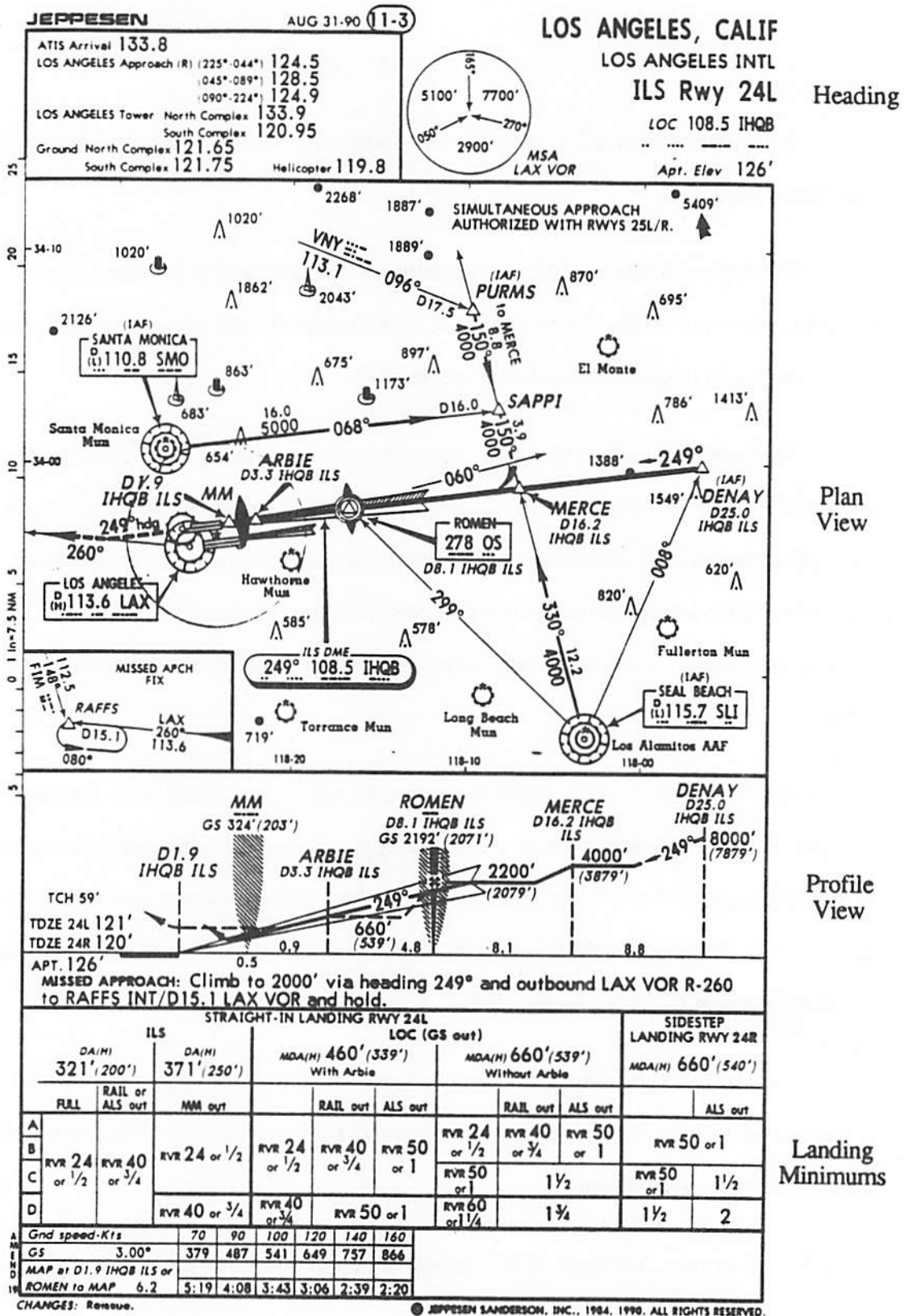
Figure 2.1 Example Instrument Approach Plate Reproduced with permission of Jeppesen Sanderson, Inc.
