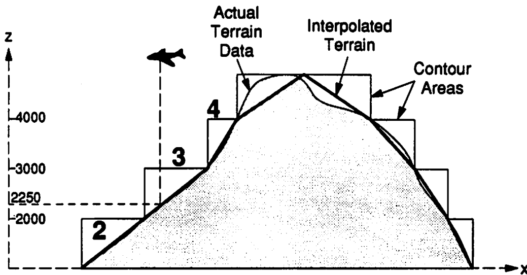
Figure 3.3 Terrain Altitude Interpolation
