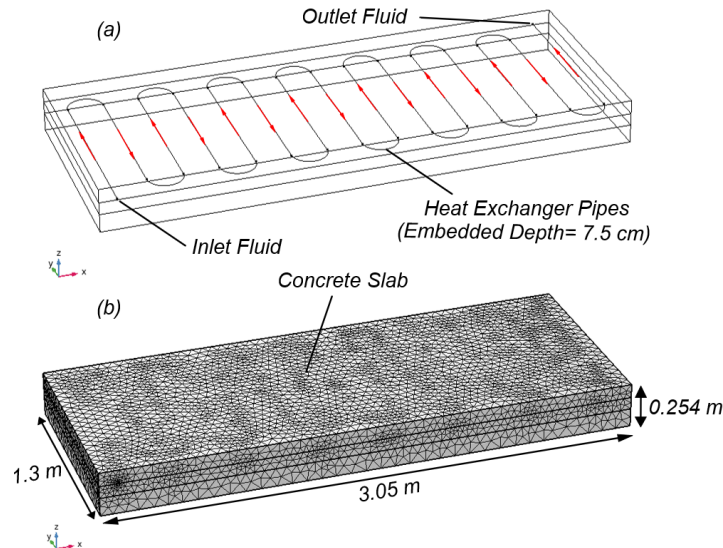
Figure 87. (a) The bridge deck model configuration, (b) Meshed 3D model
