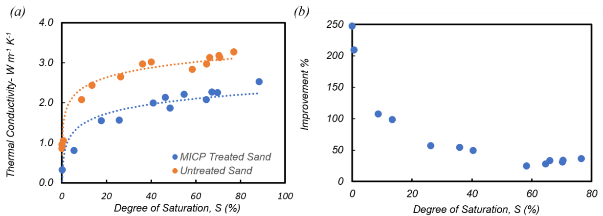
Figure 50(a), the influence of water content on thermal conductivity is most pronounced at lower saturation levels. As saturation increases, the rate of conductivity increase slows for both treated and untreated soils. At higher degrees of saturation, within the capillary and funicular regimes, thermal conductivity is primarily governed by particle-to-particle contact and the presence of continuous water films, while the influence of residual air voids becomes negligible (Likos, 2015).
