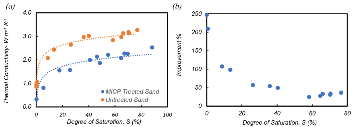
Figure 50(a) and (b) illustrate the variation in thermal conductivity across different degrees of saturation ( S ), ranging from 0% to 100%, for both untreated and bio-treated soil specimens. Since the thermal conductivity of water is significantly higher than that of air, an increase in water content enhances heat flow through the soil, resulting in higher overall thermal conductivity. Martinez et al. (2019) demonstrated that the thermal conductivity of a dry soil specimen ( S = 0 ) increased by 860% upon full saturation. As shown in
