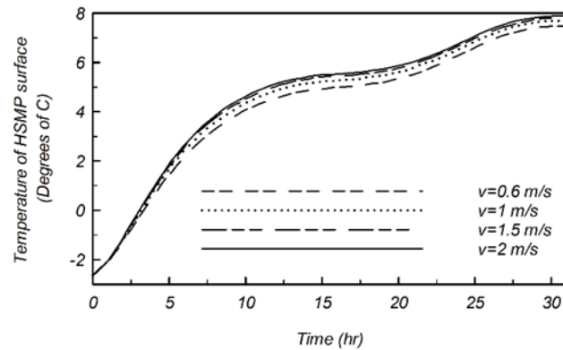
Figure 58. Surface temperature with variation of inlet flow rate (Feng & Yin, 2019)
