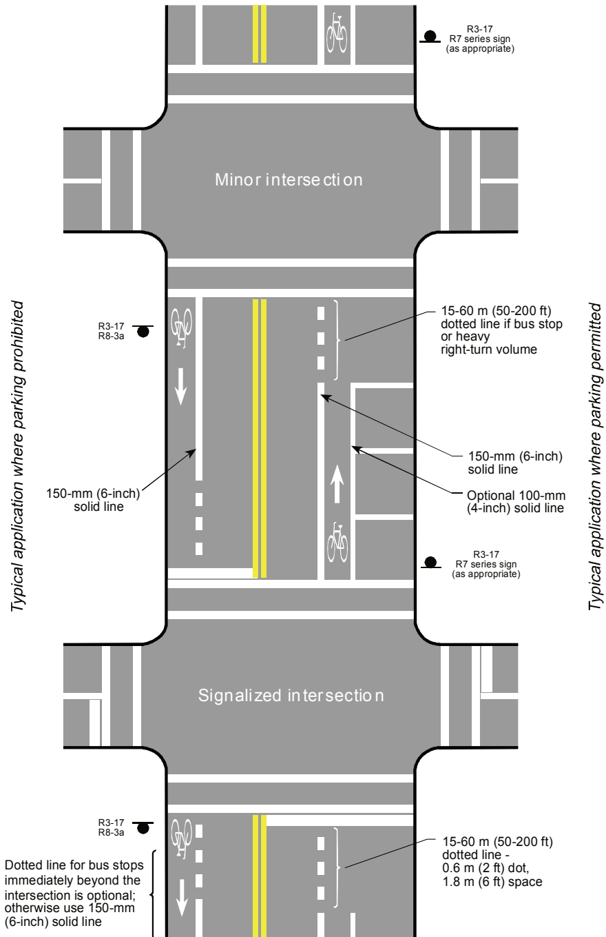
Figure 15-10. Illustration. Typical pavement markings for bike lane on two-way street. Source: American Association of State Highway and Transportation Officials (1)
