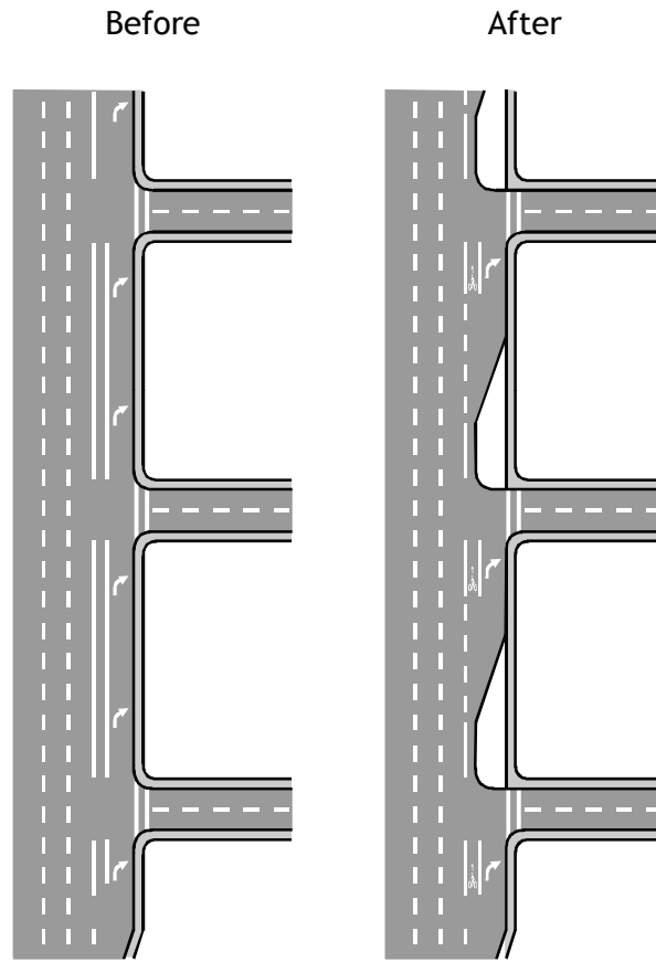
Figure 15-24. Illustration. Reconfiguration of a continuous right-turn lane to be bicycle-friendly. Source: Oregon Bicycle and Pedestrian Plan (3)
