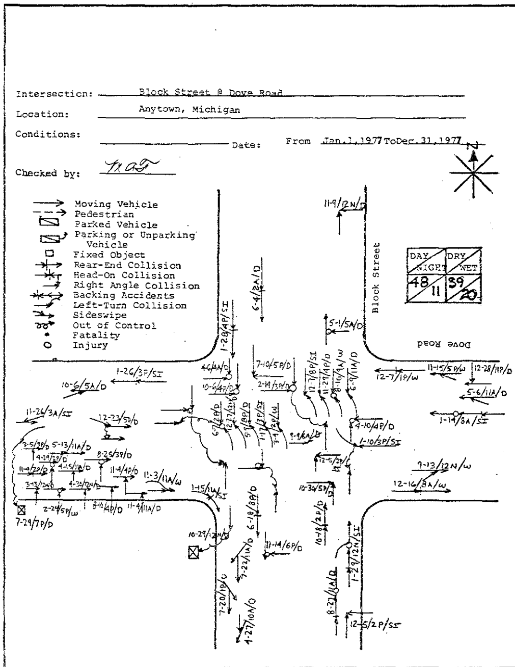
Figure 14. Collision diagram (example) - 1977.
