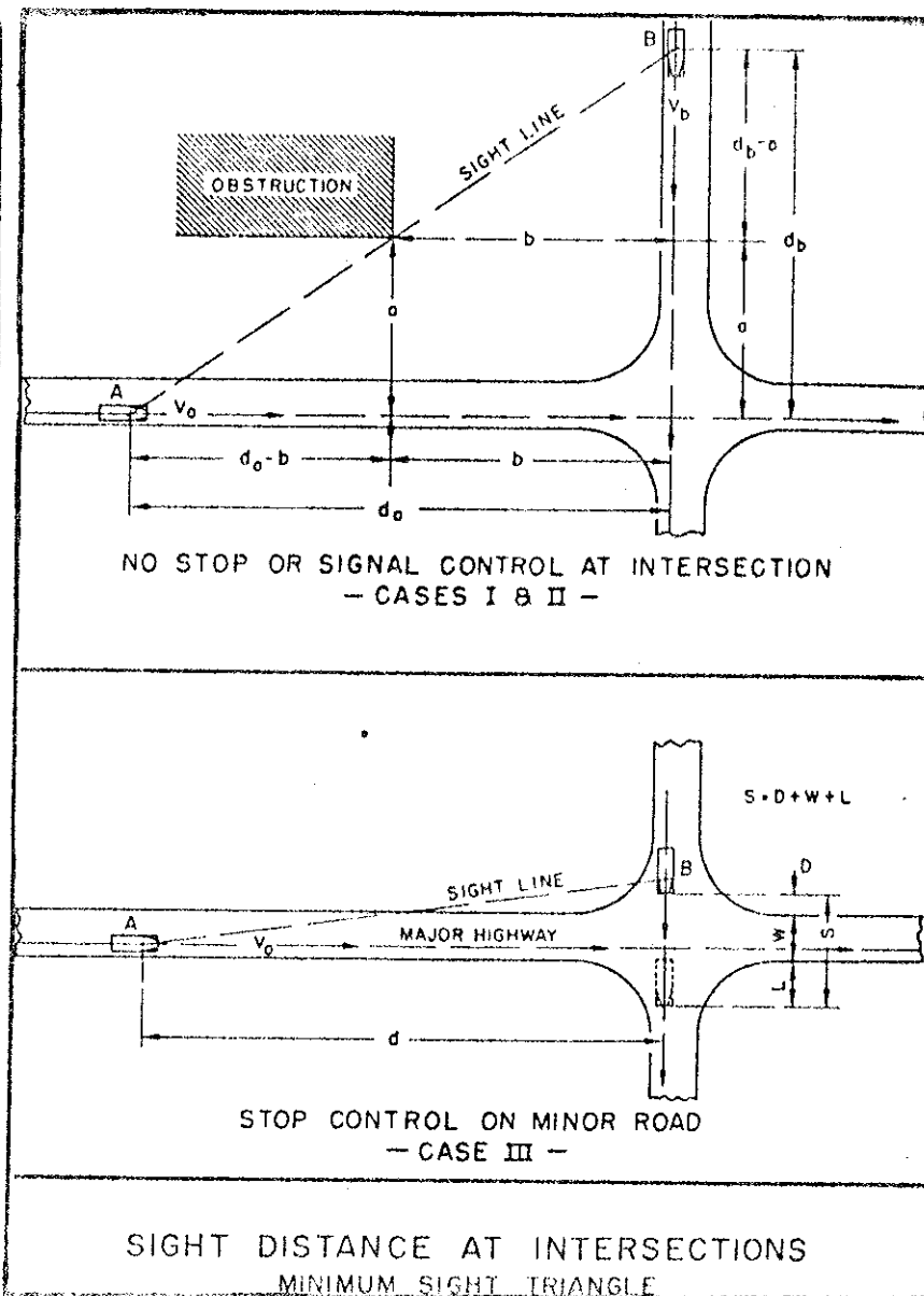
Figure 38. Intersection sight triangles.
