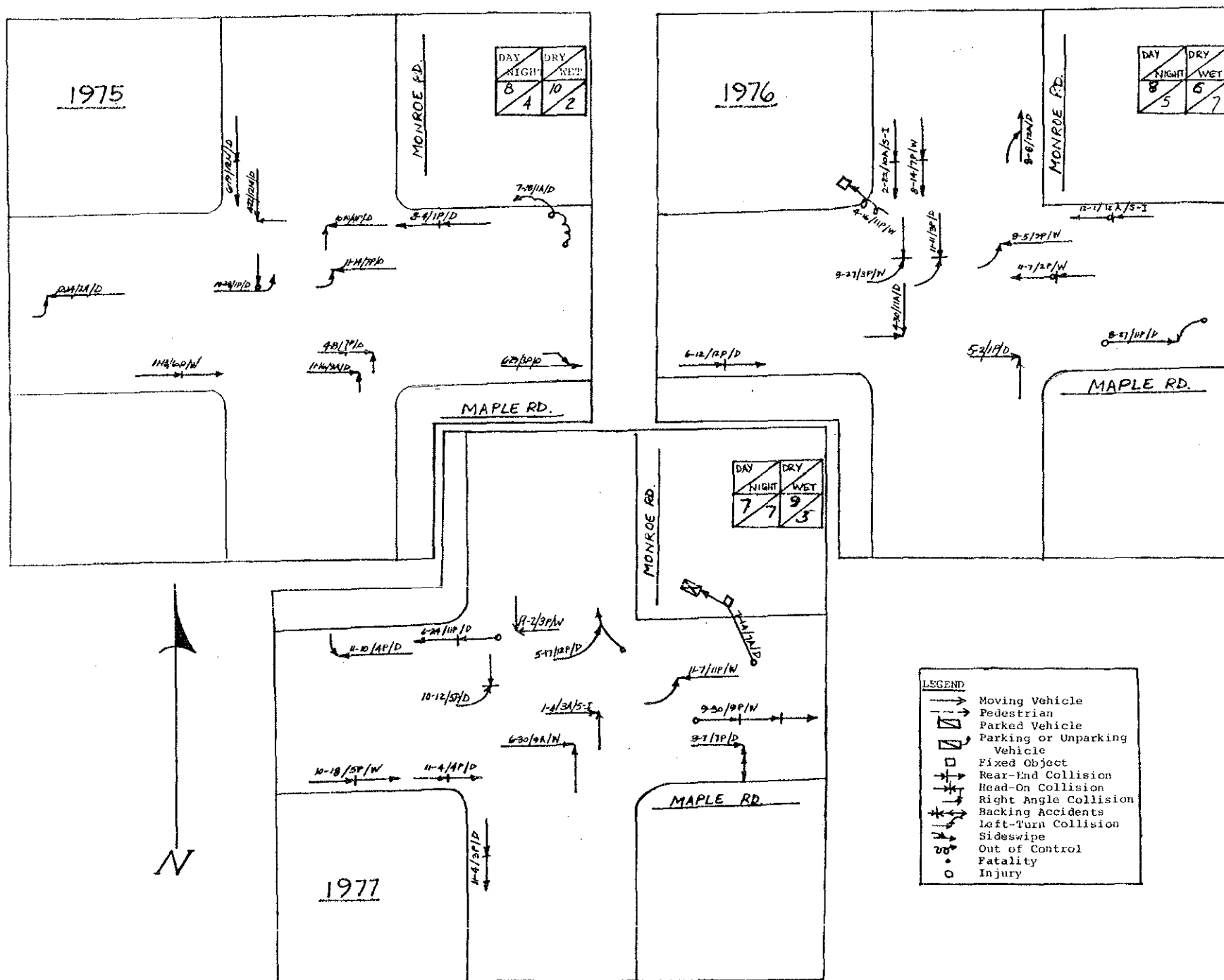
Figure J . Accident collision diagrams.
