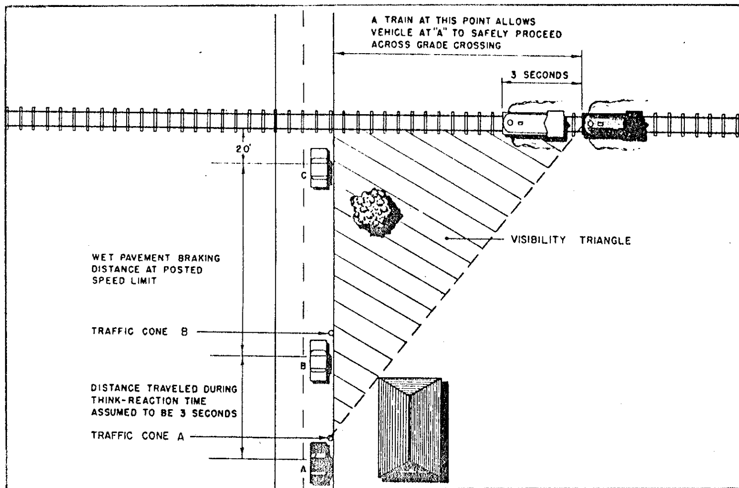
Figure 55. Sight distance check points at rail-highway crossings.
