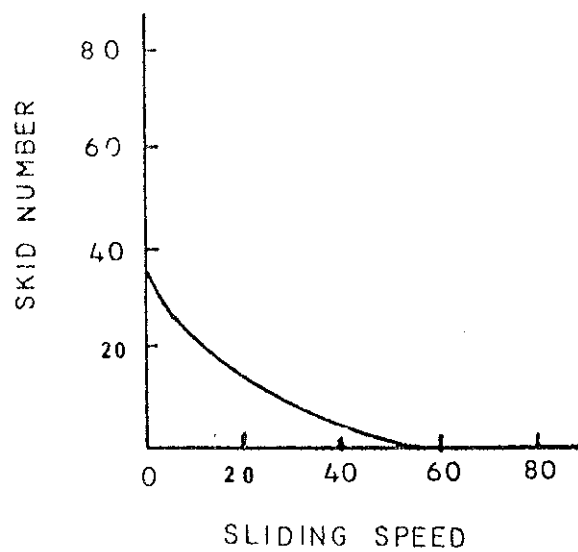
Figure 43. Skid resistance vs. vehicle speed.
