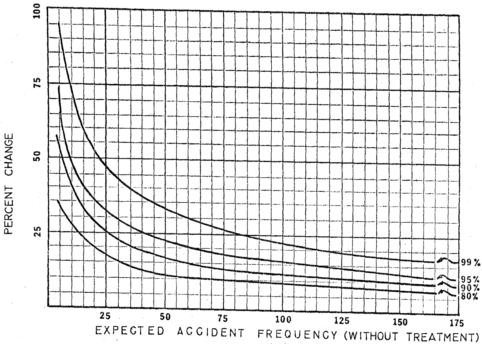
Figure S-11 Poisson Curves
