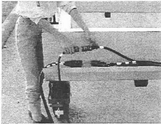
Figure 11.5 Connecting Cables
