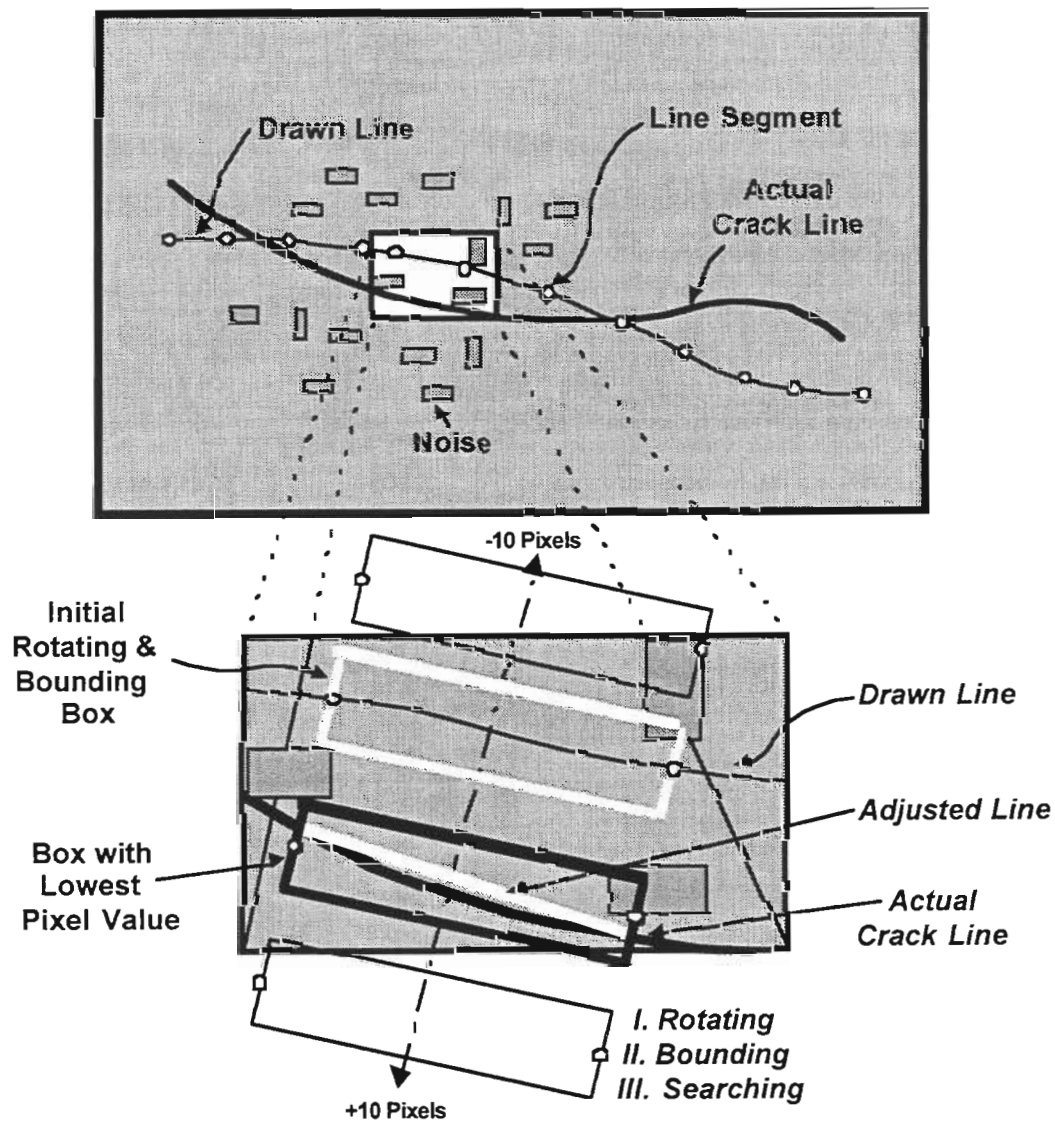
Figure 10.1 Illustration of Rotating & Bounding Box Algorithm
