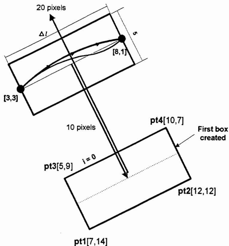
Figure 10.4 Create_Bounding_Box Function
