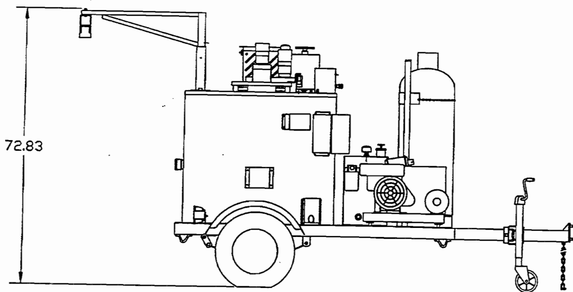
Figure 12.6 Crafcro Super Shot 60 Propane Melter Drawing (Side View)
