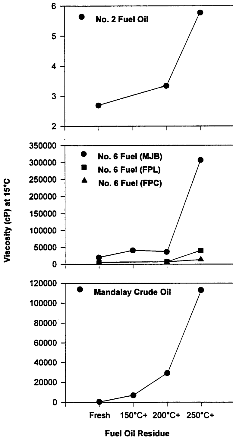
Figure 3-5. Viscosity of fuel oil residues at 15°C.
