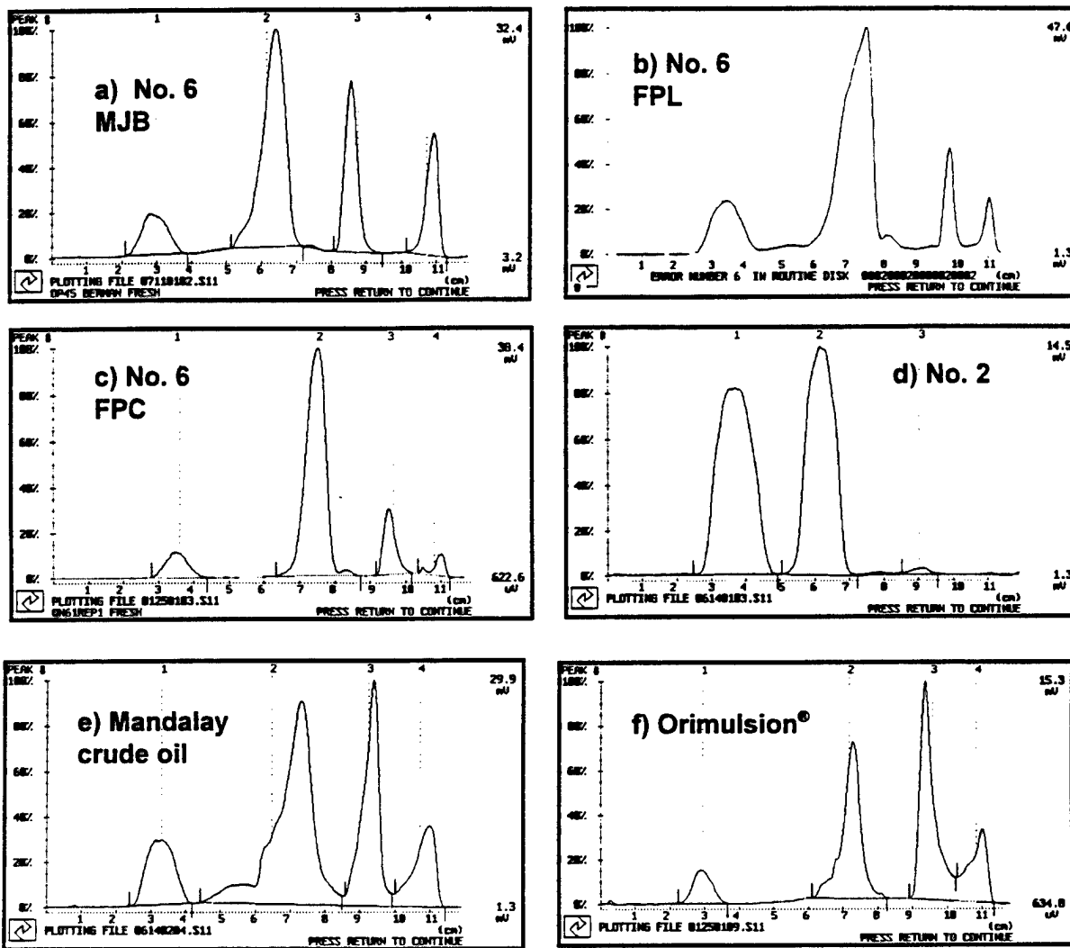
Figure 3-8. Iatroscan chromatograms of a) No. 6 fuel oil ( Morris J. Berman cargo oil), b) No. 6 fuel oil Florida Power and Light Corporation, c) No. 6 fuel oil Florida Power Corporation, d) No. 2 fuel oil, e) Mandalay crude oil, and f) Orimulsion®.
