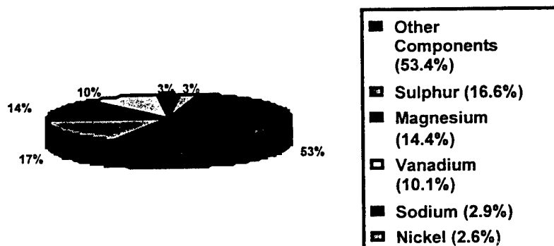
Figure 1. Summary of ash composition elemental analysis.
