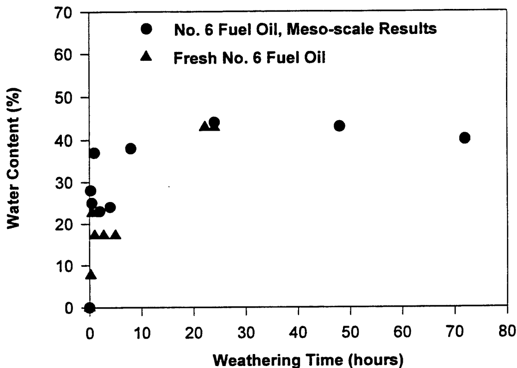
Figure 3-12. Water content of water-in-oil emulsion as a function of weathering state.
