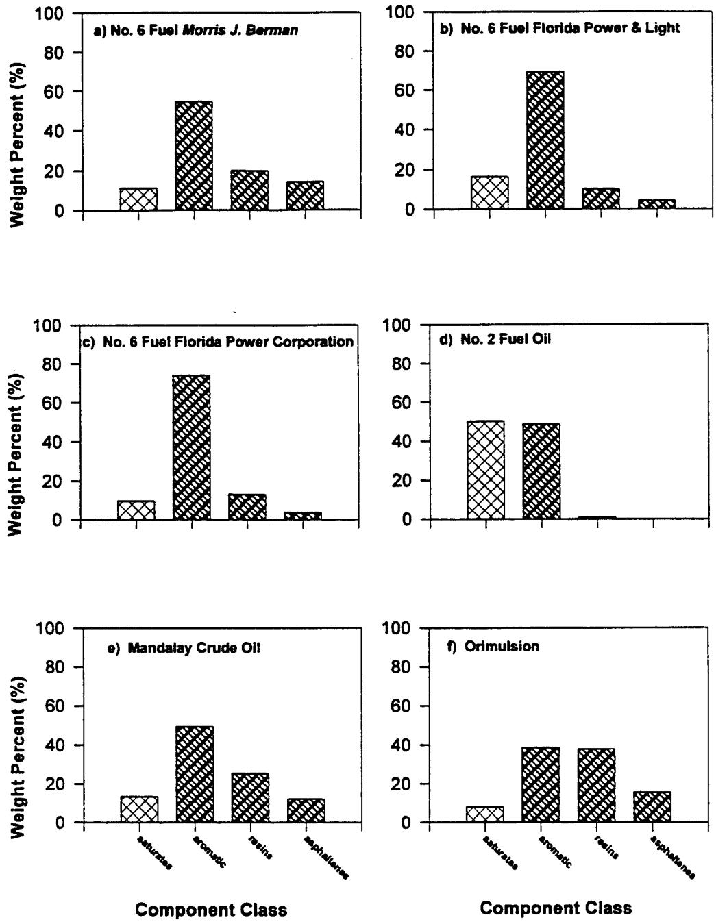
Figure 3-9. Histograms of the component class analysis for fuel oils.
