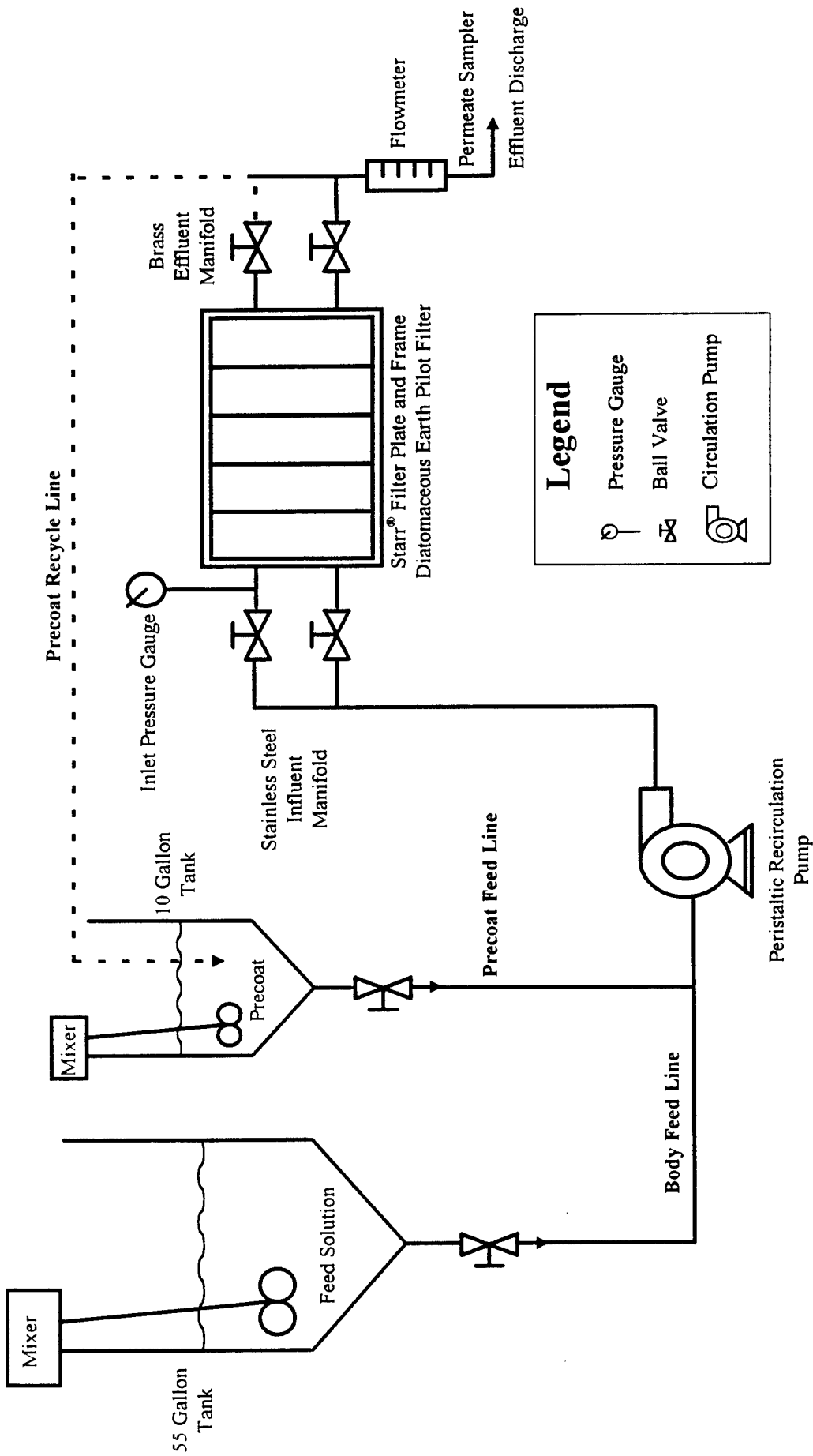
Figure 3. Schematic diagram of diatomaceous earth plate and frame pilot filter.
