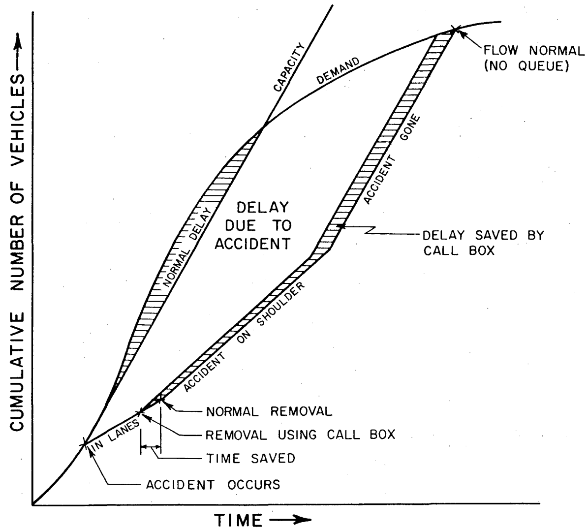
FIGURE 9. RELATIONSHIP OF FLOW CAPACITY AND DELAY.
