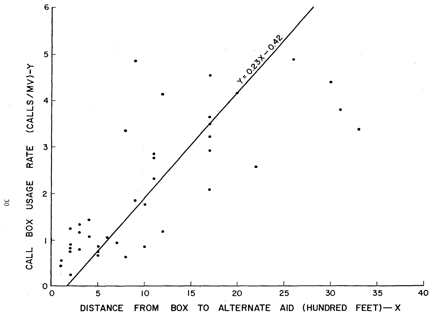
FIGURE 7. RELATIONSHIP OF CALL BOX USAGE TO DISTANCE TO ALTERNATE AID.
