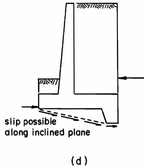
FIG. 8 - Possible Slip Surfaces Beneath Footing
