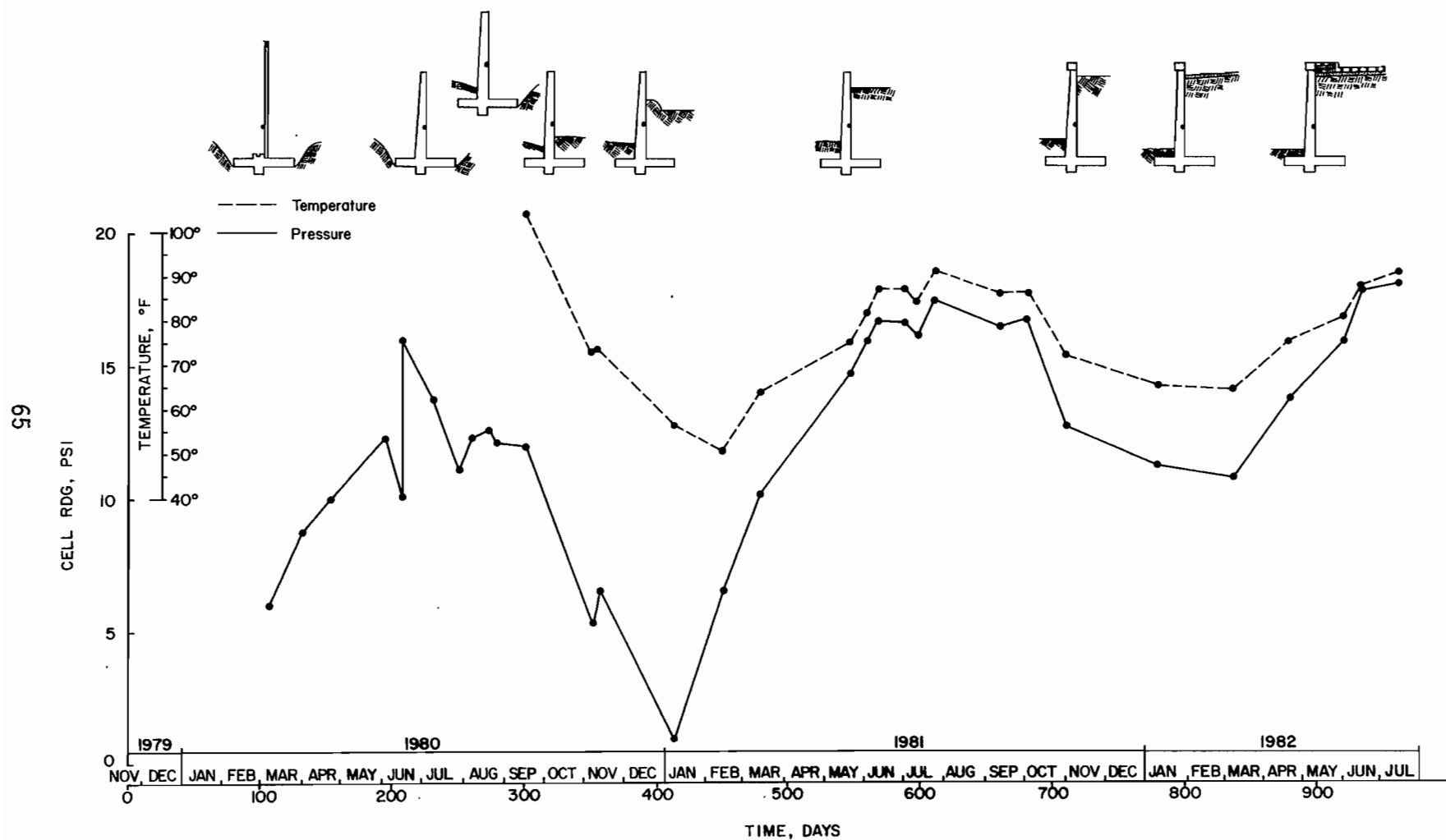
FIG. 25 - Cell 927: Pressure, Temperature, Backfill Measurements ( ^{\circ}\text{C} = 0.56 (^{\circ}\text{F} - 32) , 1 \text{ psi} = 6.89 \text{ kPa} )
