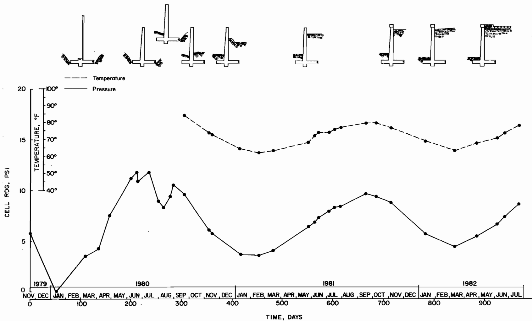
FIG. 27 - Cell 924: Pressure, Temperature, Backfill Measurements ( ^{\circ}\text{C} = 0.56 (^{\circ}\text{F} - 32) , 1 \text{ psi} = 6.89 \text{ kPa} )
