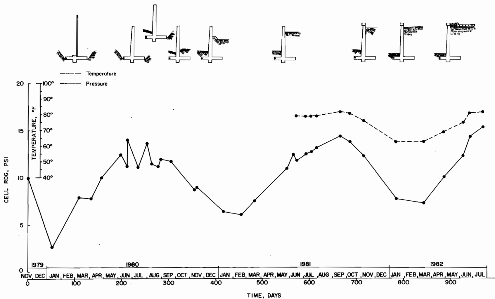
FIG. 28 - Cell 935: Pressure, Temperature, Backfill Measurements ( ^{\circ}\text{C} = 0.56 (^{\circ}\text{F} - 32) , 1 \text{ psi} = 6.89 \text{ kPa} )
