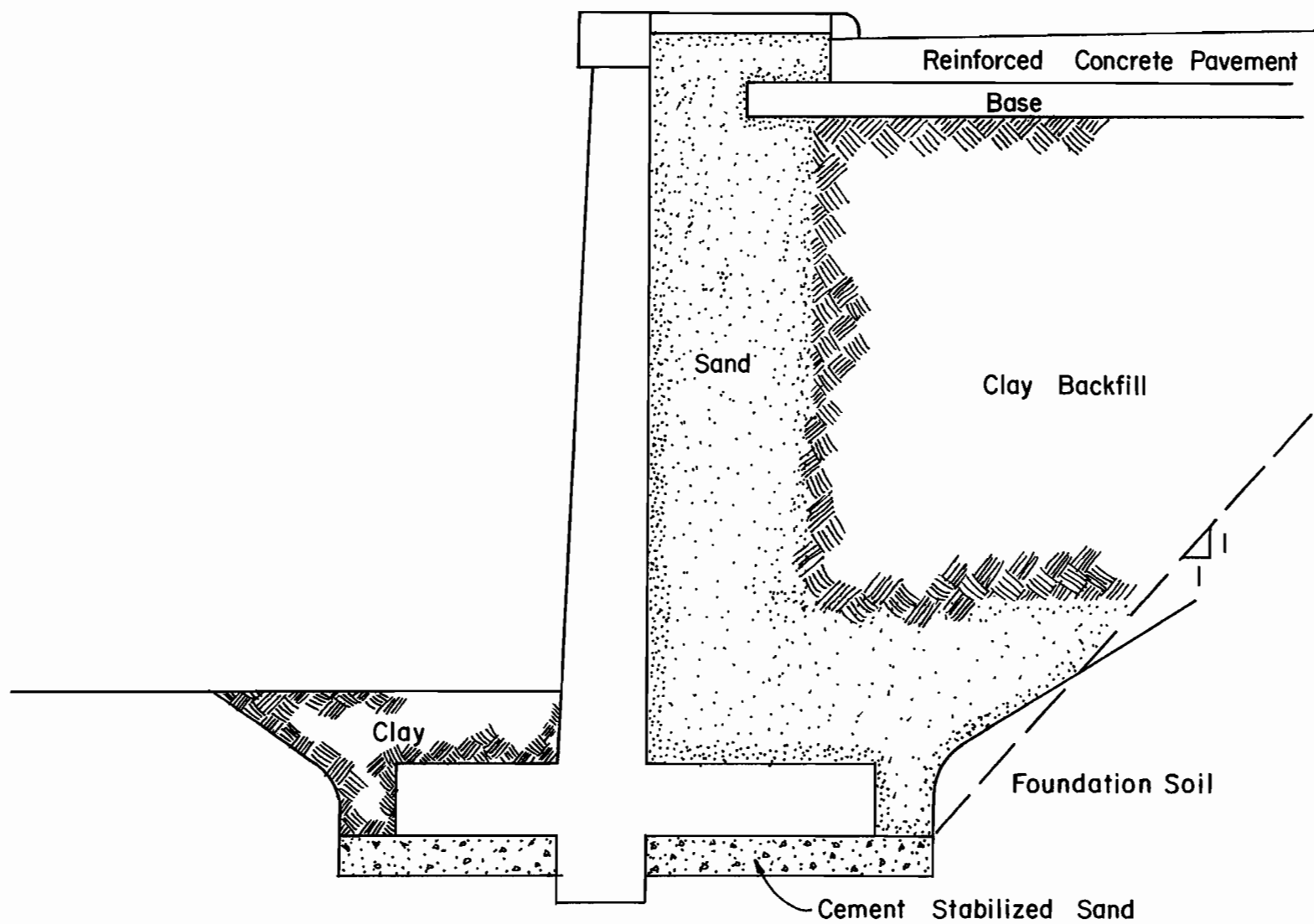
FIG. 17 - As-Built Profile
