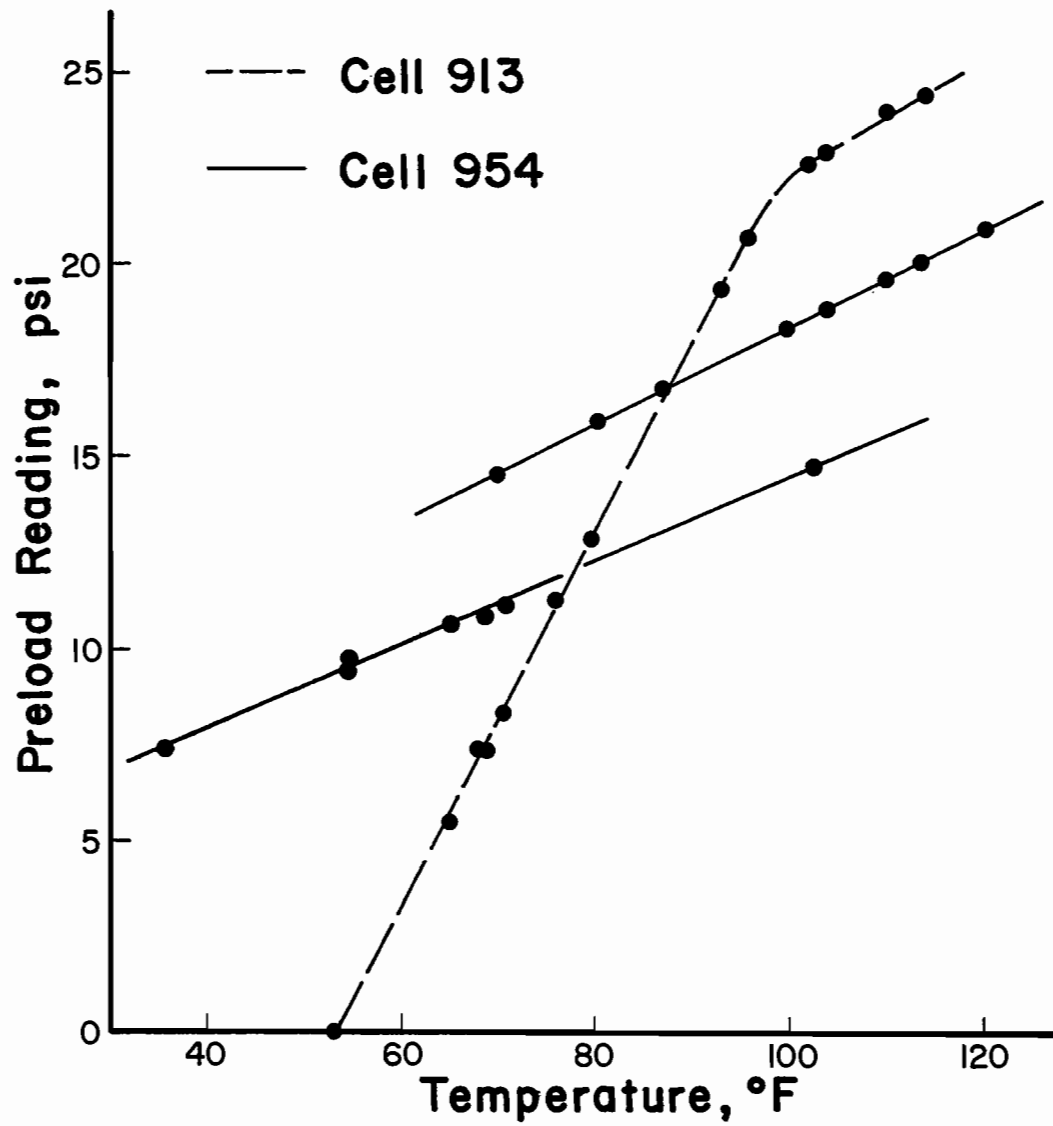
FIG. 35 - Laboratory Temperature-Preload Relationship ( ^{\circ}\text{C} = 0.56 (^{\circ}\text{F} - 32) , 1 psi = 6.89 kPa)
