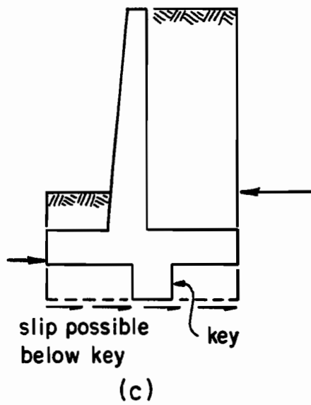
FIG. 8 - Possible Slip Surfaces Beneath Footing
