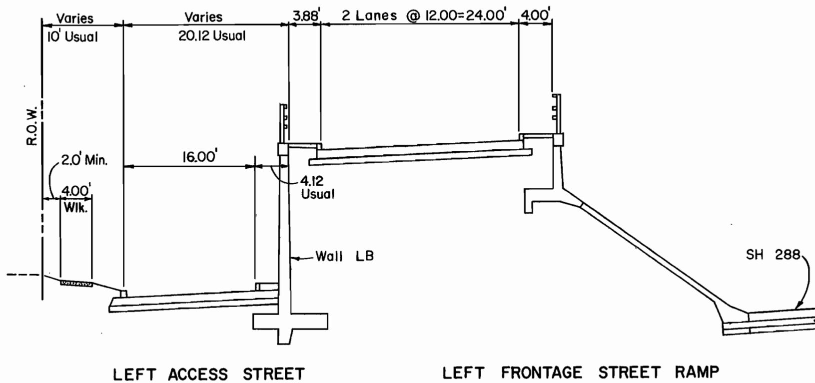
FIG. 10 - Typical Section at Test Panel (1 ft = 0.305 m)
