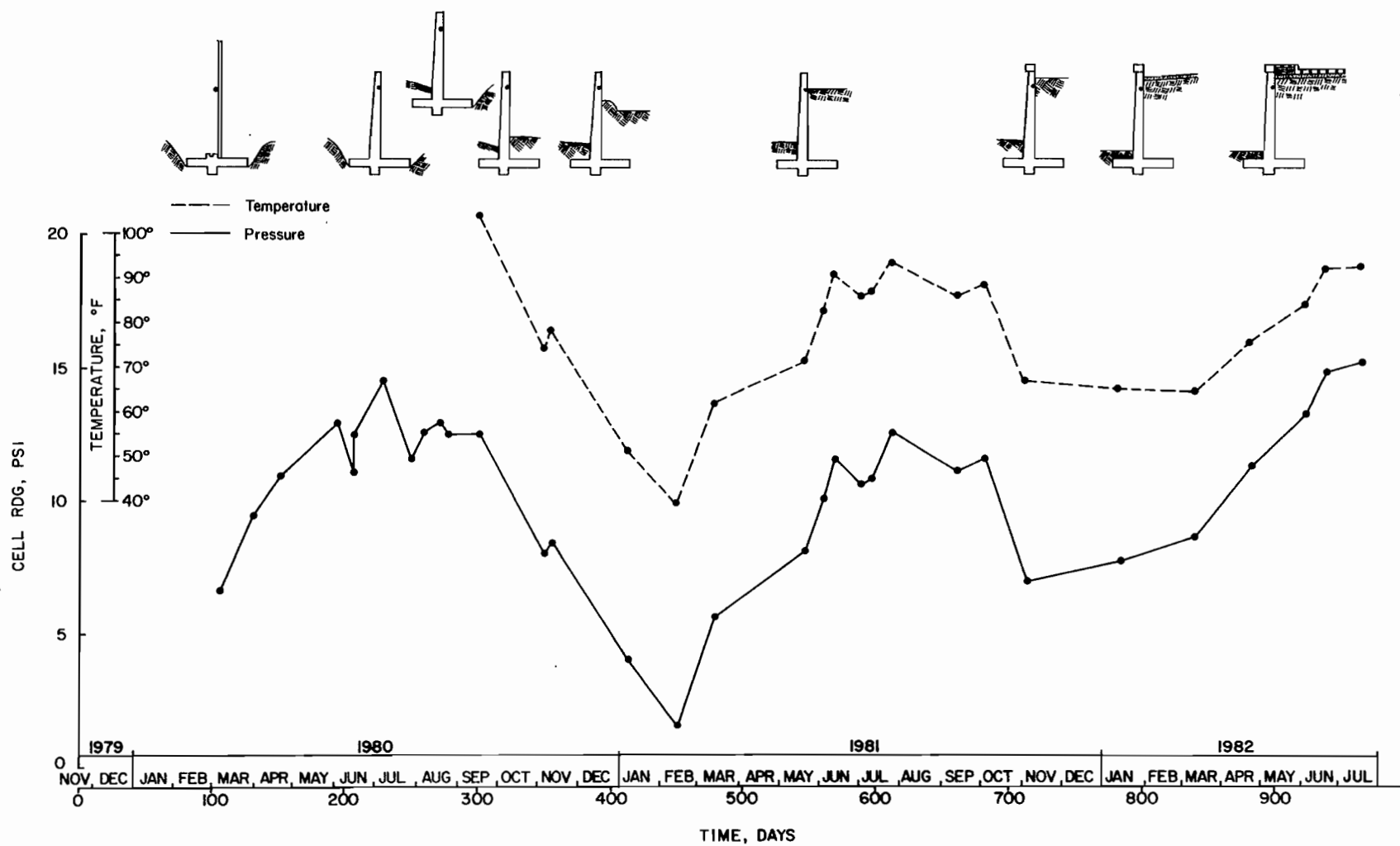
FIG. 23. - Cell 930: Pressure, Temperature, Backfill Measurements ( ^{\circ}\text{C} = 0.56 (^{\circ}\text{F} - 32) , 1 \text{ psi} = 6.89 \text{ kPa} )
