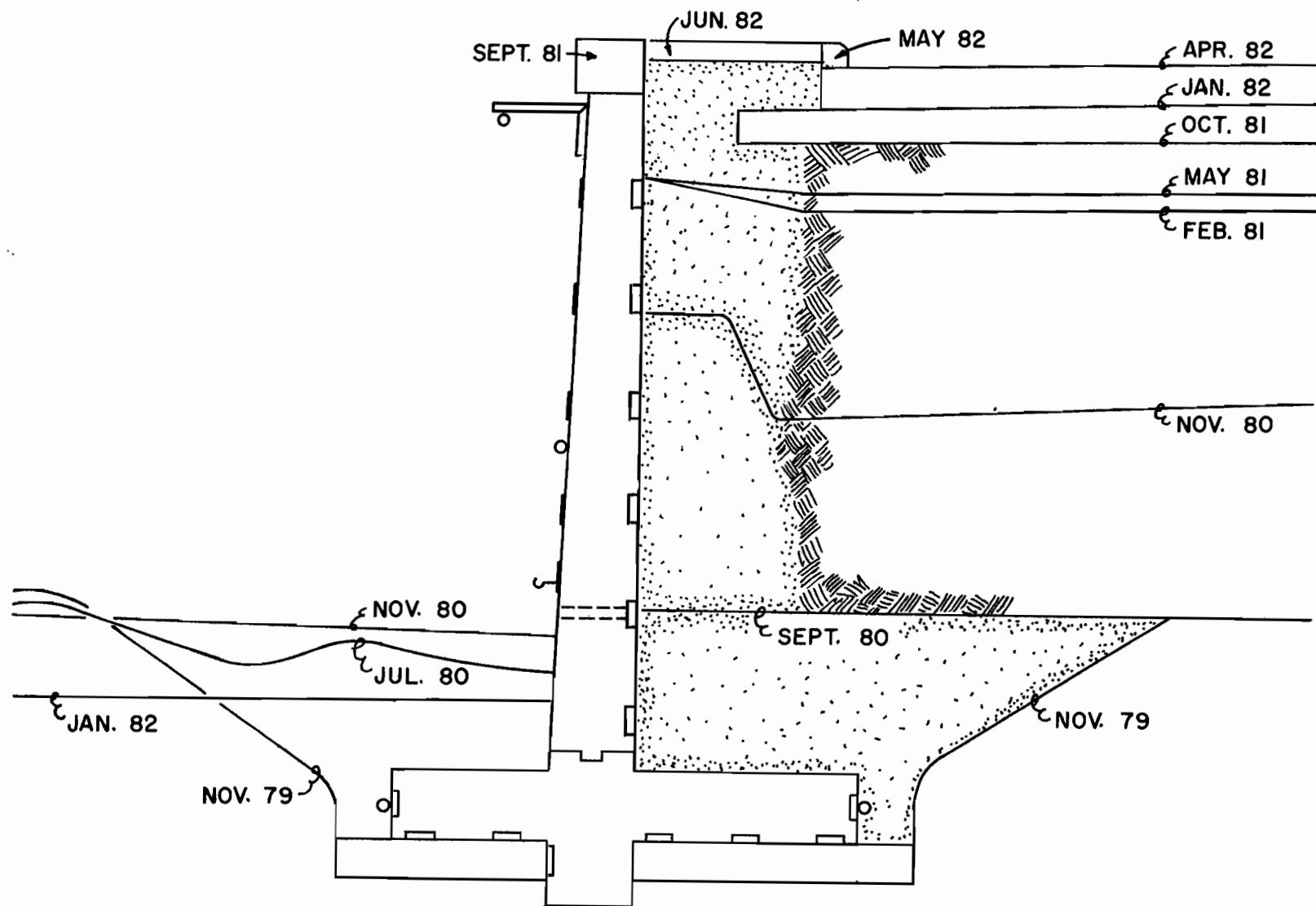
FIG. 22 - Construction Sequence
