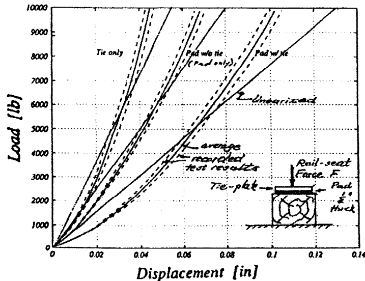
Figure 16. Test Results for Manufactured Pad and/or Tie
