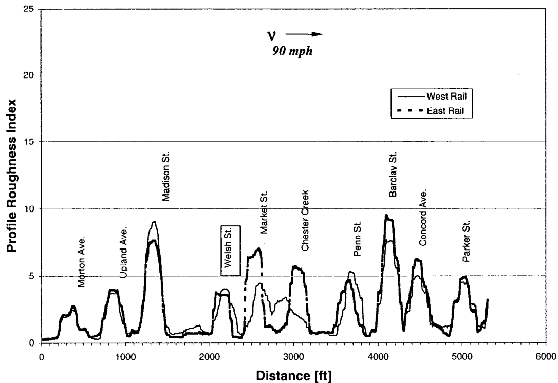
Figure 24. R^2 - Profile Plots for the Chester Station Bridges Before Pad Installation (MP13-MP14, Track No. 3, June 1996)
