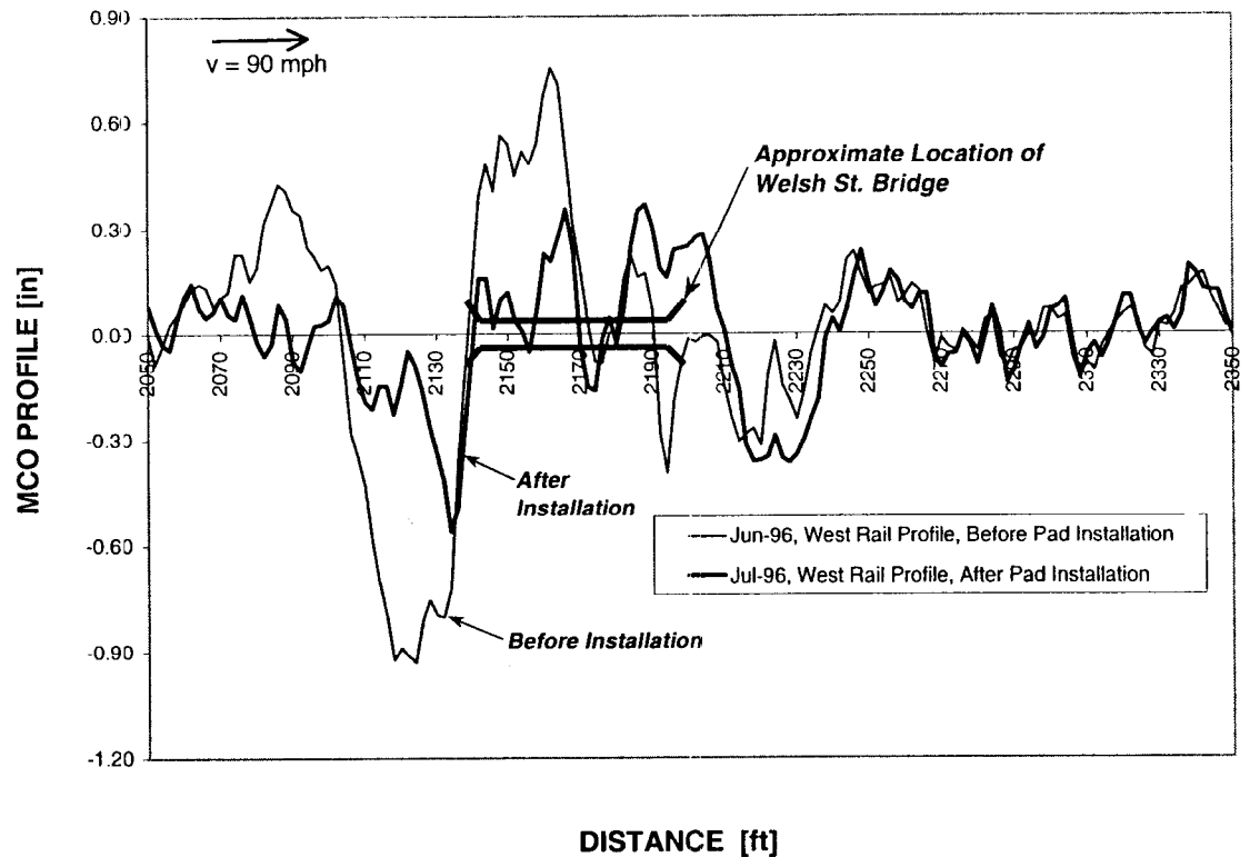
Figure 18. Effect of Matched Pads on West Rail Profile of Track No. 3 of Welsh Street Bridge (near Chester, Pennsylvania Station)
