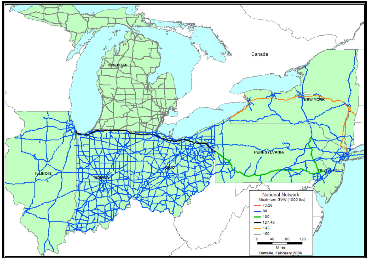
Figure 2-4. Single Trailer Gross Vehicle Weight Limits in Corridor
