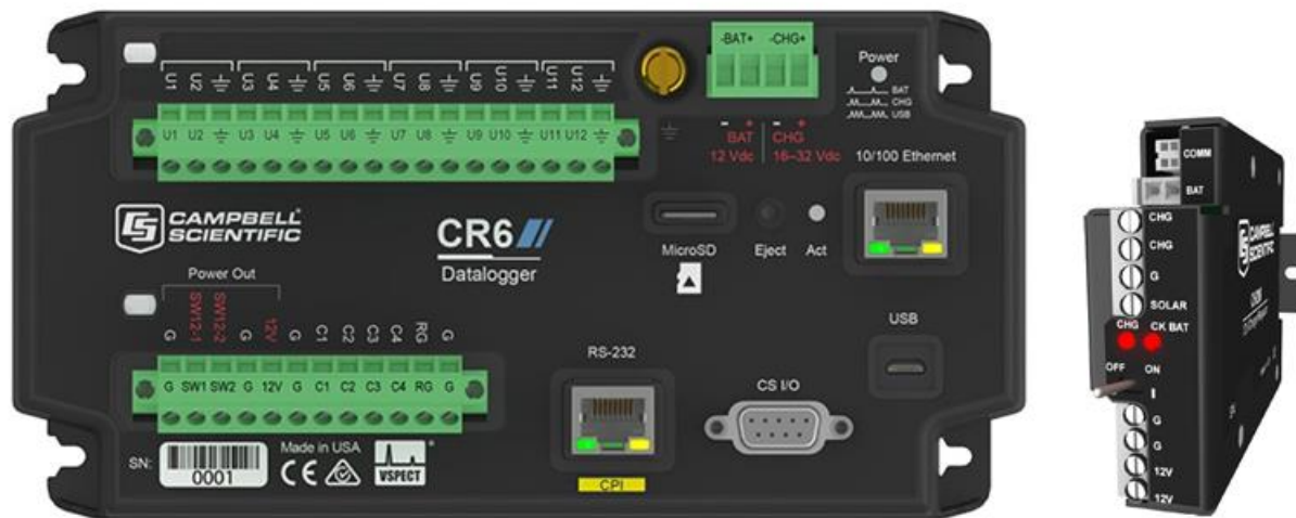
Figure 54. CR6 datalogger and CH200 charging regulator (source: campbellsci.com)
