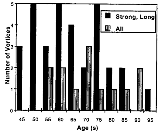
Figure 21 Age Distribution
