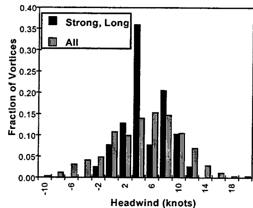
Figure 17. Headwind Distribution
