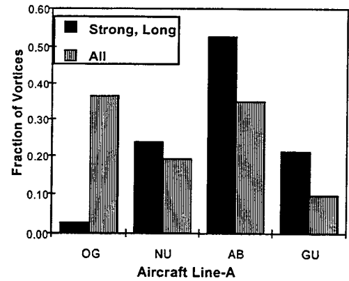
Figure 20. Aircraft Line-A Attitude Distribution
