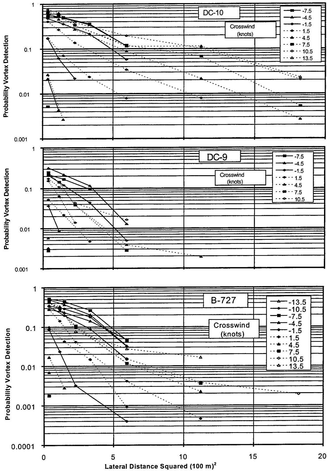
Figure 8. Dependence of GWSS Takeoff Detection Probability on Lateral Distance Squared
