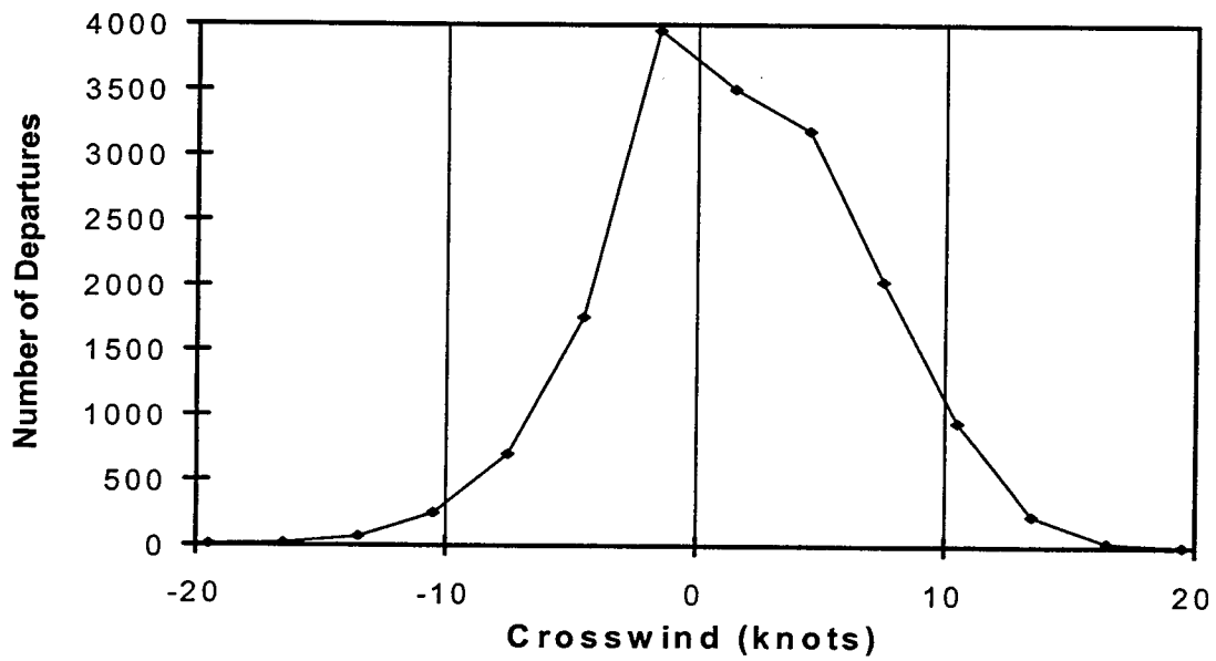
Figure 2. Crosswind Distribution for Departures
