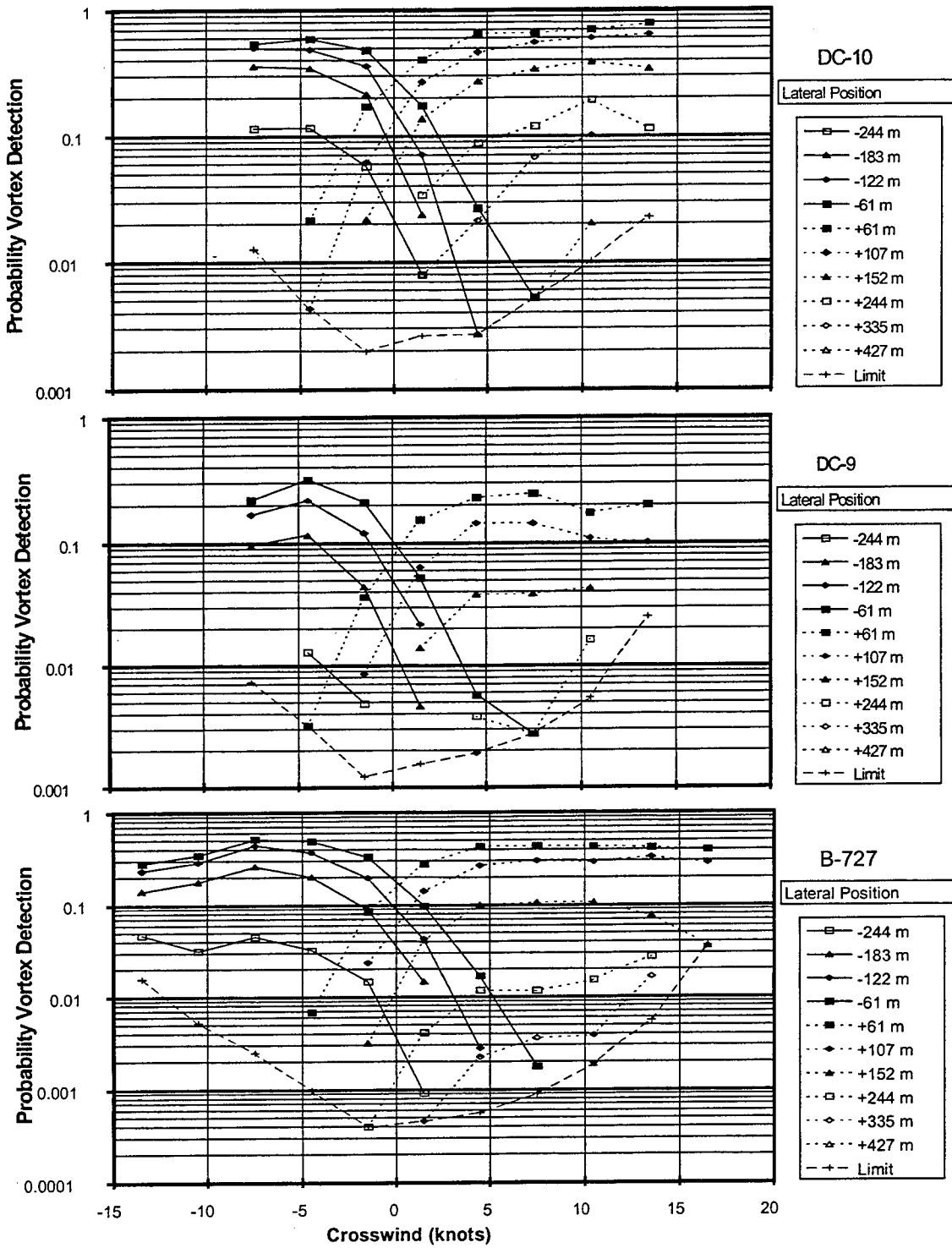
Figure 5. Dependence of GWSS Takeoff Detection Probability on Crosswind
