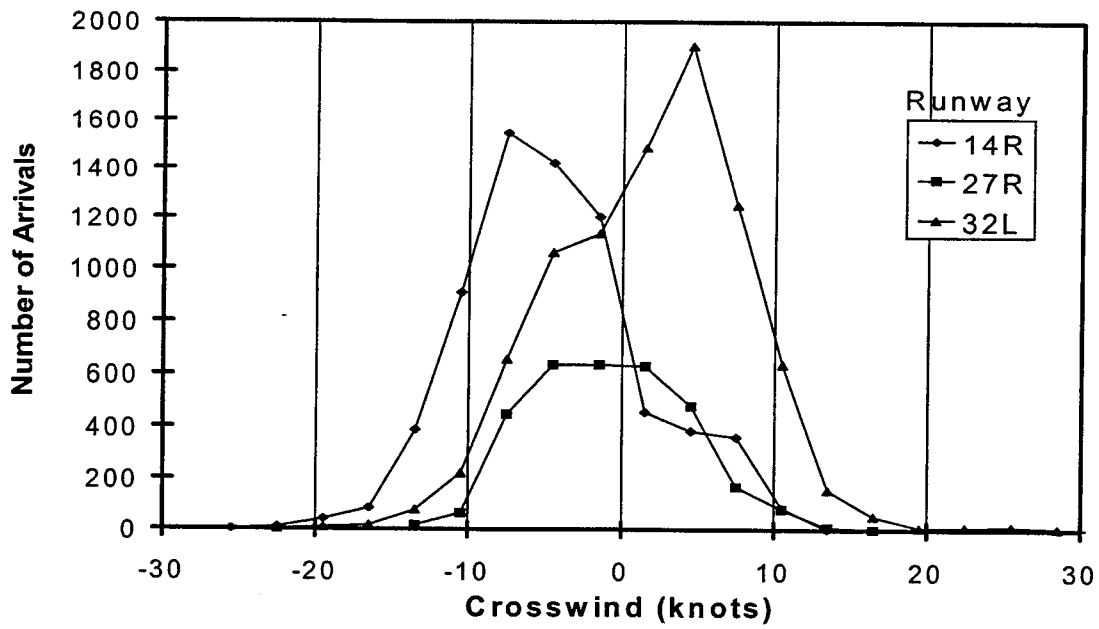
Figure 1. Crosswind Distribution for Arrivals
