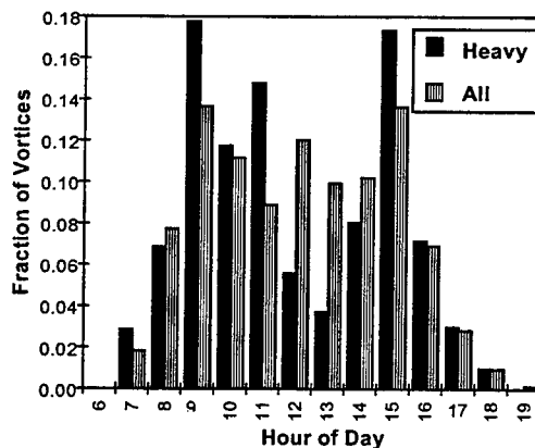
Figure 14. Comparison of Hour-of-Day Distribution for Heavy Departures and All Starboard-Side Cases
