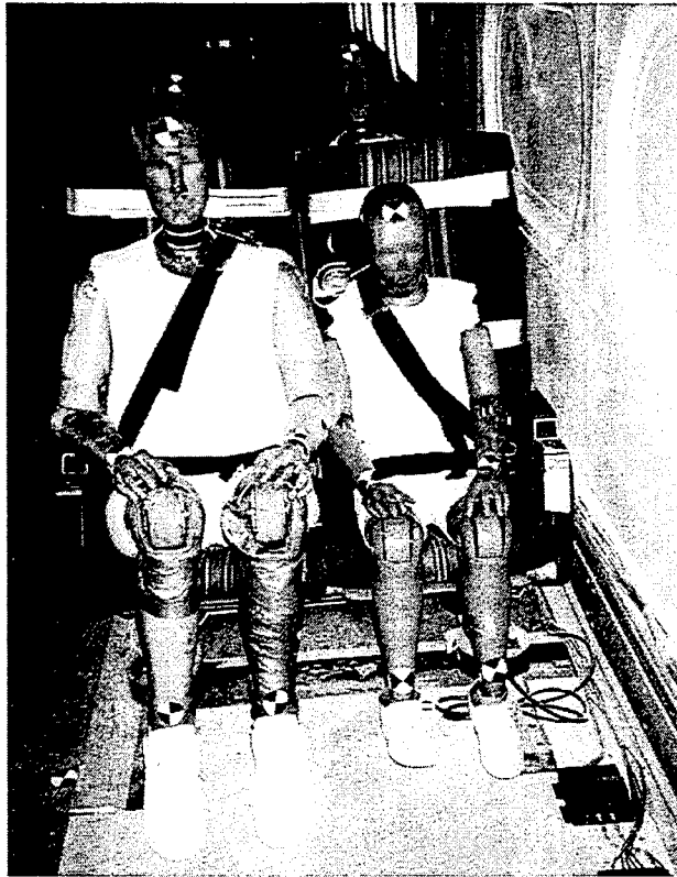
Figure 3. Pre-Test Photo of Experiment No. 2 – Row-to-Row Amtrak Seats with Restraints
