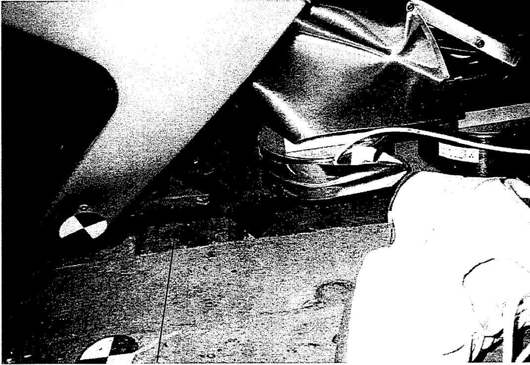
Figure 7. Experiment No. 1 – Front-Row Seat Pedestal Collapse and Seat Deformation
