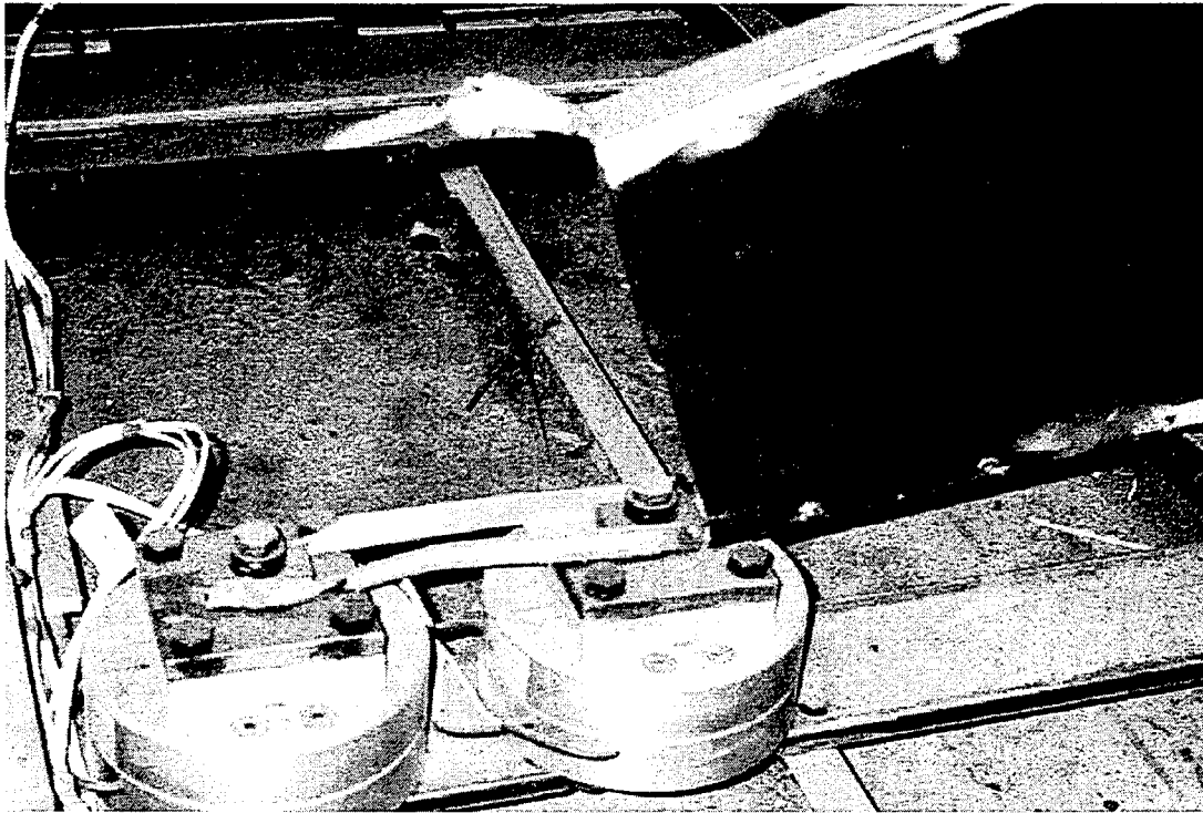
Figure 12. Experiment No. 3 – Seat Pedestal Sheared Near the Floor Attachment
