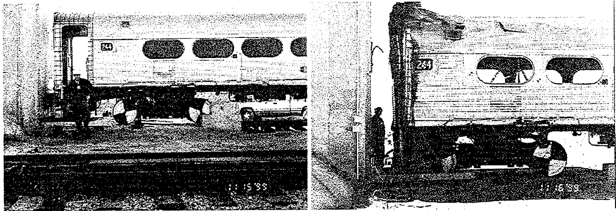
Figure 9. Pre-Test and Post-Test Photos of the Single-Car Test
