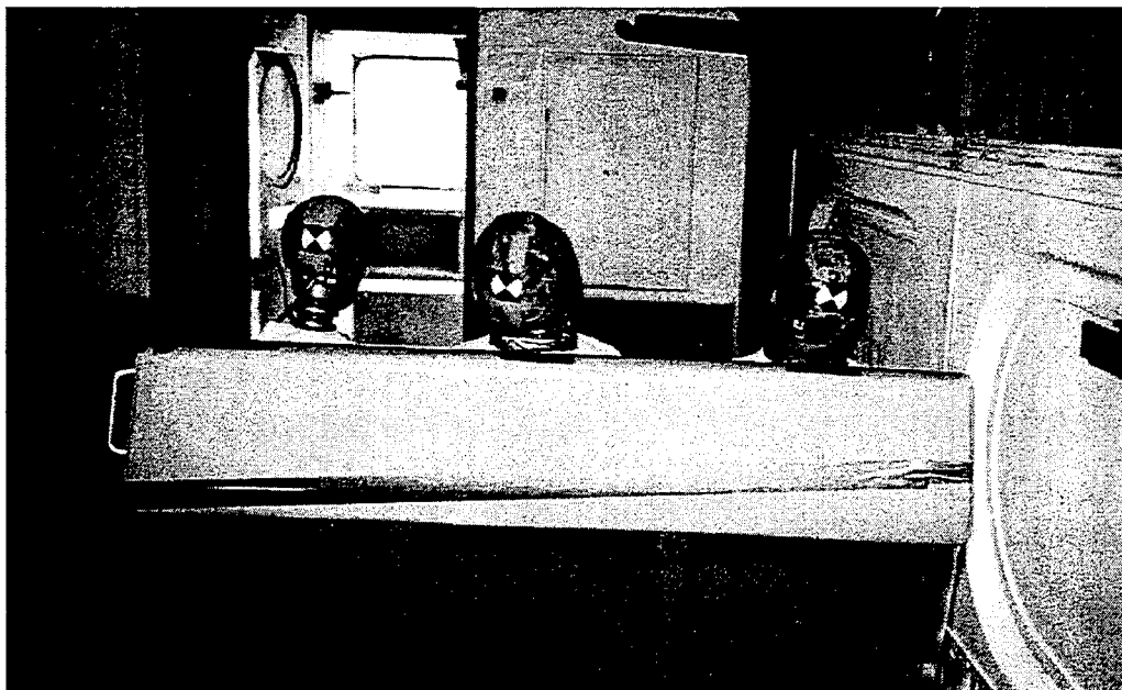
Figure 4. Pre-Test Photo of Experiment No. 3 – Rear-Facing Commuter Seat
