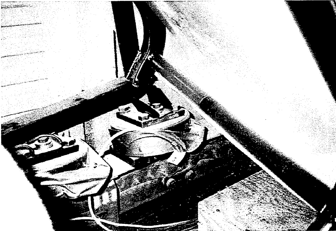
Figure 8. Experiment No. 1 – Front-Row Seat Frame Deformation and Weld Seam Failure
