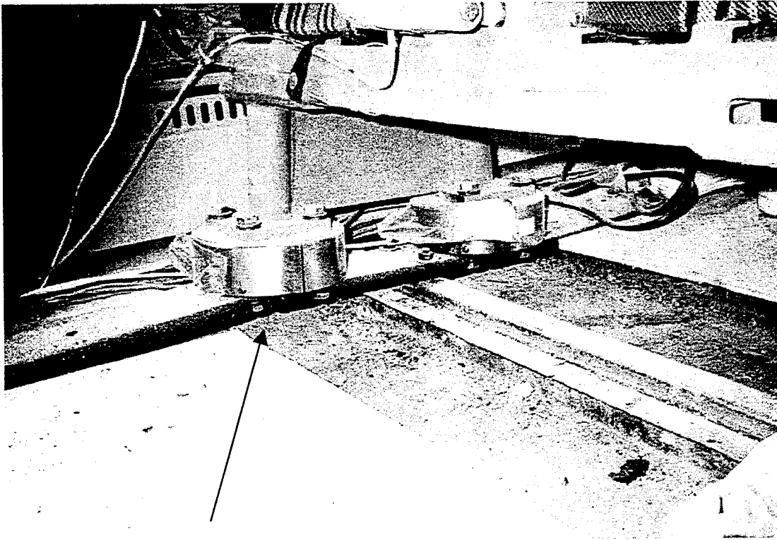
Figure 11. Experiment No. 2 – Metal Floor Attachment Bar Deformed Under Load
