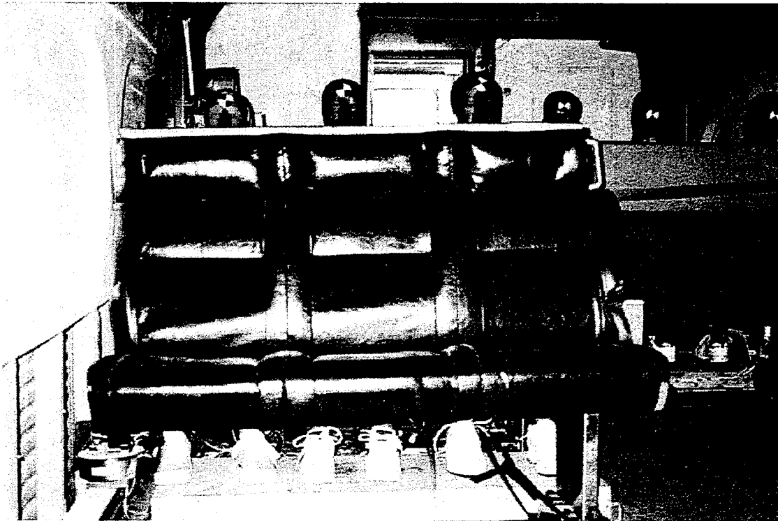
Figure 2. Pre-Test Photo of Experiment No. 1 – Row-to-Row Commuter Seats
