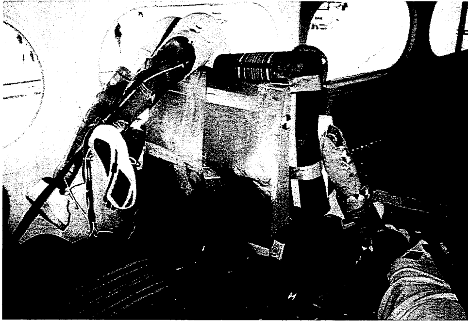
Figure 9. Experiment No. 2 – ATD Not Compartmentalized
