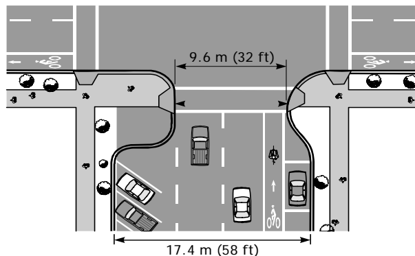
Figure 11-11. Illustration. Curb extensions improve the visibility of pedestrians by motorists and vice versa.
