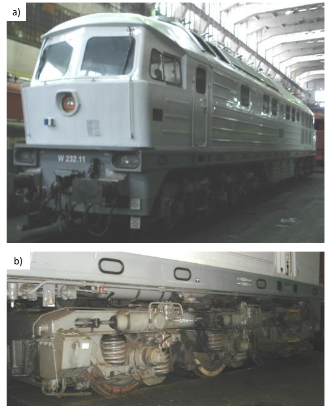
Fig. 1. View of the BR232 diesel locomotive – a), view of the bogie with the suspension system, power transmission and braking system – b)
