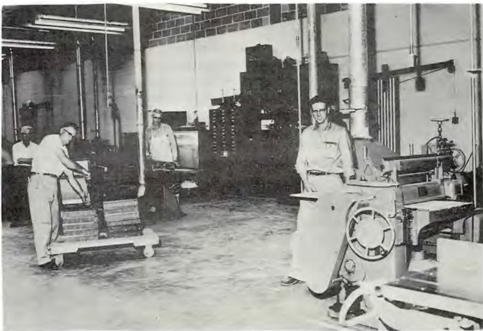
A PORTION of the Area "G" in the warehouse building where the Operations Section stores the wall panels for the pre-fabricated buildings that are used in most of the Air Navigation Facility sites. These panels are used to erect buildings which vary in length and width in multiples of four feet.
