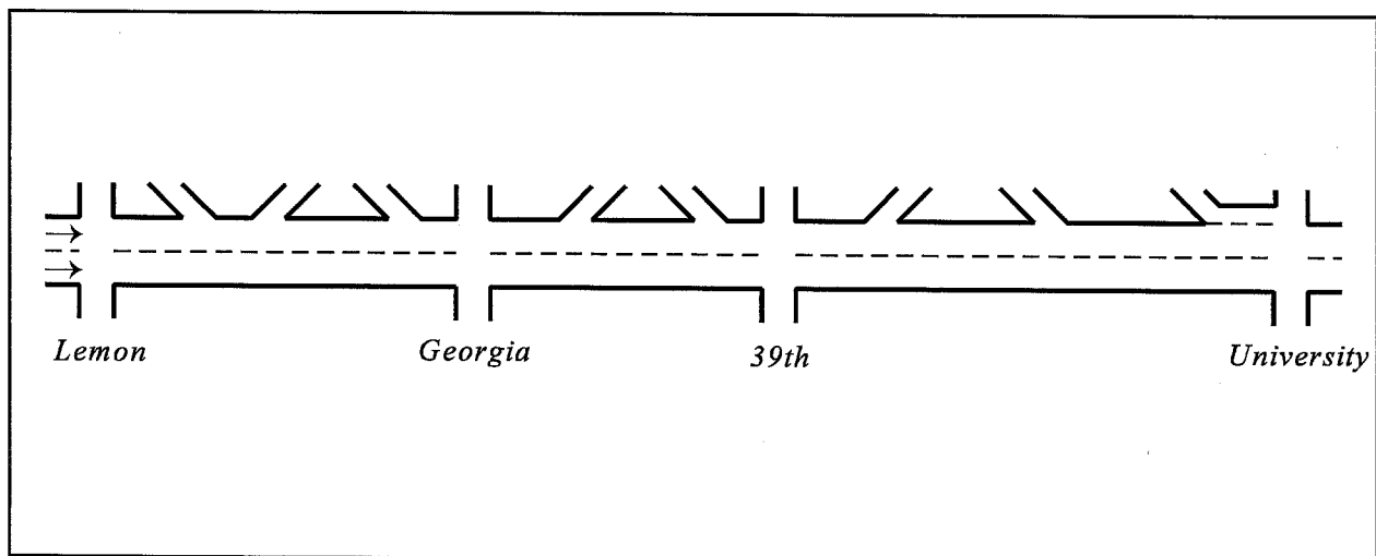
Figure 5-3. Schematic of One-Way Frontage Road Study Section.
